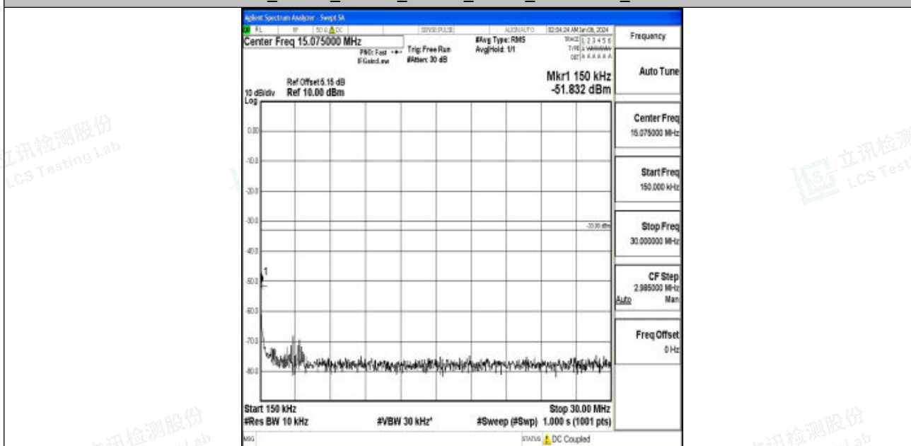
Band66_10MHz_16QAM_132322_1RB#0_0.15~30_0.15~30
