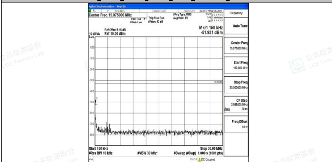
Band66_20MHz_16QAM_132072_1RB#0_0.15~30_0.15~30
