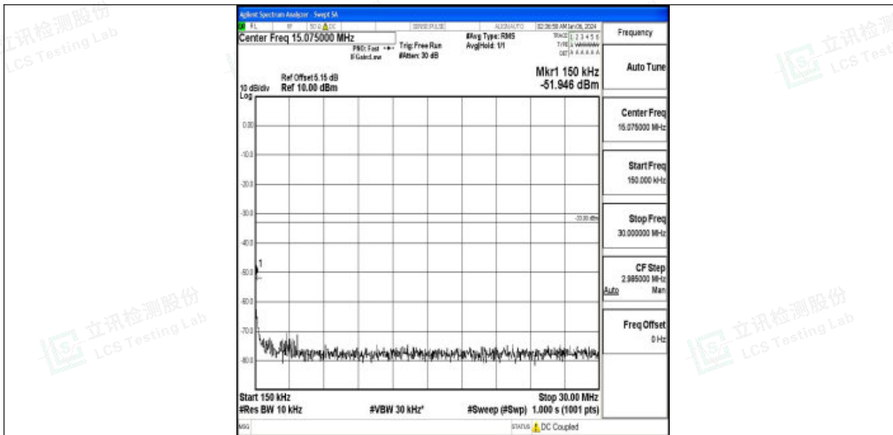
Band66_20MHz_QPSK_132572_1RB#0_0.15~30_0.15~30
