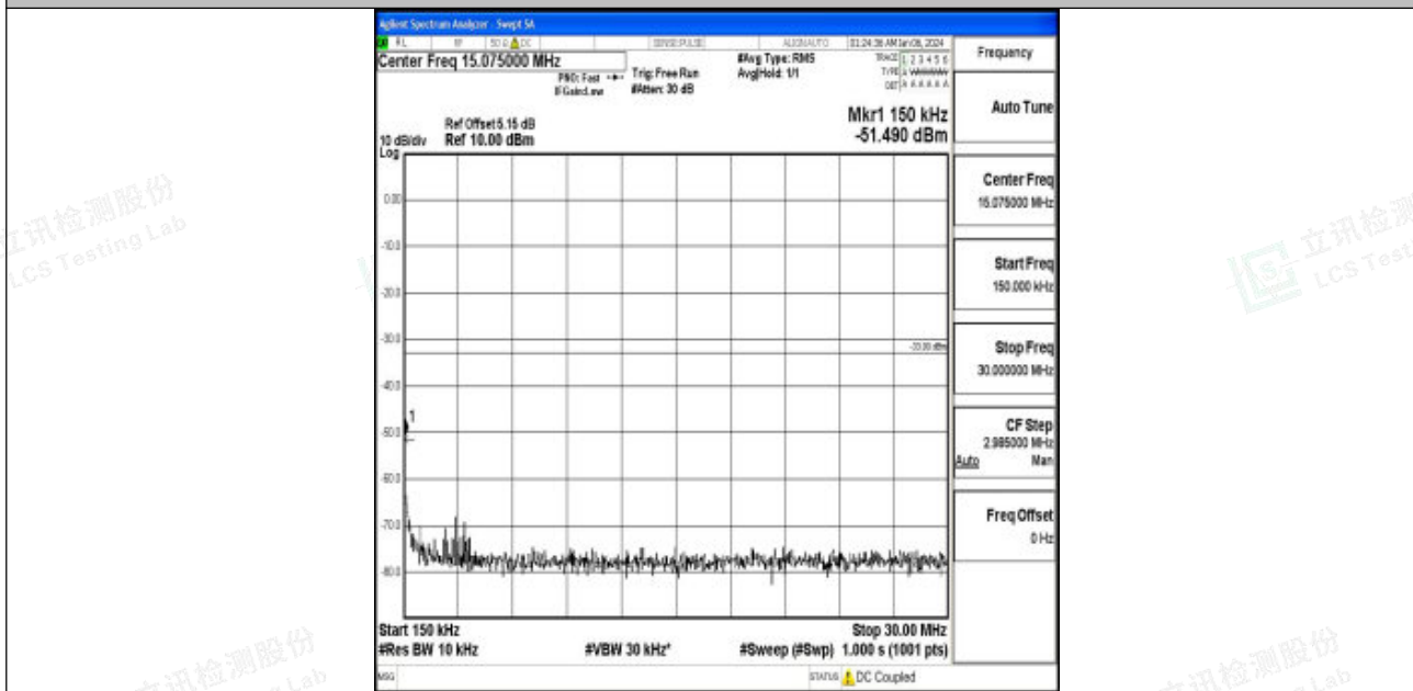
Band66_3MHz_16QAM_131987_1RB#0_0.15~30_0.15~30
