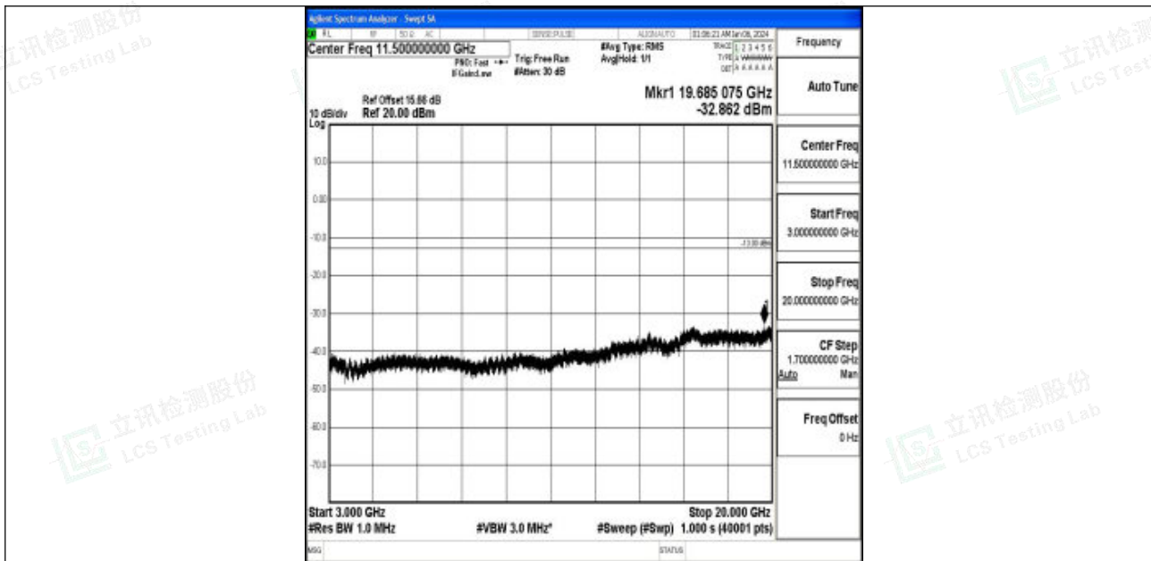
Band66_1.4MHz_16QAM_132665_1RB#0_3000~20000_3000~20000
