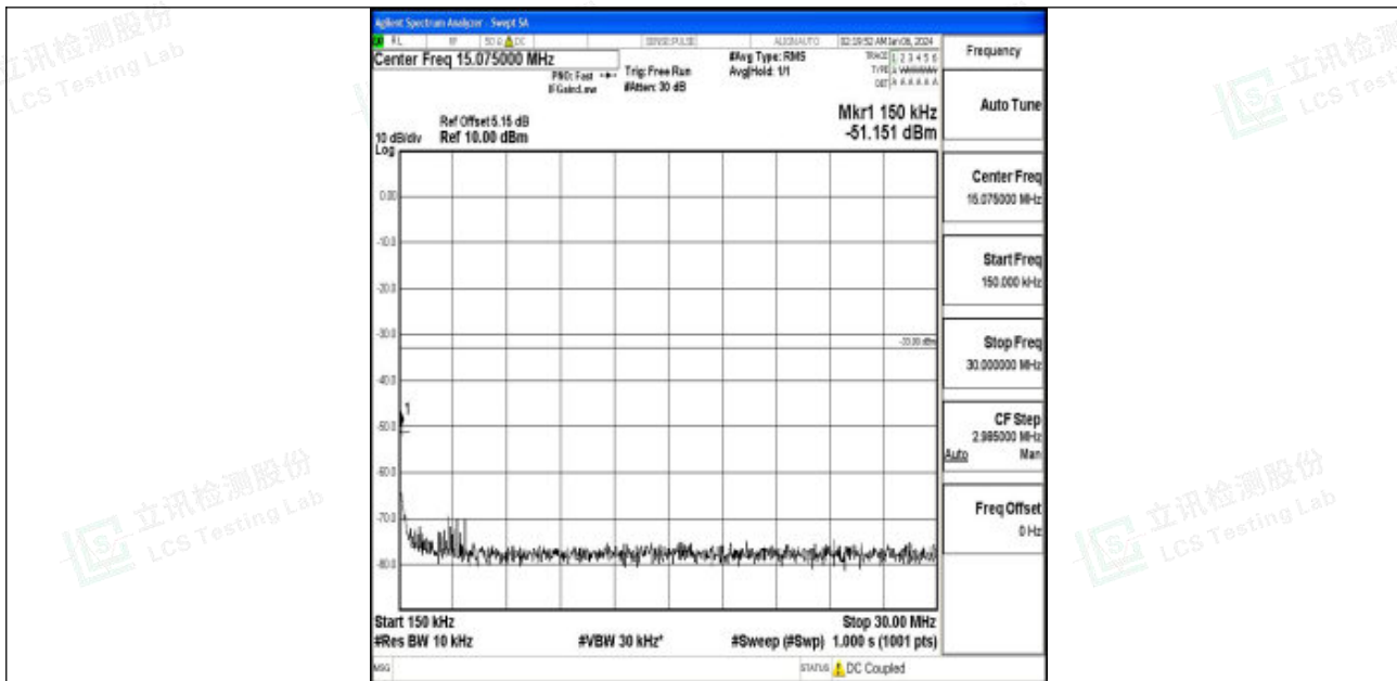
Band66_15MHz_QPSK_132322_1RB#0_0.15~30_0.15~30
