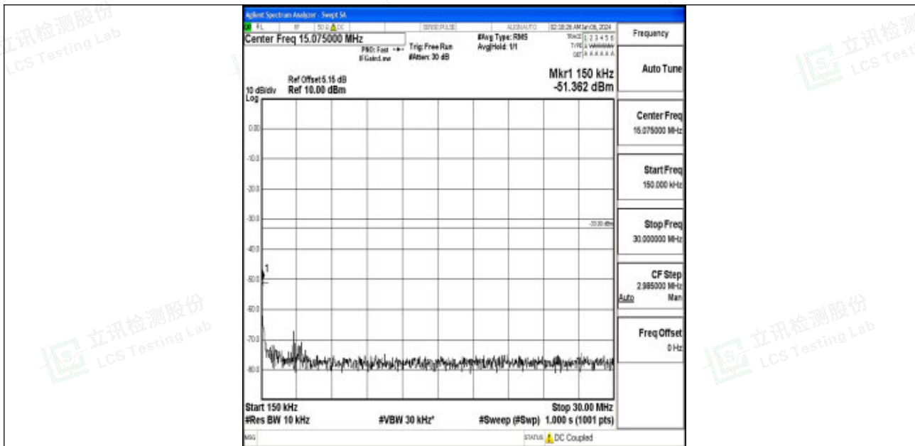
Band66_15MHz_QPSK_132047_1RB#0_0.15~30_0.15~30
