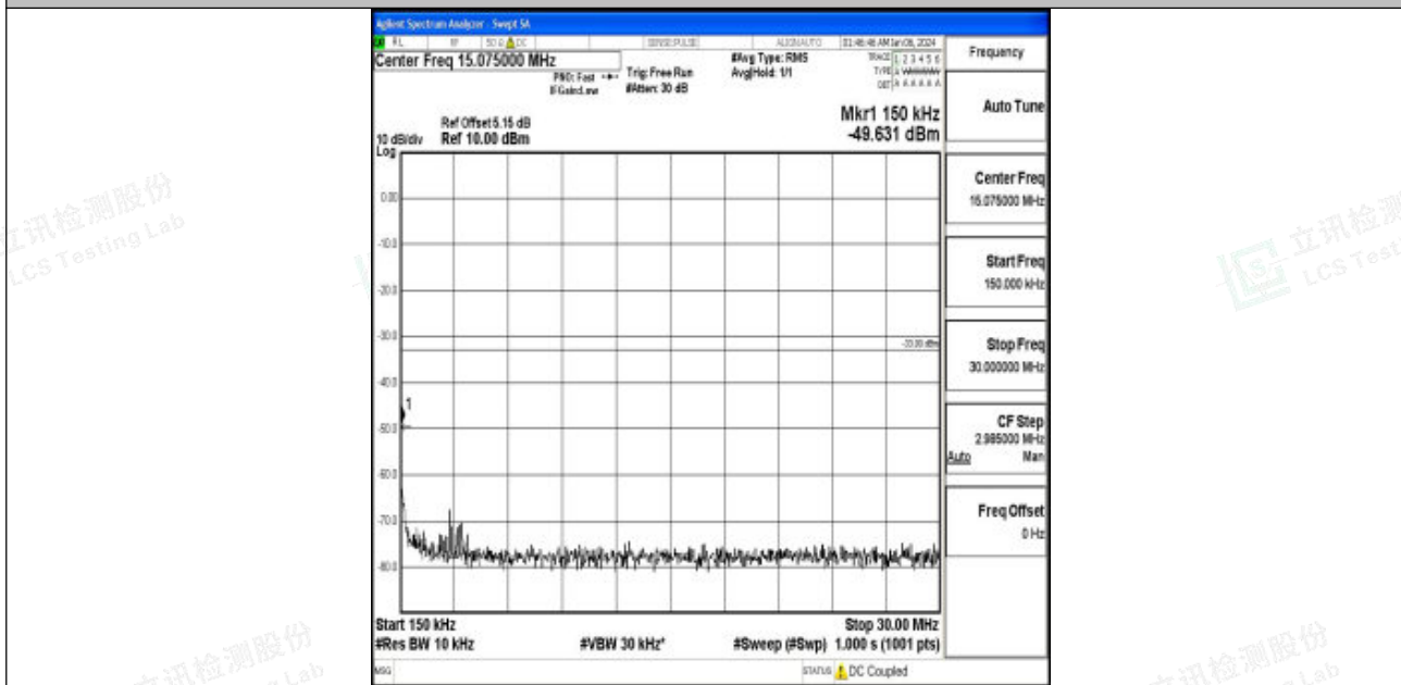
Band66_5MHz_16QAM_132647_1RB#0_0.15~30_0.15~30
