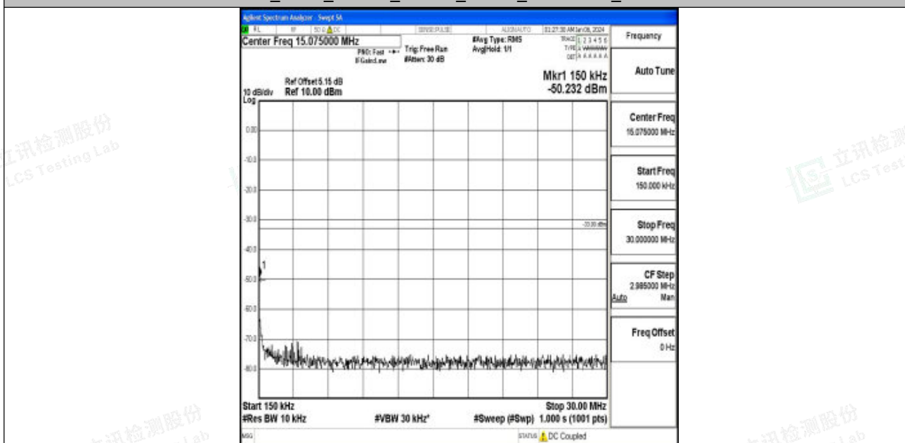
Band66_3MHz_16QAM_132657_1RB#0_0.15~30_0.15~30
