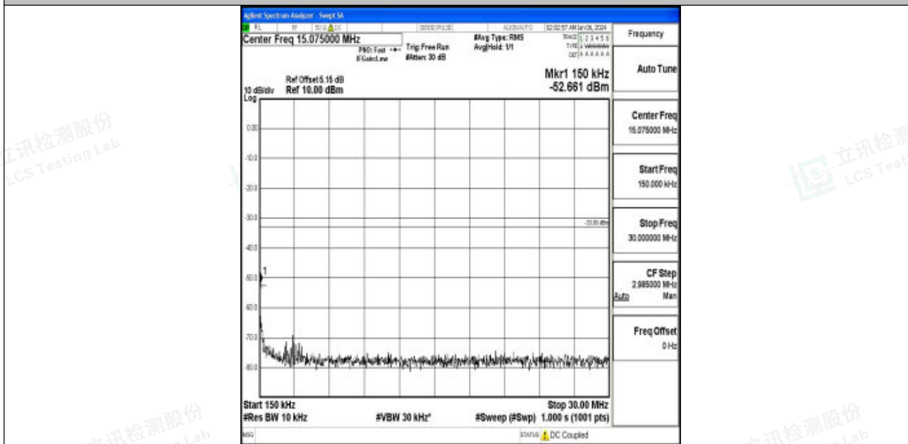
Band66_10MHz_16QAM_132022_1RB#0_0.15~30_0.15~30
