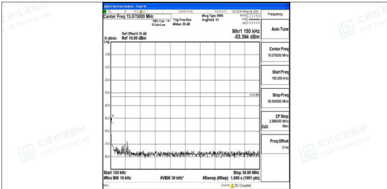
Band66_3MHz_QPSK_131987_1RB#0_0.15~30_0.15~30
