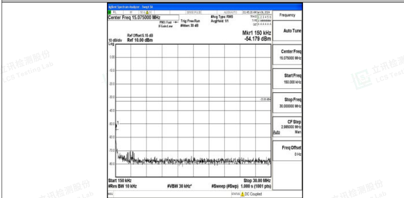
Band66_5MHz_16QAM_132322_1RB#0_0.15~30_0.15~30
