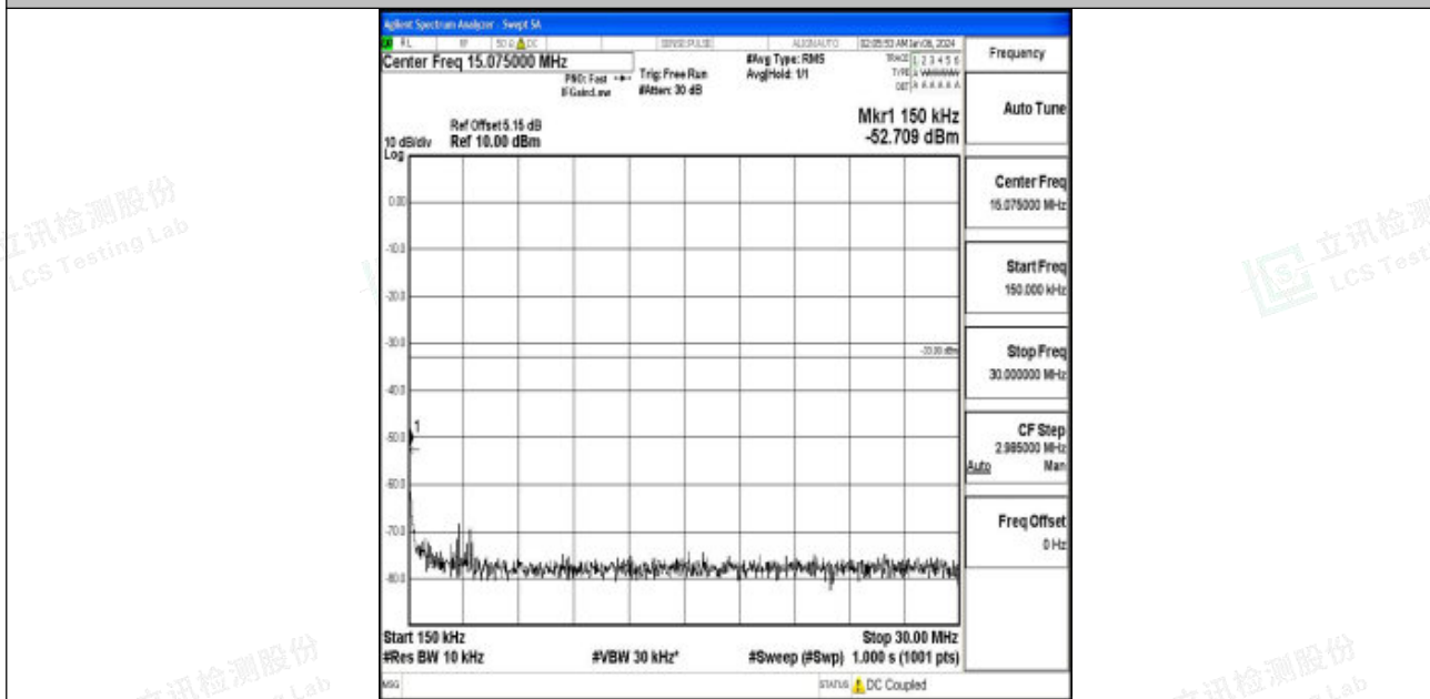
Band66_10MHz_16QAM_132622_1RB#0_0.15~30_0.15~30
