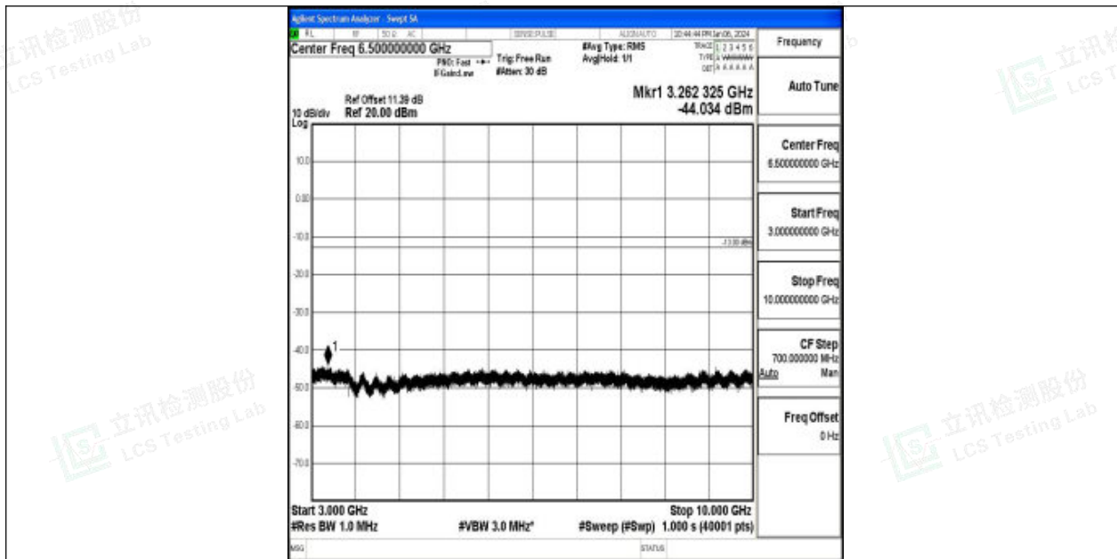
Band26_10MHz_QPSK_26990_1RB#0_3000~10000_3000~10000
