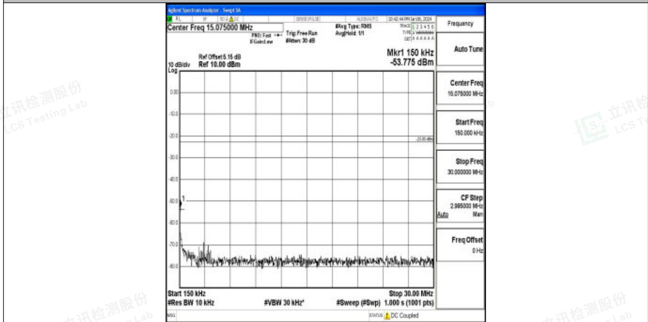
Band26_10MHz_QPSK_26915_1RB#0_0.15~30_0.15~30
