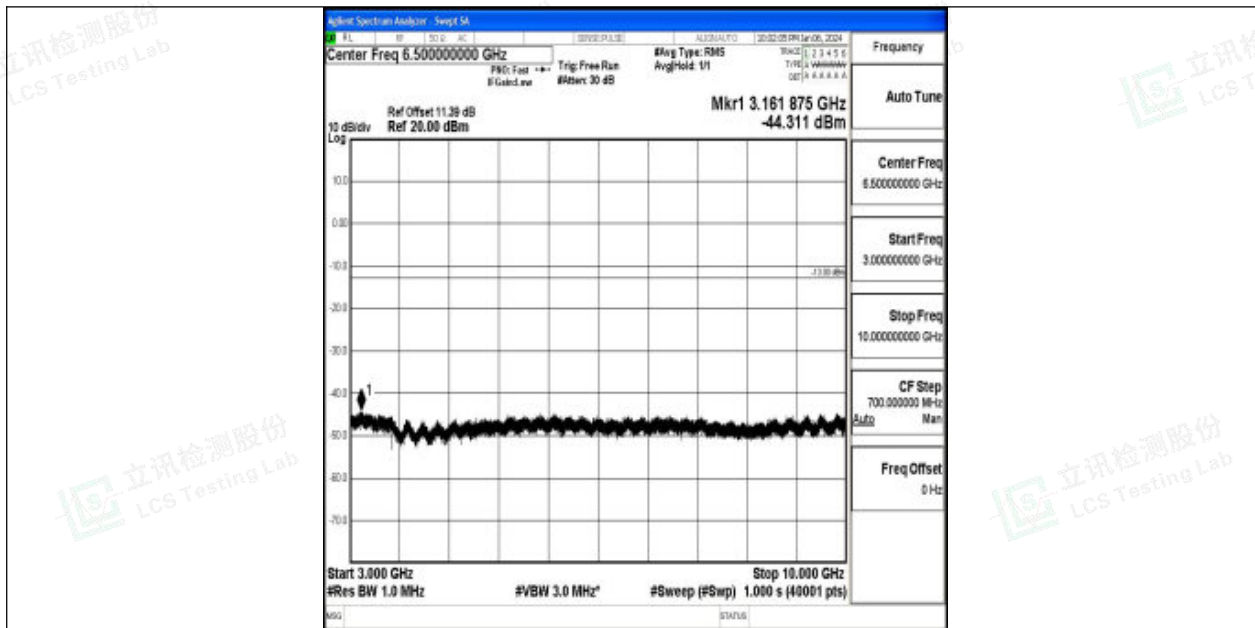
Band26_3MHz_QPSK_26915_1RB#0_3000~10000_3000~10000
