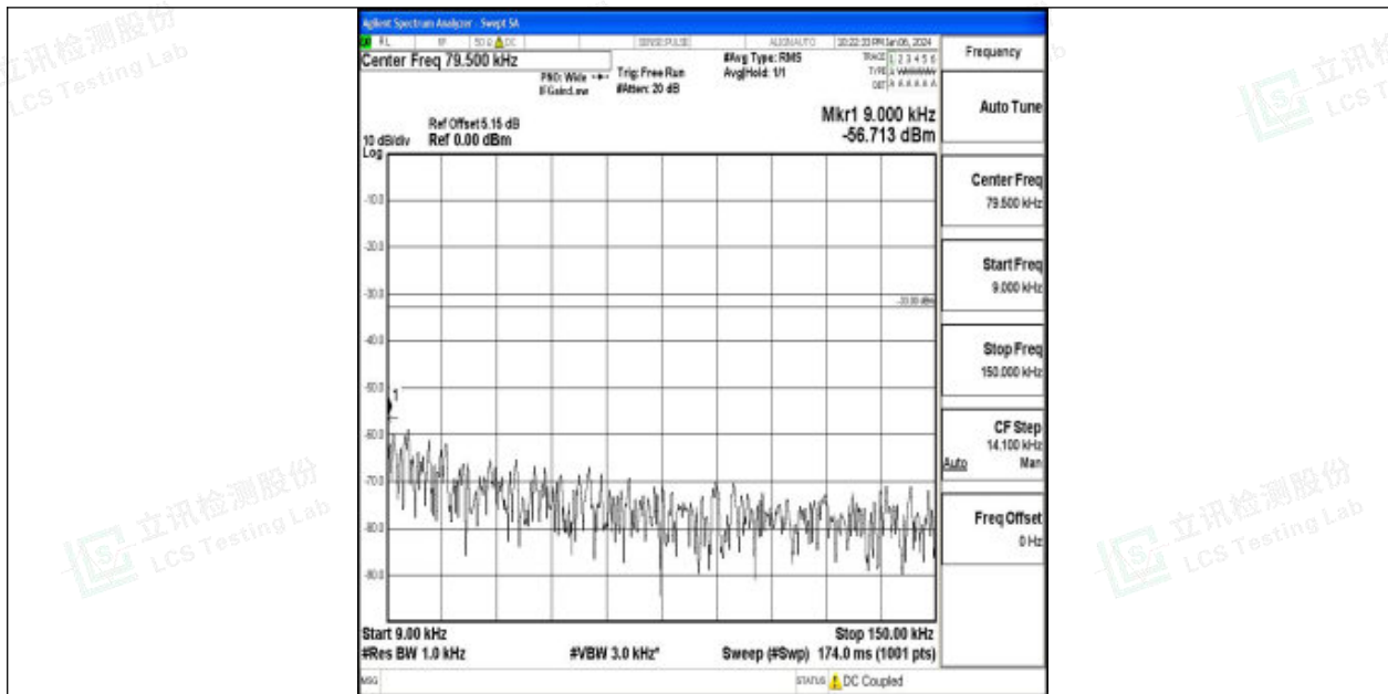
Band26_5MHz_QPSK_26915_1RB#0_0.009~0.15_0.009~0.15
