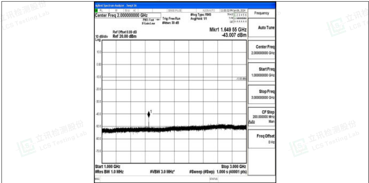
Band26_15MHz_16QAM_26865_1RB#0_1000~3000_1000~3000
