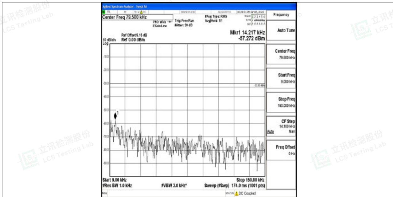
Band26_5MHz_QPSK_27015_1RB#0_0.009~0.15_0.009~0.15
