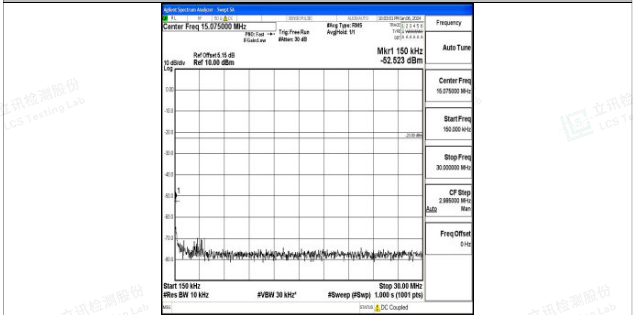
Band26_3MHz_QPSK_27025_1RB#0_0.15~30_0.15~30
