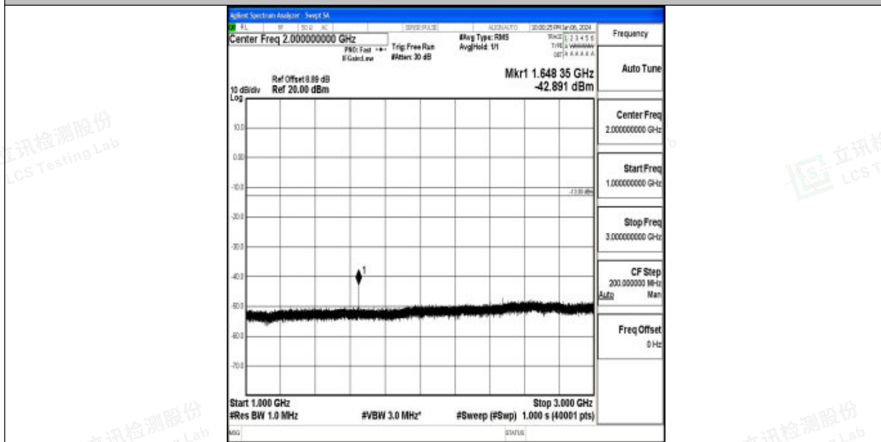
Band26_3MHz_QPSK_26805_1RB#0_1000~3000_1000~3000
