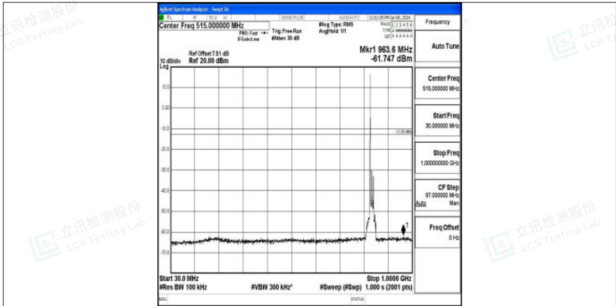
Band26_15MHz_QPSK_26915_1RB#0_30~1000_30~1000
