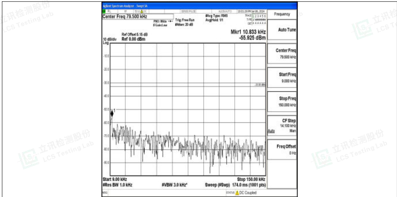
Band26_3MHz_QPSK_26915_1RB#0_0.009~0.15_0.009~0.15
