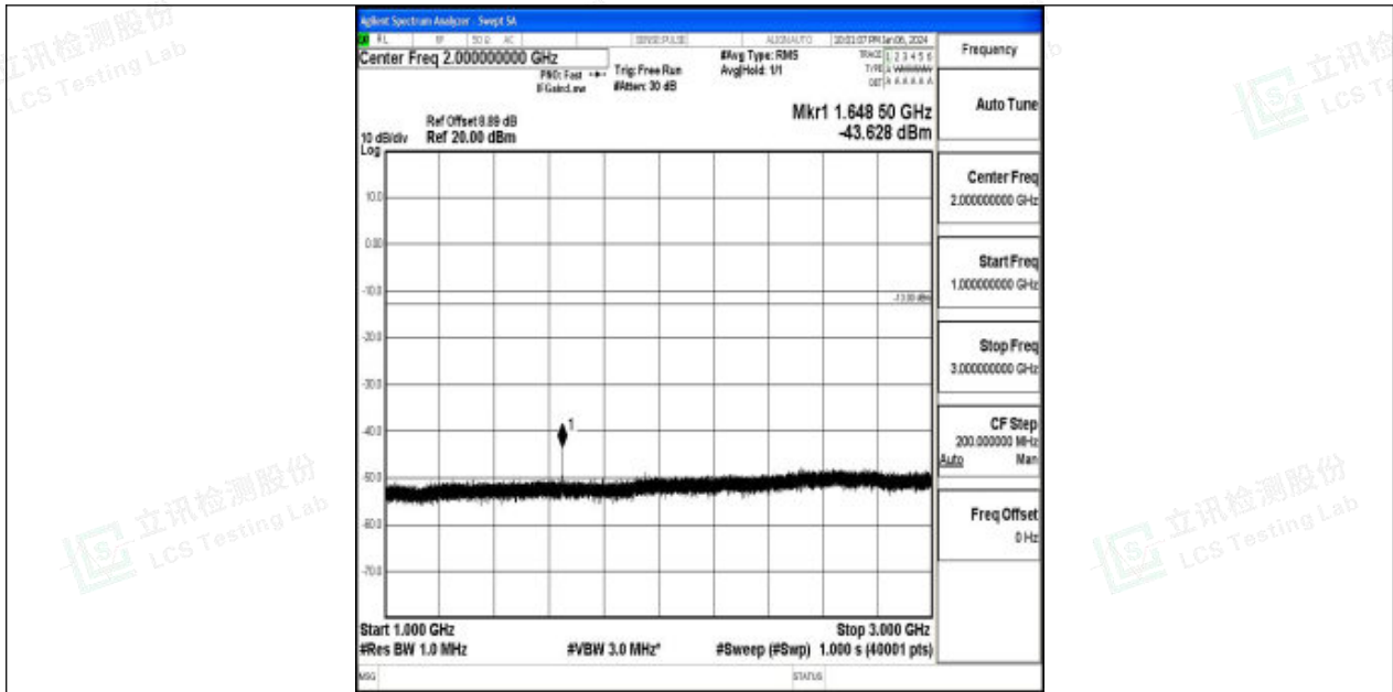
Band26_3MHz_16QAM_26805_1RB#0_1000~3000_1000~3000
