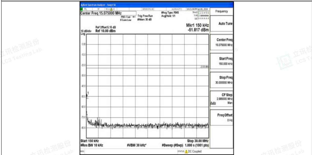
Band26_5MHz_QPSK_26815_1RB#0_0.15~30_0.15~30
