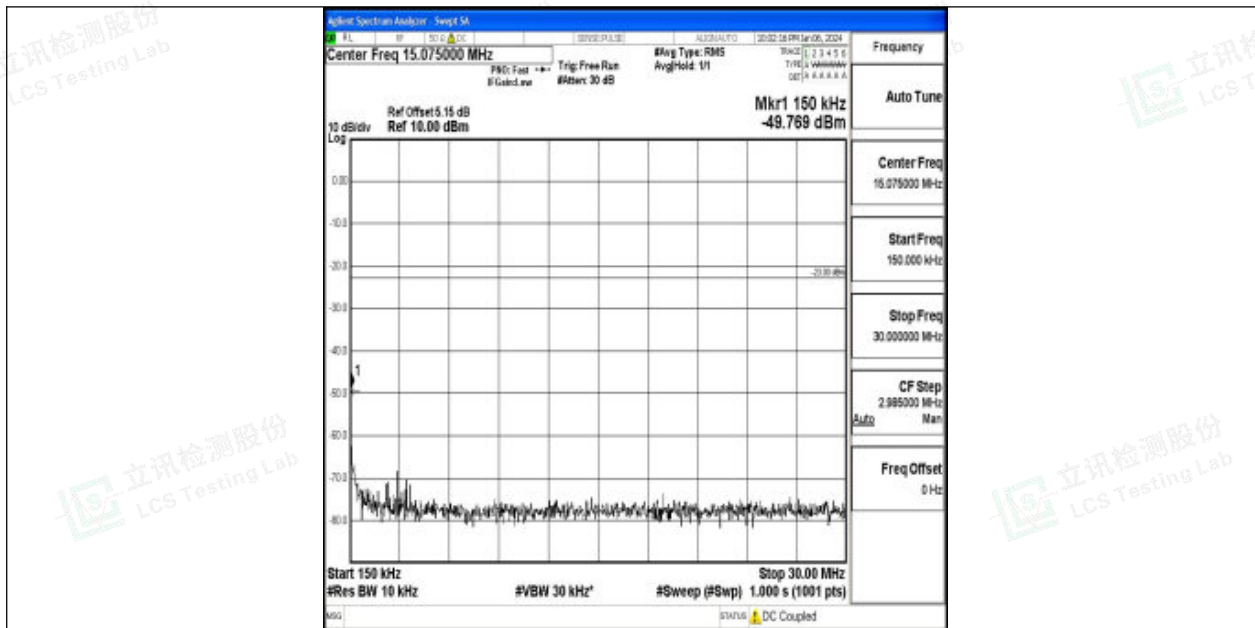
Band26_3MHz_16QAM_26915_1RB#0_0.15~30_0.15~30
