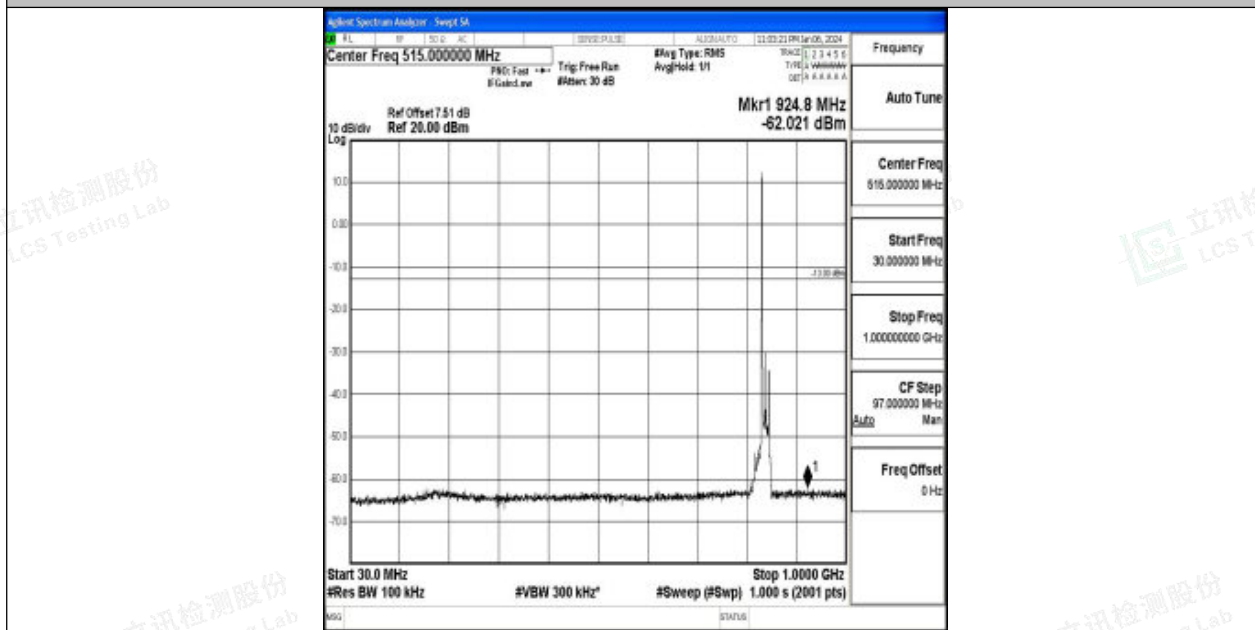
Band26_15MHz_16QAM_26965_1RB#0_30~1000_30~1000
