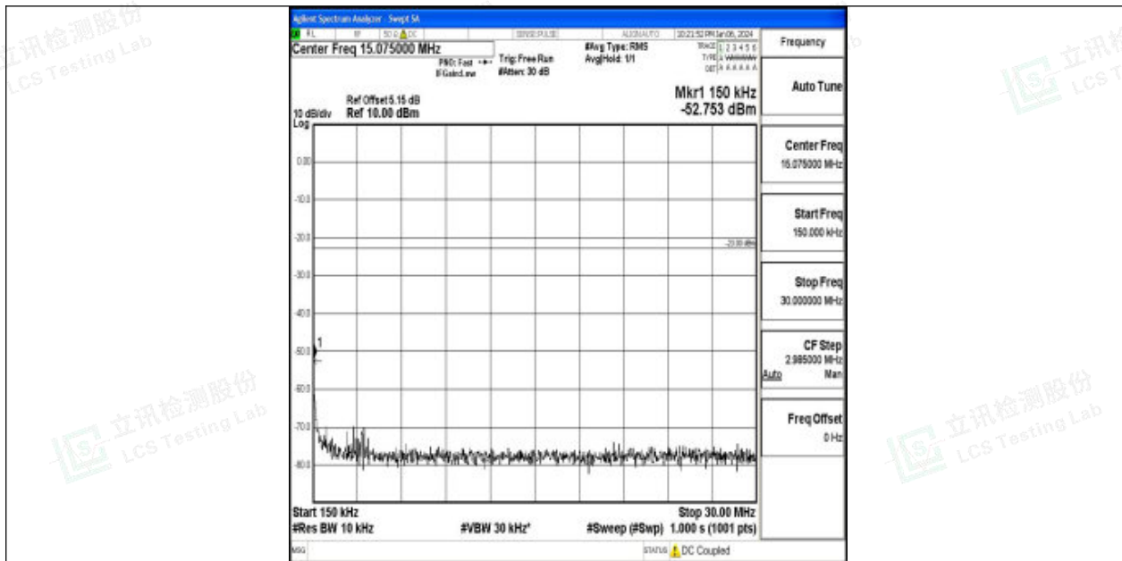
Band26_5MHz_16QAM_26815_1RB#0_0.15~30_0.15~30
