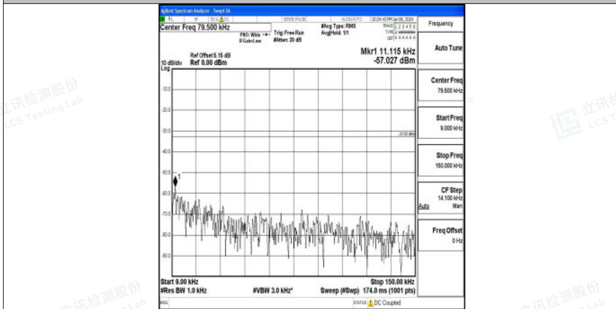
Band26_5MHz_16QAM_27015_1RB#0_0.009~0.15_0.009~0.15
