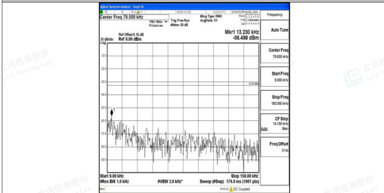
Band26_10MHz_16QAM_26990_1RB#0_0.009~0.15_0.009~0.15
