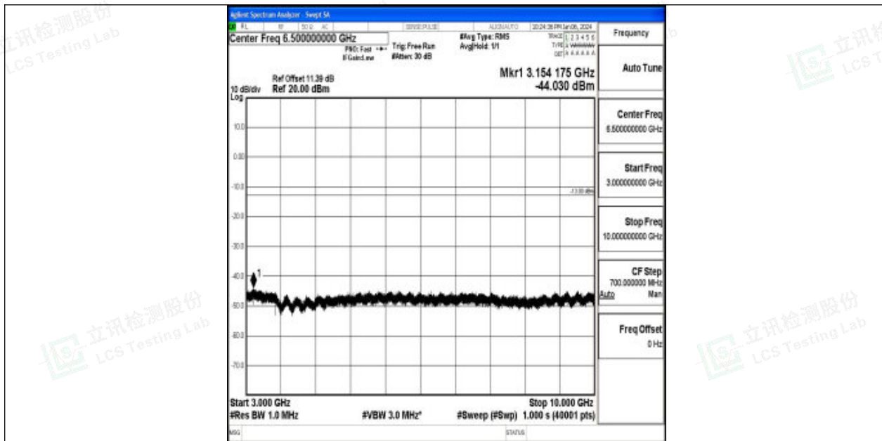
Band26_5MHz_QPSK_27015_1RB#0_3000~10000_3000~10000
