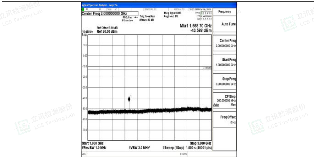
Band26_5MHz_16QAM_26915_1RB#0_1000~3000_1000~3000
