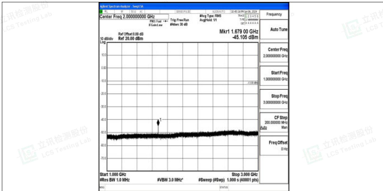
Band26_10MHz_16QAM_26990_1RB#0_1000~3000_1000~3000
