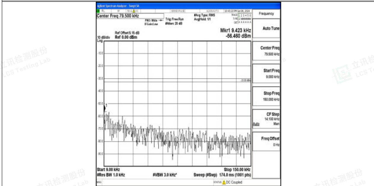
Band26_10MHz_16QAM_26915_1RB#0_0.009~0.15_0.009~0.15
