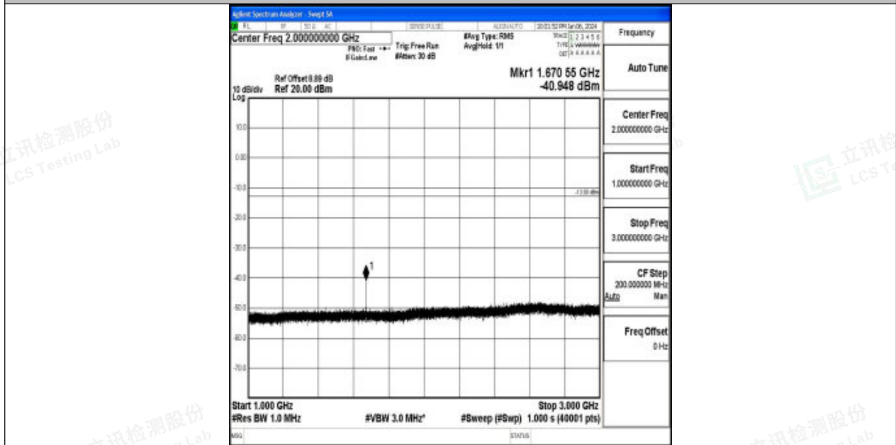
Band26_3MHz_QPSK_26915_1RB#0_1000~3000_1000~3000
