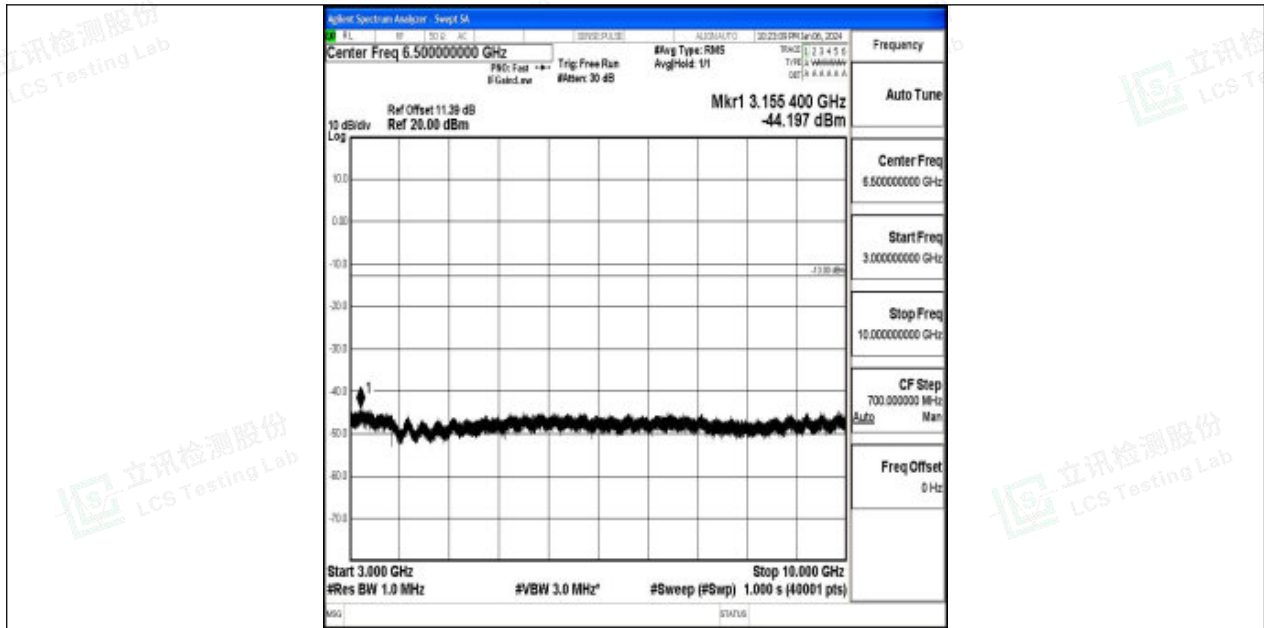
Band26_5MHz_QPSK_26915_1RB#0_3000~10000_3000~10000
