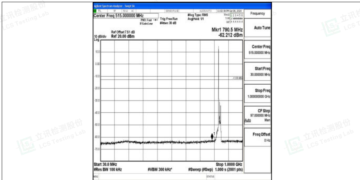
Band26_15MHz_QPSK_26965_1RB#0_30~1000_30~1000
