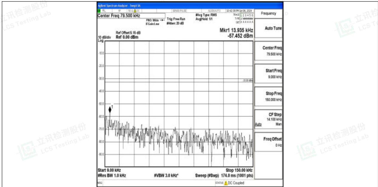
Band26_10MHz_QPSK_26915_1RB#0_0.009~0.15_0.009~0.15
