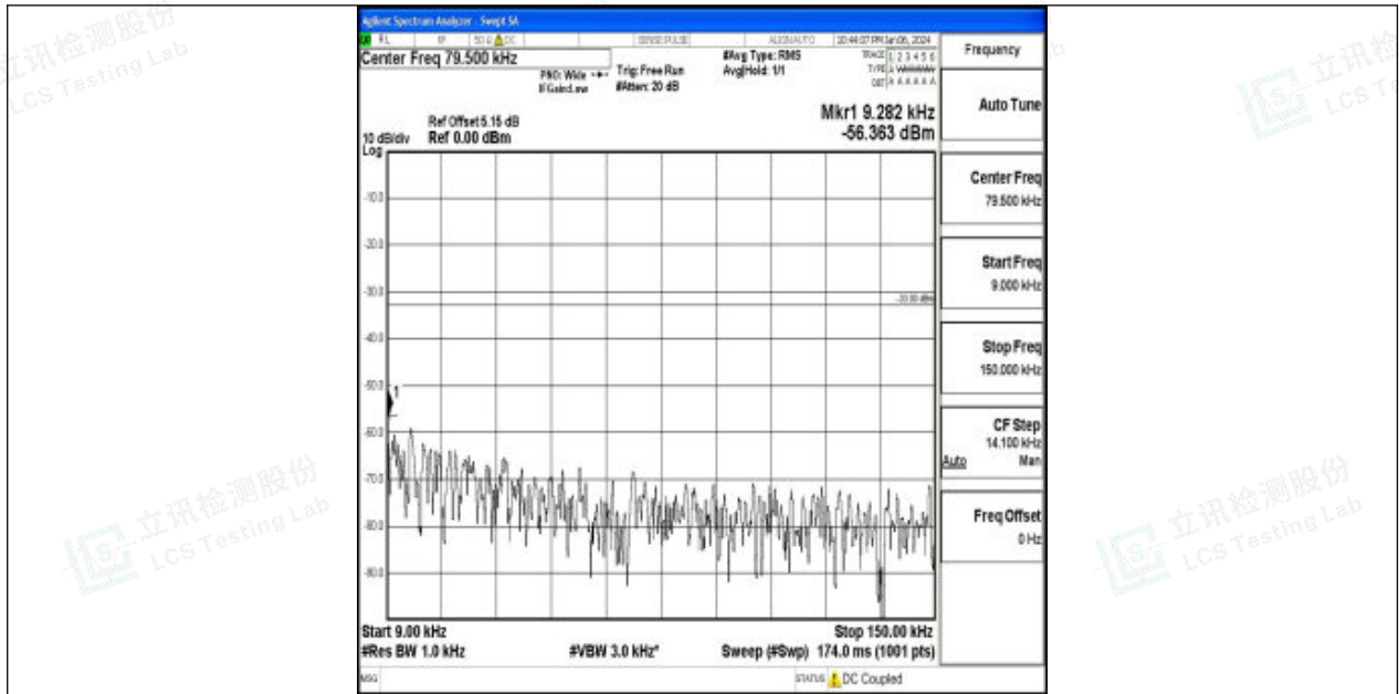
Band26_10MHz_QPSK_26990_1RB#0_0.009~0.15_0.009~0.15
