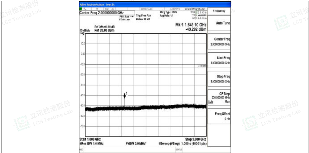
Band26_10MHz_16QAM_26840_1RB#0_1000~3000_1000~3000
