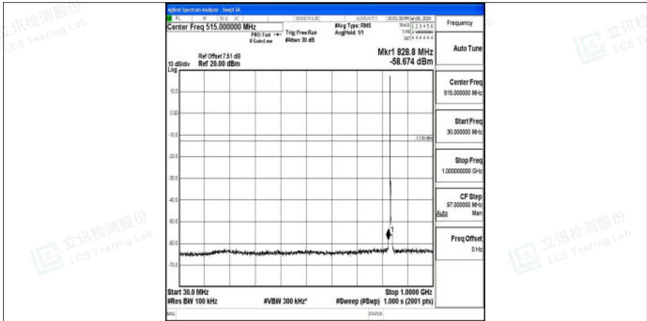
Band26_3MHz_QPSK_26915_1RB#0_30~1000_30~1000
