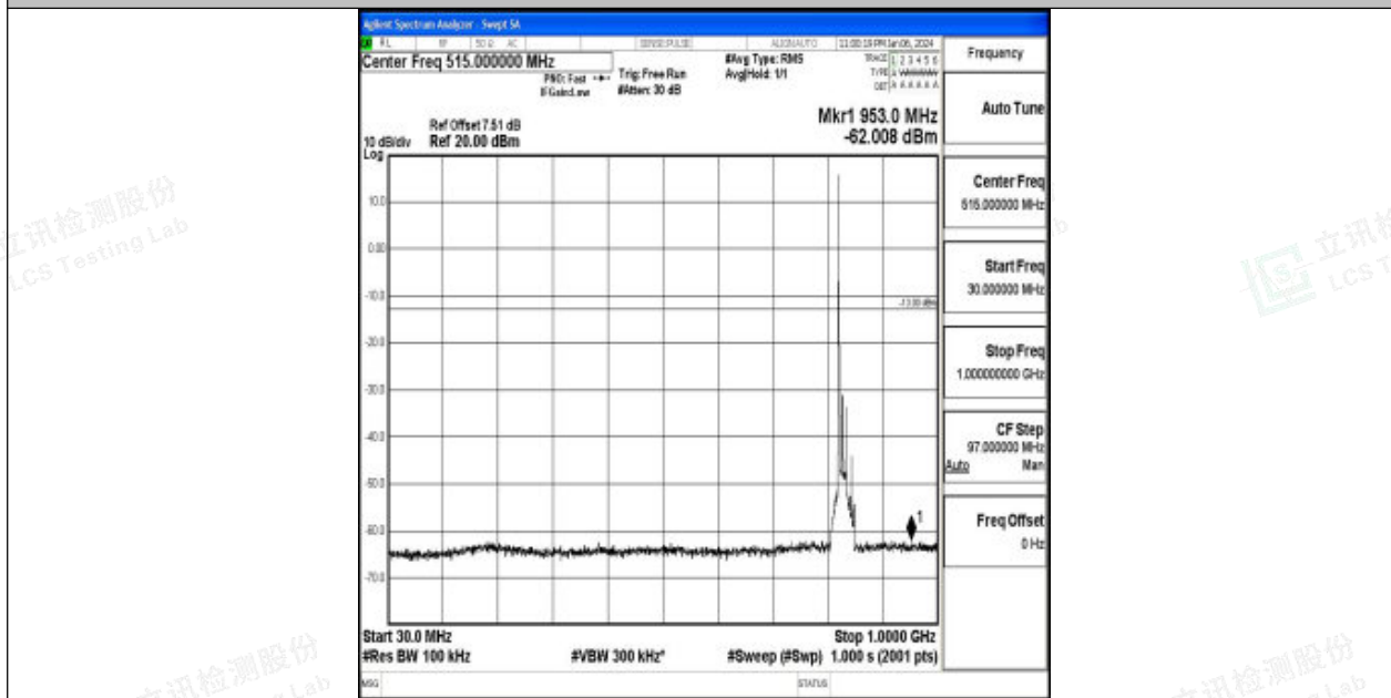
Band26_15MHz_16QAM_26865_1RB#0_30~1000_30~1000
