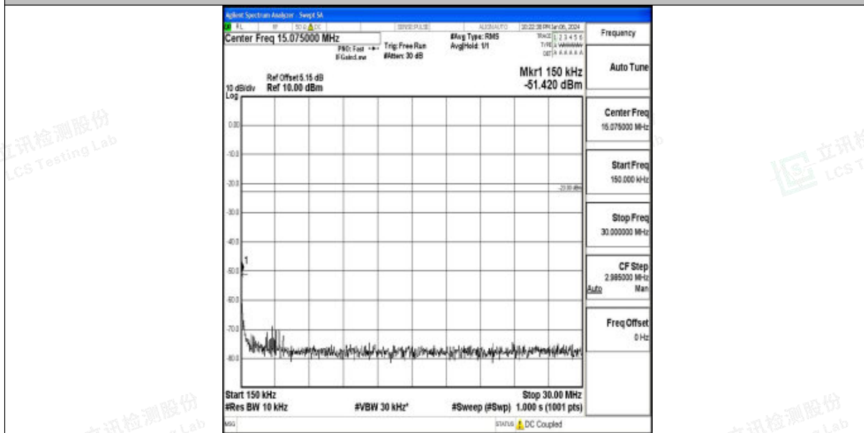
Band26_5MHz_QPSK_26915_1RB#0_0.15~30_0.15~30
