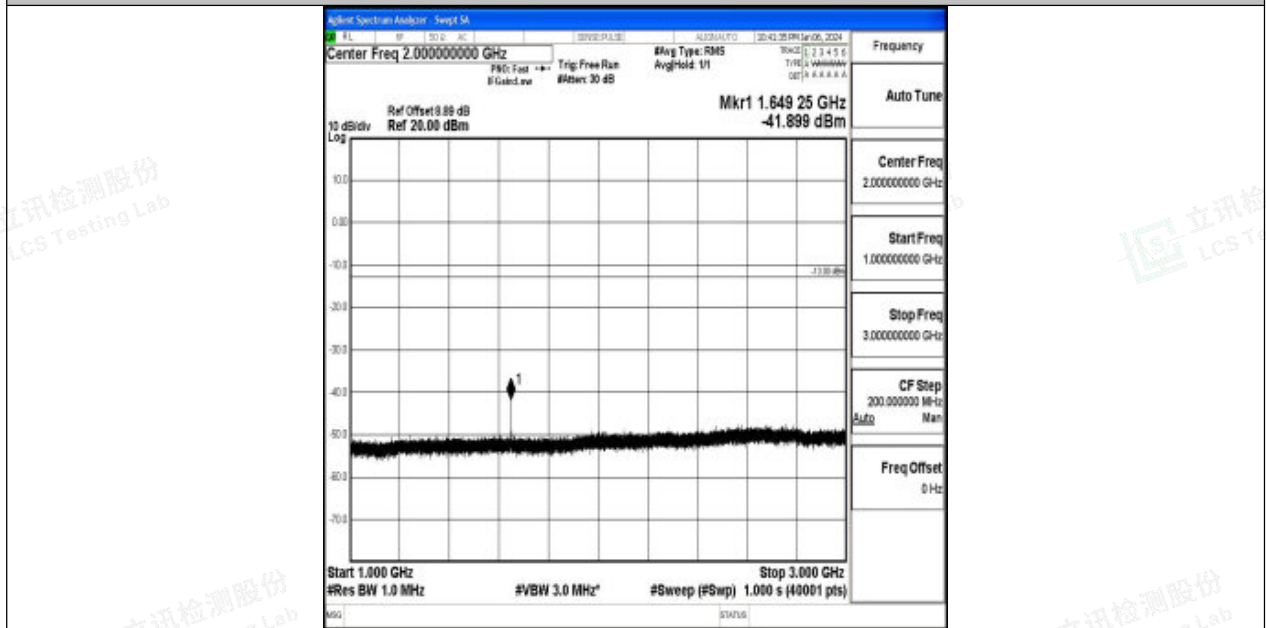
Band26_10MHz_QPSK_26840_1RB#0_1000~3000_1000~3000
