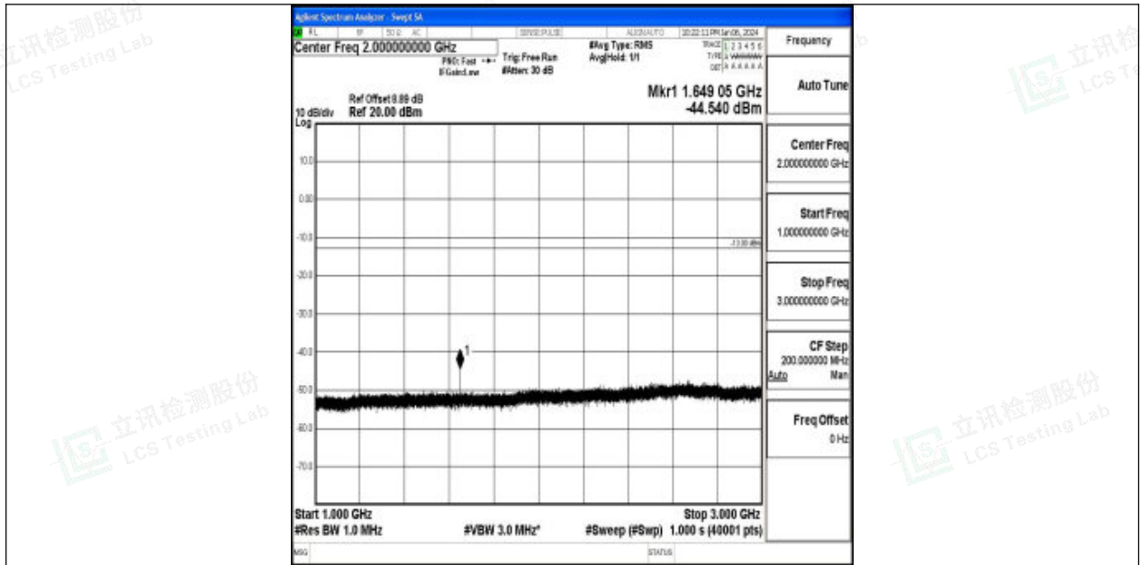
Band26_5MHz_16QAM_26815_1RB#0_1000~3000_1000~3000
