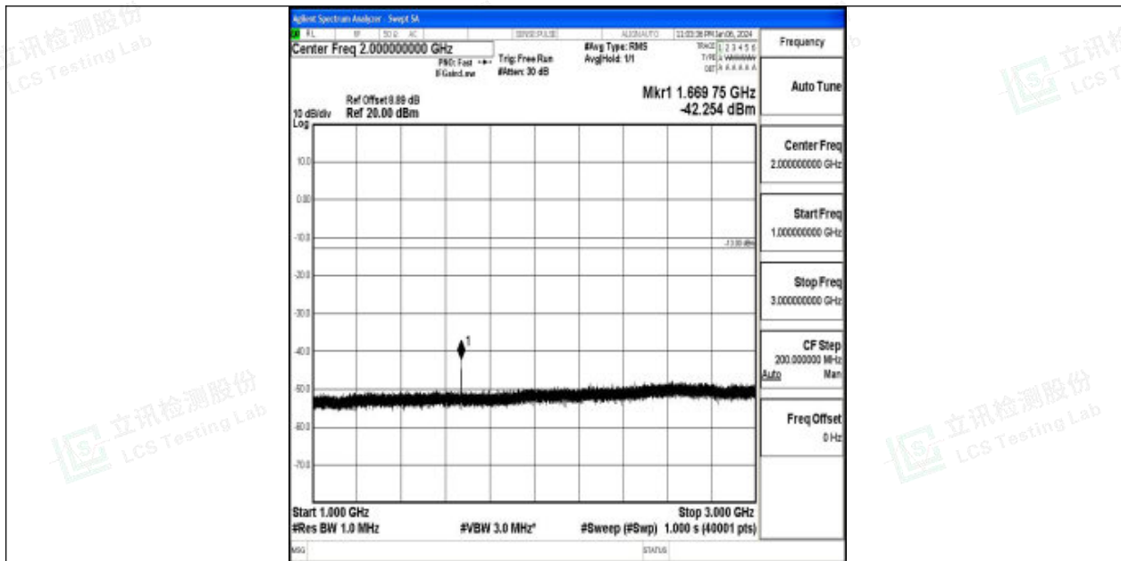
Band26_15MHz_16QAM_26965_1RB#0_1000~3000_1000~3000
