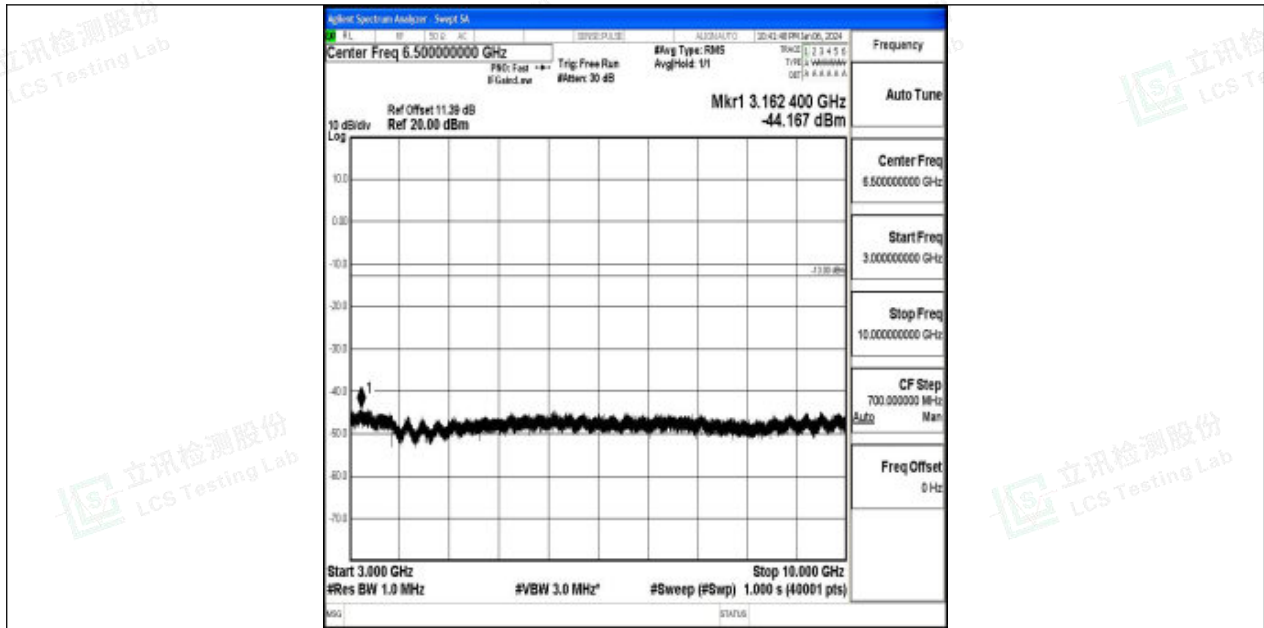
Band26_10MHz_QPSK_26840_1RB#0_3000~10000_3000~10000
