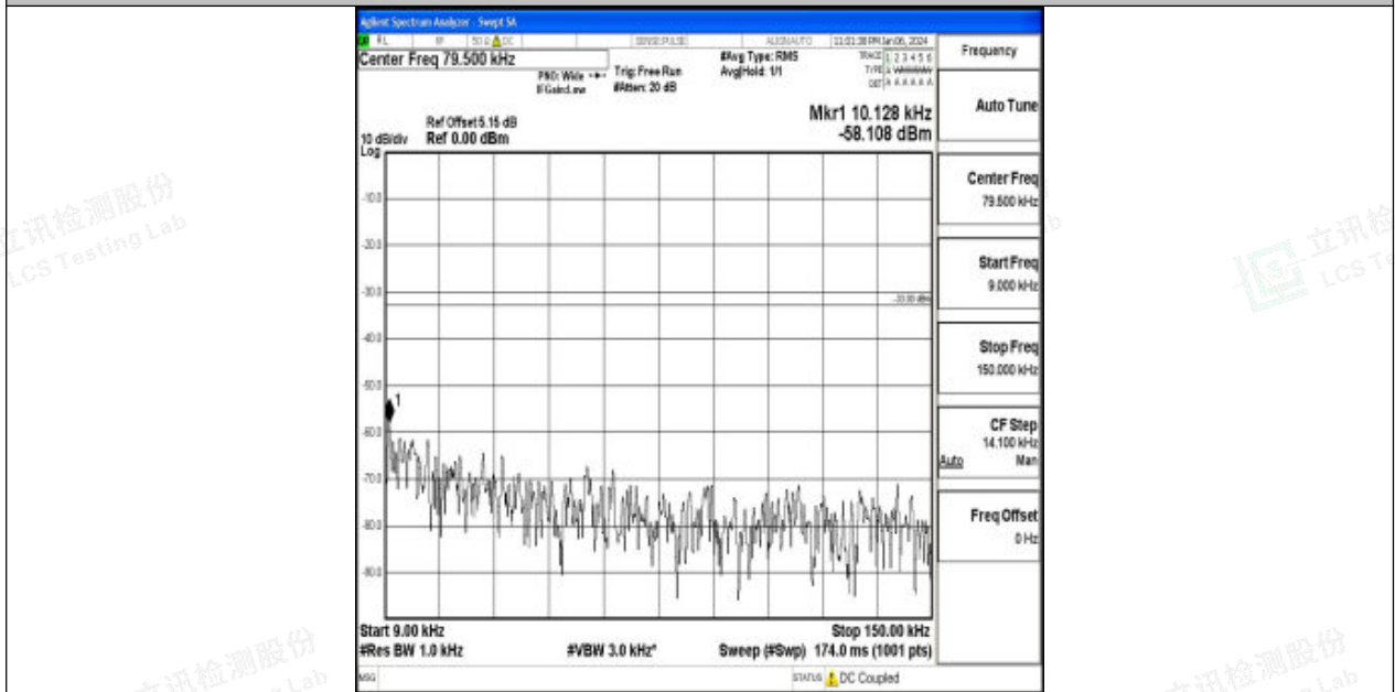
Band26_15MHz_16QAM_26915_1RB#0_0.009~0.15_0.009~0.15
