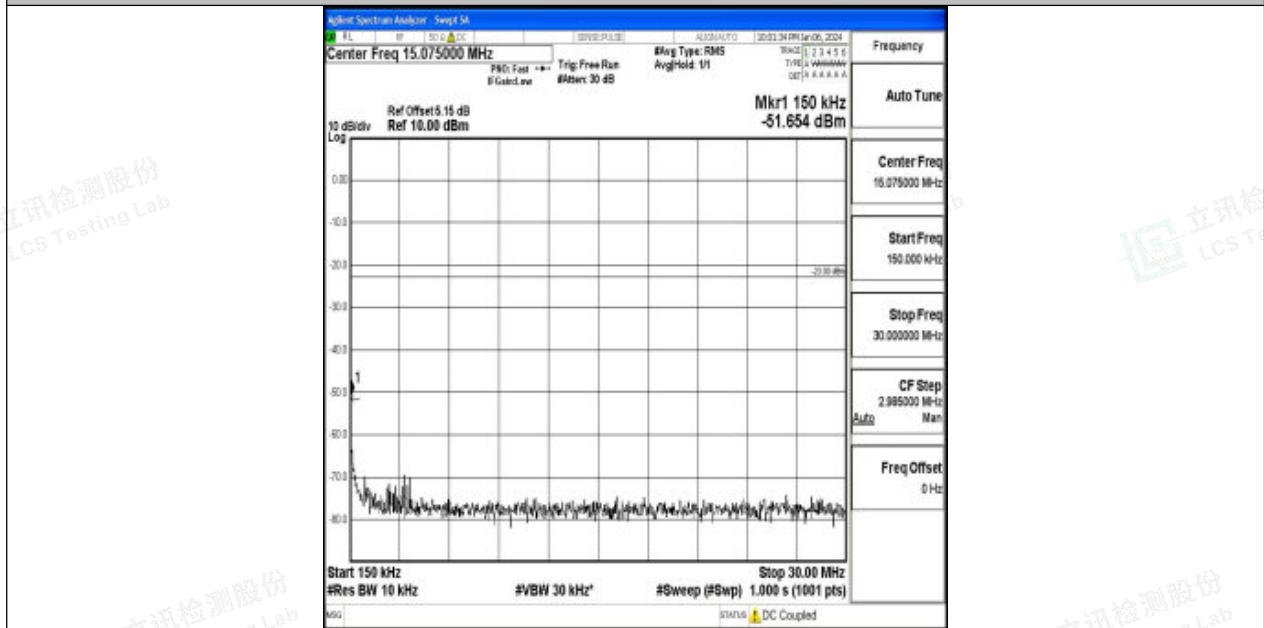
Band26_3MHz_QPSK_26915_1RB#0_0.15~30_0.15~30
