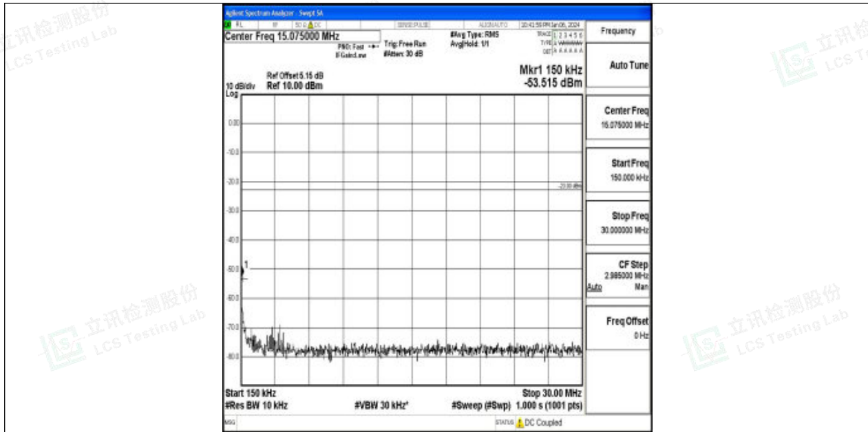
Band26_10MHz_16QAM_26840_1RB#0_0.15~30_0.15~30
