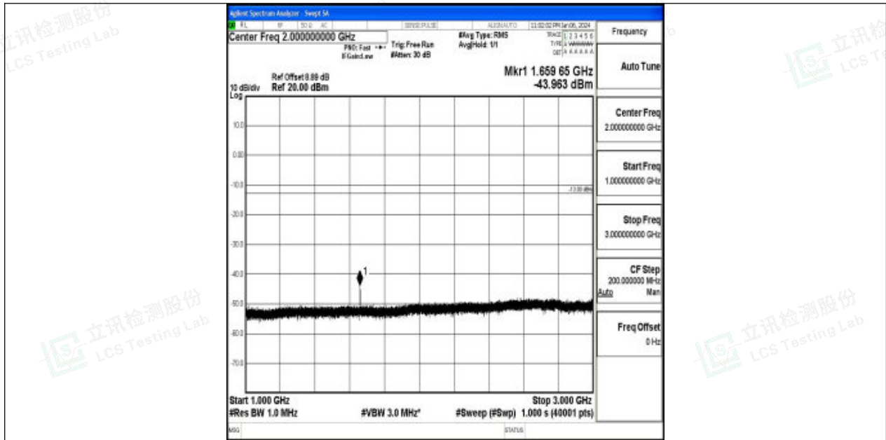
Band26_15MHz_16QAM_26915_1RB#0_1000~3000_1000~3000
