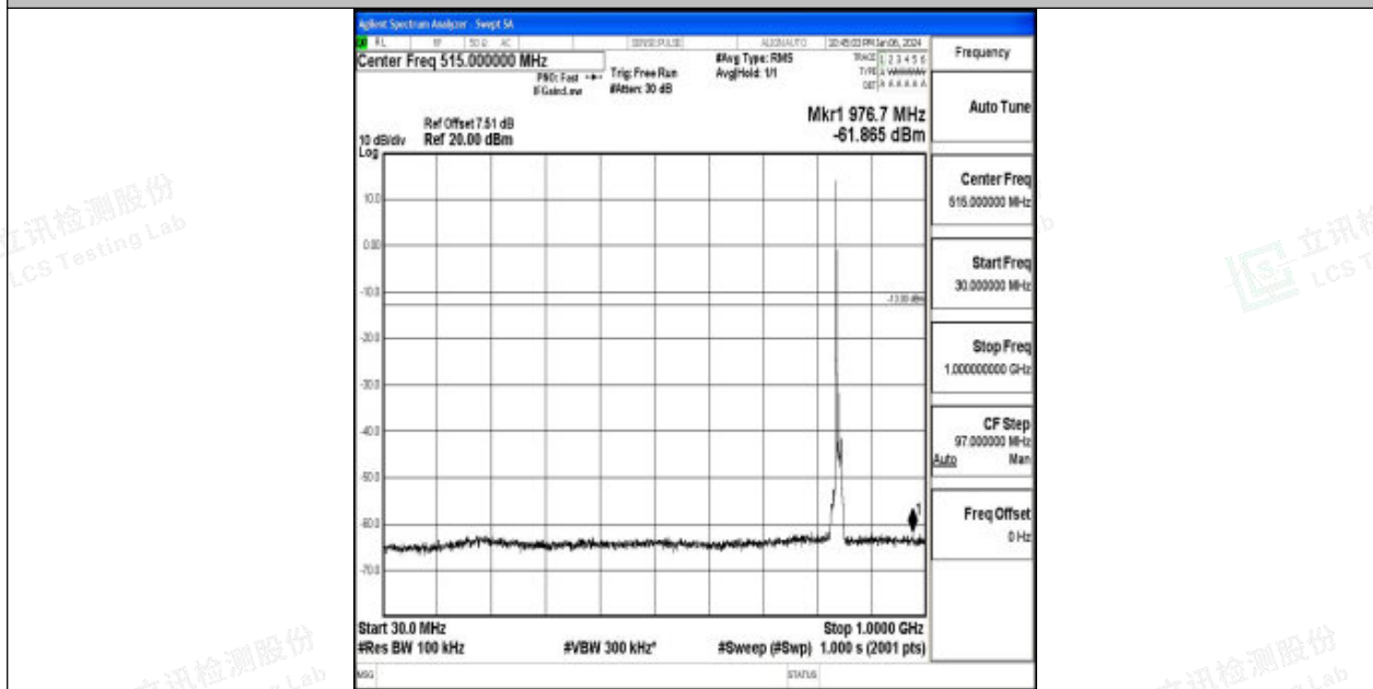
Band26_10MHz_16QAM_26990_1RB#0_30~1000_30~1000
