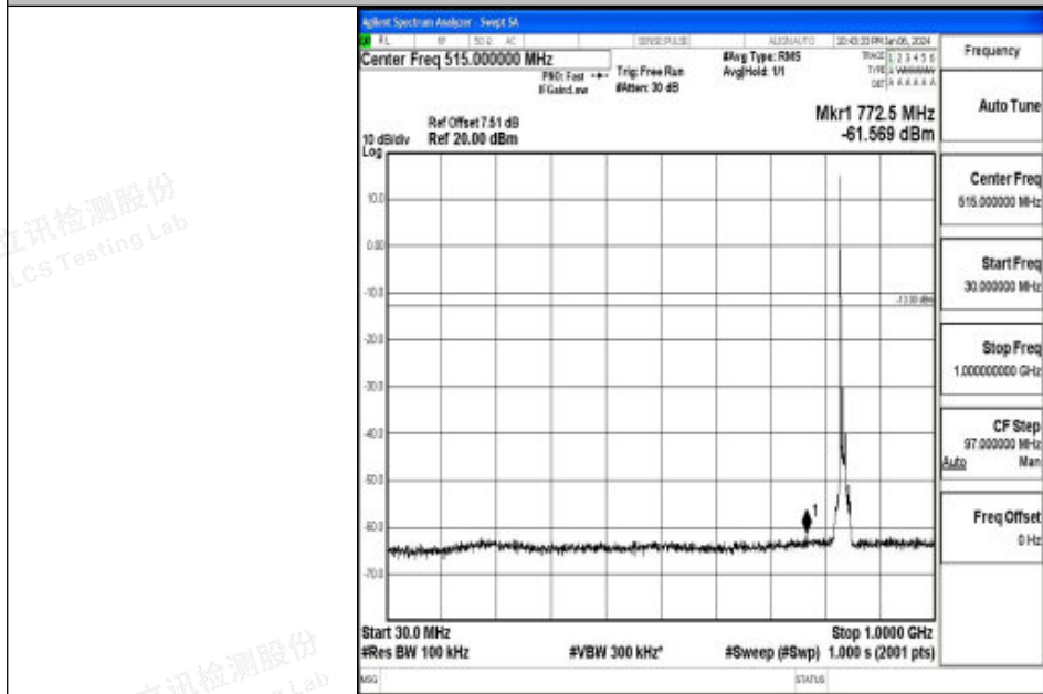
Band26_10MHz_16QAM_26915_1RB#0_30~1000_30~1000
