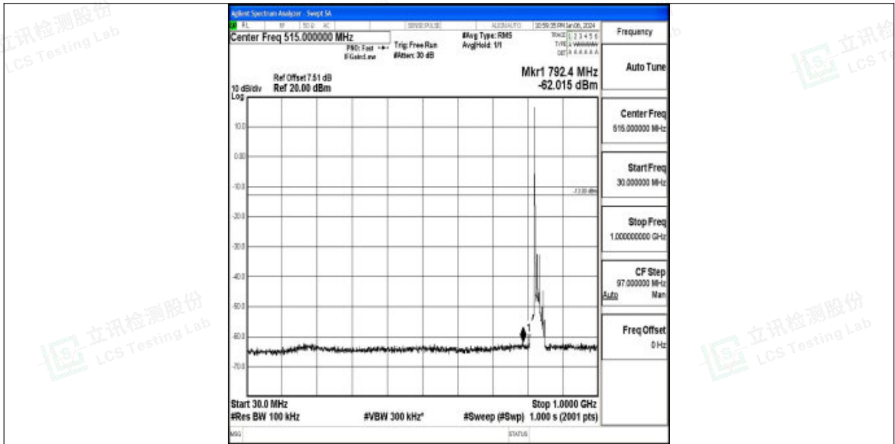
Band26_15MHz_QPSK_26865_1RB#0_30~1000_30~1000
