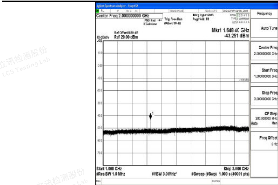
Band26_5MHz_QPSK_26815_1RB#0_1000~3000_1000~3000
