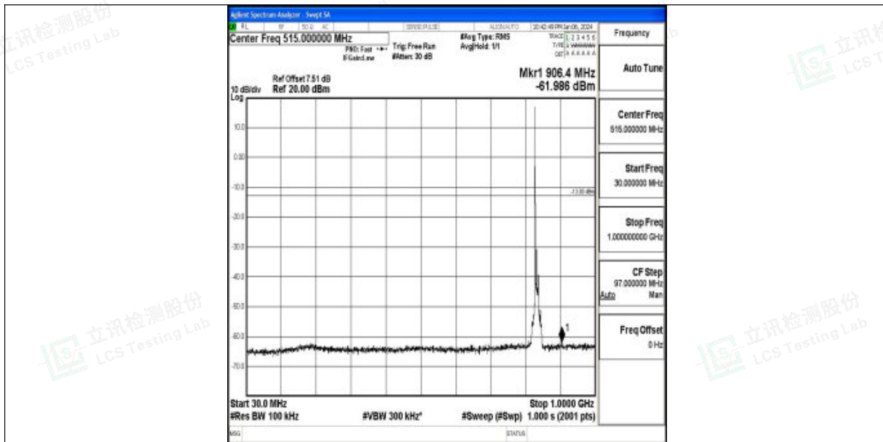
Band26_10MHz_QPSK_26915_1RB#0_30~1000_30~1000
