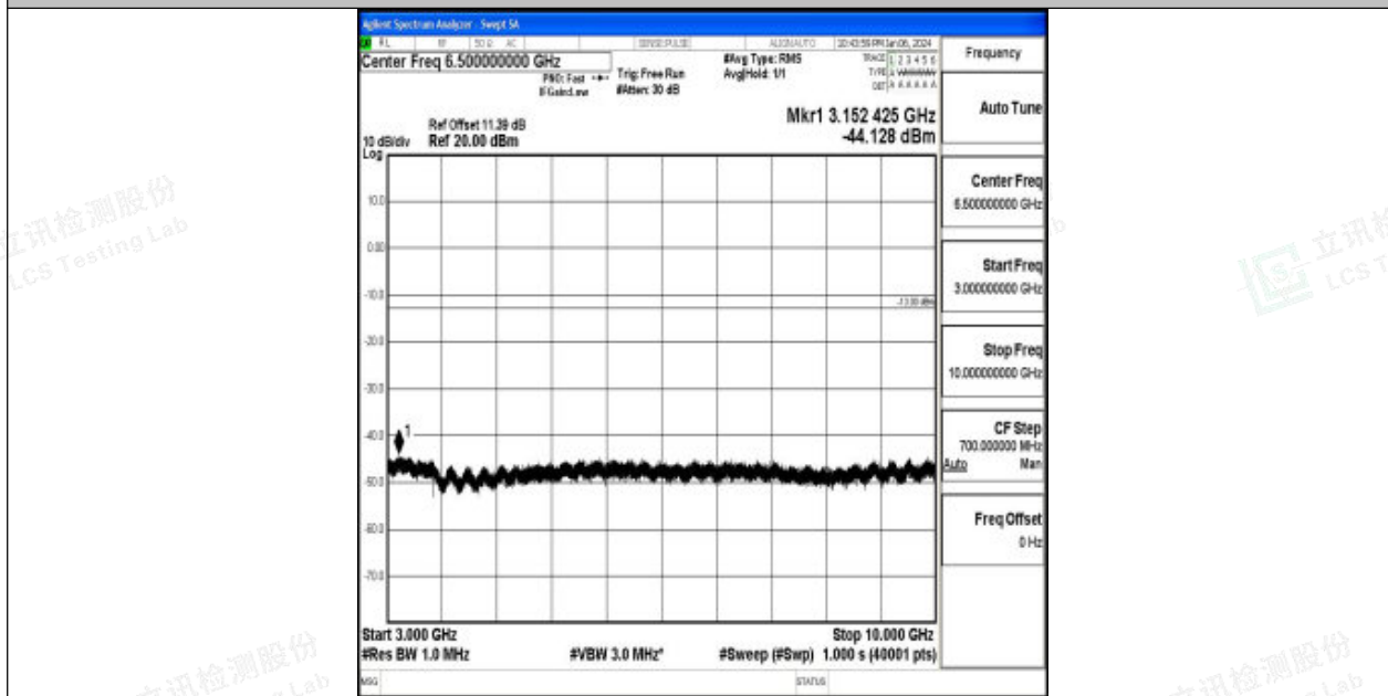
Band26_10MHz_16QAM_26915_1RB#0_3000~10000_3000~10000
