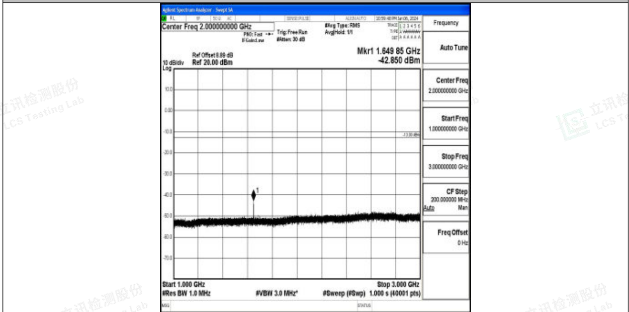
Band26_15MHz_QPSK_26865_1RB#0_1000~3000_1000~3000
