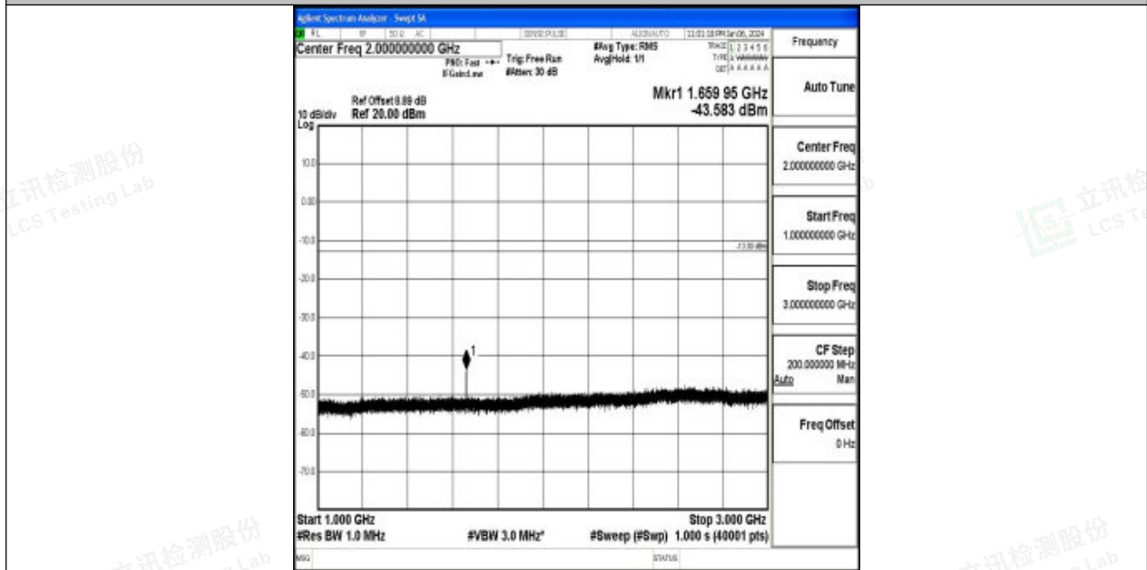
Band26_15MHz_QPSK_26915_1RB#0_1000~3000_1000~3000
