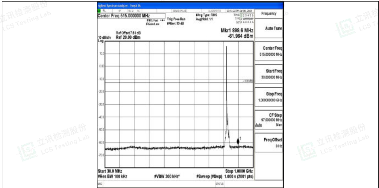
Band26_10MHz_QPSK_26840_1RB#0_30~1000_30~1000
