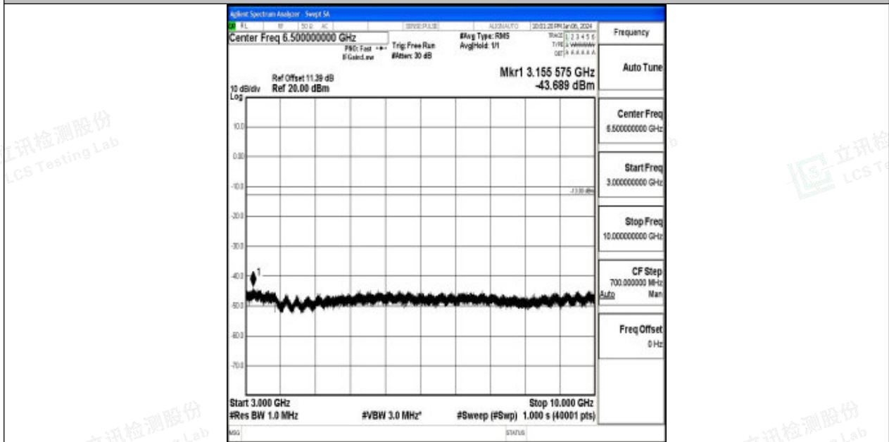
Band26_3MHz_16QAM_26805_1RB#0_3000~10000_3000~10000
