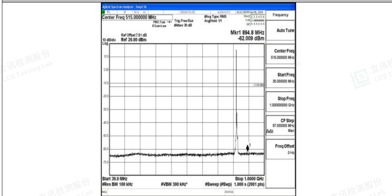
Band26_5MHz_16QAM_26815_1RB#0_30~1000_30~1000
