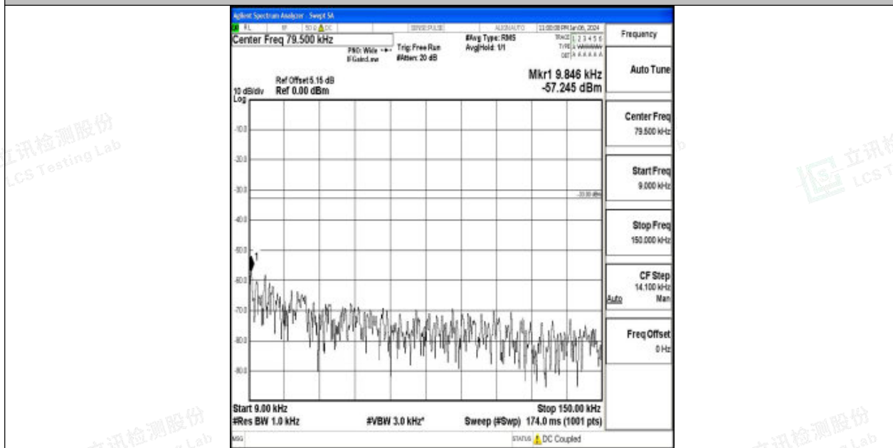
Band26_15MHz_16QAM_26865_1RB#0_0.009~0.15_0.009~0.15
