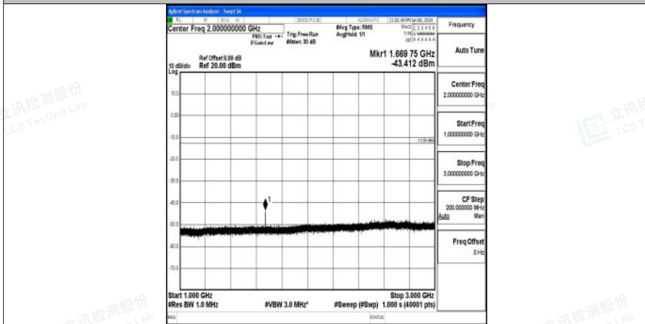
Band26_15MHz_QPSK_26965_1RB#0_1000~3000_1000~3000
