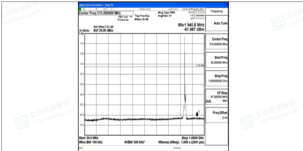
Band26_10MHz_QPSK_26990_1RB#0_30~1000_30~1000
