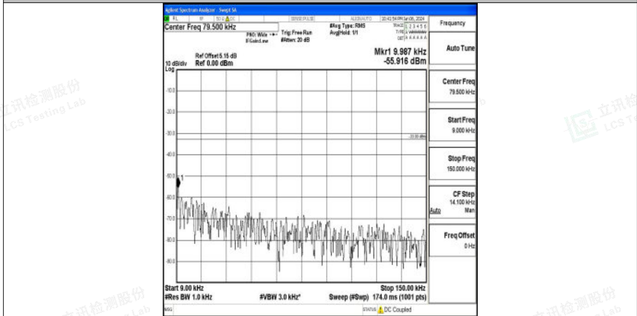
Band26_10MHz_16QAM_26840_1RB#0_0.009~0.15_0.009~0.15
