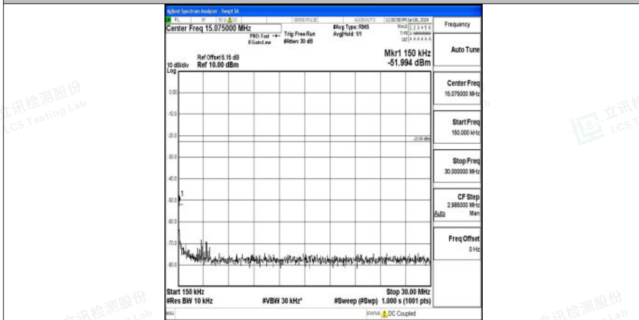
Band26_15MHz_QPSK_26915_1RB#0_0.15~30_0.15~30
