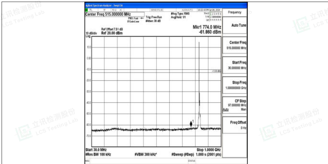
Band26_5MHz_QPSK_26915_1RB#0_30~1000_30~1000
