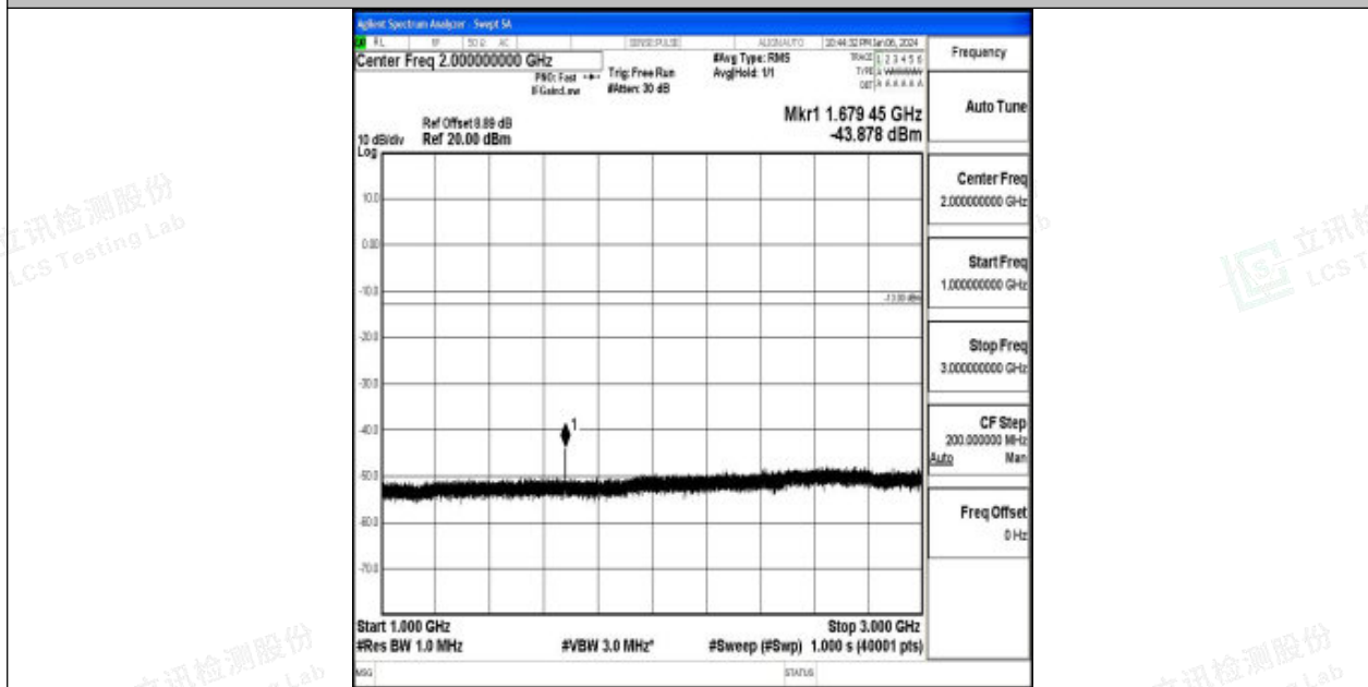
Band26_10MHz_QPSK_26990_1RB#0_1000~3000_1000~3000
