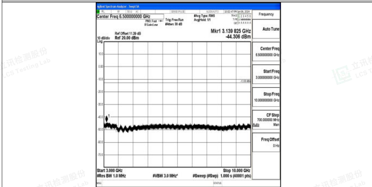
Band26_3MHz_16QAM_26915_1RB#0_3000~10000_3000~10000
