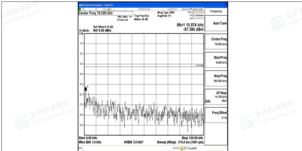
Band26_10MHz_QPSK_26840_1RB#0_0.009~0.15_0.009~0.15
