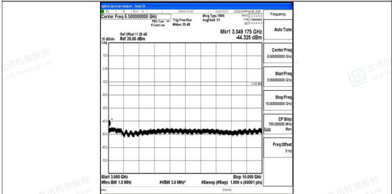
Band26_5MHz_16QAM_26815_1RB#0_3000~10000_3000~10000
