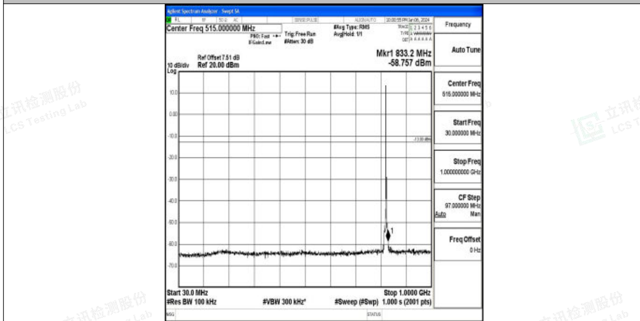
Band26_3MHz_16QAM_26805_1RB#0_30~1000_30~1000
