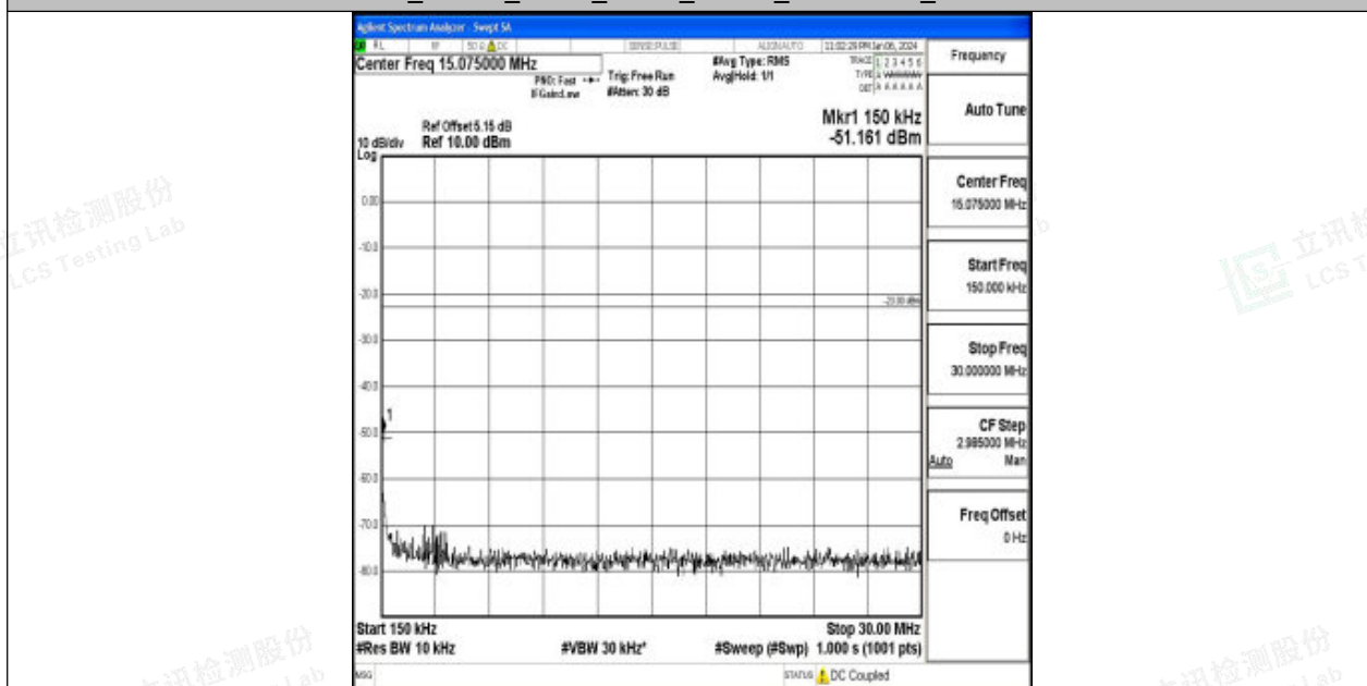
Band26_15MHz_QPSK_26965_1RB#0_0.15~30_0.15~30
