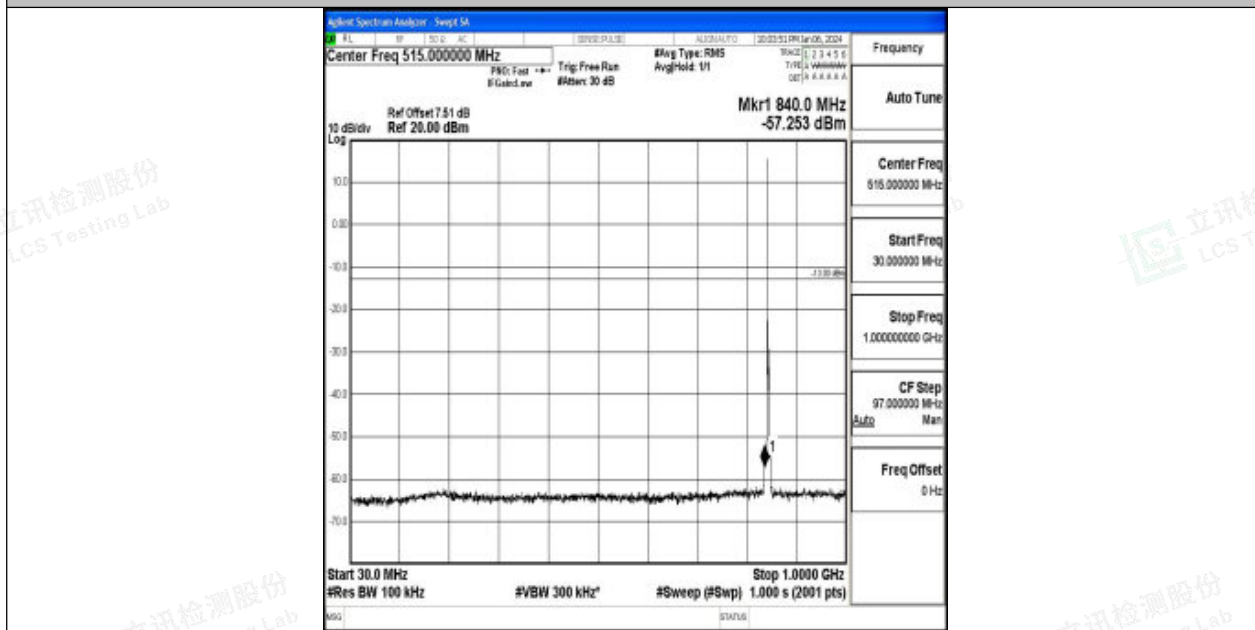
Band26_3MHz_16QAM_27025_1RB#0_30~1000_30~1000
