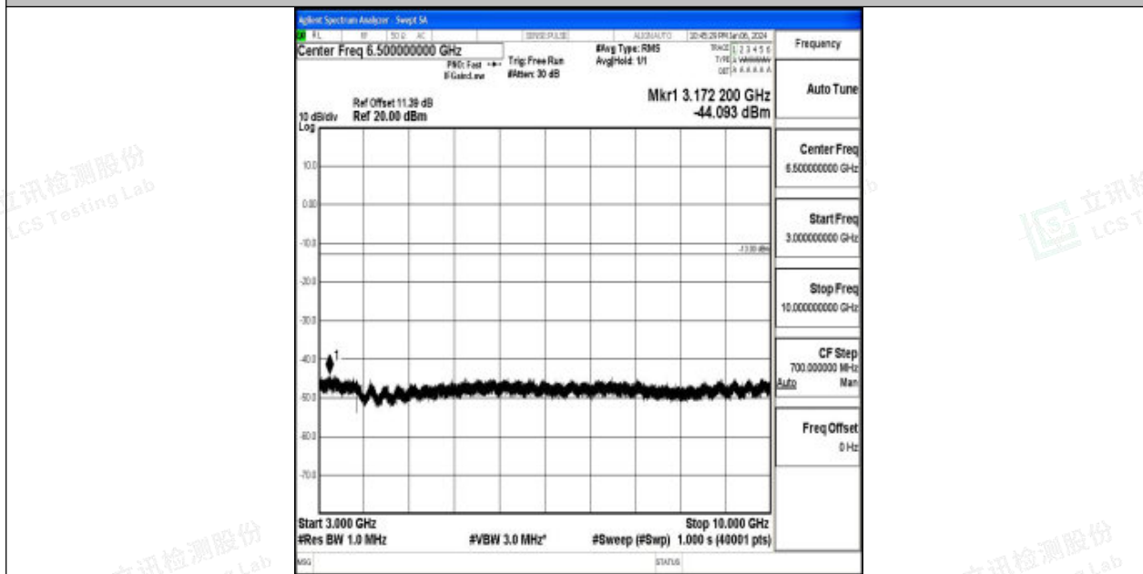
Band26_10MHz_16QAM_26990_1RB#0_3000~10000_3000~10000
