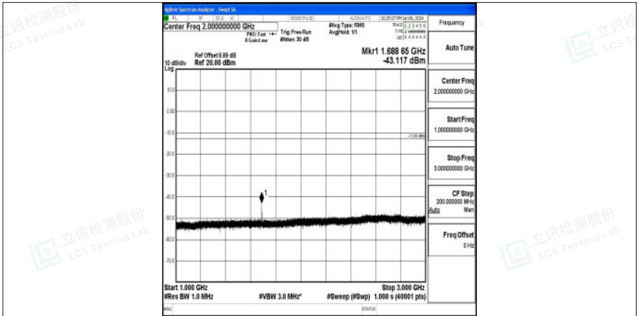
Band26_5MHz_16QAM_27015_1RB#0_1000~3000_1000~3000
