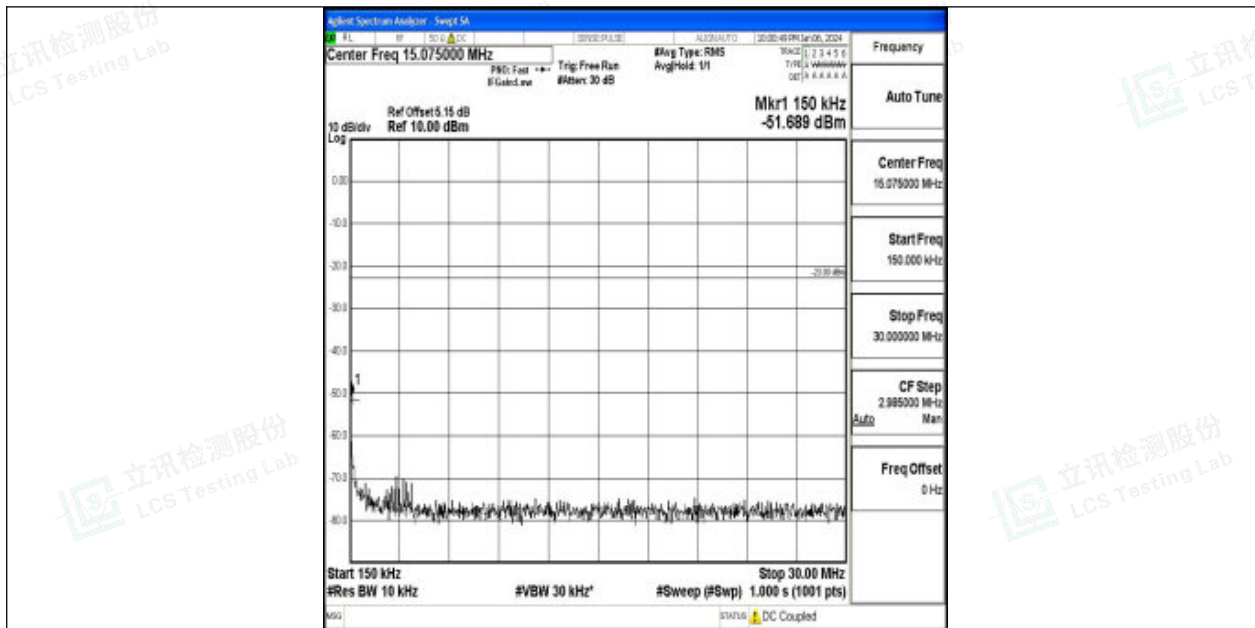
Band26_3MHz_16QAM_26805_1RB#0_0.15~30_0.15~30
