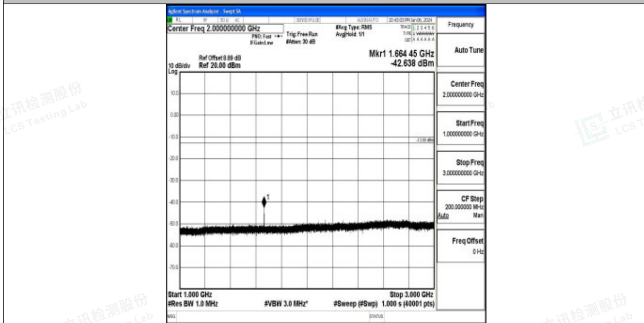
Band26_10MHz_QPSK_26915_1RB#0_1000~3000_1000~3000
