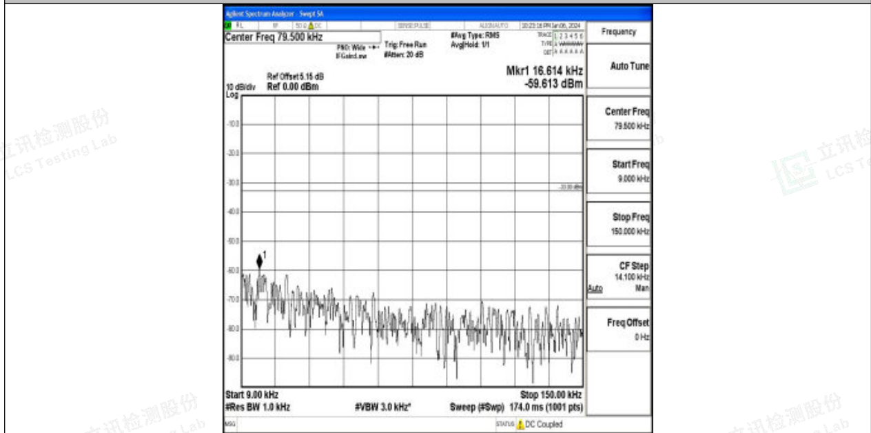
Band26_5MHz_16QAM_26915_1RB#0_0.009~0.15_0.009~0.15
