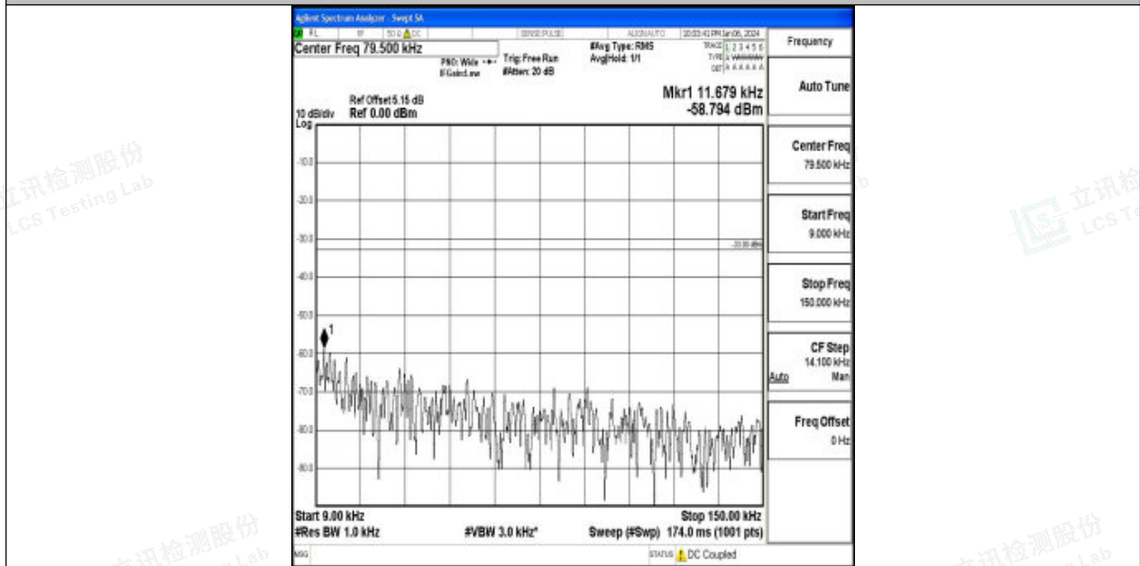
Band26_3MHz_16QAM_27025_1RB#0_0.009~0.15_0.009~0.15
