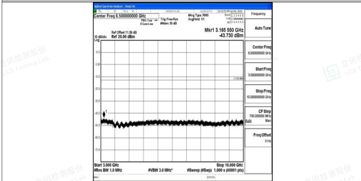
Band26_5MHz_16QAM_26915_1RB#0_3000~10000_3000~10000
