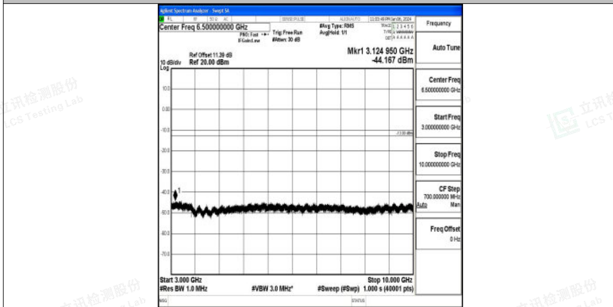
Band26_15MHz_16QAM_26965_1RB#0_3000~10000_3000~10000
