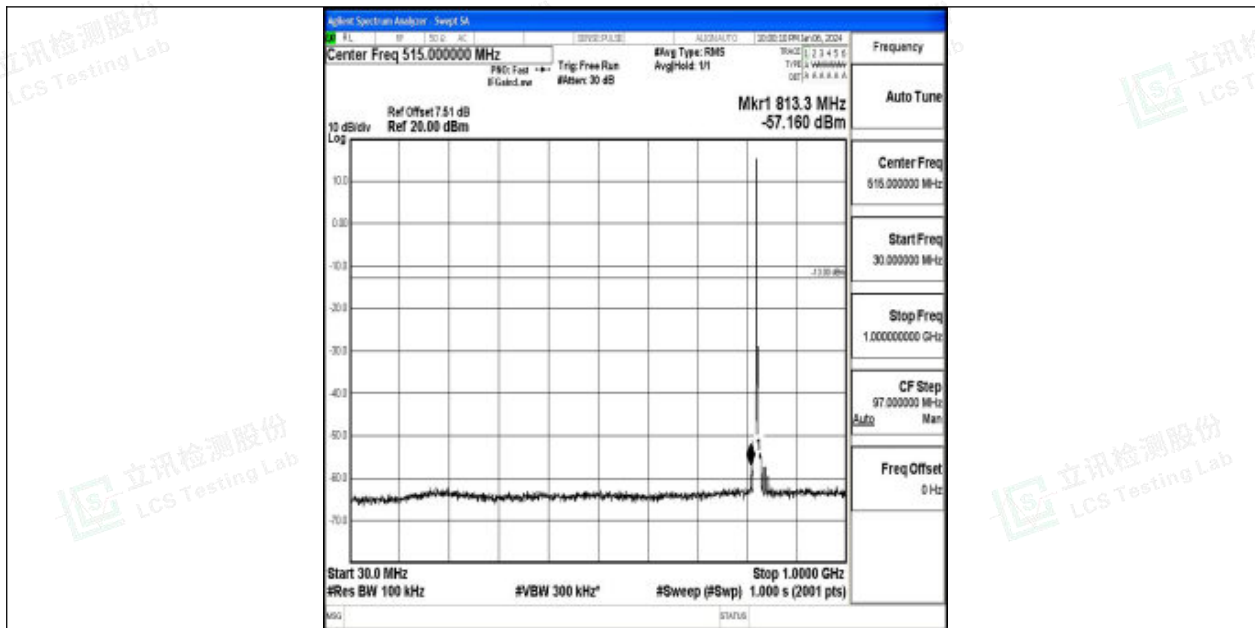
Band26_3MHz_QPSK_26805_1RB#0_30~1000_30~1000
