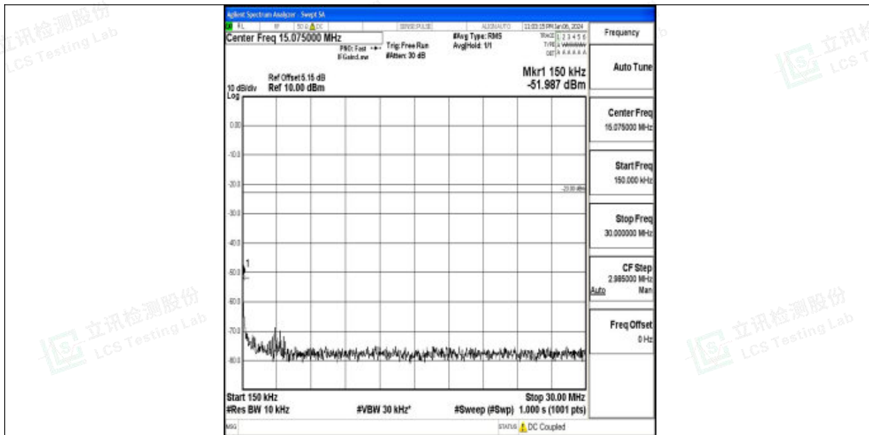
Band26_15MHz_16QAM_26965_1RB#0_0.15~30_0.15~30
