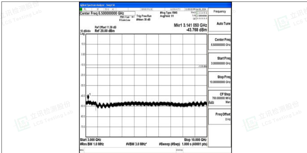
Band26_15MHz_QPSK_26865_1RB#0_3000~10000_3000~10000
