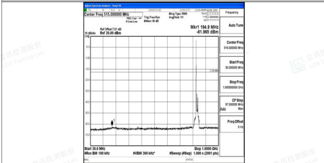
Band26_15MHz_16QAM_26915_1RB#0_30~1000_30~1000
