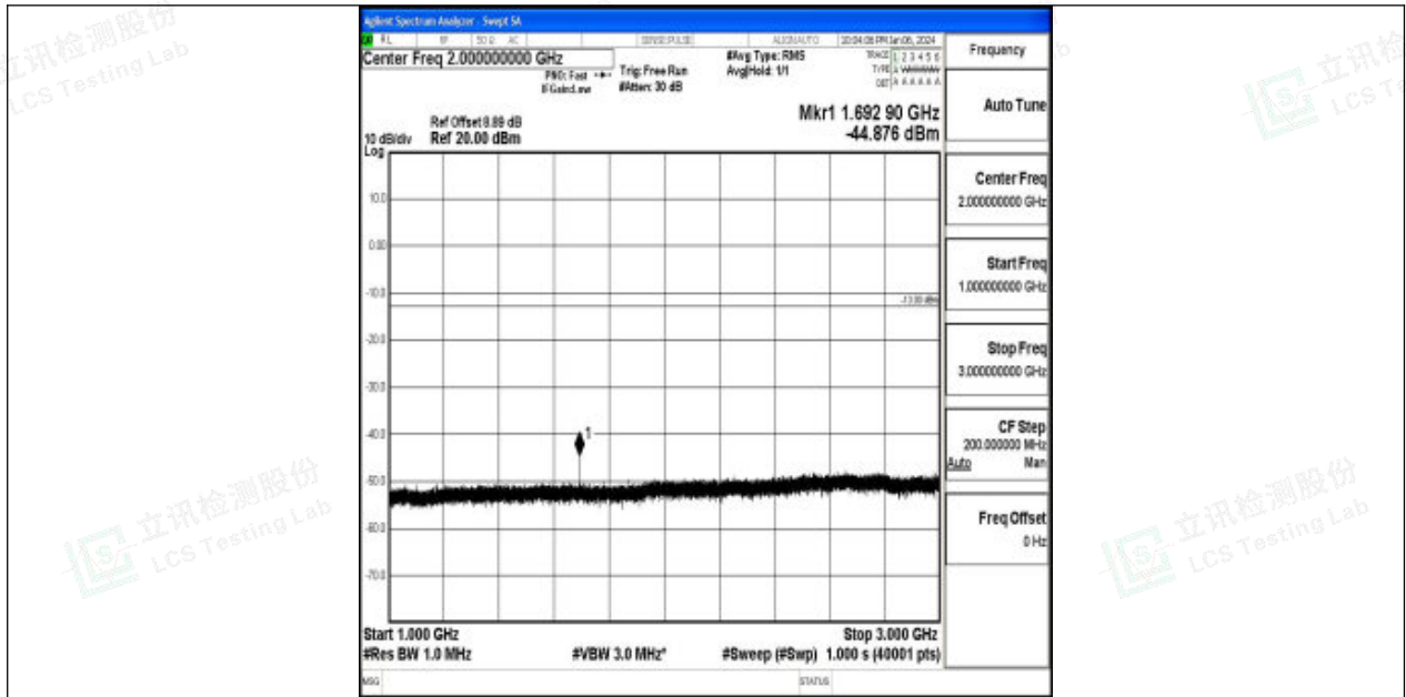
Band26_3MHz_16QAM_27025_1RB#0_1000~3000_1000~3000
