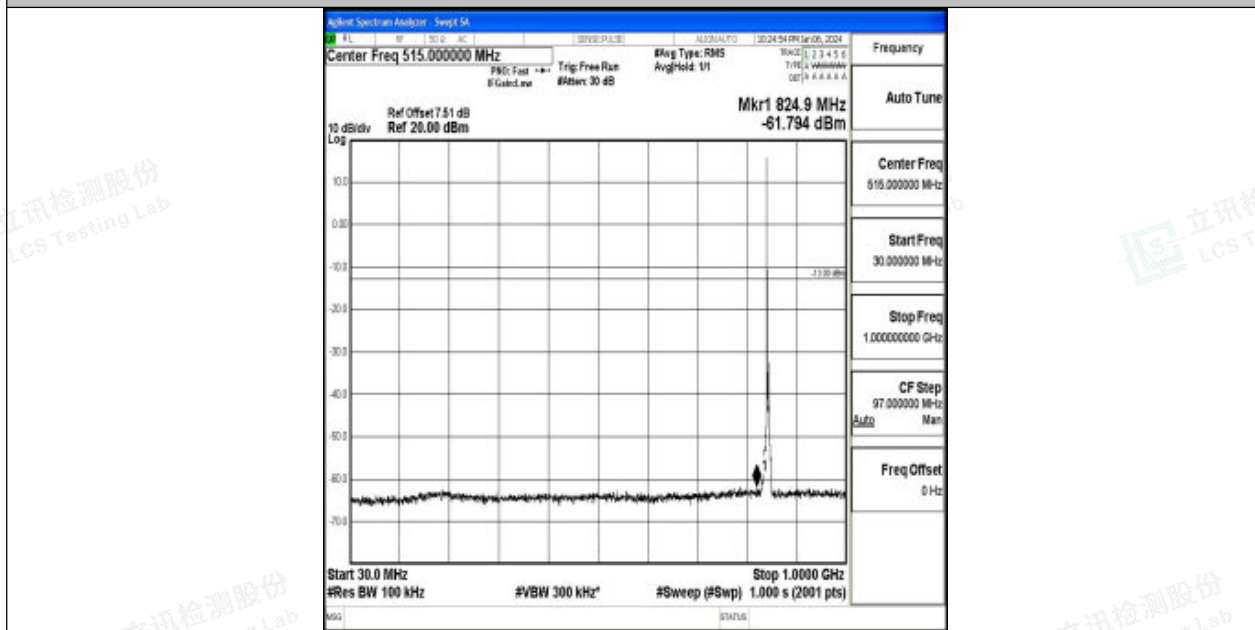
Band26_5MHz_16QAM_27015_1RB#0_30~1000_30~1000
