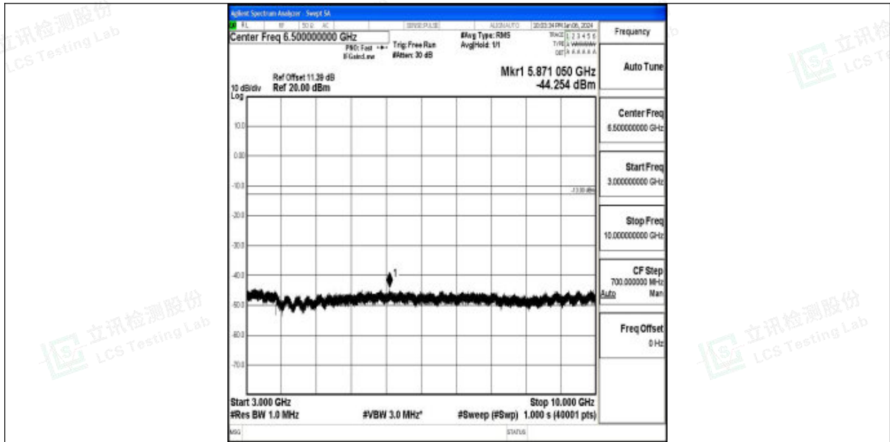
Band26_3MHz_QPSK_27025_1RB#0_3000~10000_3000~10000
