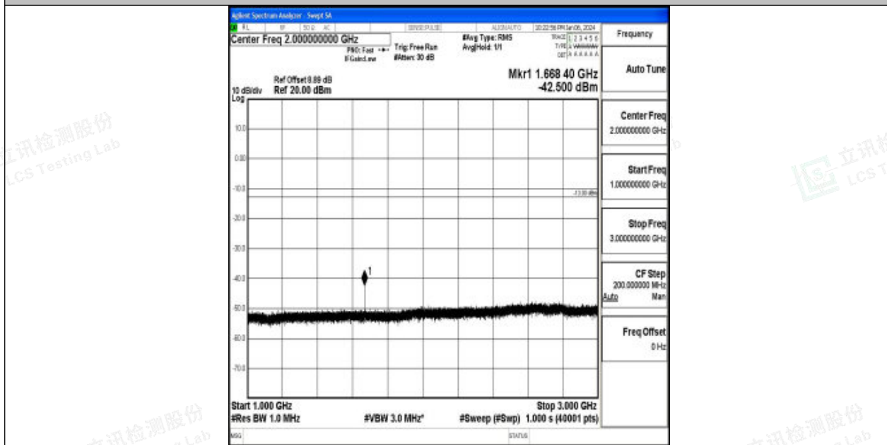
Band26_5MHz_QPSK_26915_1RB#0_1000~3000_1000~3000
