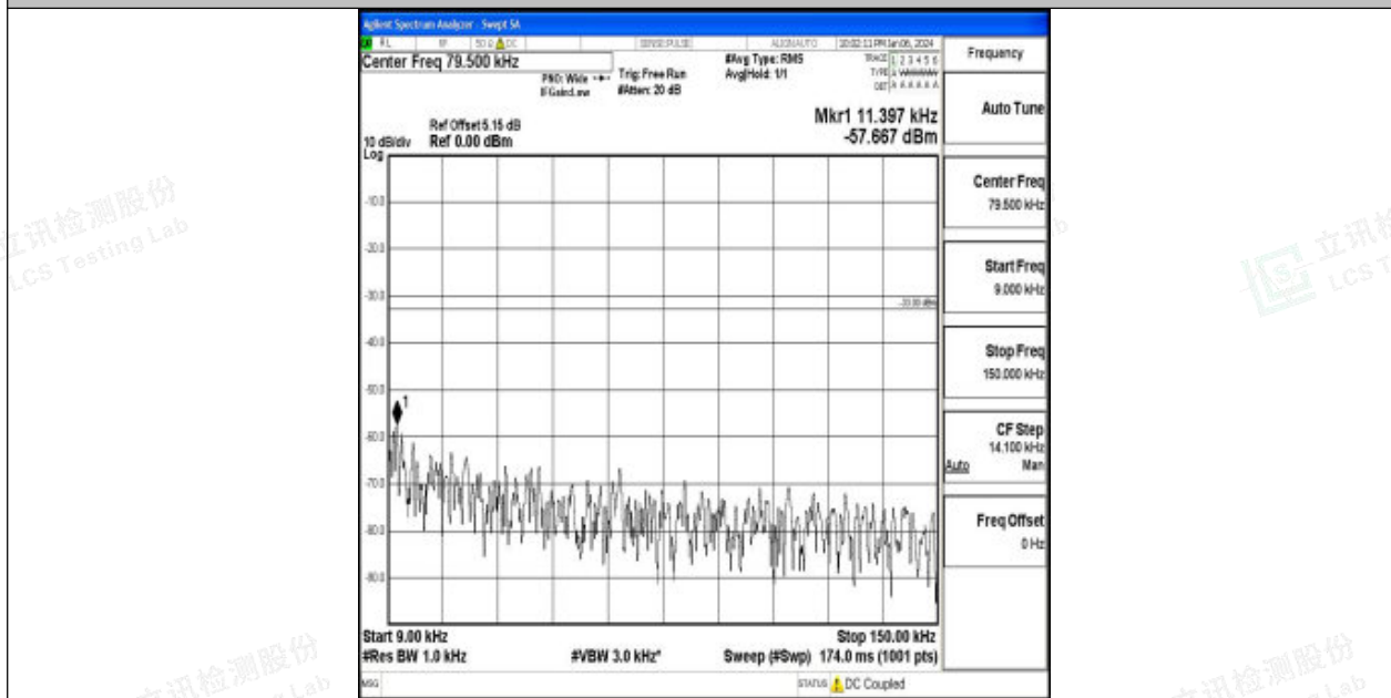
Band26_3MHz_16QAM_26915_1RB#0_0.009~0.15_0.009~0.15
