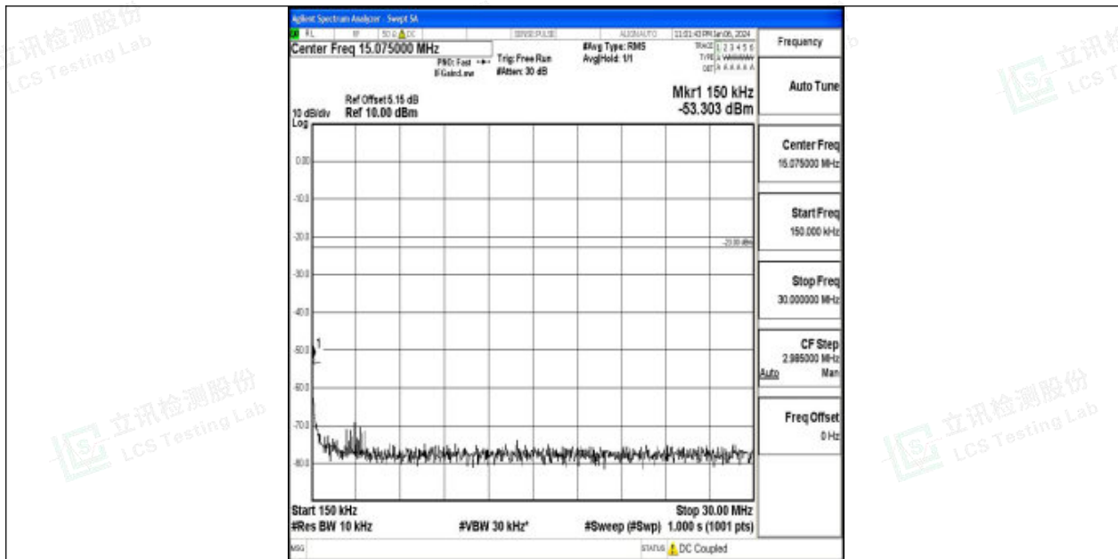
Band26_15MHz_16QAM_26915_1RB#0_0.15~30_0.15~30
