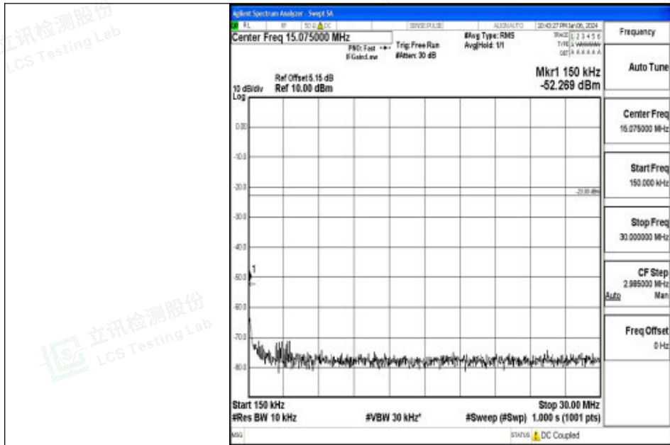
Band26_10MHz_16QAM_26915_1RB#0_0.15~30_0.15~30
