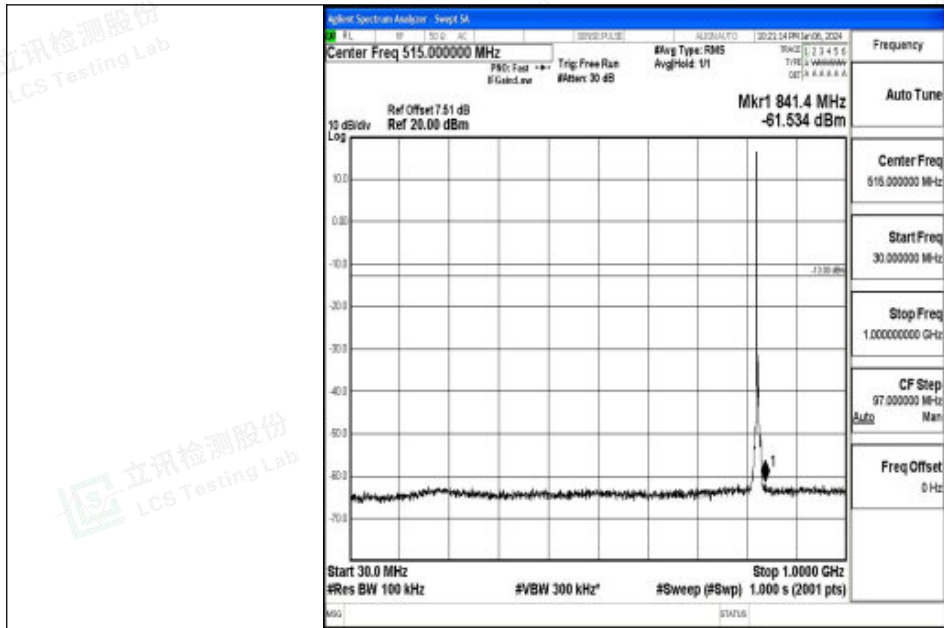
Band26_5MHz_QPSK_26815_1RB#0_30~1000_30~1000
