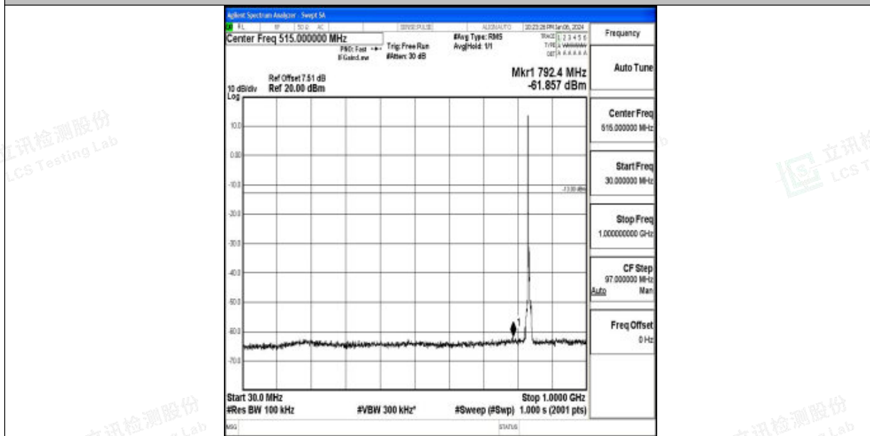
Band26_5MHz_16QAM_26915_1RB#0_30~1000_30~1000
