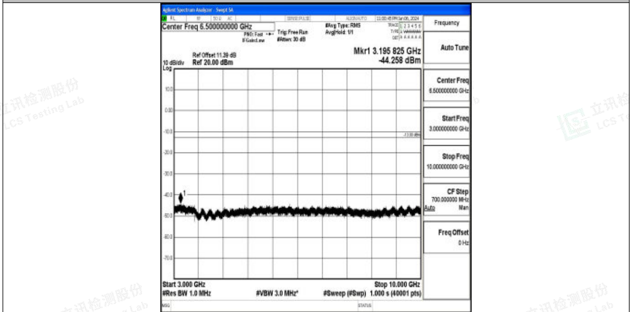
Band26_15MHz_16QAM_26865_1RB#0_3000~10000_3000~10000
