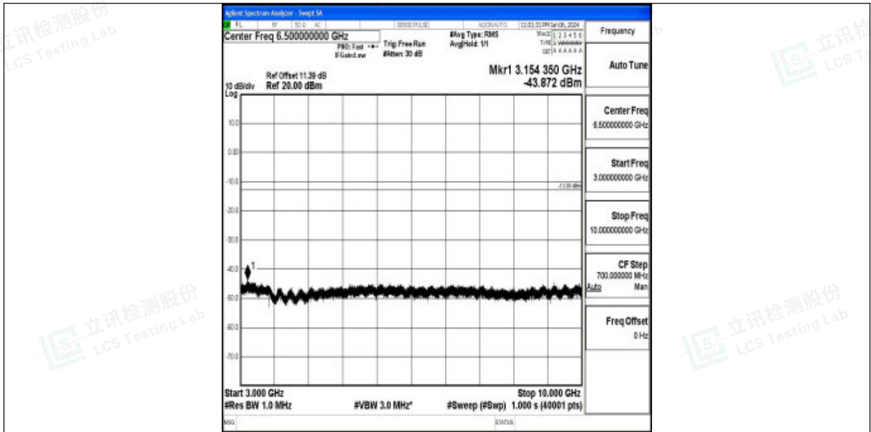
Band26_15MHz_QPSK_26915_1RB#0_3000~10000_3000~10000
