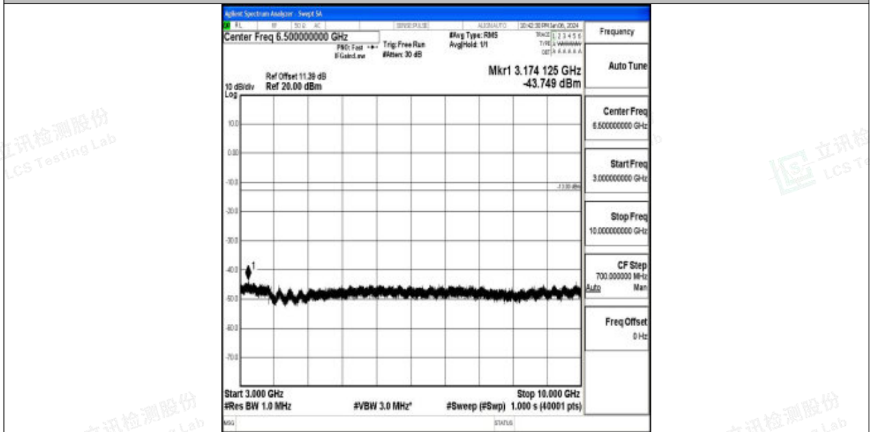
Band26_10MHz_16QAM_26840_1RB#0_3000~10000_3000~10000
