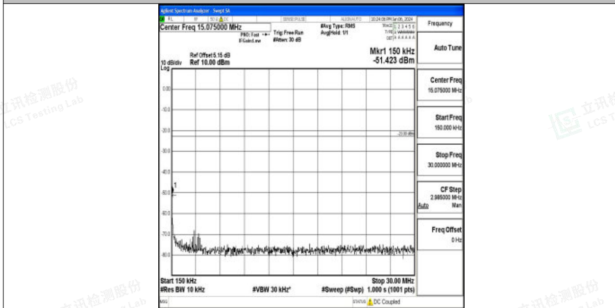
Band26_5MHz_QPSK_27015_1RB#0_0.15~30_0.15~30
