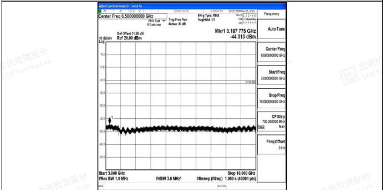
Band26_5MHz_16QAM_27015_1RB#0_3000~10000_3000~10000
