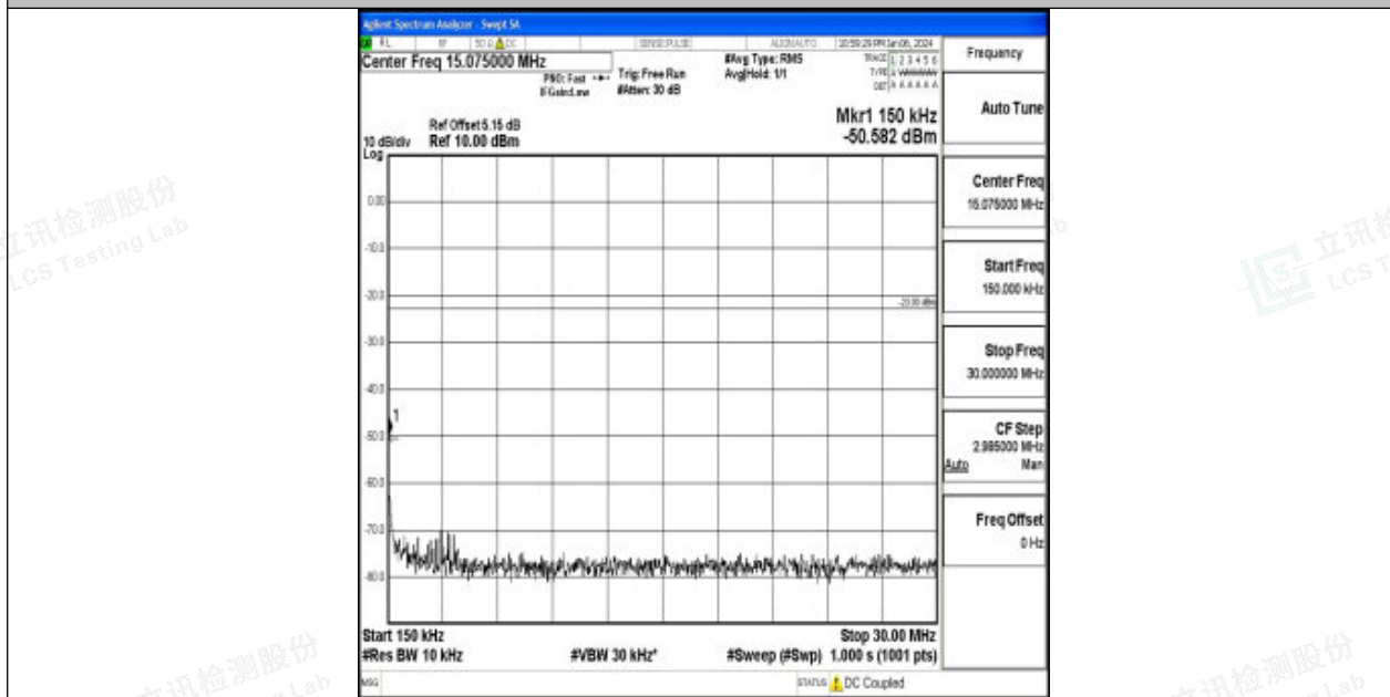
Band26_15MHz_QPSK_26865_1RB#0_0.15~30_0.15~30
