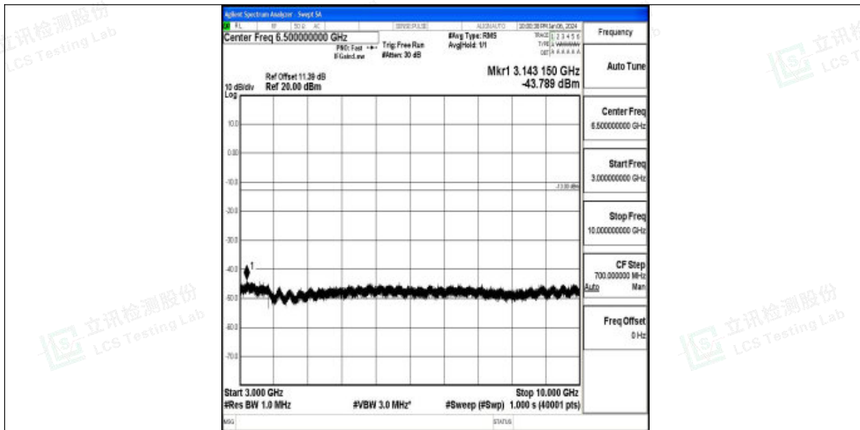
Band26_3MHz_QPSK_26805_1RB#0_3000~10000_3000~10000
