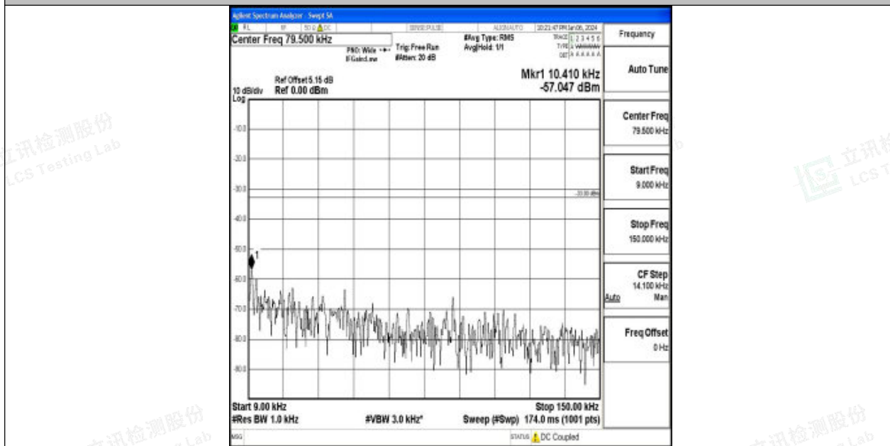
Band26_5MHz_16QAM_26815_1RB#0_0.009~0.15_0.009~0.15
