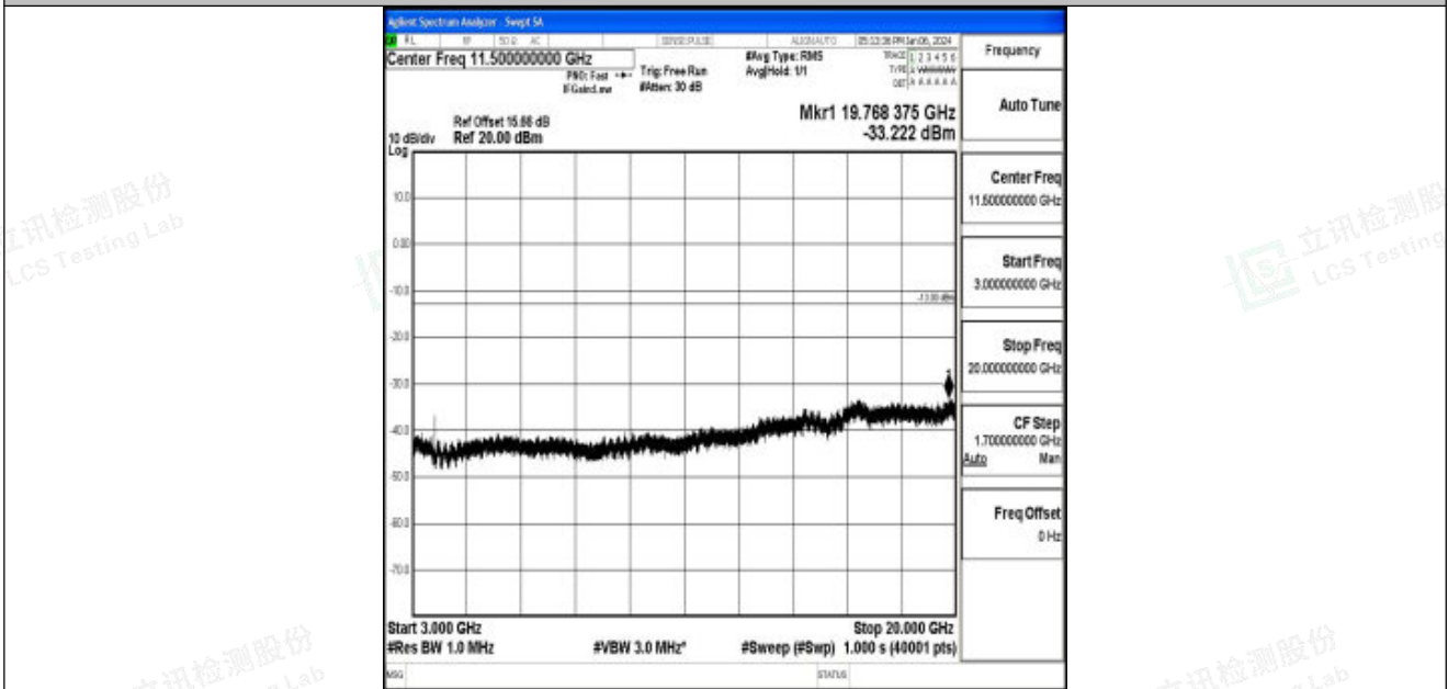
Band25_5MHz_QPSK_26065_1RB#0_3000~20000_3000~20000
