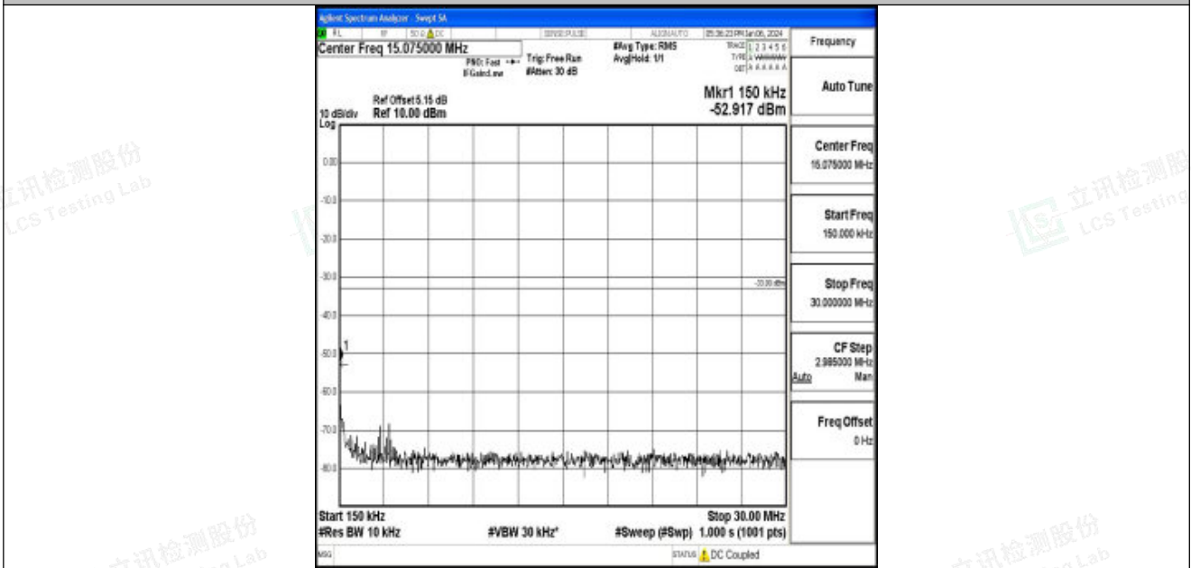
Band25_10MHz_16QAM_26640_1RB#0_0.15~30_0.15~30
