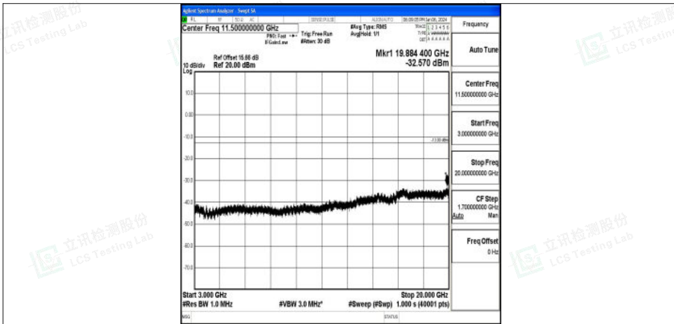
Band25_20MHz_16QAM_26590_1RB#0_3000~20000_3000~20000
