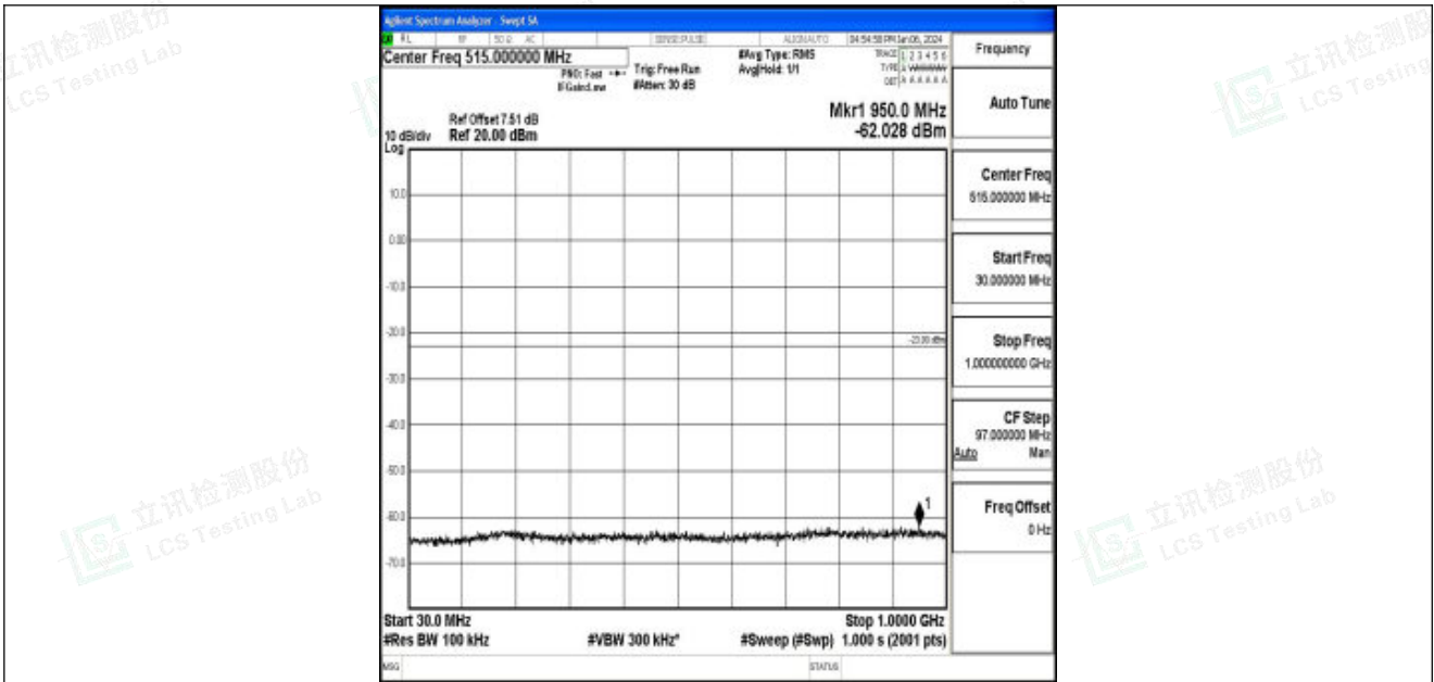
Band25_3MHz_16QAM_26055_1RB#0_30~1000_30~1000
