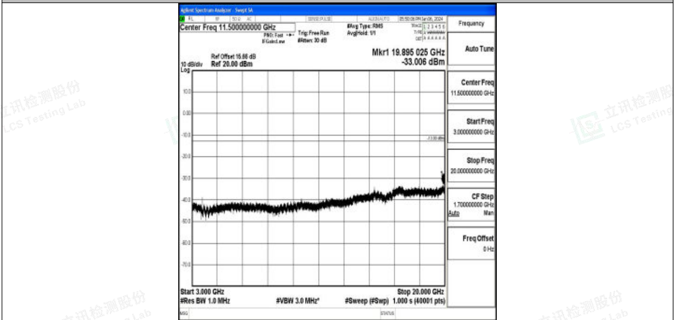
Band25_15MHz_QPSK_26115_1RB#0_3000~20000_3000~20000
