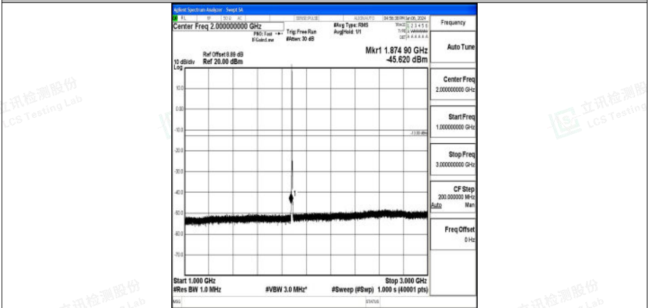
Band25_3MHz_16QAM_26365_1RB#0_1000~3000_1000~3000
