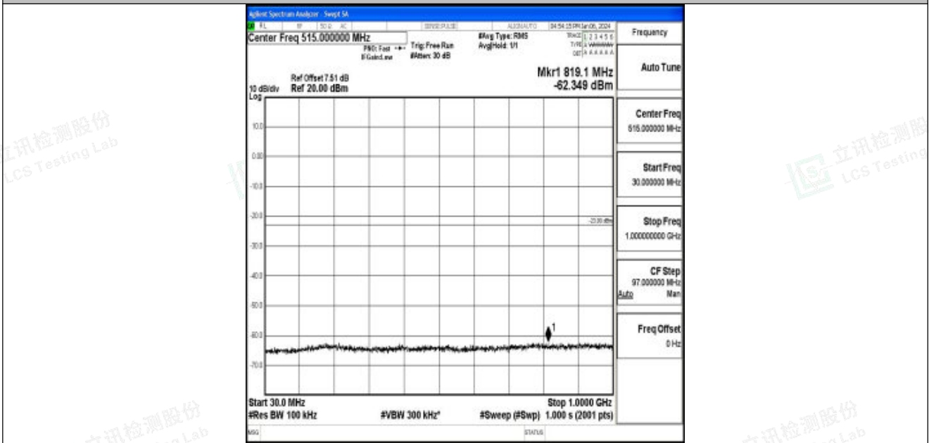
Band25_3MHz_QPSK_26055_1RB#0_30~1000_30~1000
