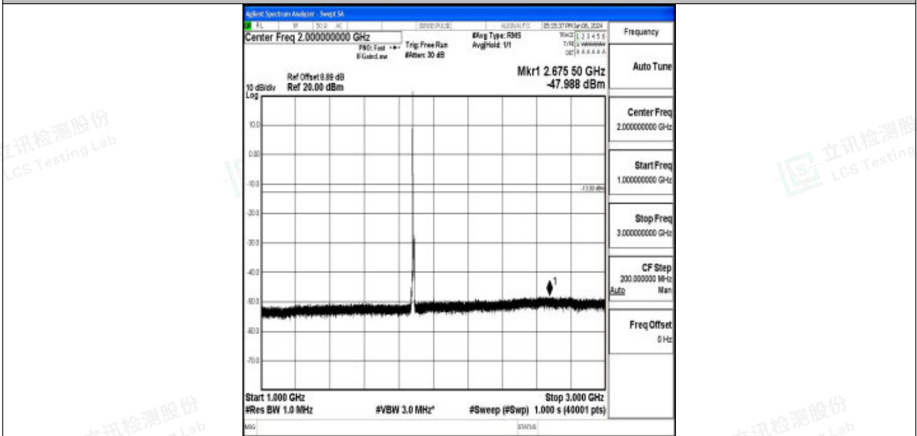
Band25_5MHz_16QAM_26365_1RB#0_1000~3000_1000~3000
