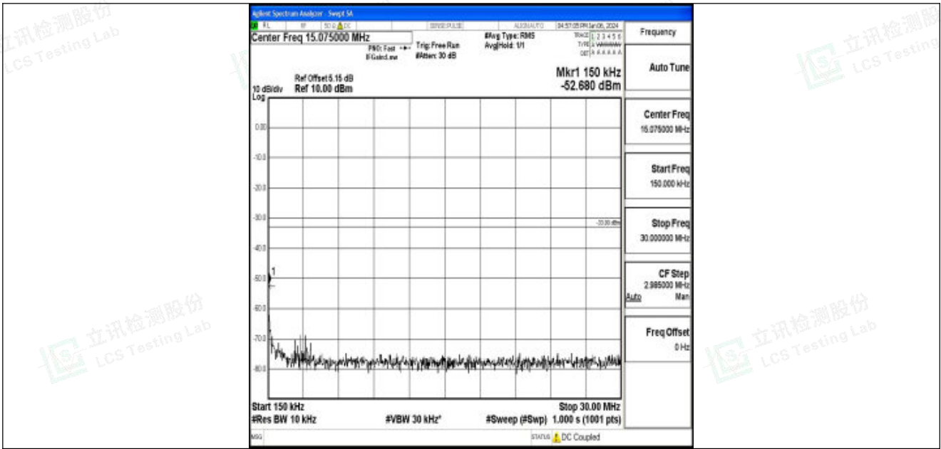
Band25_3MHz_QPSK_26675_1RB#0_0.15~30_0.15~30
