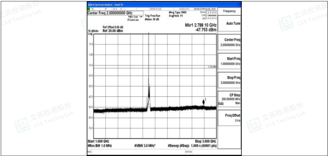
Band25_20MHz_QPSK_26590_1RB#0_1000~3000_1000~3000
