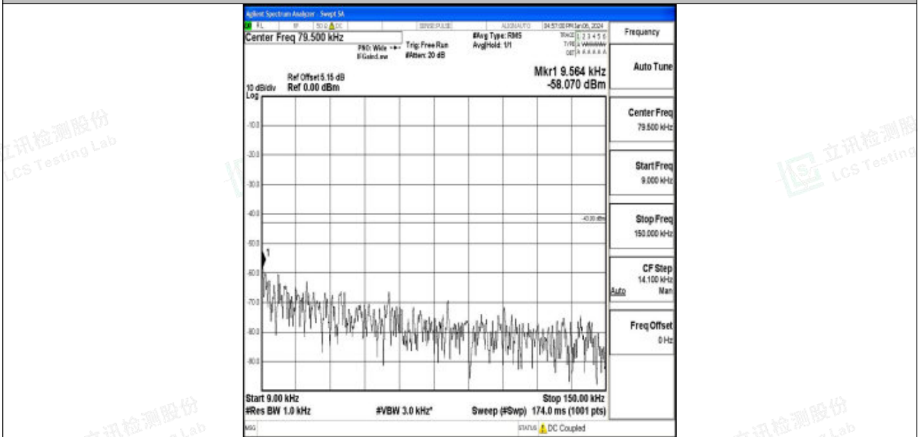
Band25_3MHz_QPSK_26675_1RB#0_0.009~0.15_0.009~0.15
