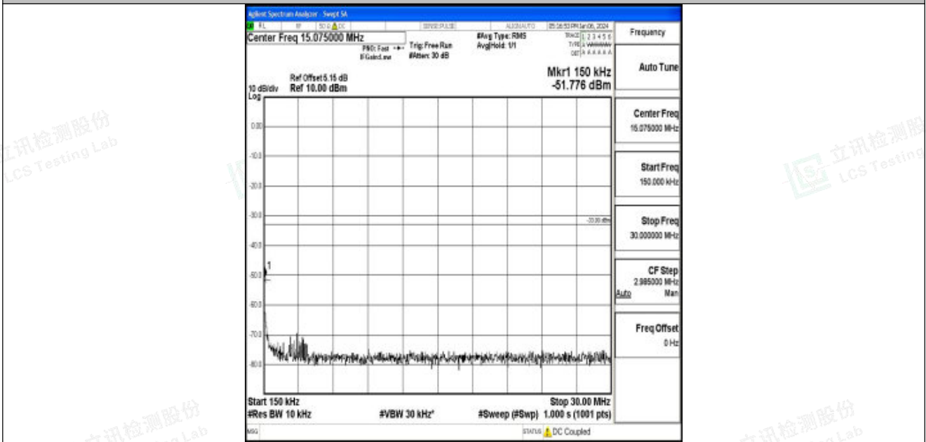
Band25_5MHz_16QAM_26665_1RB#0_0.15~30_0.15~30
