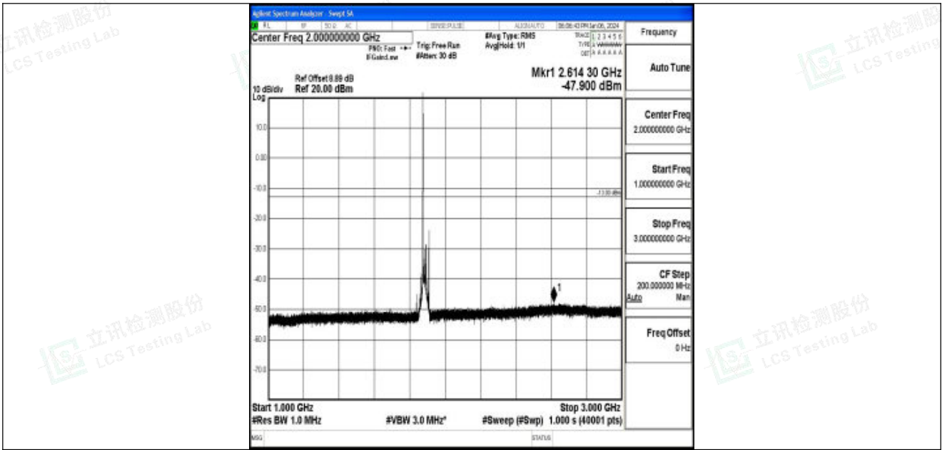
Band25_20MHz_QPSK_26365_1RB#0_1000~3000_1000~3000
