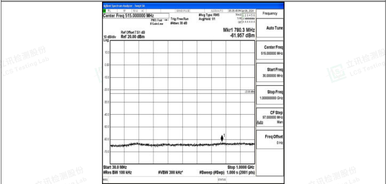
Band25_10MHz_QPSK_26640_1RB#0_30~1000_30~1000
