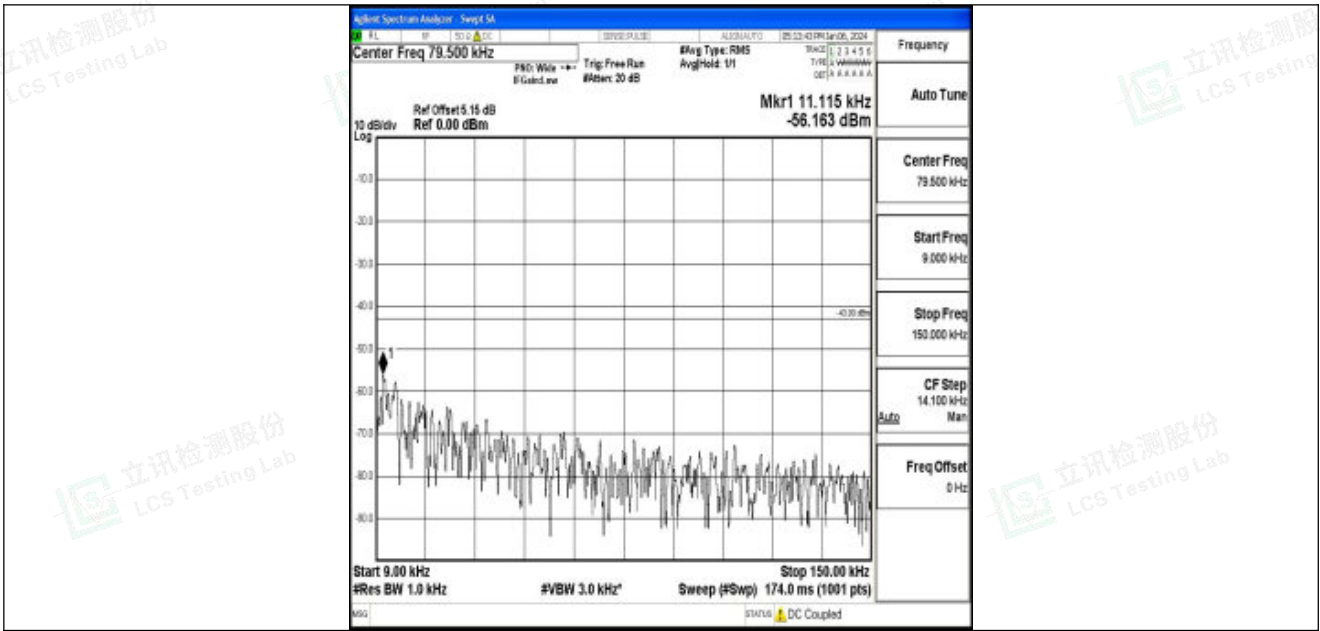
Band25_5MHz_16QAM_26065_1RB#0_0.009~0.15_0.009~0.15
