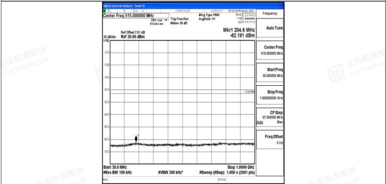
Band25_10MHz_QPSK_26090_1RB#0_30~1000_30~1000
