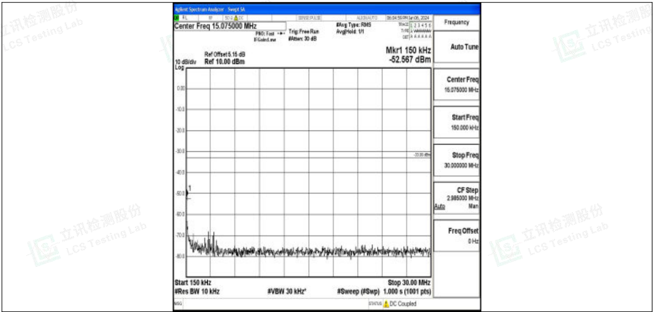
Band25_20MHz_QPSK_26140_1RB#0_0.15~30_0.15~30
