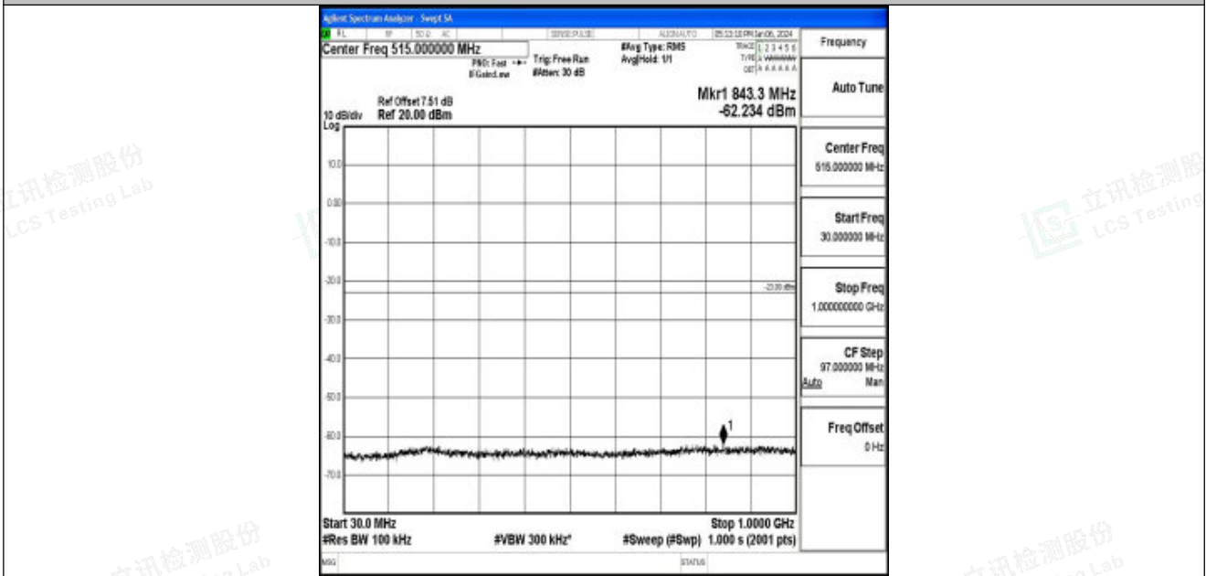
Band25_5MHz_QPSK_26065_1RB#0_30~1000_30~1000
