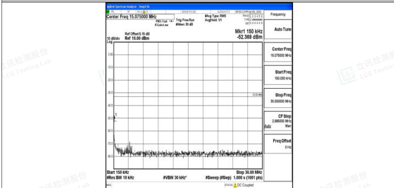
Band25_15MHz_16QAM_26615_1RB#0_0.15~30_0.15~30
