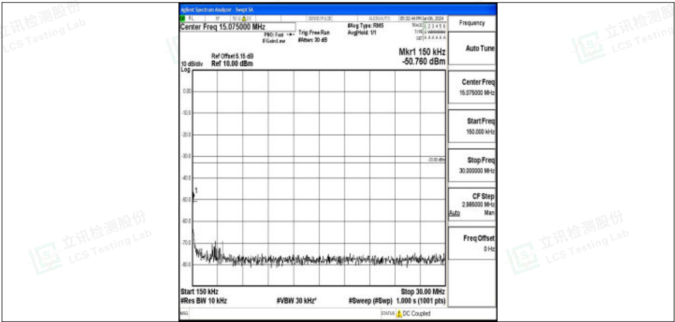
Band25_10MHz_QPSK_26090_1RB#0_0.15~30_0.15~30
