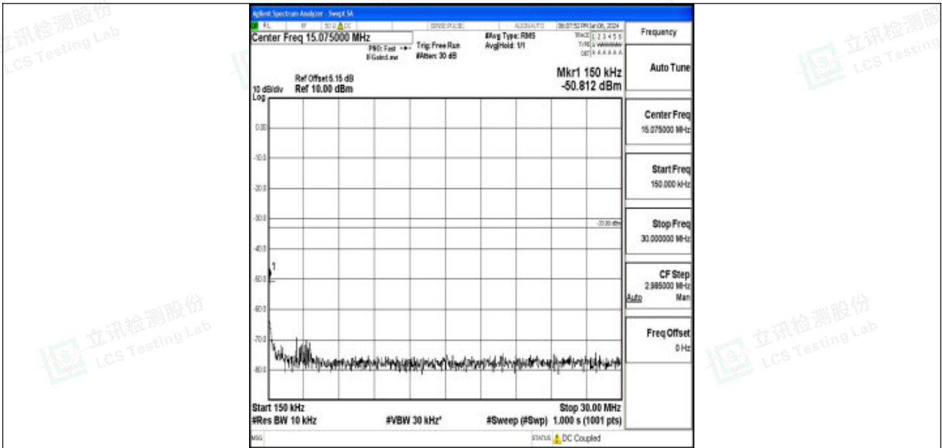
Band25_20MHz_QPSK_26590_1RB#0_0.15~30_0.15~30
