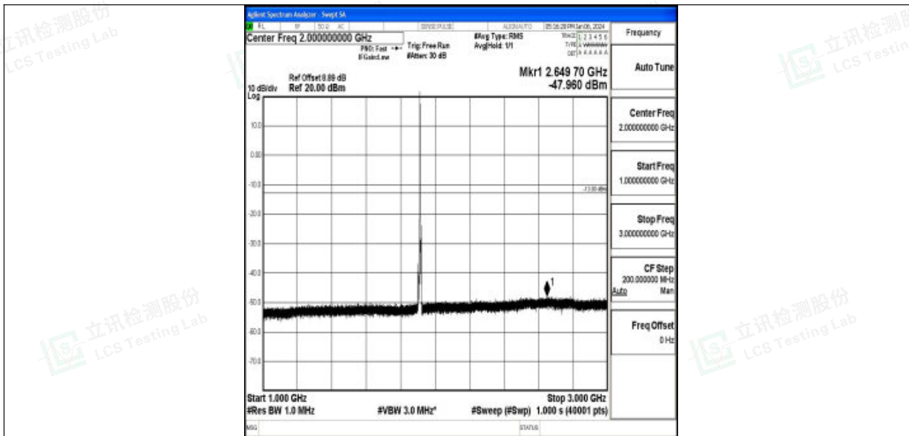
Band25_5MHz_QPSK_26665_1RB#0_1000~3000_1000~3000
