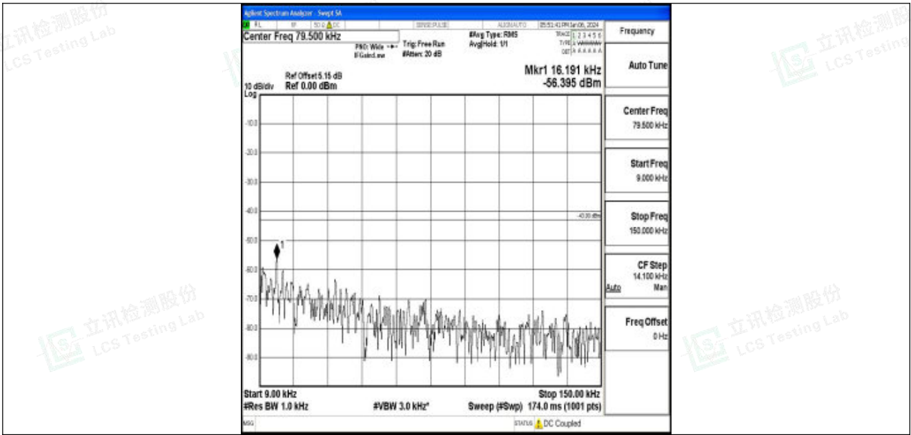
Band25_15MHz_16QAM_26365_1RB#0_0.009~0.15_0.009~0.15
