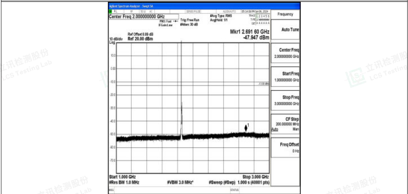
Band25_5MHz_16QAM_26065_1RB#0_1000~3000_1000~3000
