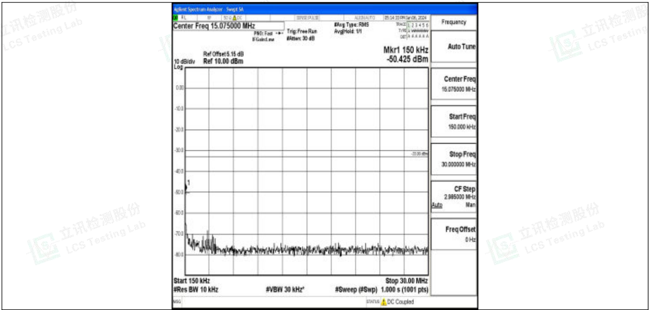
Band25_5MHz_QPSK_26365_1RB#0_0.15~30_0.15~30
