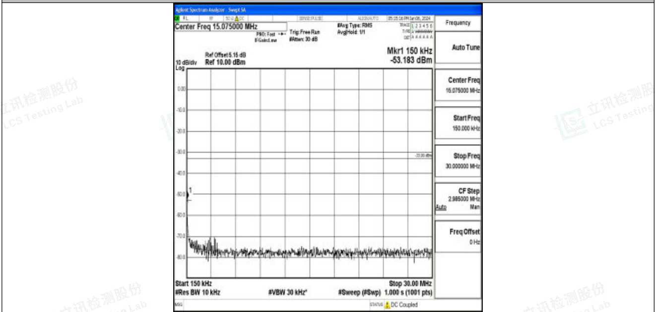
Band25_5MHz_16QAM_26365_1RB#0_0.15~30_0.15~30
