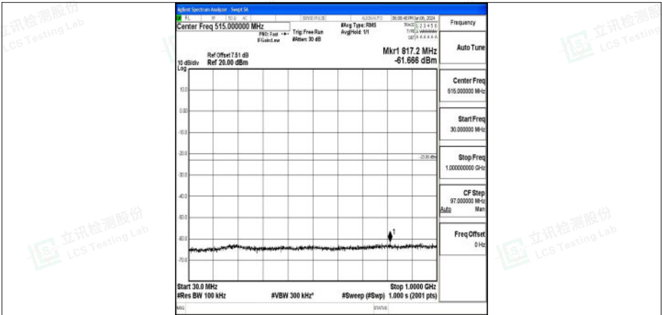
Band25_20MHz_16QAM_26590_1RB#0_30~1000_30~1000
