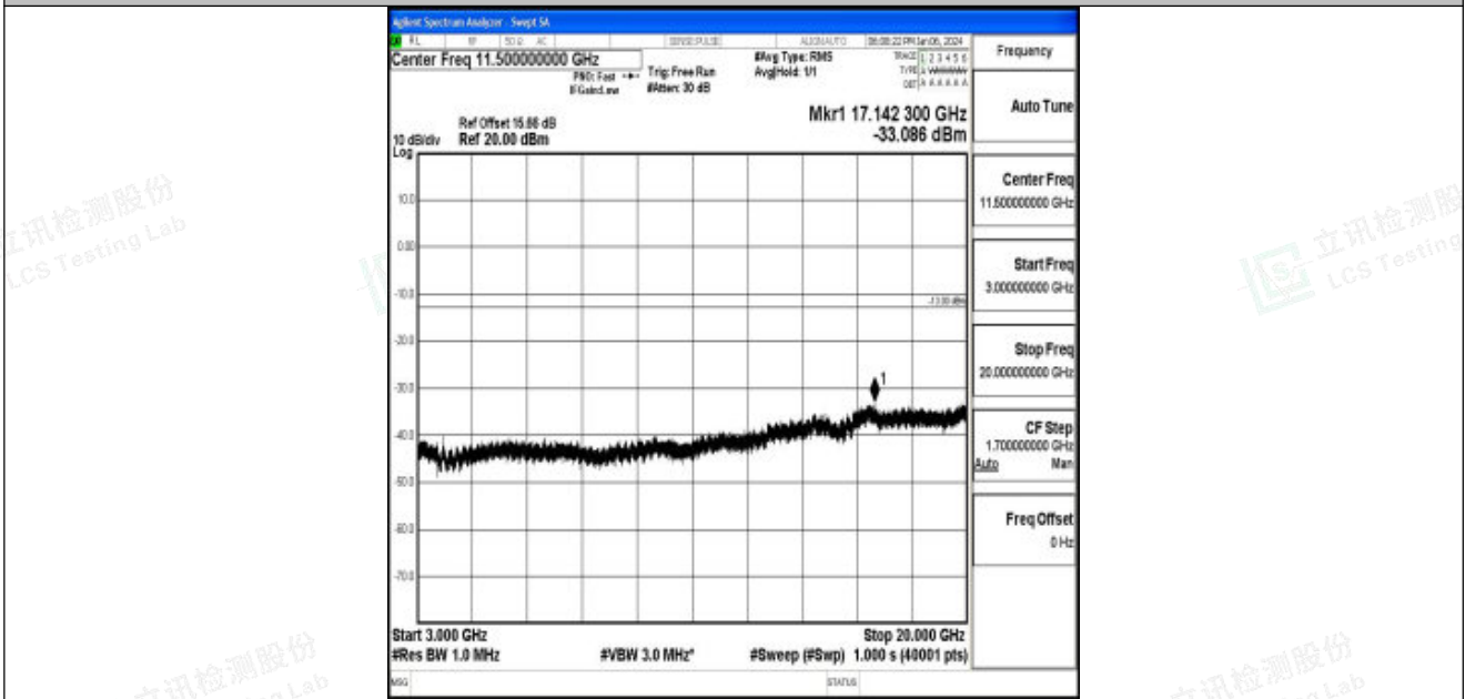
Band25_20MHz_QPSK_26590_1RB#0_3000~20000_3000~20000
