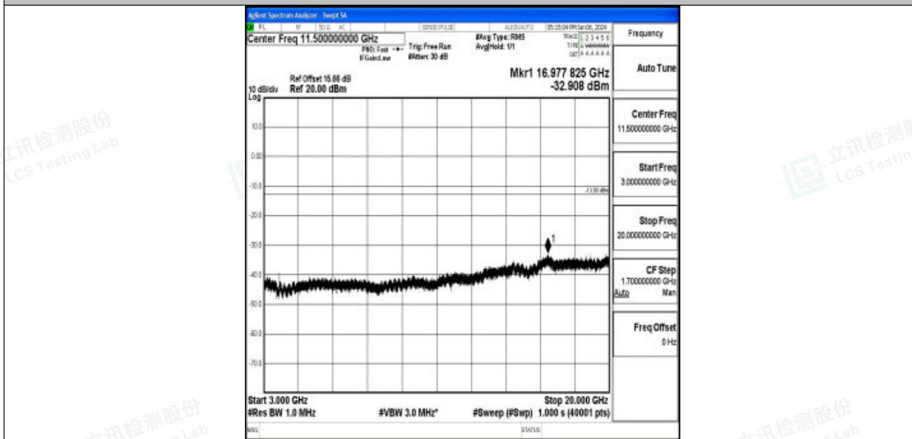
Band25_5MHz_QPSK_26365_1RB#0_3000~20000_3000~20000
