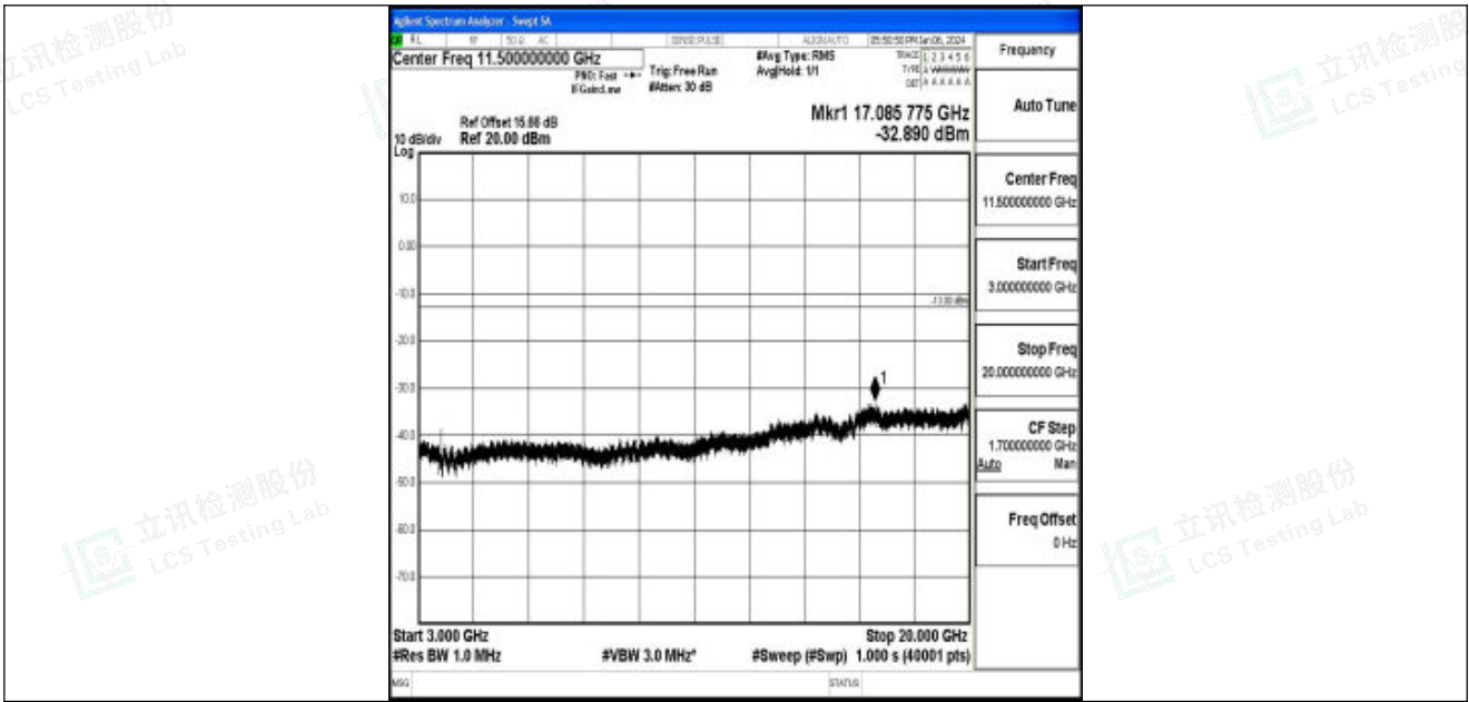
Band25_15MHz_16QAM_26115_1RB#0_3000~20000_3000~20000
