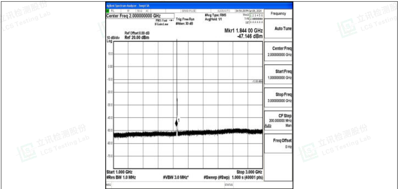
Band25_3MHz_QPSK_26055_1RB#0_1000~3000_1000~3000
