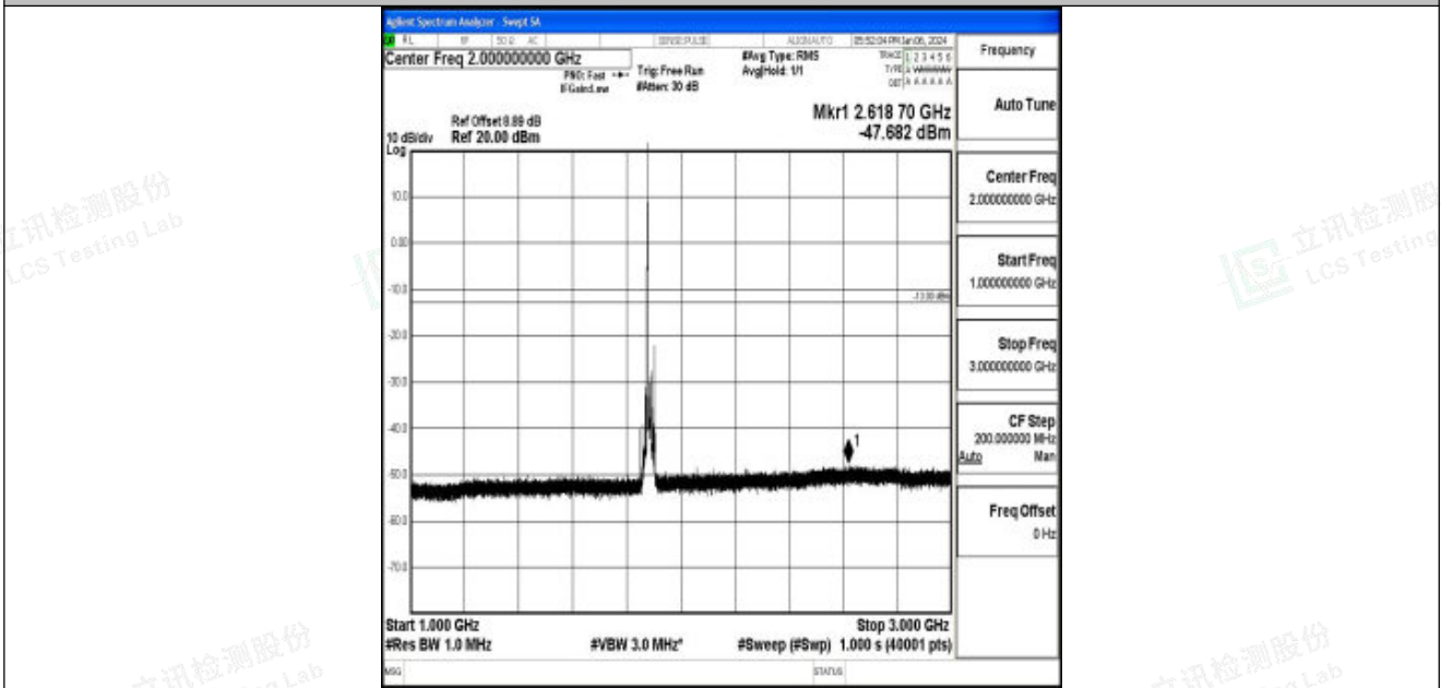
Band25_15MHz_16QAM_26365_1RB#0_1000~3000_1000~3000
