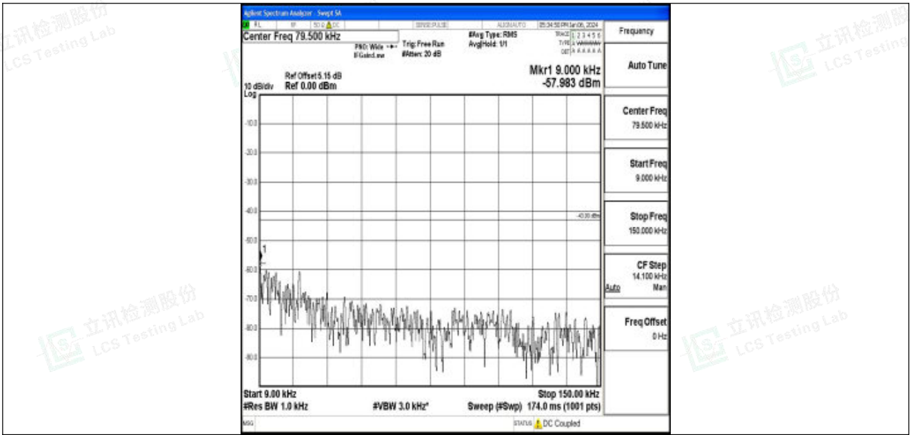
Band25_10MHz_16QAM_26365_1RB#0_0.009~0.15_0.009~0.15
