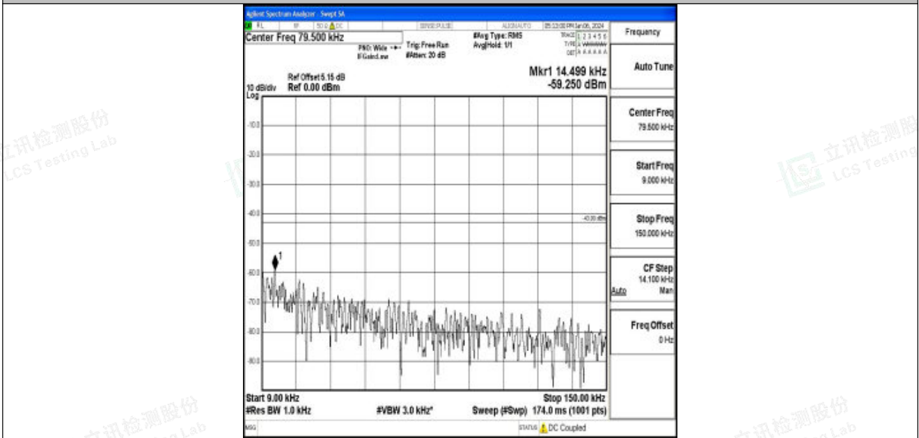
Band25_5MHz_QPSK_26065_1RB#0_0.009~0.15_0.009~0.15
