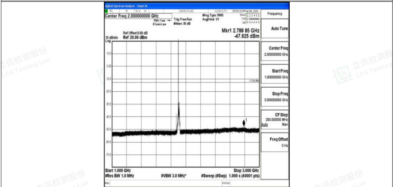
Band25_15MHz_16QAM_26615_1RB#0_1000~3000_1000~3000
