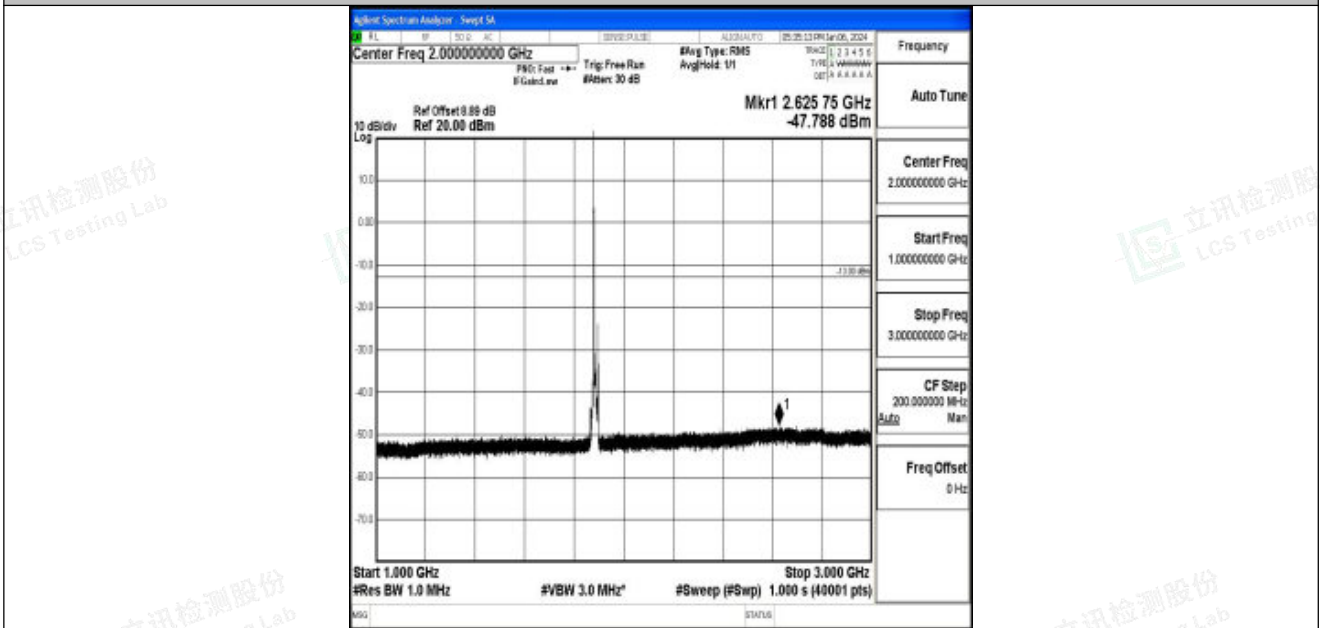
Band25_10MHz_16QAM_26365_1RB#0_1000~3000_1000~3000
