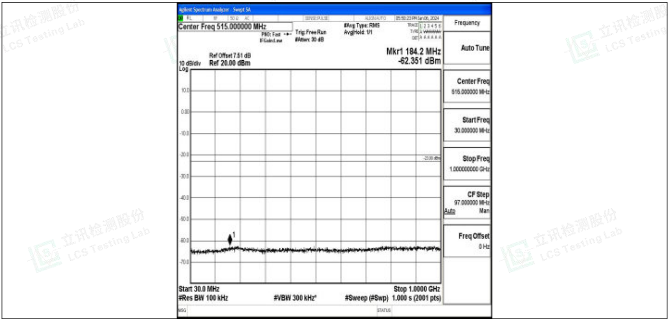
Band25_15MHz_16QAM_26115_1RB#0_30~1000_30~1000
