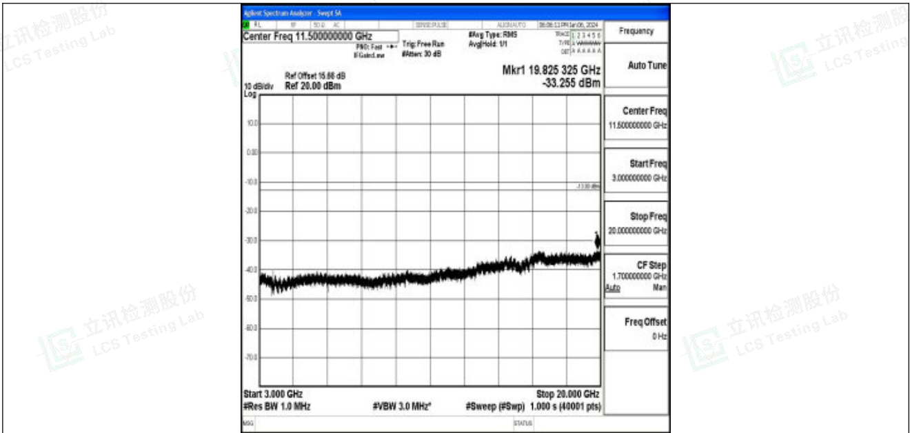
Band25_20MHz_16QAM_26140_1RB#0_3000~20000_3000~20000
