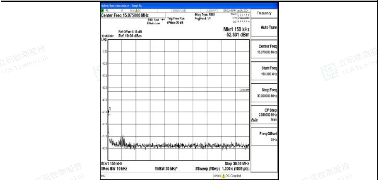
Band25_5MHz_16QAM_26065_1RB#0_0.15~30_0.15~30
