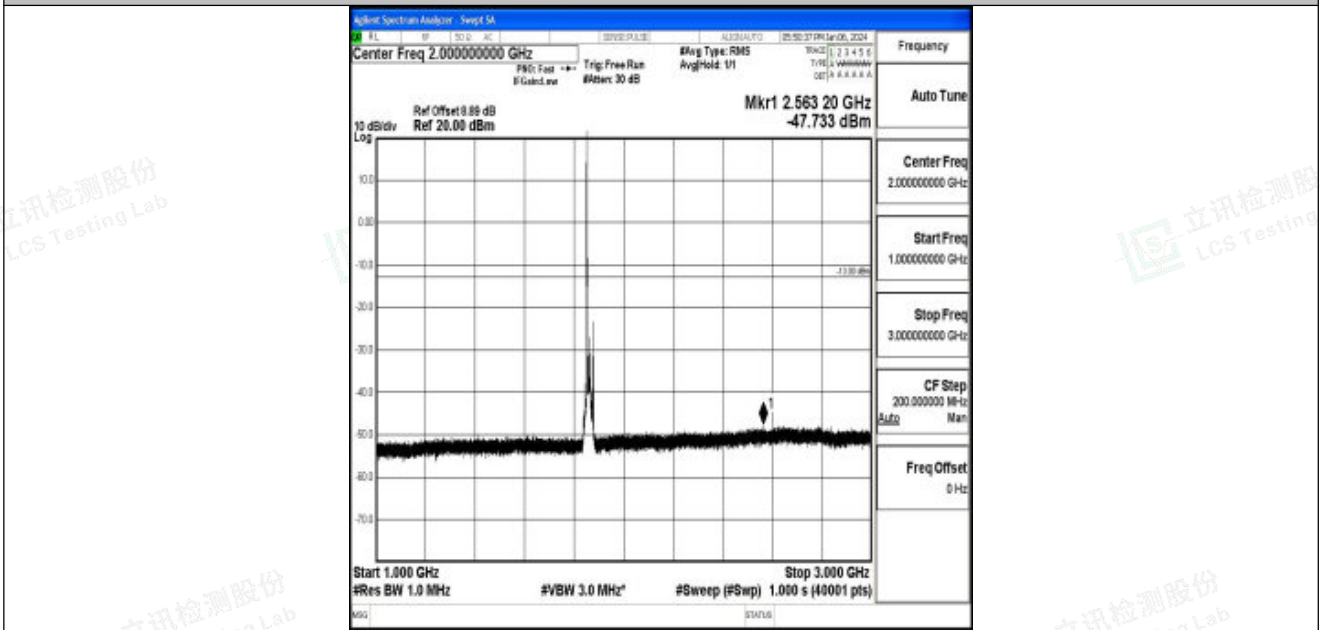
Band25_15MHz_16QAM_26115_1RB#0_1000~3000_1000~3000
