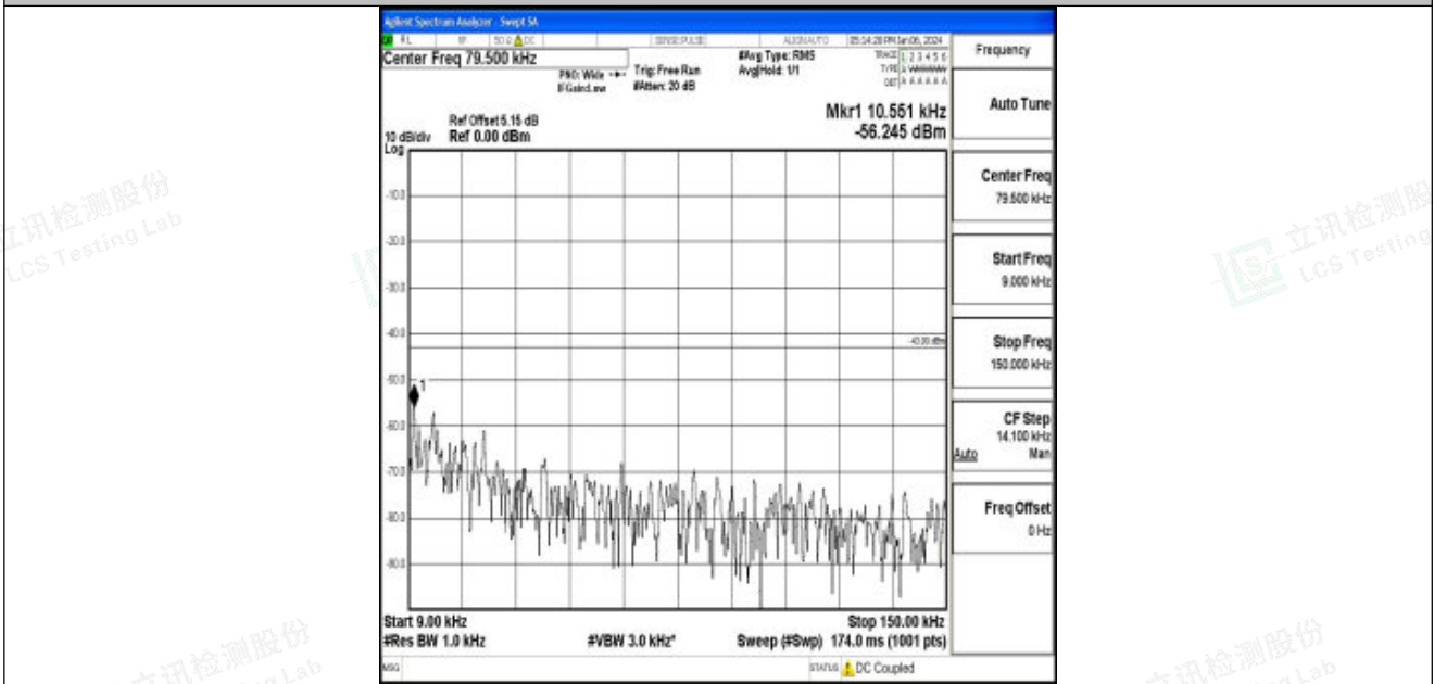
Band25_5MHz_QPSK_26365_1RB#0_0.009~0.15_0.009~0.15
