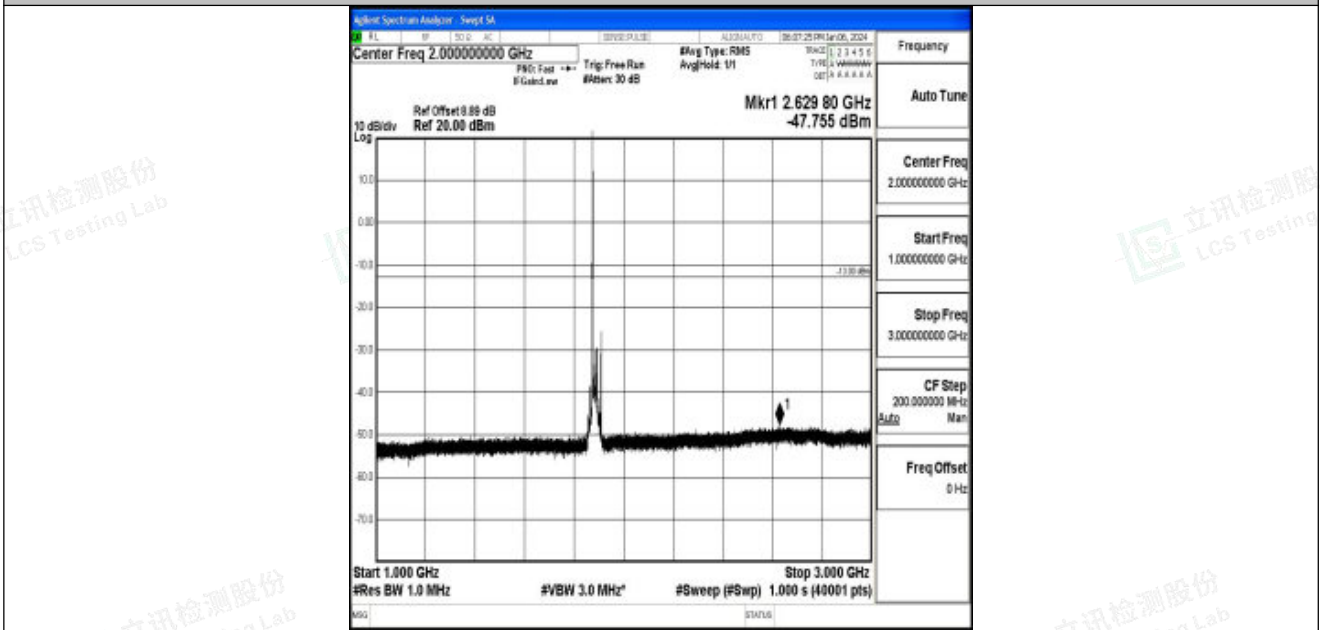
Band25_20MHz_16QAM_26365_1RB#0_1000~3000_1000~3000
