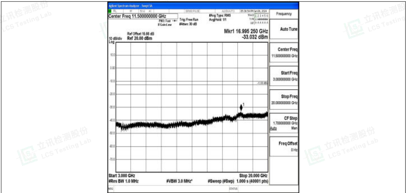
Band25_10MHz_16QAM_26640_1RB#0_3000~20000_3000~20000
