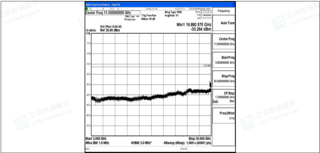
Band25_5MHz_16QAM_26365_1RB#0_3000~20000_3000~20000
