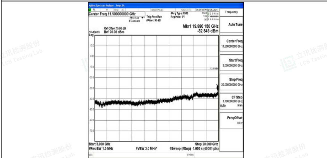
Band25_10MHz_QPSK_26365_1RB#0_3000~20000_3000~20000
