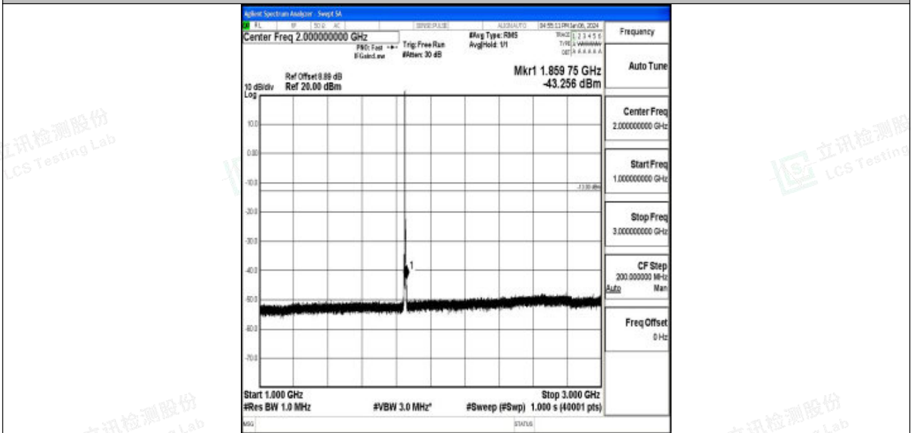
Band25_3MHz_16QAM_26055_1RB#0_1000~3000_1000~3000
