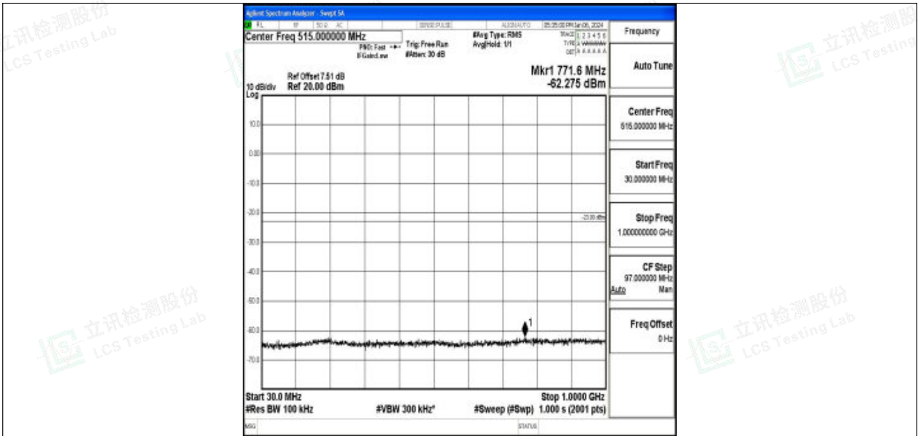
Band25_10MHz_16QAM_26365_1RB#0_30~1000_30~1000
