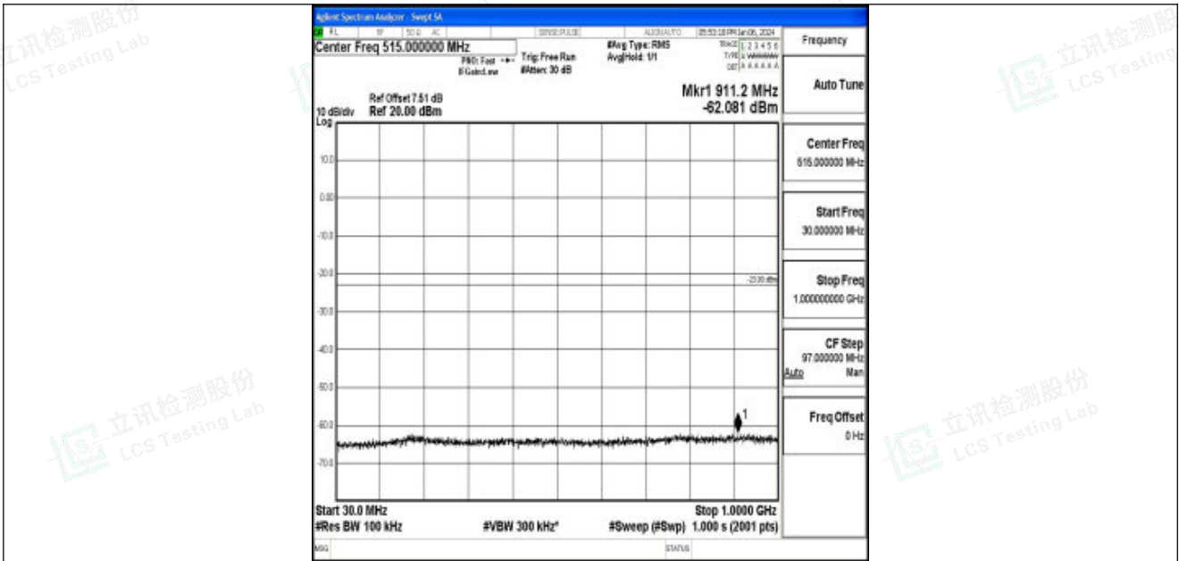
Band25_15MHz_16QAM_26615_1RB#0_30~1000_30~1000
