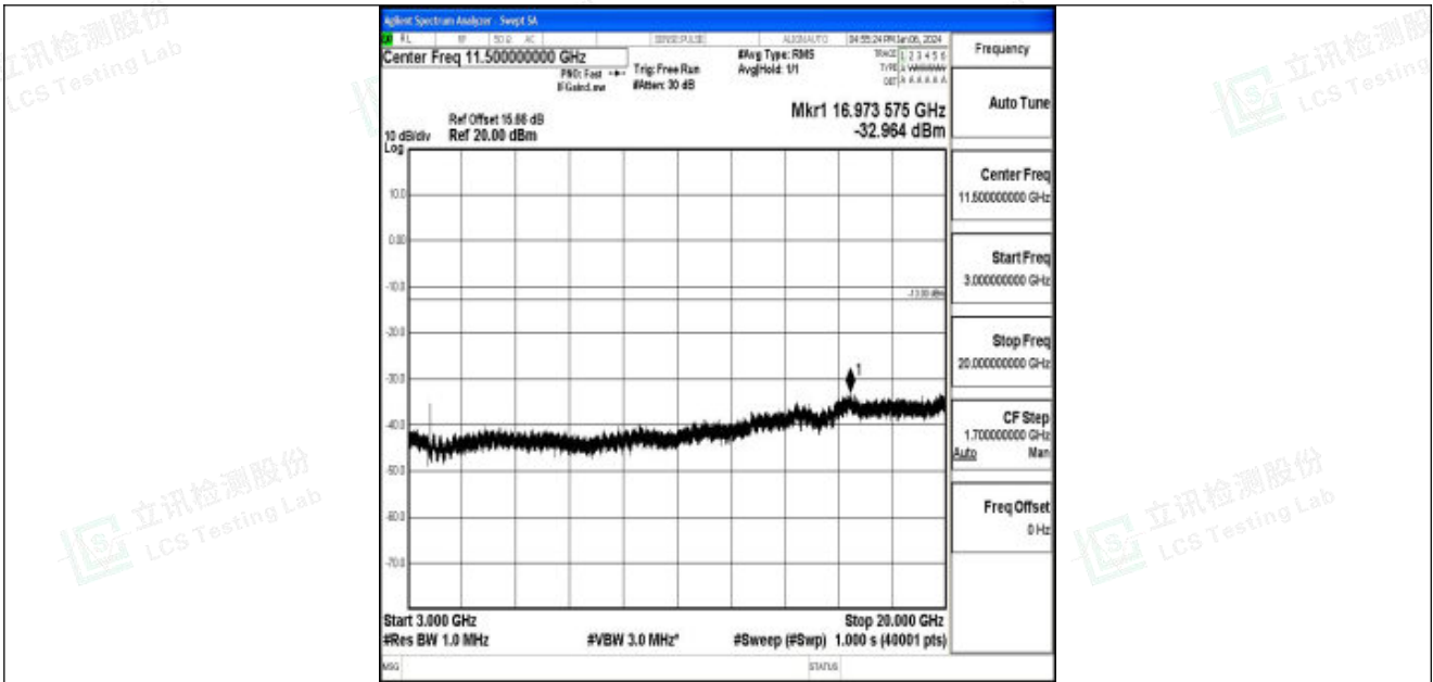
Band25_3MHz_16QAM_26055_1RB#0_3000~20000_3000~20000
