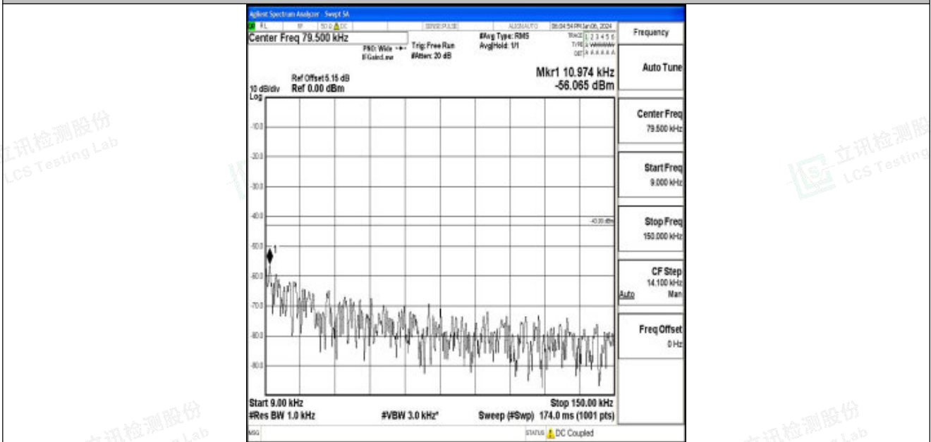
Band25_20MHz_QPSK_26140_1RB#0_0.009~0.15_0.009~0.15
