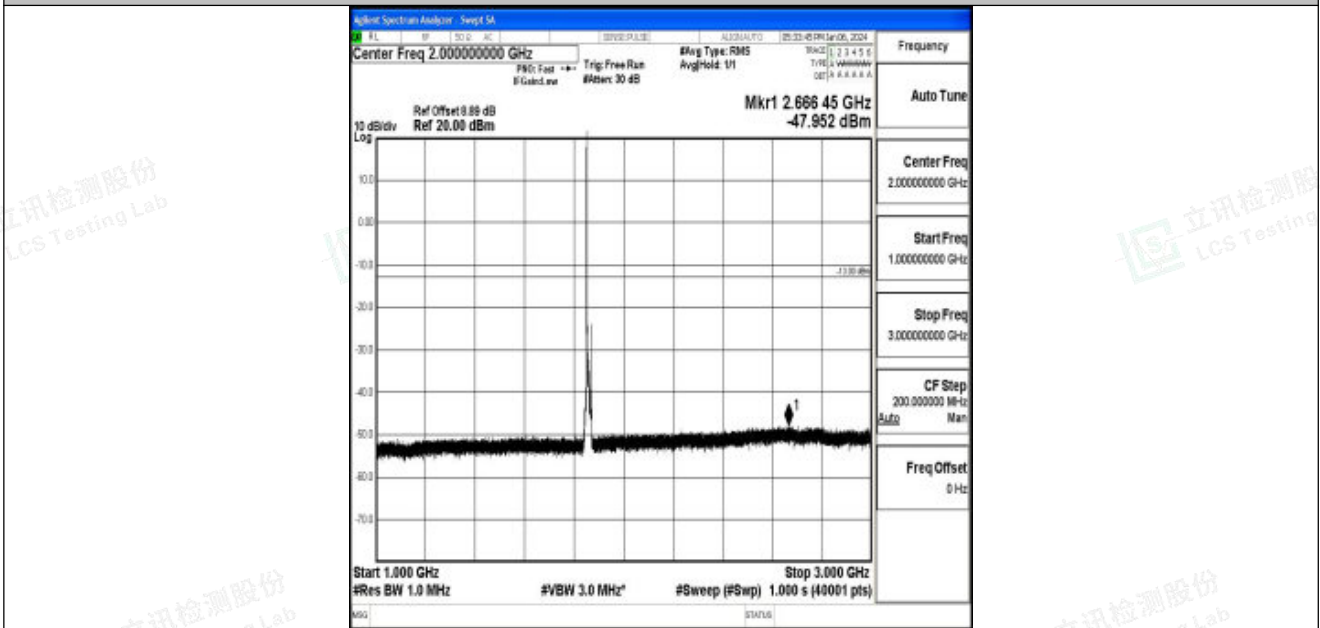
Band25_10MHz_16QAM_26090_1RB#0_1000~3000_1000~3000
