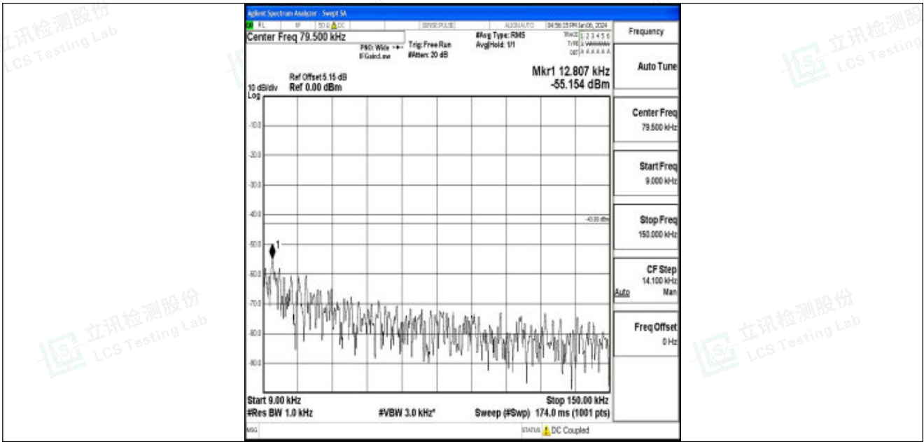
Band25_3MHz_16QAM_26365_1RB#0_0.009~0.15_0.009~0.15
