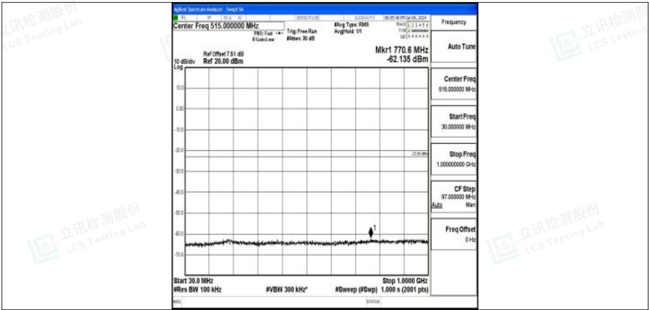
Band25_20MHz_16QAM_26140_1RB#0_30~1000_30~1000
