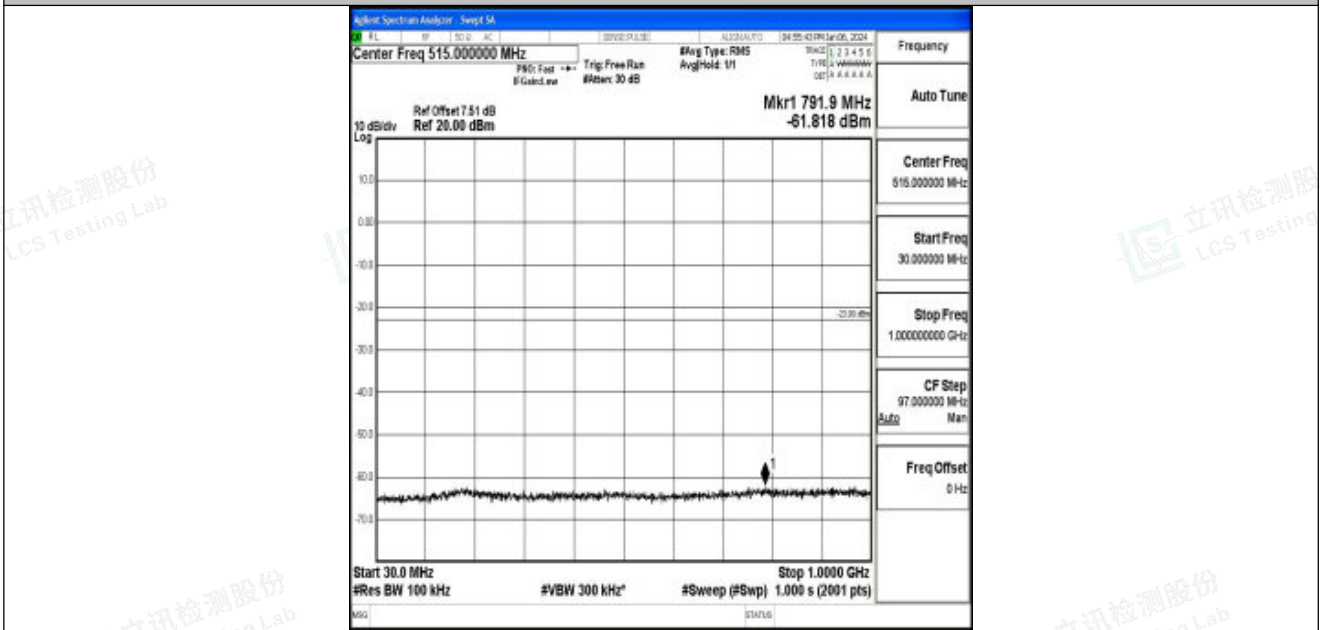
Band25_3MHz_QPSK_26365_1RB#0_30~1000_30~1000
