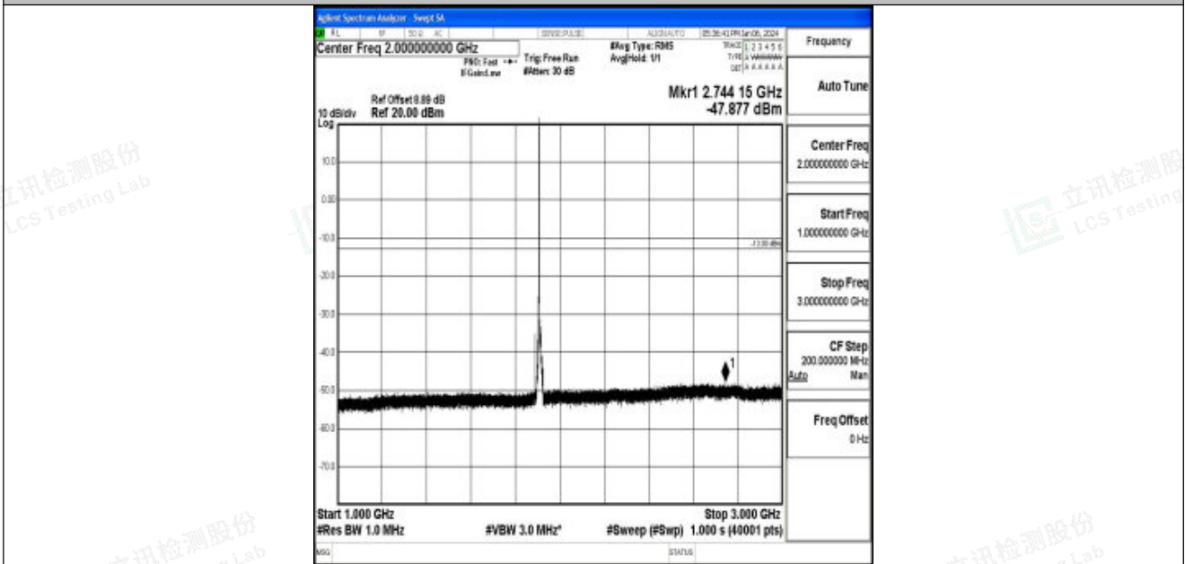
Band25_10MHz_16QAM_26640_1RB#0_1000~3000_1000~3000
