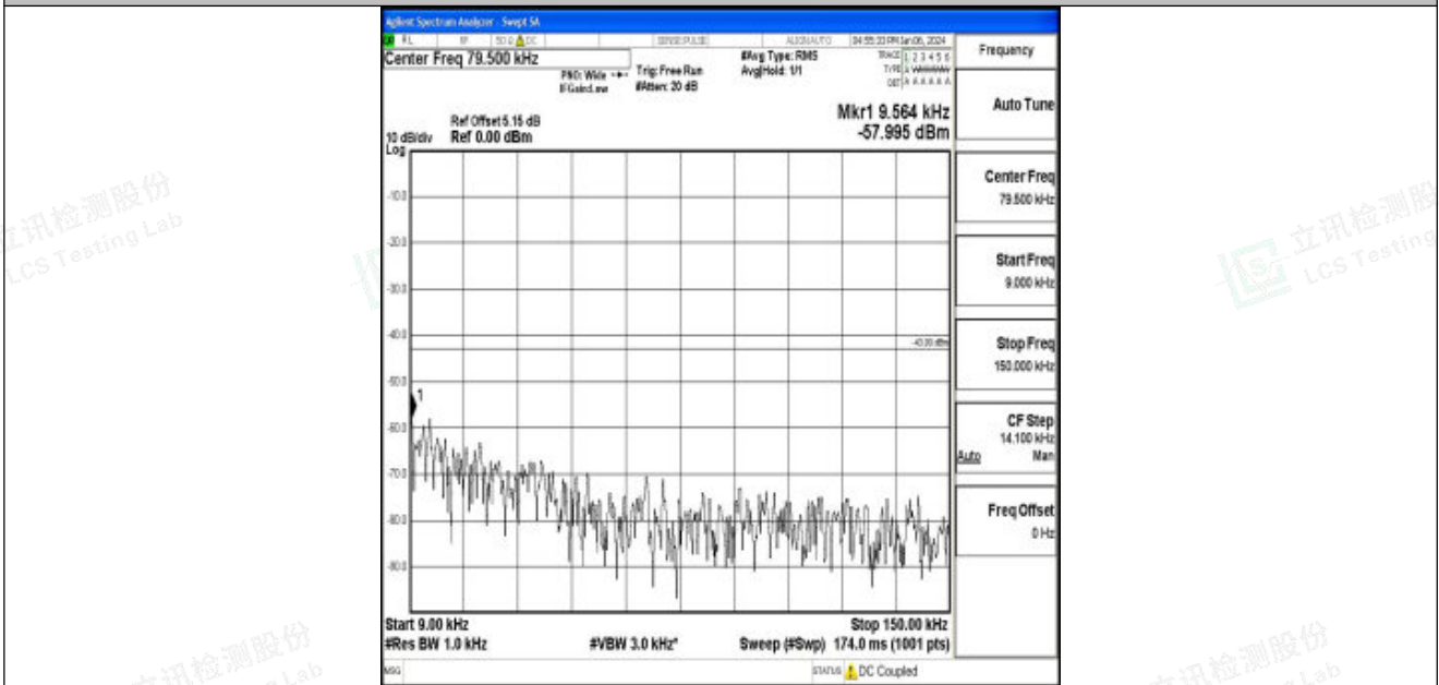
Band25_3MHz_QPSK_26365_1RB#0_0.009~0.15_0.009~0.15
