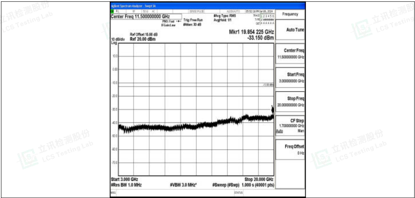
Band25_15MHz_16QAM_26365_1RB#0_3000~20000_3000~20000
