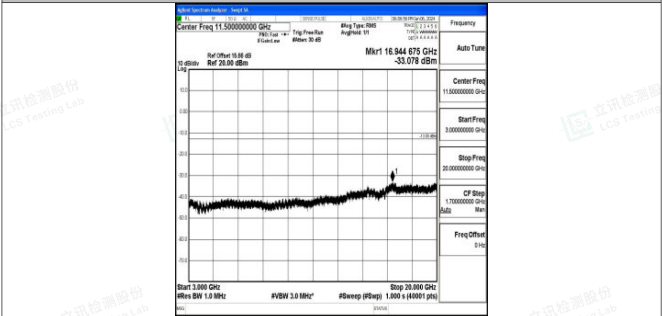
Band25_20MHz_QPSK_26365_1RB#0_3000~20000_3000~20000
