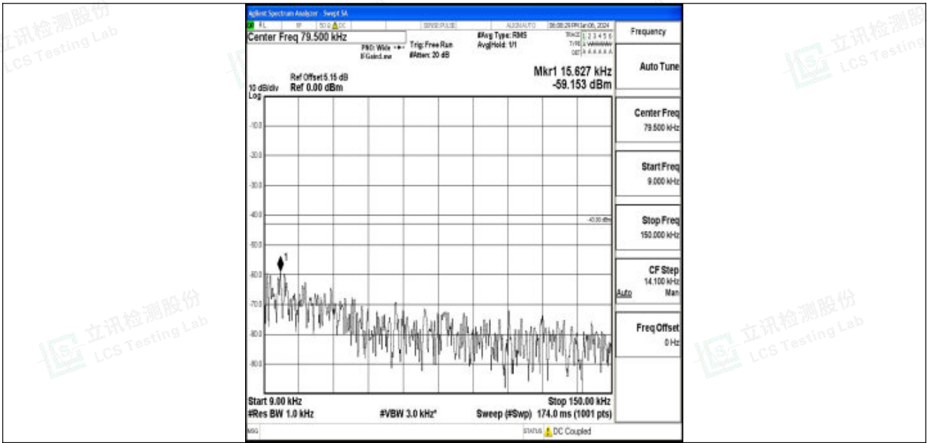
Band25_20MHz_16QAM_26590_1RB#0_0.009~0.15_0.009~0.15
