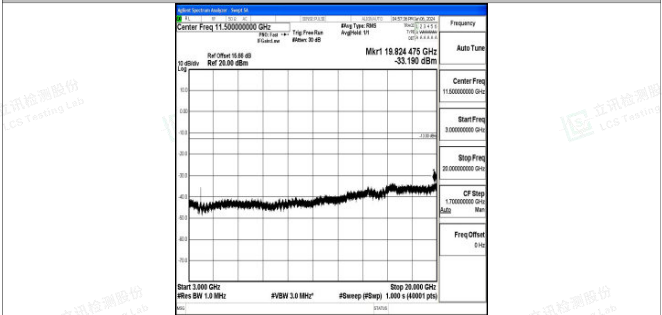
Band25_3MHz_QPSK_26675_1RB#0_3000~20000_3000~20000
