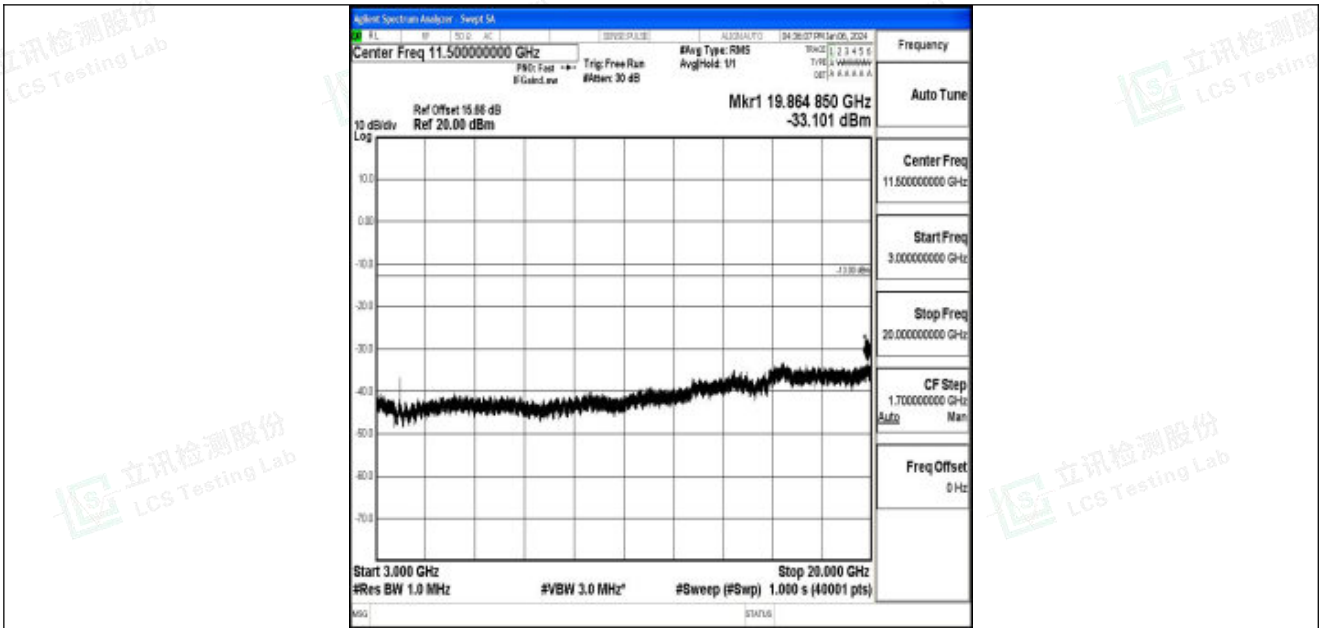
Band25_1.4MHz_16QAM_26683_1RB#0_3000~20000_3000~20000
