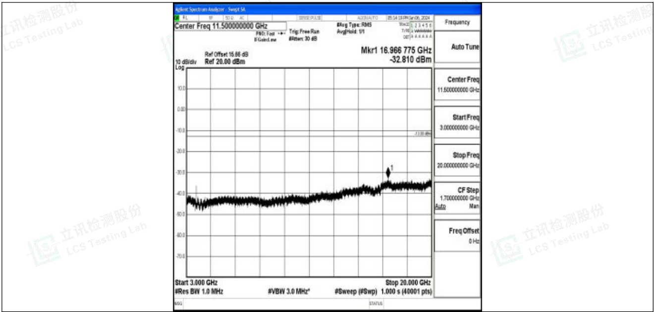
Band25_5MHz_16QAM_26065_1RB#0_3000~20000_3000~20000
