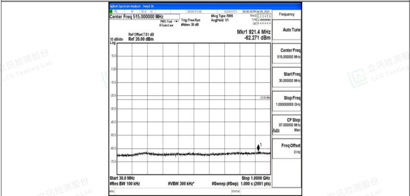
Band25_20MHz_QPSK_26365_1RB#0_30~1000_30~1000
