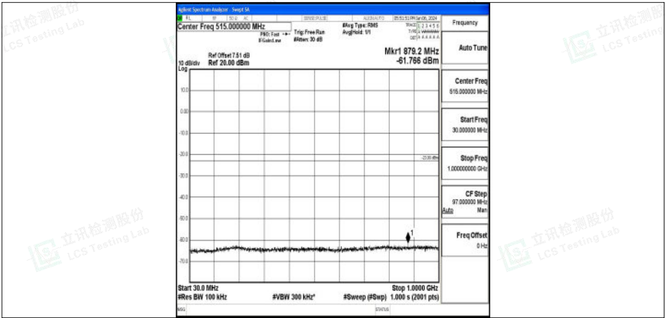
Band25_15MHz_16QAM_26365_1RB#0_30~1000_30~1000
