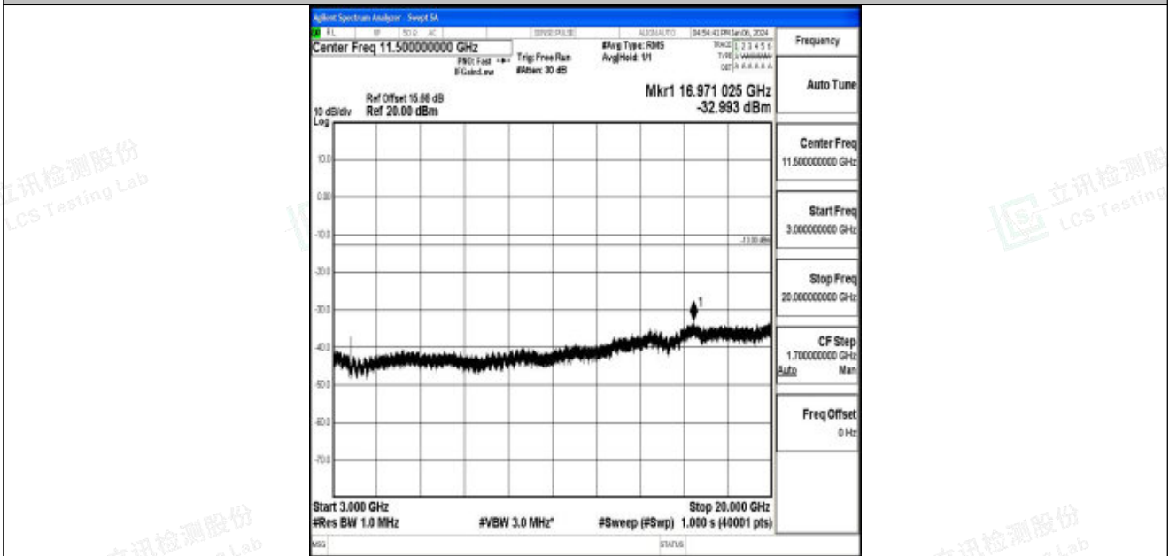
Band25_3MHz_QPSK_26055_1RB#0_3000~20000_3000~20000
