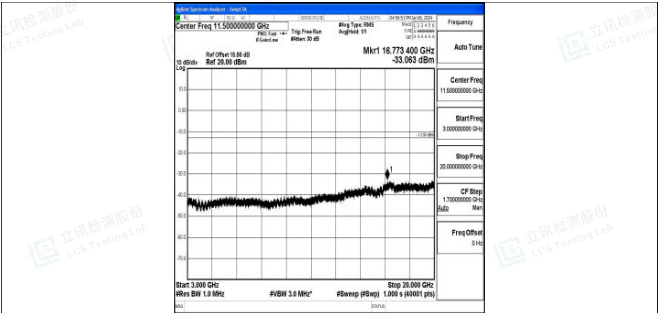
Band25_3MHz_16QAM_26365_1RB#0_3000~20000_3000~20000
