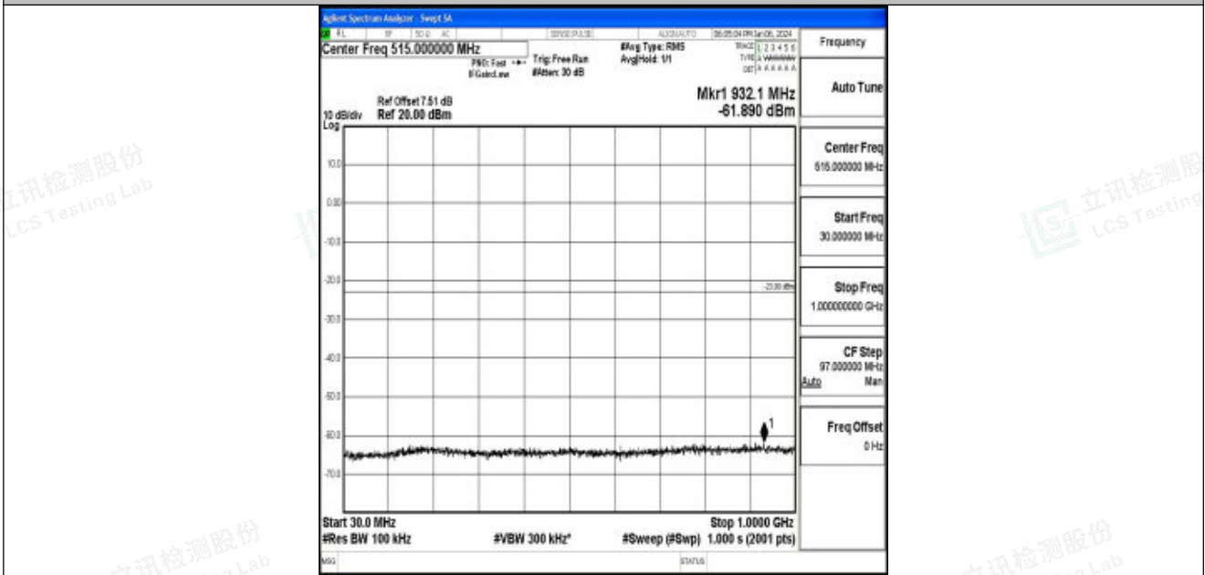
Band25_20MHz_QPSK_26140_1RB#0_30~1000_30~1000
