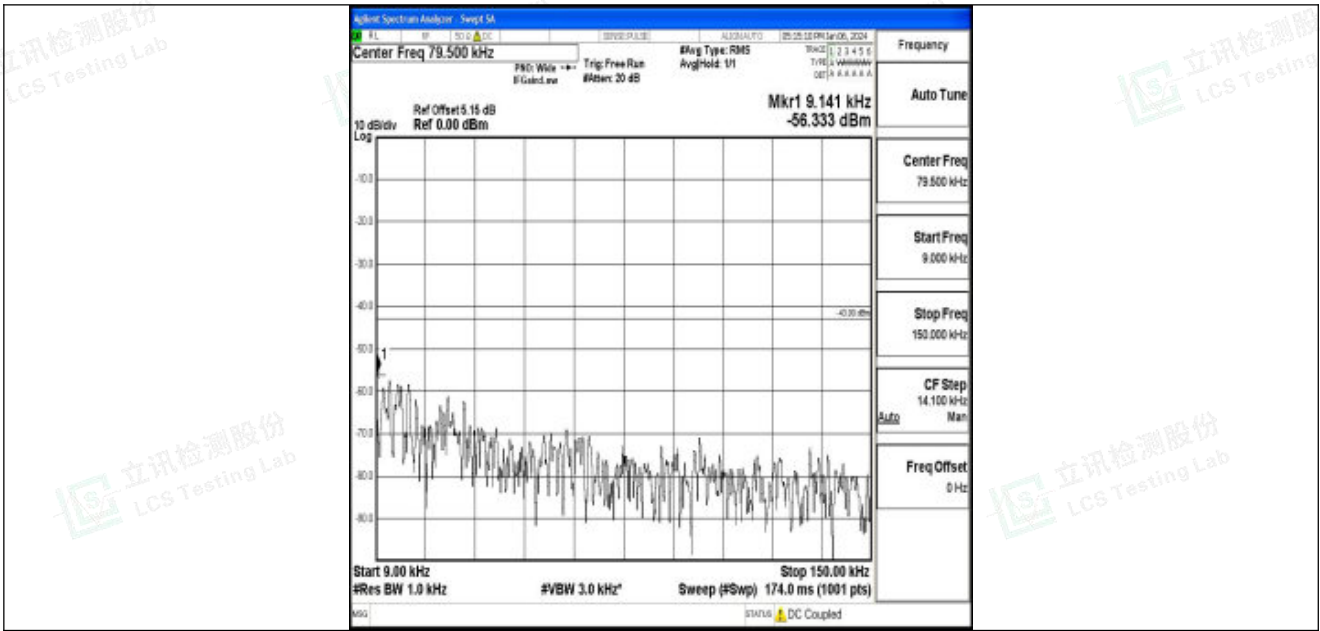
Band25_5MHz_16QAM_26365_1RB#0_0.009~0.15_0.009~0.15
