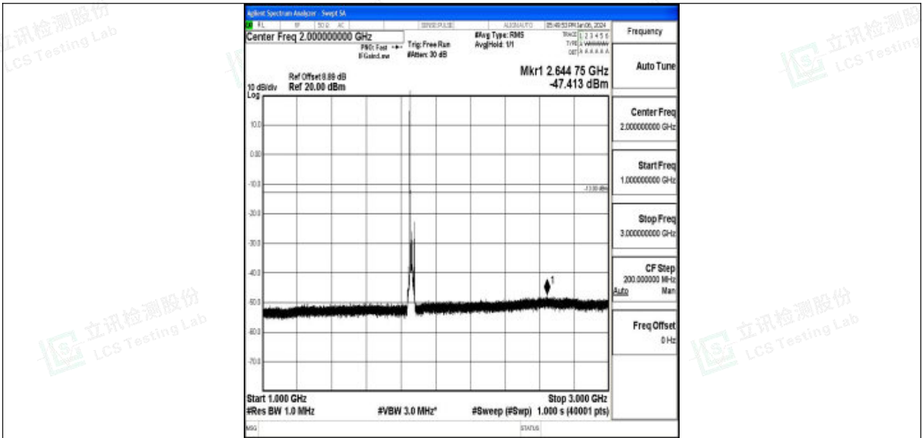
Band25_15MHz_QPSK_26115_1RB#0_1000~3000_1000~3000
