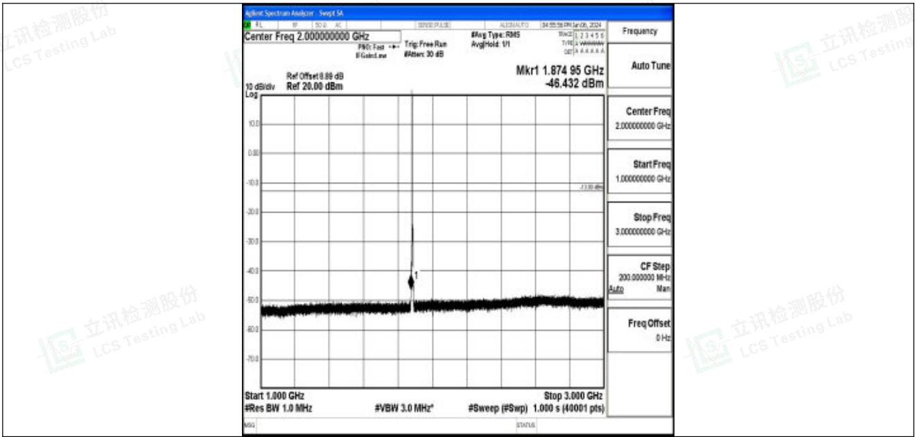
Band25_3MHz_QPSK_26365_1RB#0_1000~3000_1000~3000
