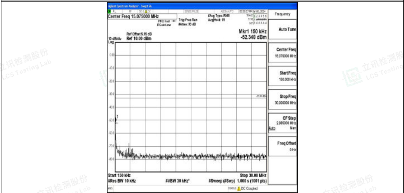
Band25_15MHz_16QAM_26115_1RB#0_0.15~30_0.15~30
