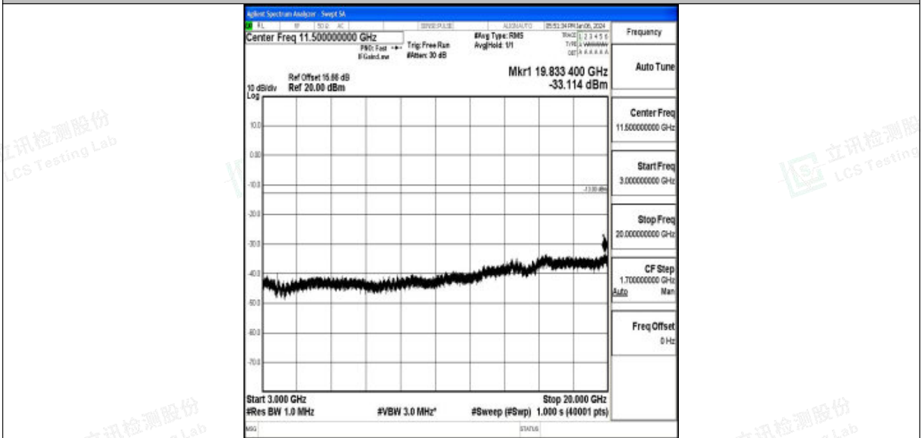
Band25_15MHz_QPSK_26365_1RB#0_3000~20000_3000~20000
