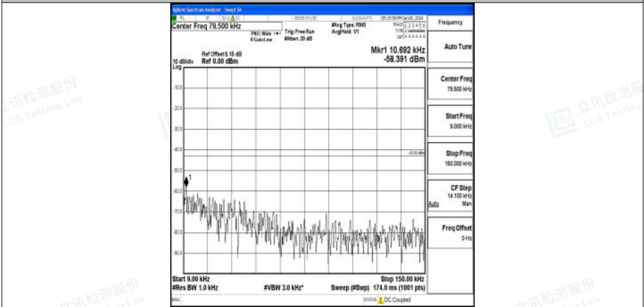
Band25_5MHz_QPSK_26665_1RB#0_0.009~0.15_0.009~0.15
