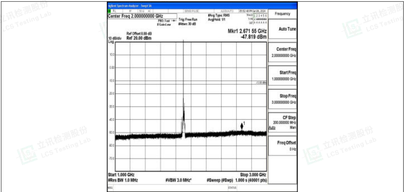
Band25_15MHz_QPSK_26615_1RB#0_1000~3000_1000~3000
