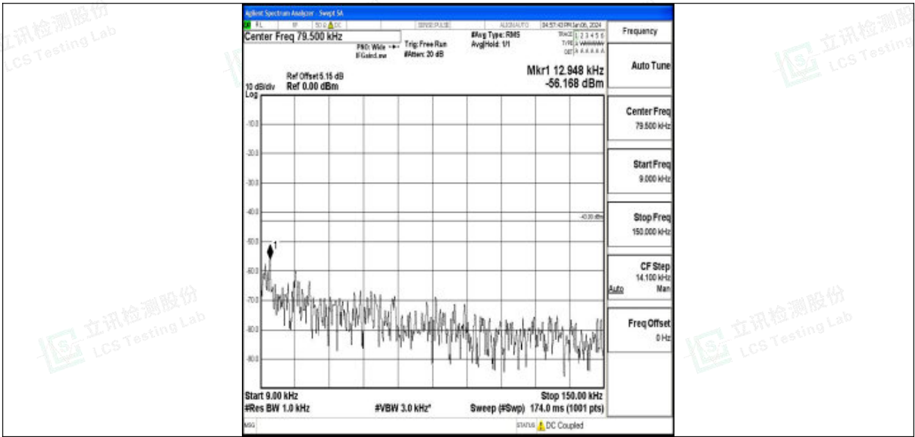
Band25_3MHz_16QAM_26675_1RB#0_0.009~0.15_0.009~0.15
