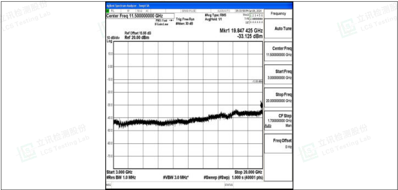
Band25_10MHz_16QAM_26090_1RB#0_3000~20000_3000~20000
