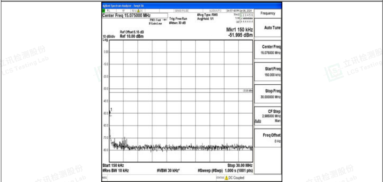
Band25_3MHz_16QAM_26675_1RB#0_0.15~30_0.15~30
