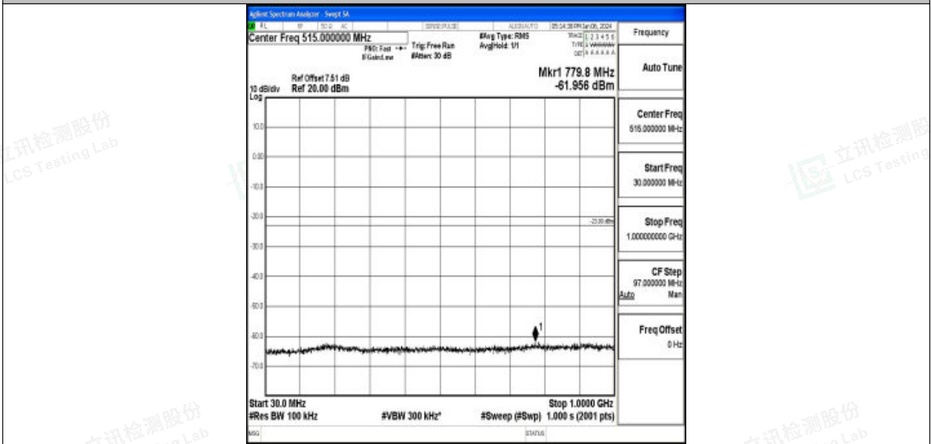
Band25_5MHz_QPSK_26365_1RB#0_30~1000_30~1000
