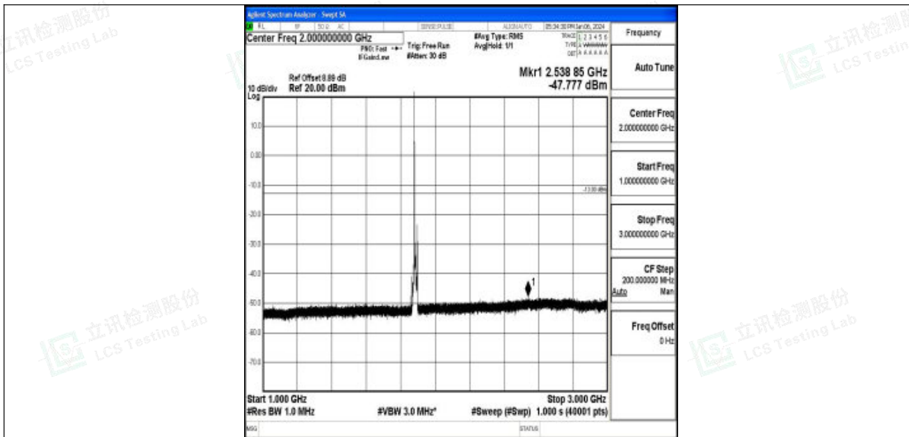
Band25_10MHz_QPSK_26365_1RB#0_1000~3000_1000~3000
