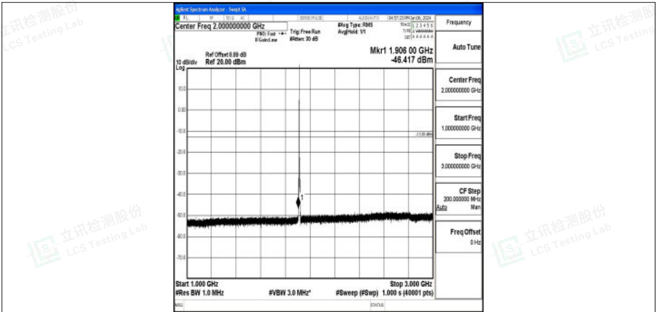
Band25_3MHz_QPSK_26675_1RB#0_1000~3000_1000~3000
