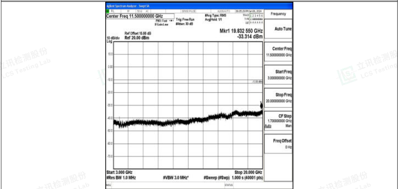
Band25_20MHz_QPSK_26140_1RB#0_3000~20000_3000~20000
