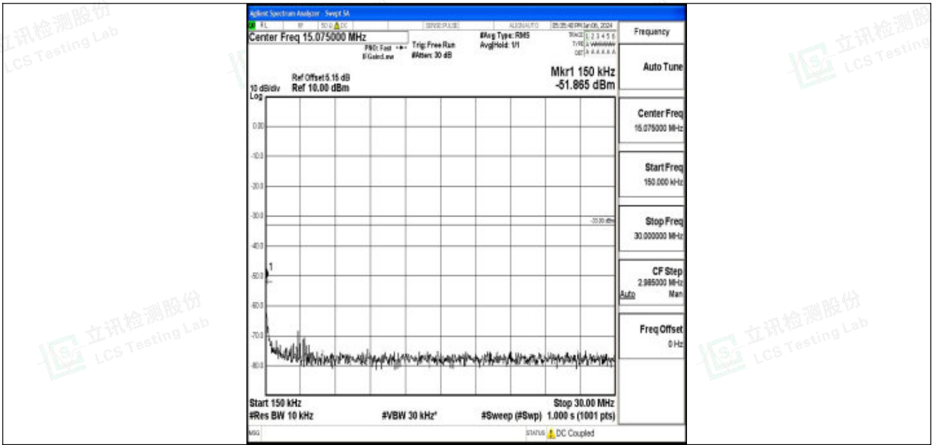
Band25_10MHz_QPSK_26640_1RB#0_0.15~30_0.15~30
