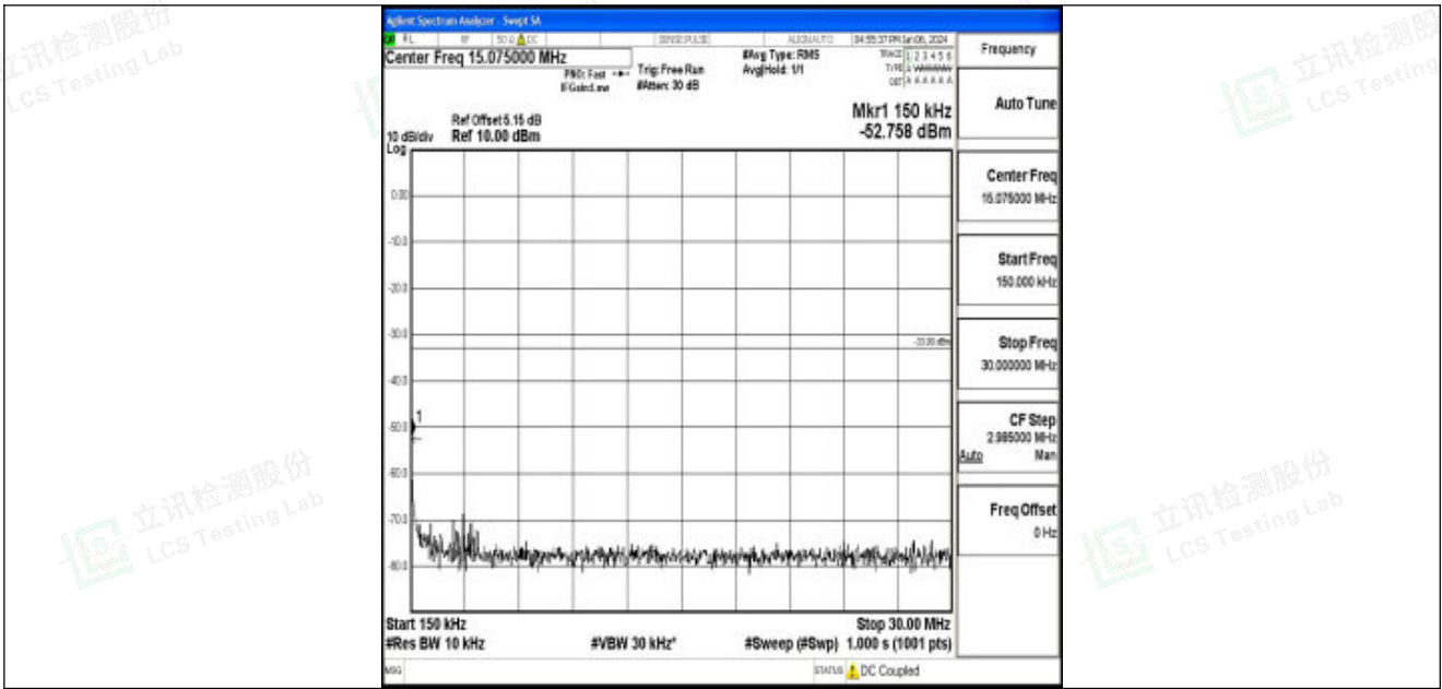
Band25_3MHz_QPSK_26365_1RB#0_0.15~30_0.15~30
