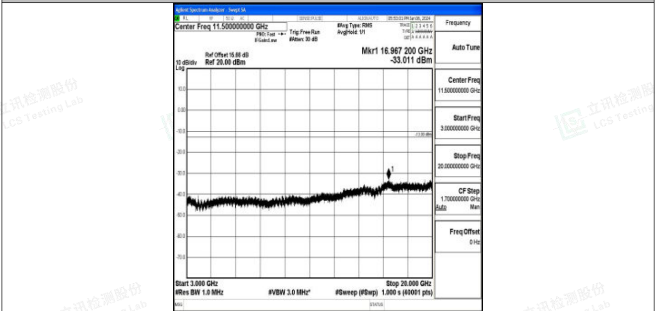
Band25_15MHz_QPSK_26615_1RB#0_3000~20000_3000~20000
