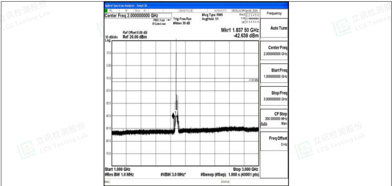
Band25_15MHz_QPSK_26365_1RB#0_1000~3000_1000~3000
