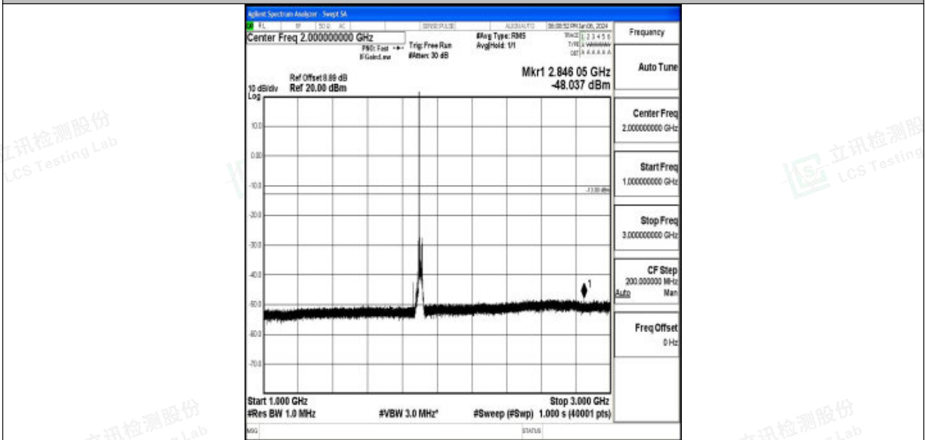
Band25_20MHz_16QAM_26590_1RB#0_1000~3000_1000~3000
