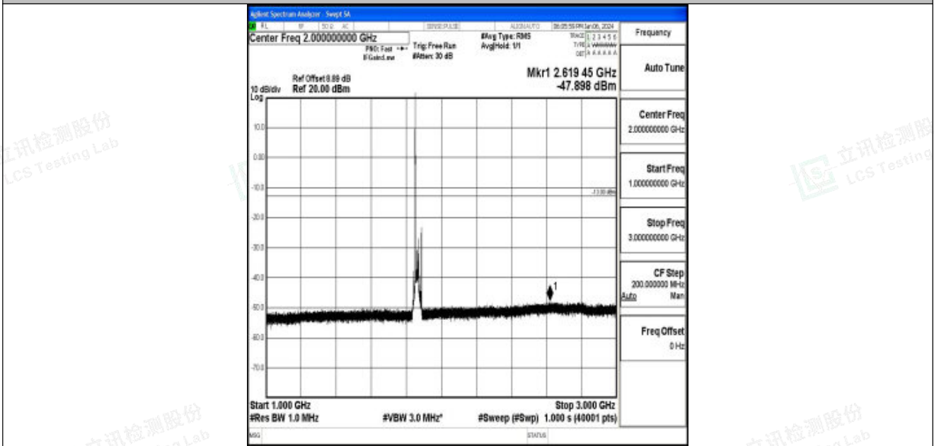
Band25_20MHz_16QAM_26140_1RB#0_1000~3000_1000~3000
