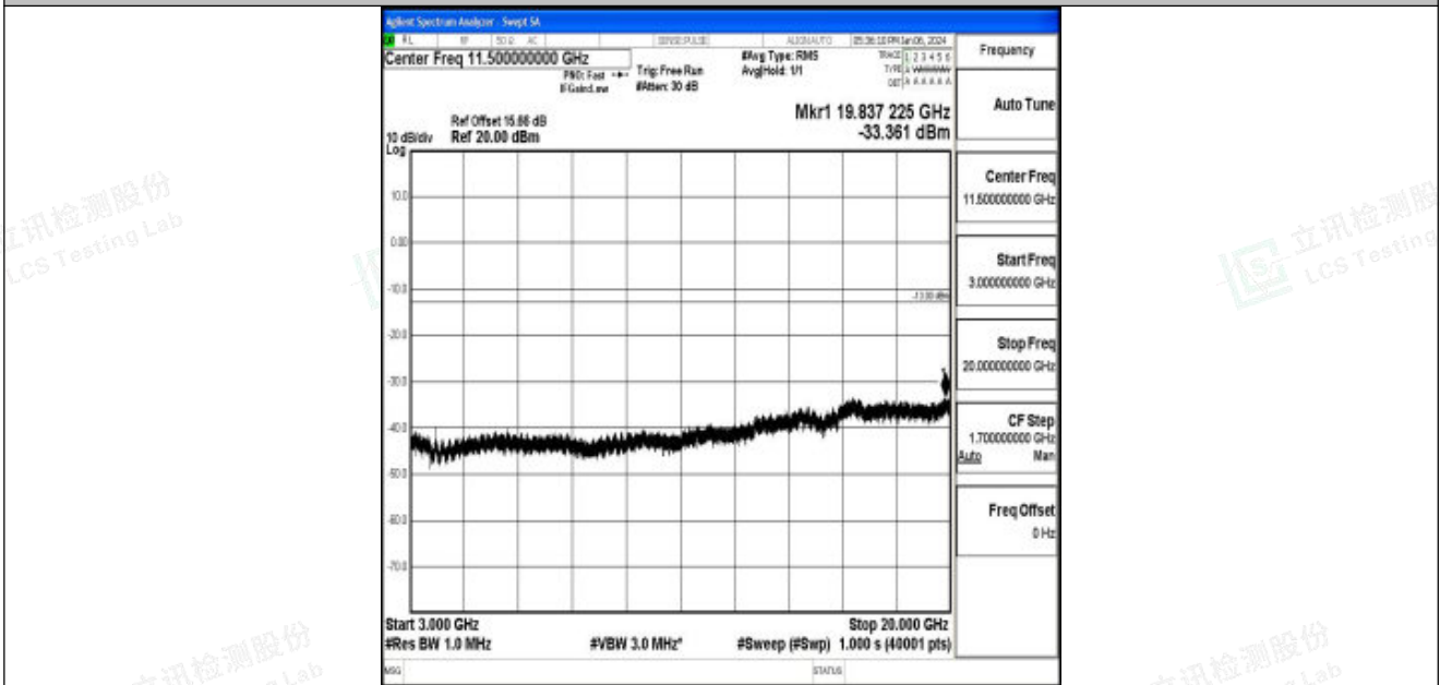
Band25_10MHz_QPSK_26640_1RB#0_3000~20000_3000~20000
