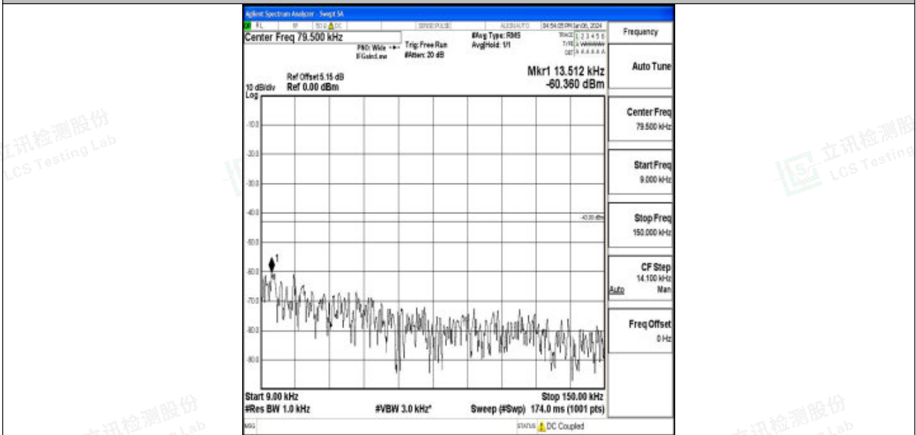
Band25_3MHz_QPSK_26055_1RB#0_0.009~0.15_0.009~0.15
