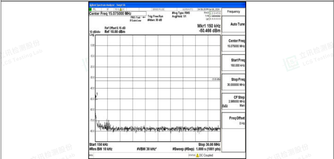
Band25_3MHz_16QAM_26365_1RB#0_0.15~30_0.15~30
