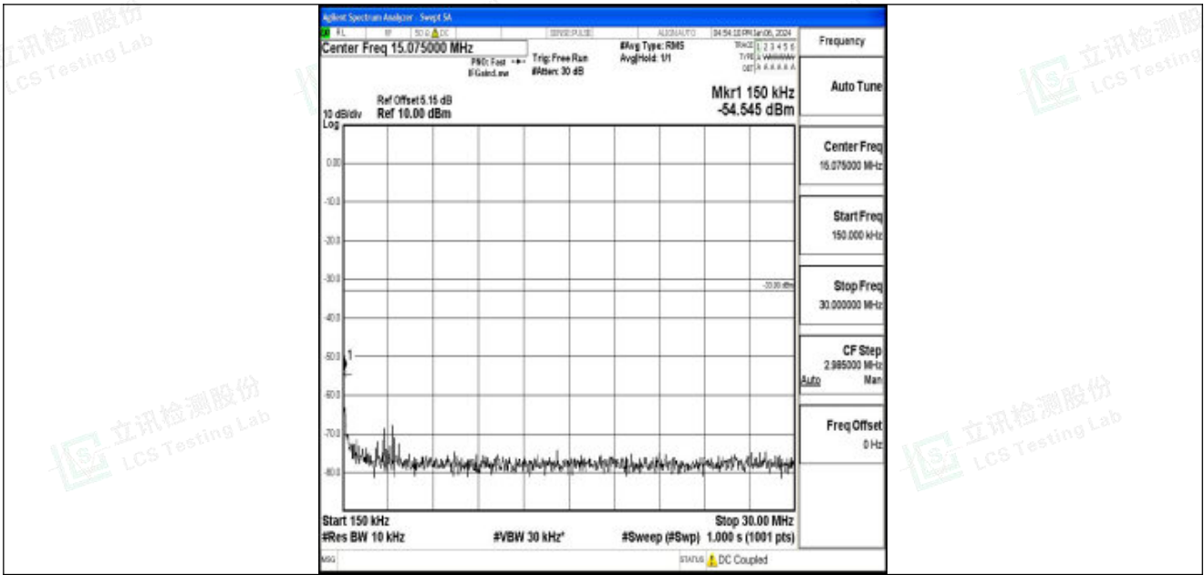
Band25_3MHz_QPSK_26055_1RB#0_0.15~30_0.15~30
