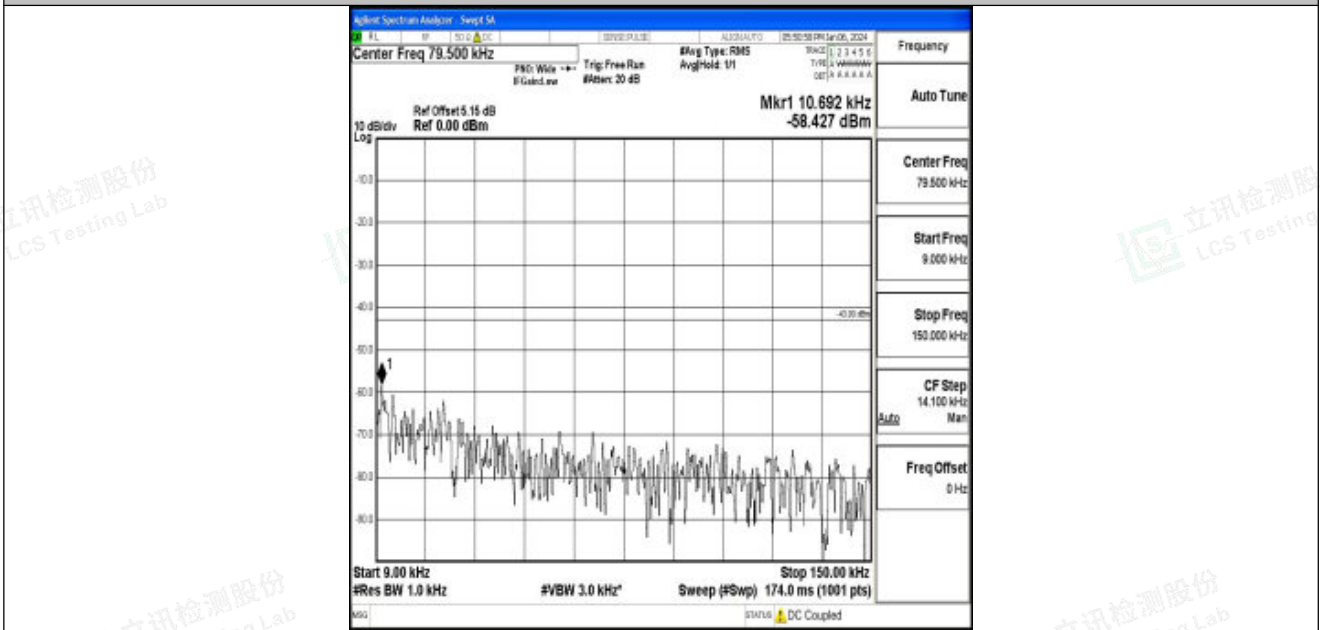
Band25_15MHz_QPSK_26365_1RB#0_0.009~0.15_0.009~0.15
