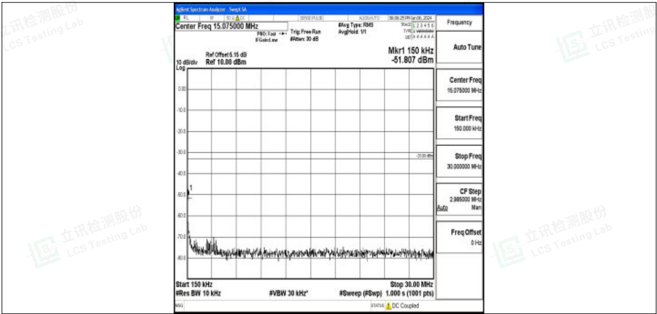
Band25_20MHz_QPSK_26365_1RB#0_0.15~30_0.15~30
