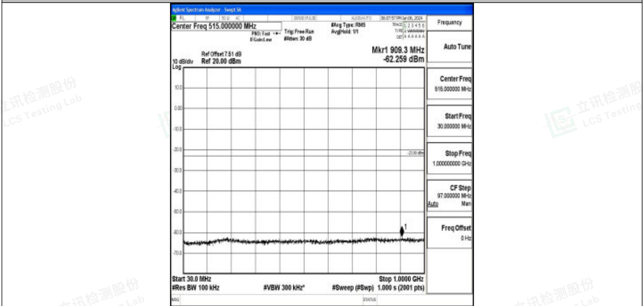
Band25_20MHz_QPSK_26590_1RB#0_30~1000_30~1000
