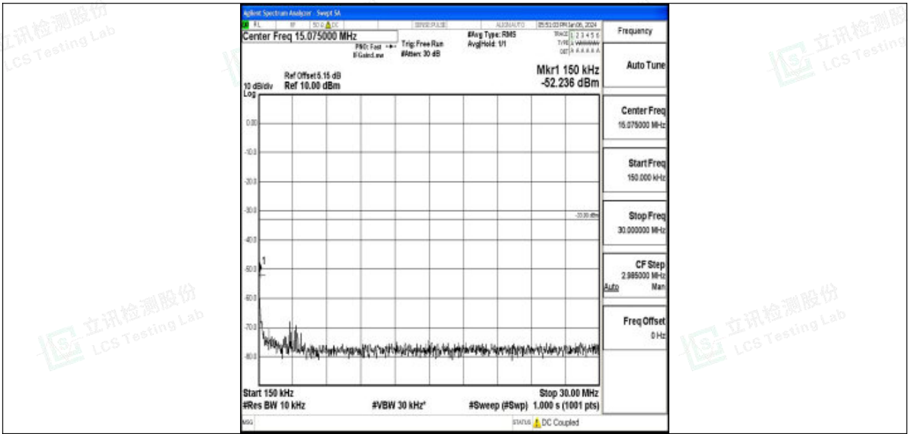
Band25_15MHz_QPSK_26365_1RB#0_0.15~30_0.15~30
