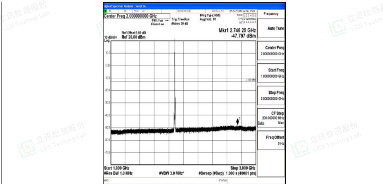
Band25_5MHz_QPSK_26365_1RB#0_1000~3000_1000~3000
