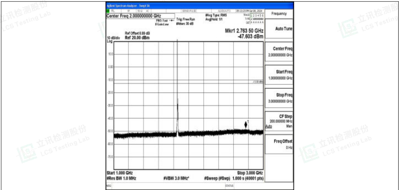
Band25_5MHz_QPSK_26065_1RB#0_1000~3000_1000~3000
