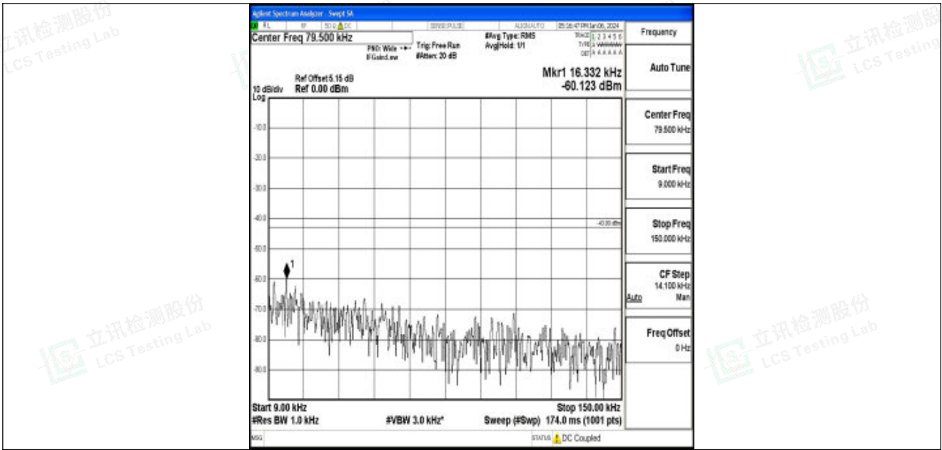
Band25_5MHz_16QAM_26665_1RB#0_0.009~0.15_0.009~0.15
