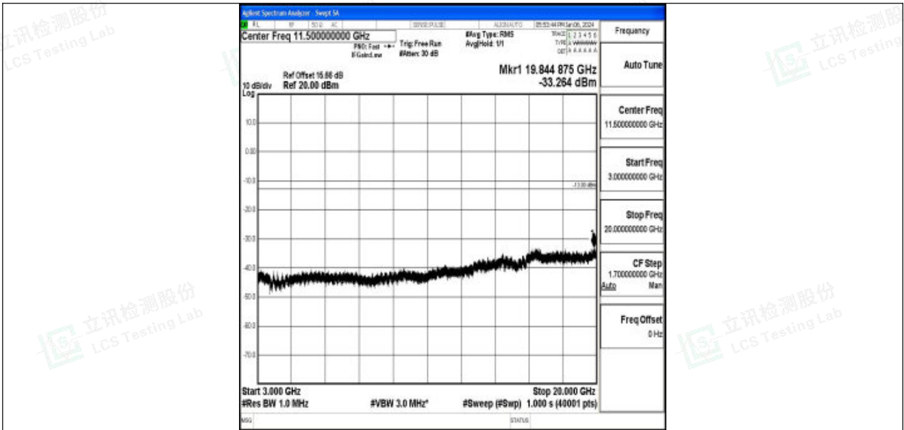
Band25_15MHz_16QAM_26615_1RB#0_3000~20000_3000~20000
