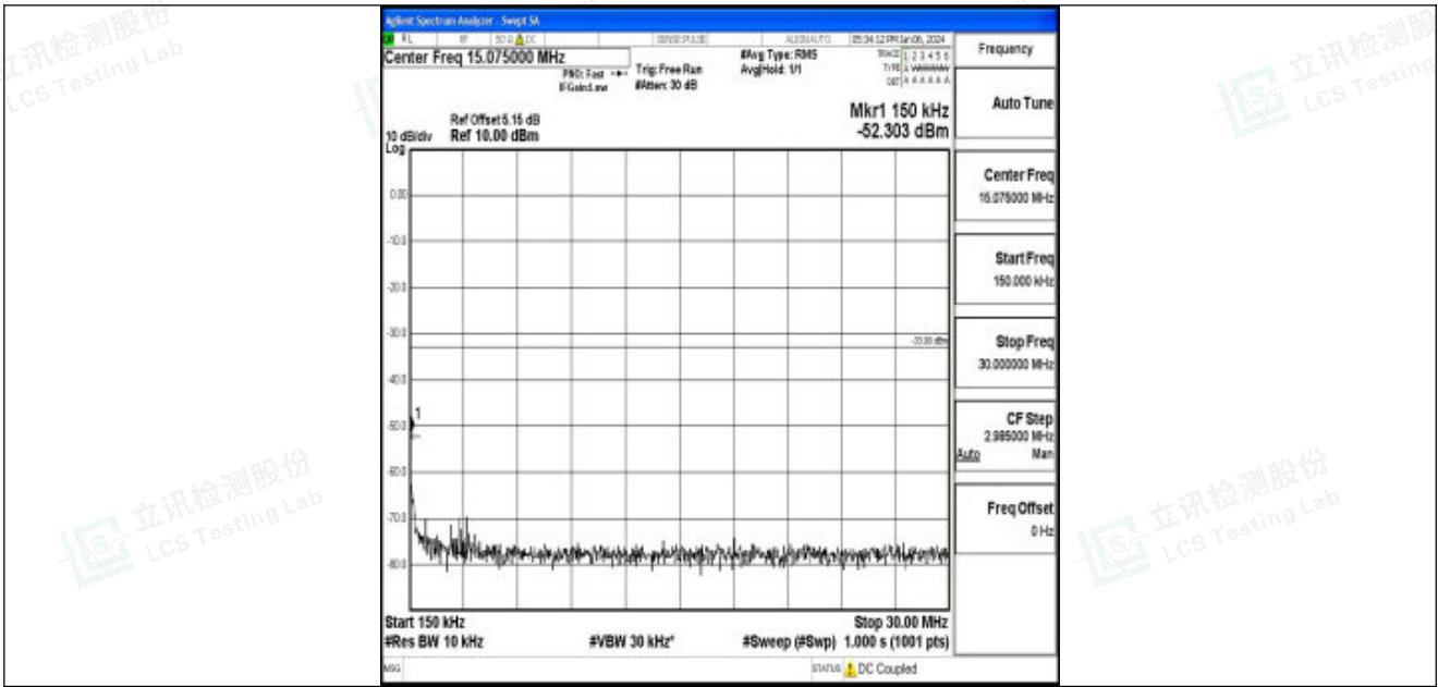
Band25_10MHz_QPSK_26365_1RB#0_0.15~30_0.15~30
