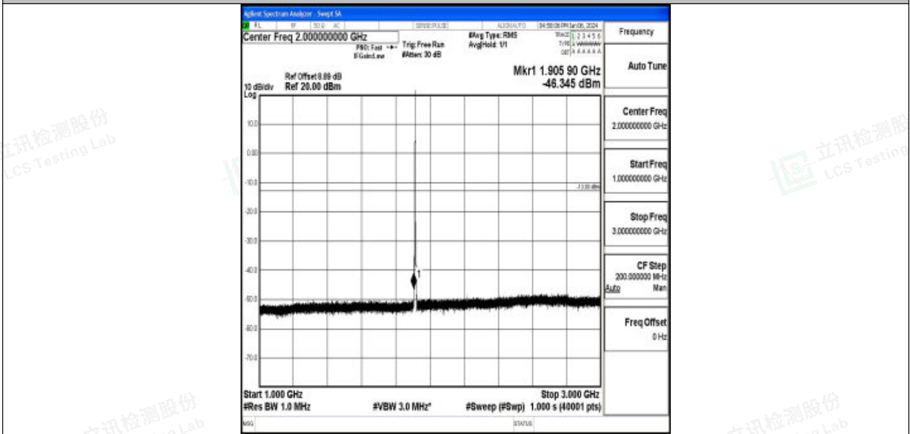
Band25_3MHz_16QAM_26675_1RB#0_1000~3000_1000~3000
