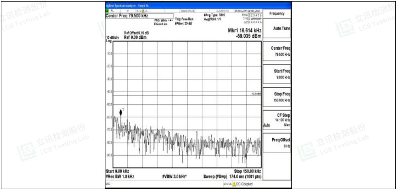
Band25_15MHz_16QAM_26115_1RB#0_0.009~0.15_0.009~0.15
