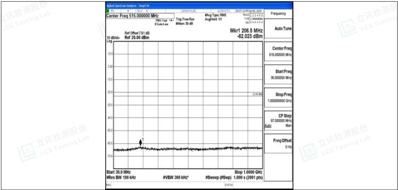
Band25_20MHz_16QAM_26365_1RB#0_30~1000_30~1000
