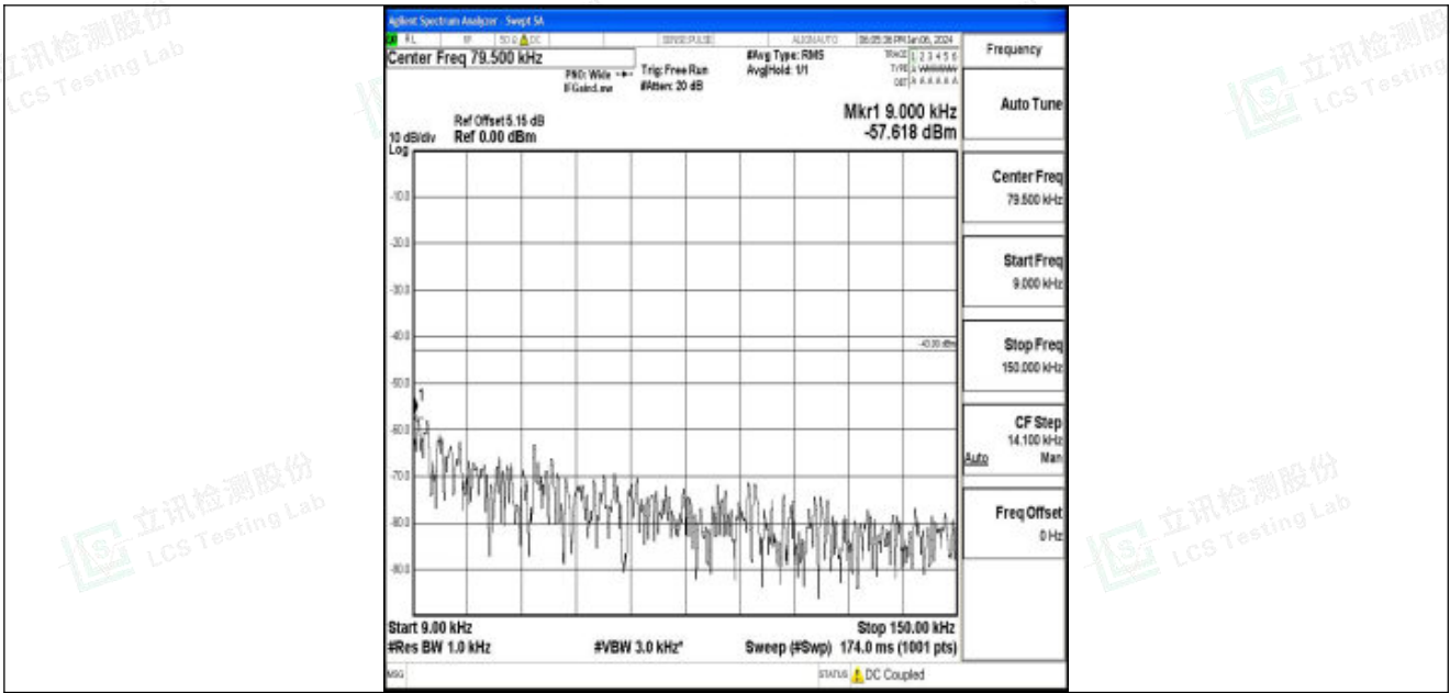
Band25_20MHz_16QAM_26140_1RB#0_0.009~0.15_0.009~0.15
