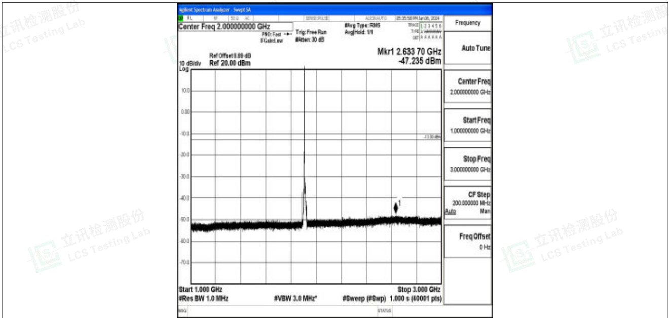
Band25_10MHz_QPSK_26640_1RB#0_1000~3000_1000~3000
