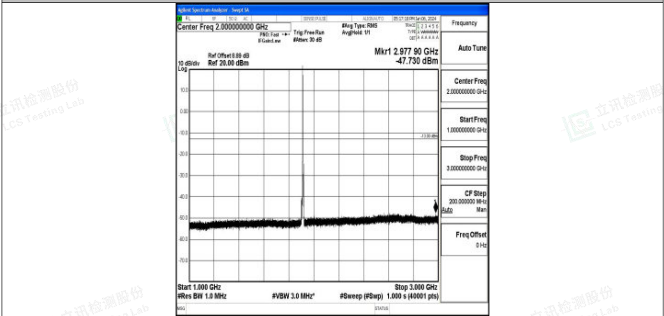
Band25_5MHz_16QAM_26665_1RB#0_1000~3000_1000~3000
