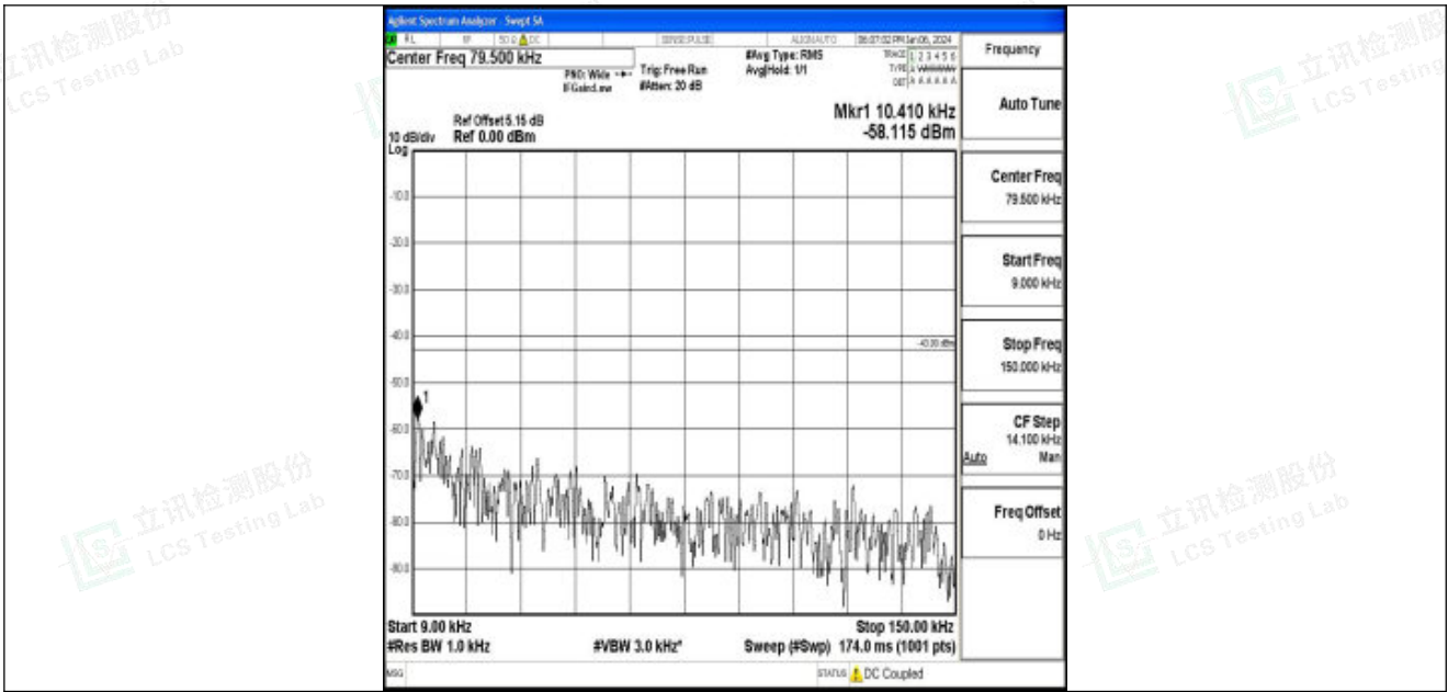
Band25_20MHz_16QAM_26365_1RB#0_0.009~0.15_0.009~0.15
