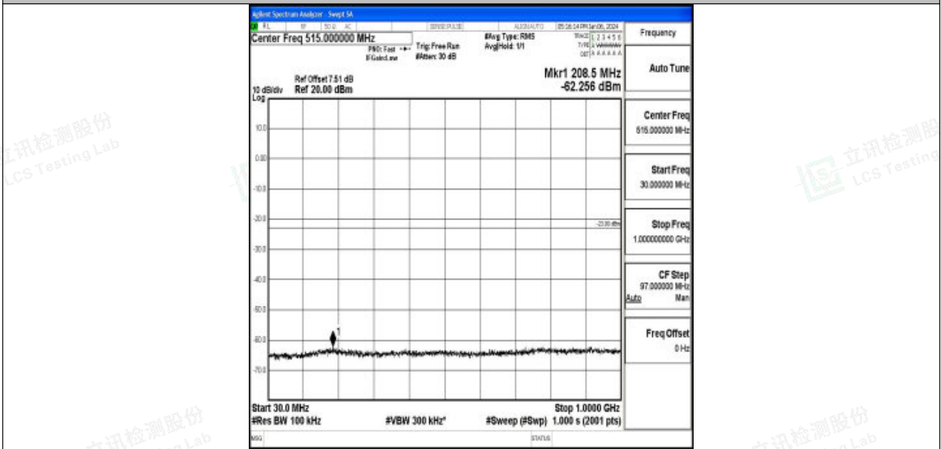
Band25_5MHz_QPSK_26665_1RB#0_30~1000_30~1000
