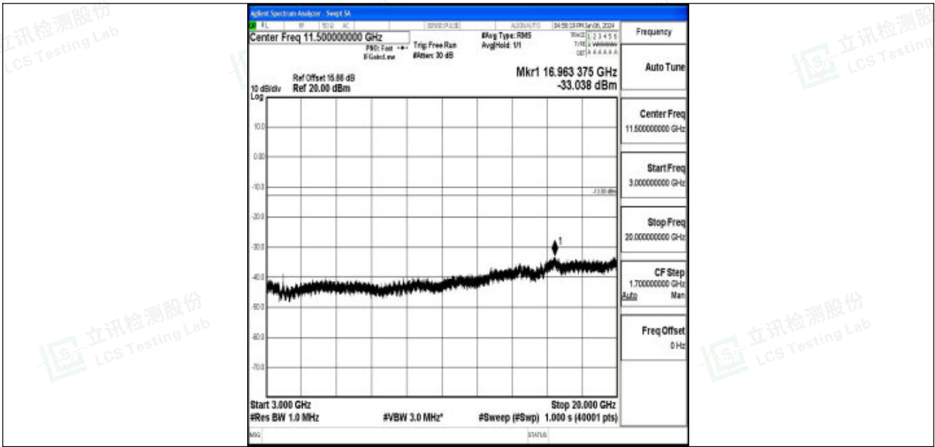
Band25_3MHz_16QAM_26675_1RB#0_3000~20000_3000~20000
