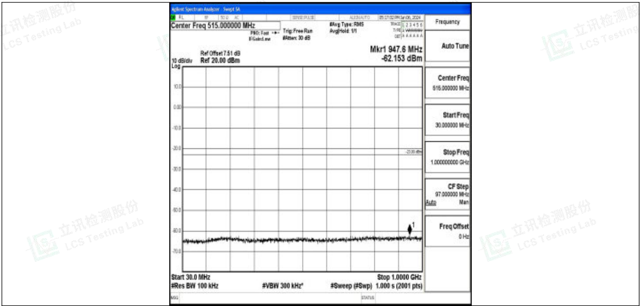
Band25_5MHz_16QAM_26665_1RB#0_30~1000_30~1000
