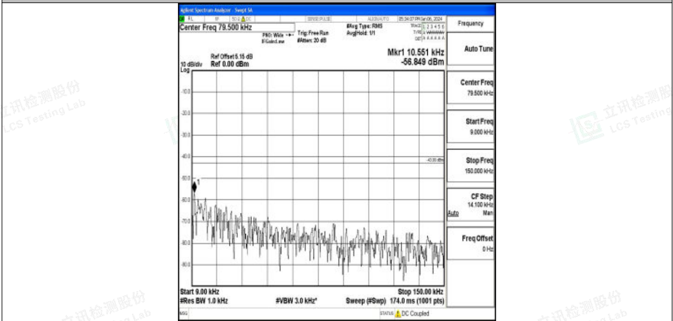
Band25_10MHz_QPSK_26365_1RB#0_0.009~0.15_0.009~0.15
