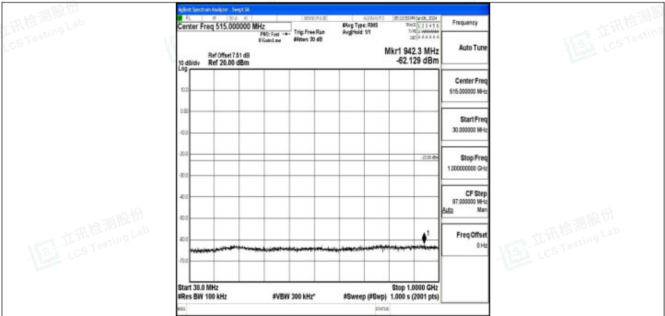
Band25_5MHz_16QAM_26065_1RB#0_30~1000_30~1000
