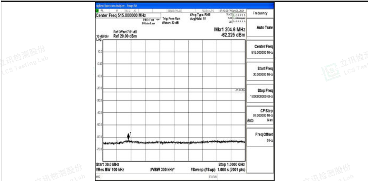
Band4_15MHz_QPSK_20175_1RB#0_30~1000_30~1000
