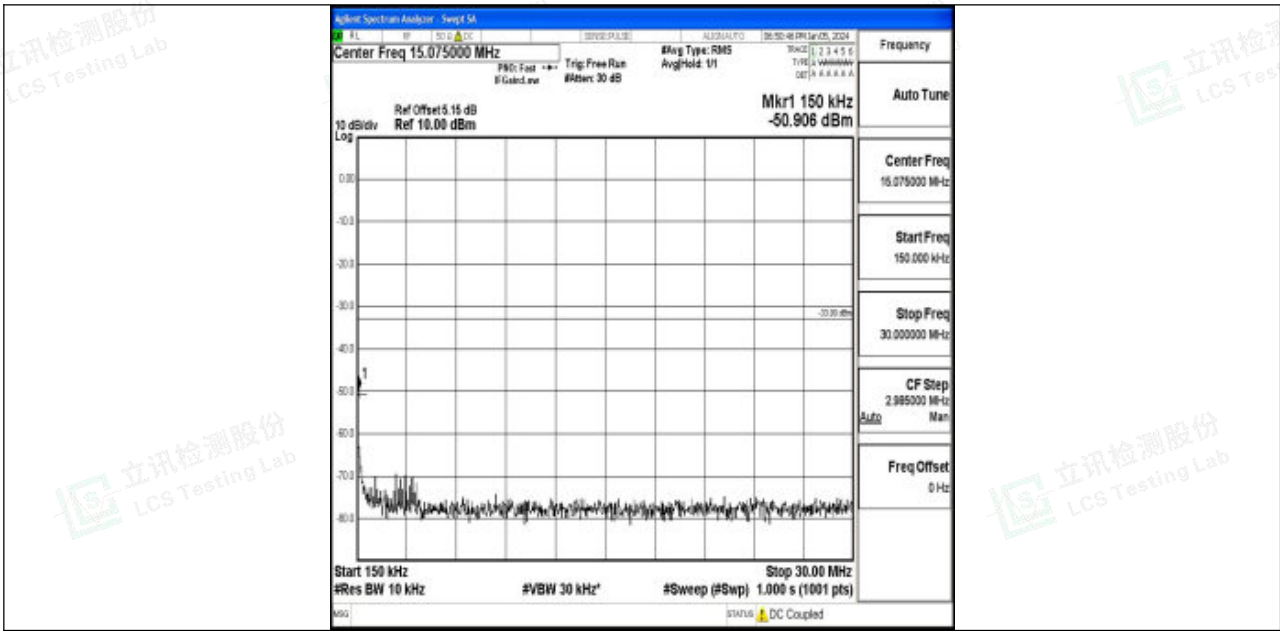
Band4_3MHz_QPSK_19965_1RB#0_0.15~30_0.15~30
