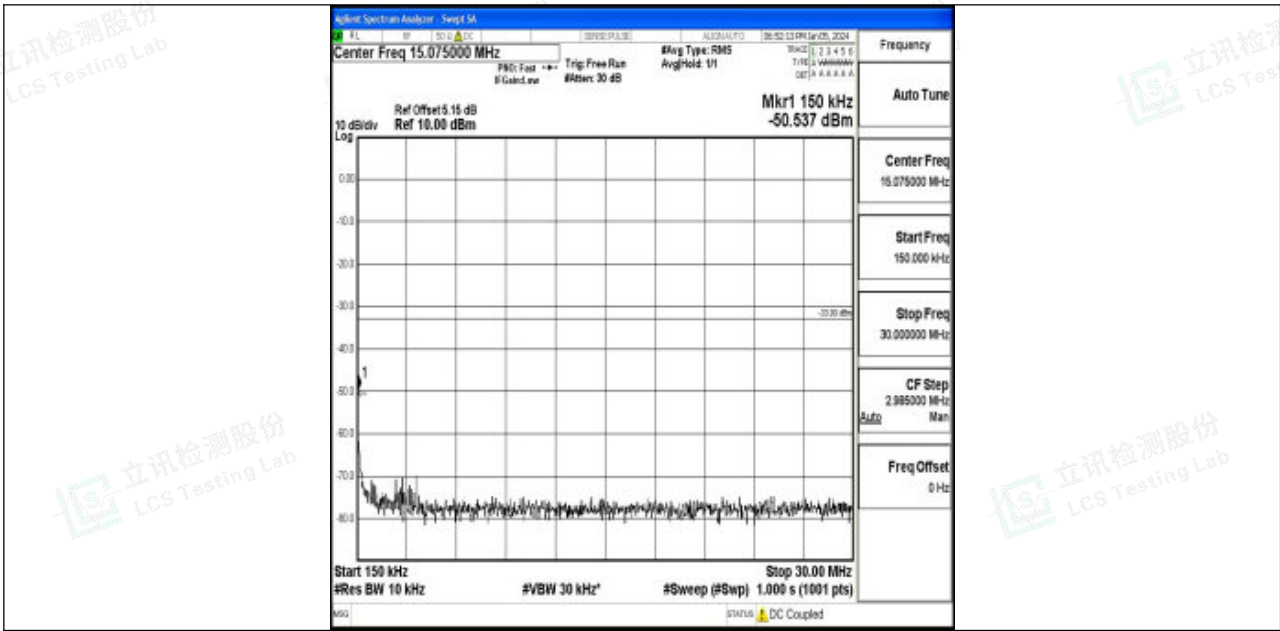
Band4_3MHz_QPSK_20175_1RB#0_0.15~30_0.15~30
