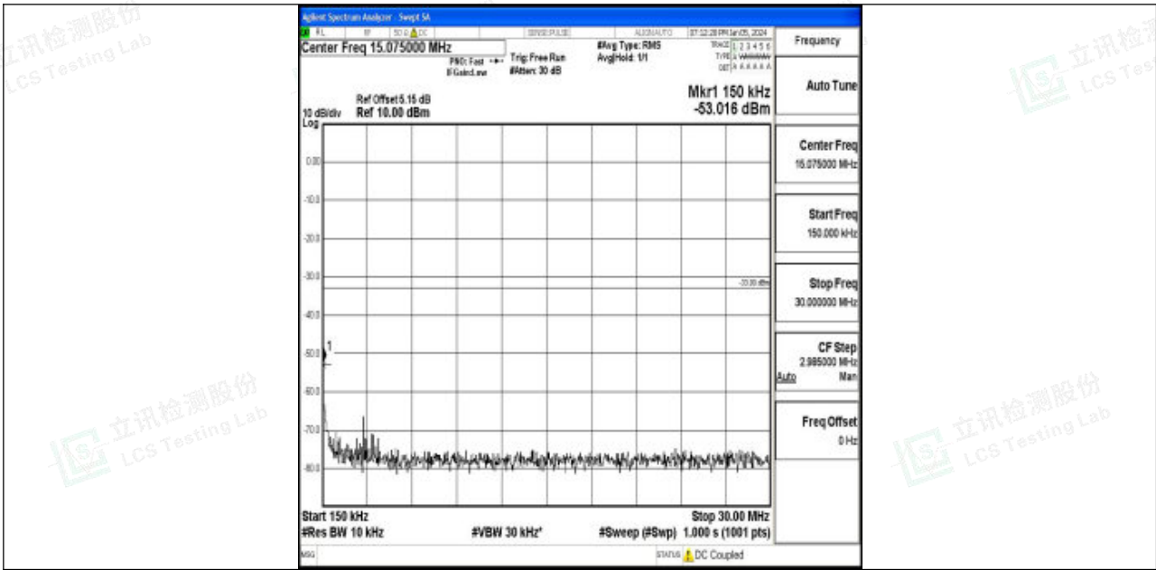
Band4_5MHz_QPSK_20375_1RB#0_0.15~30_0.15~30
