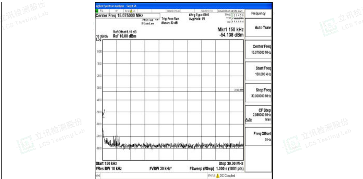
Band2_20MHz_QPSK_19100_1RB#0_0.15~30_0.15~30
