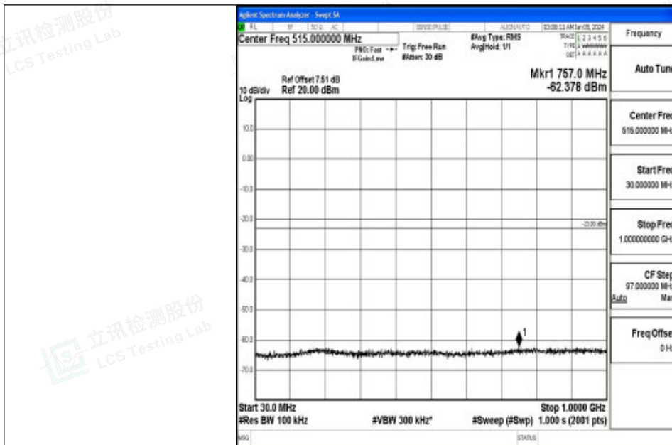
Band2_15MHz_16QAM_18900_1RB#0_30~1000_30~1000
