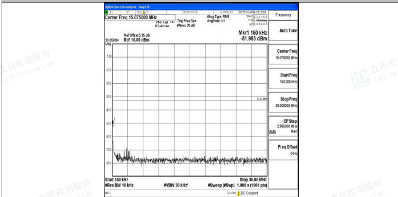
Band2_10MHz_16QAM_19150_1RB#0_0.15~30_0.15~30
