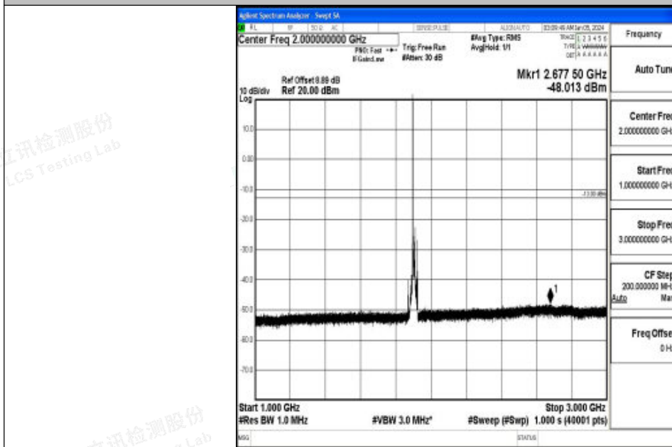
Band2_15MHz_16QAM_19125_1RB#0_1000~3000_1000~3000
