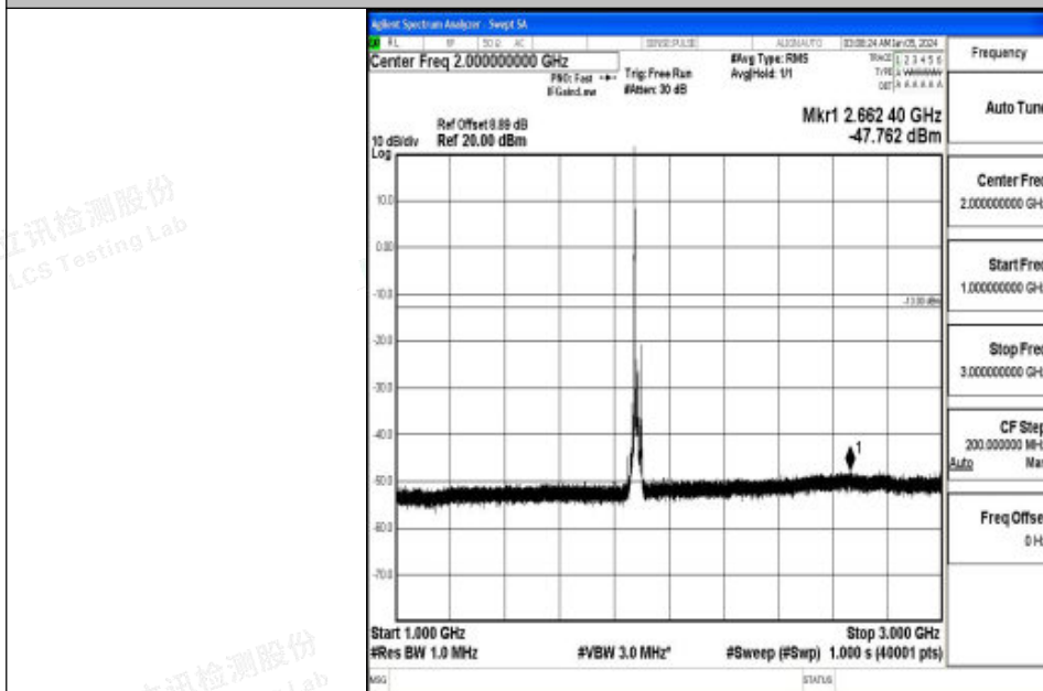
Band2_15MHz_16QAM_18900_1RB#0_1000~3000_1000~3000
