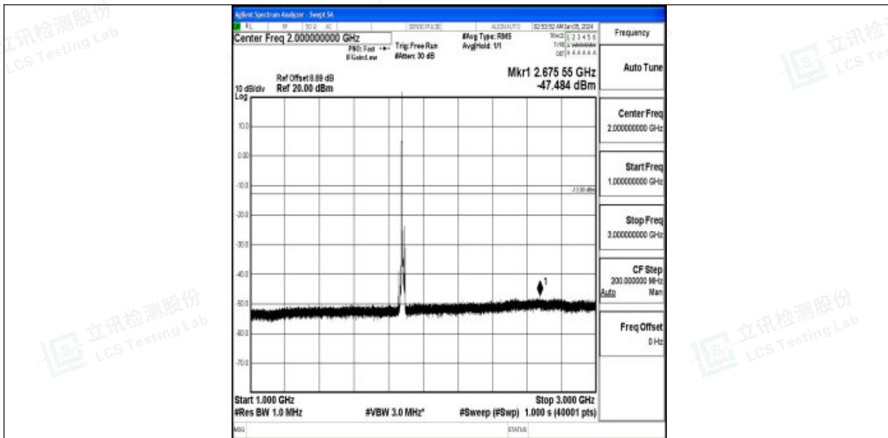
Band2_10MHz_QPSK_18900_1RB#0_1000~3000_1000~3000
