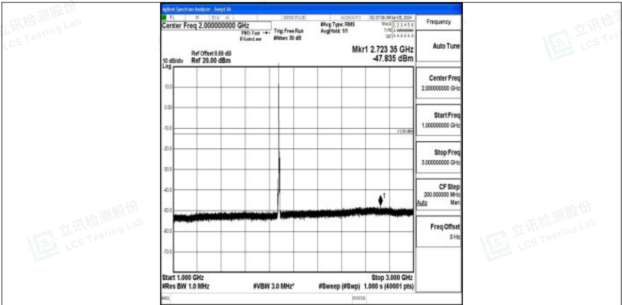
Band2_5MHz_QPSK_18900_1RB#0_1000~3000_1000~3000
