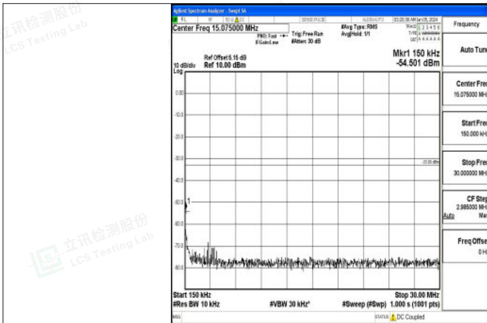
Band2_20MHz_QPSK_18900_1RB#0_0.15~30_0.15~30
