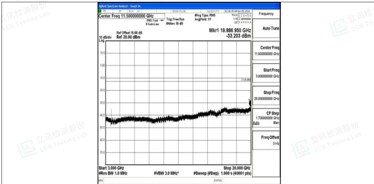
Band2_5MHz_16QAM_18625_1RB#0_3000~20000_3000~20000
