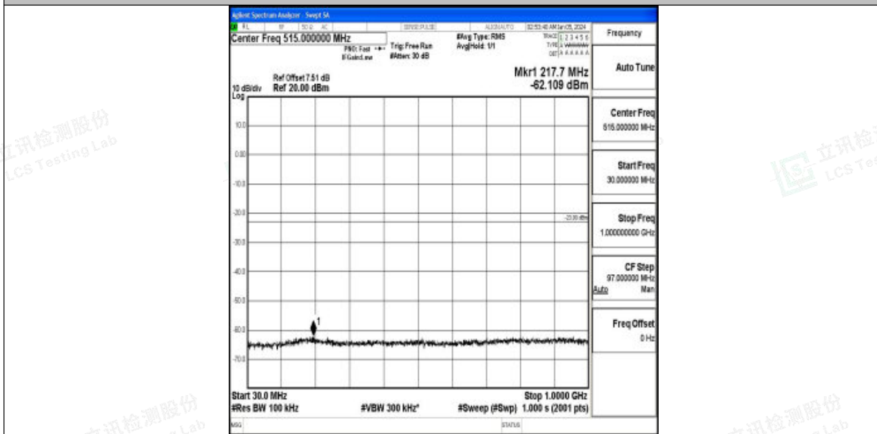
Band2_10MHz_QPSK_18900_1RB#0_30~1000_30~1000
