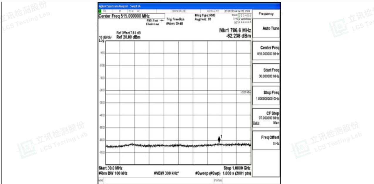
Band2_20MHz_16QAM_18700_1RB#0_30~1000_30~1000
