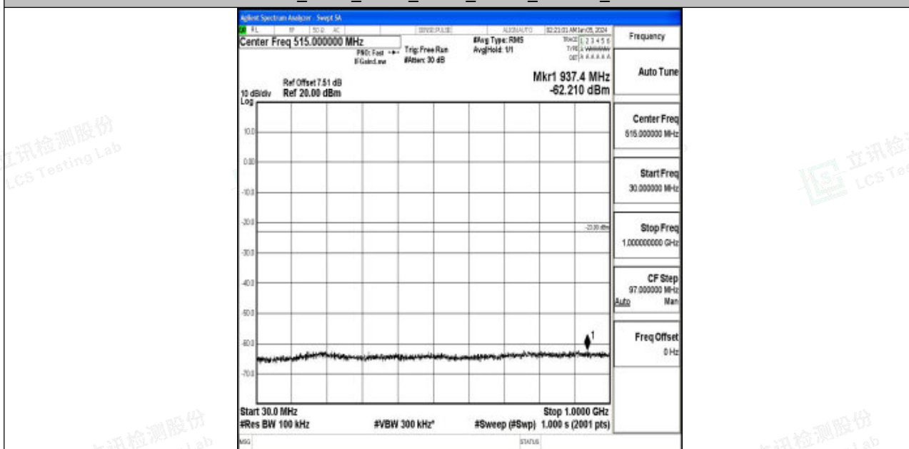
Band2_3MHz_QPSK_19185_1RB#0_30~1000_30~1000
