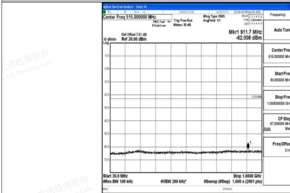
Band2_20MHz_QPSK_18900_1RB#0_30~1000_30~1000
