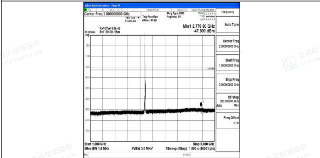
Band2_5MHz_16QAM_18900_1RB#0_1000~3000_1000~3000
