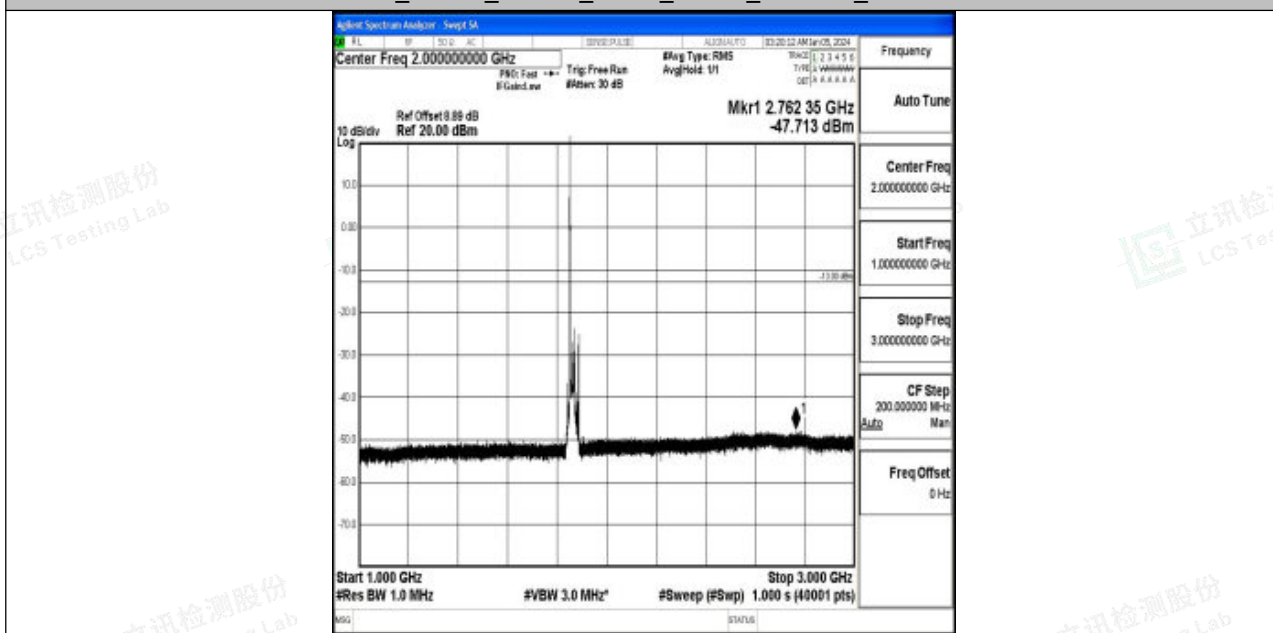
Band2_20MHz_16QAM_18700_1RB#0_1000~3000_1000~3000
