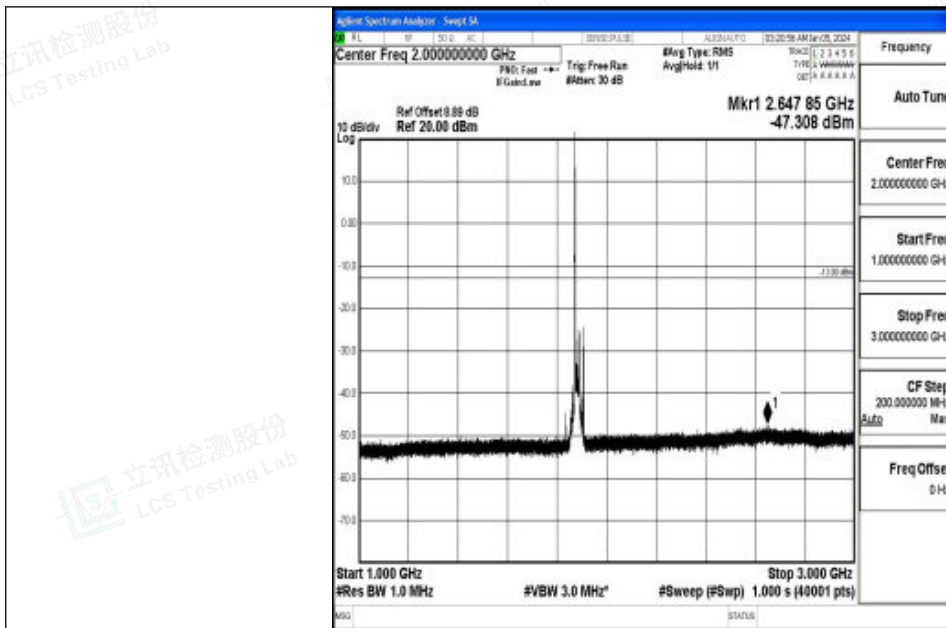
Band2_20MHz_QPSK_18900_1RB#0_1000~3000_1000~3000
