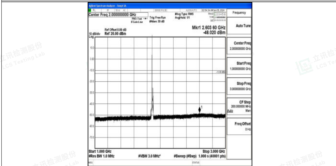
Band2_10MHz_16QAM_18900_1RB#0_1000~3000_1000~3000
