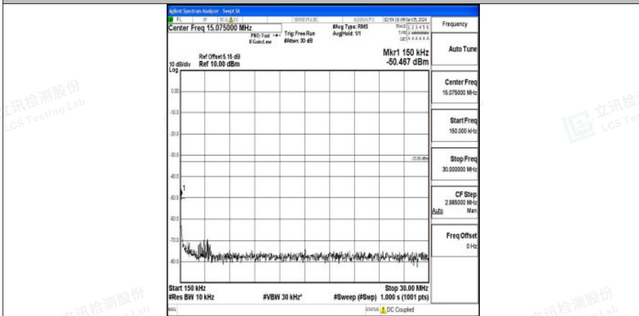
Band2_10MHz_16QAM_18900_1RB#0_0.15~30_0.15~30
