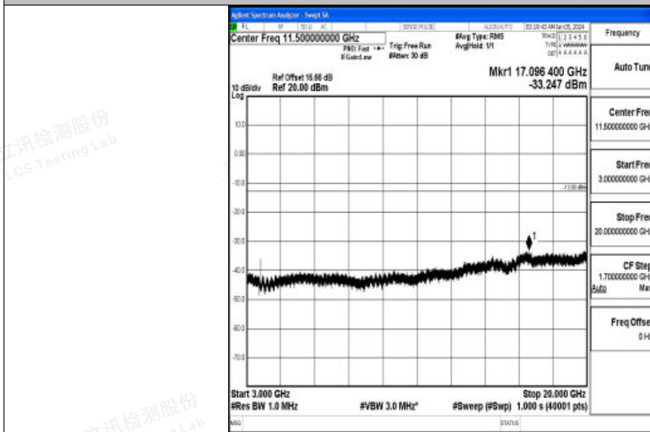
Band2_20MHz_QPSK_18700_1RB#0_3000~20000_3000~20000
