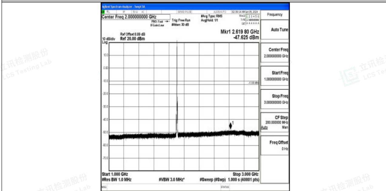
Band2_5MHz_16QAM_19175_1RB#0_1000~3000_1000~3000
