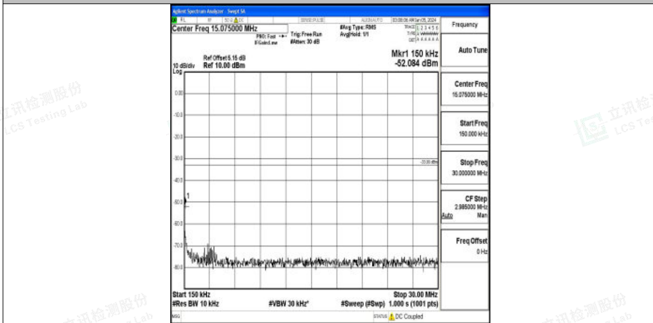
Band2_15MHz_16QAM_18900_1RB#0_0.15~30_0.15~30
