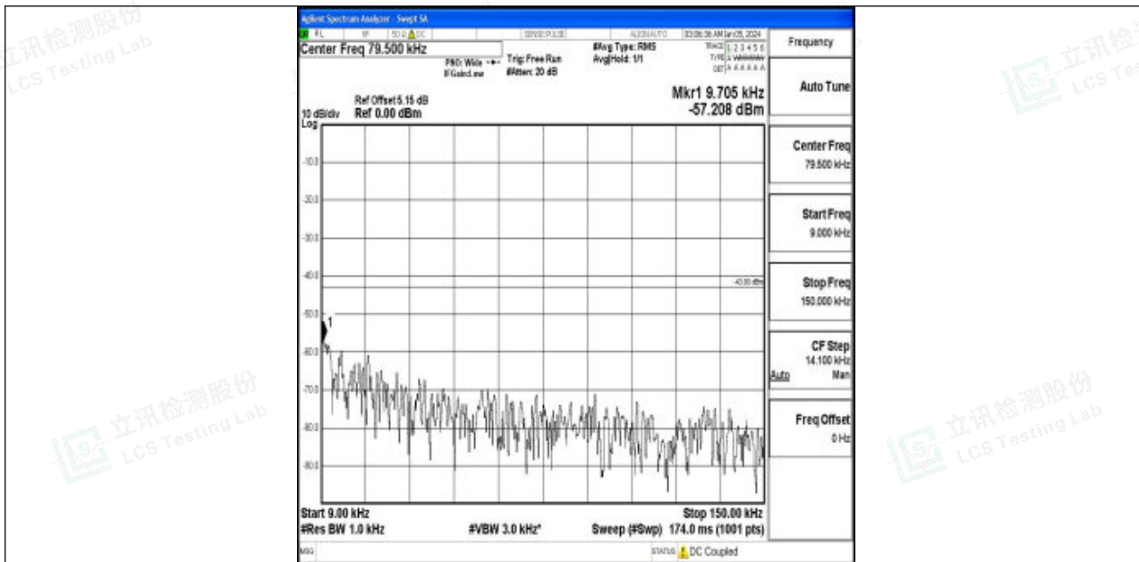
Band2_15MHz_16QAM_18675_1RB#0_0.009~0.15_0.009~0.15
