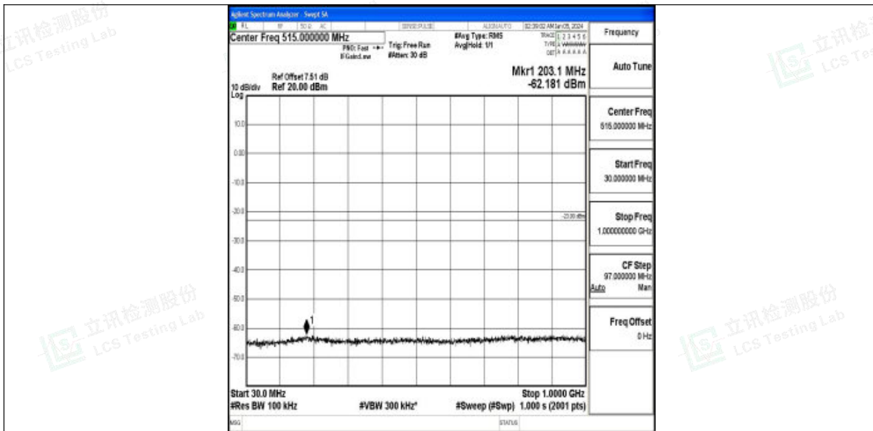
Band2_5MHz_16QAM_19175_1RB#0_30~1000_30~1000
