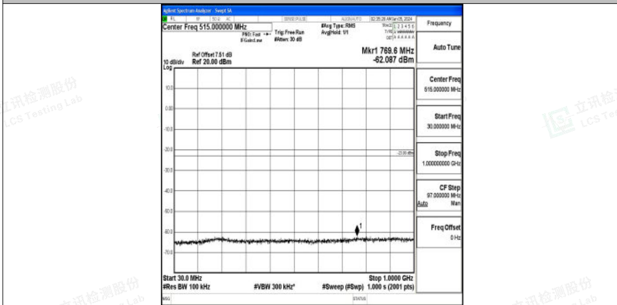
Band2_5MHz_QPSK_18625_1RB#0_30~1000_30~1000
