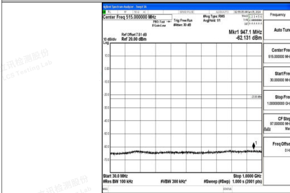
Band2_10MHz_QPSK_19150_1RB#0_30~1000_30~1000
