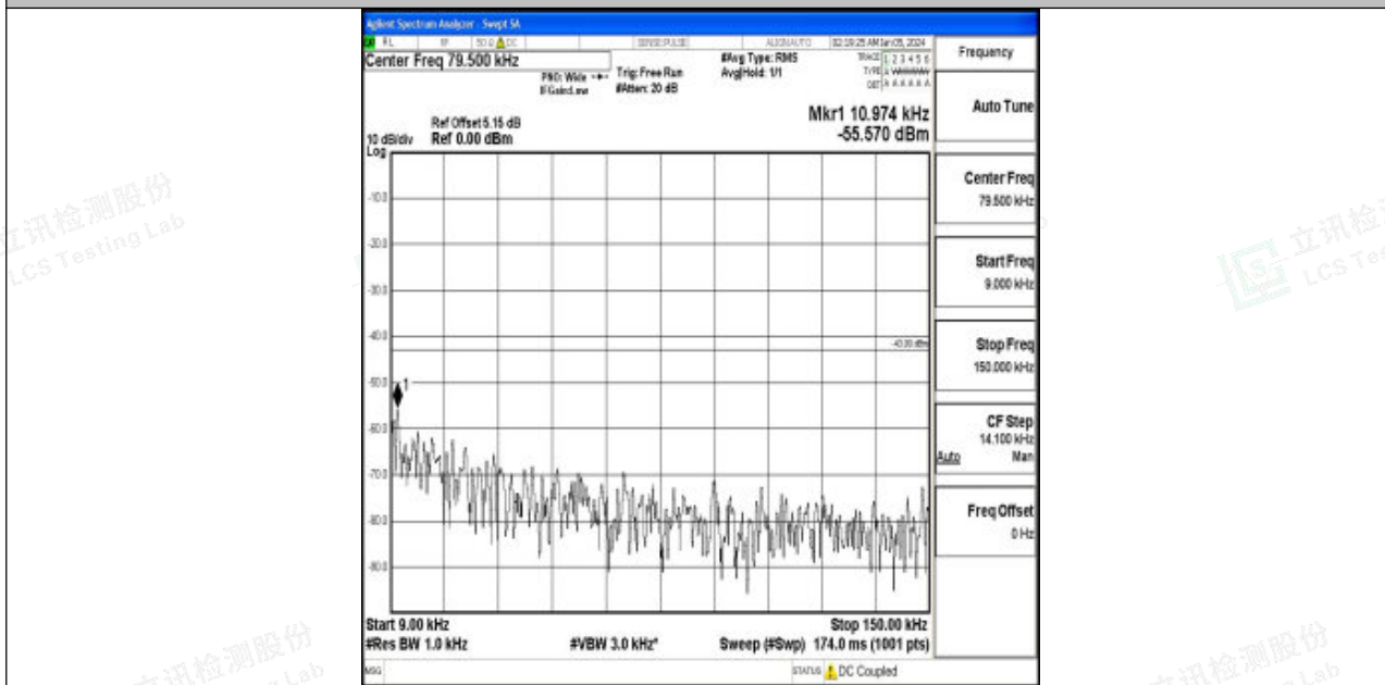
Band2_3MHz_QPSK_18900_1RB#0_0.009~0.15_0.009~0.15
