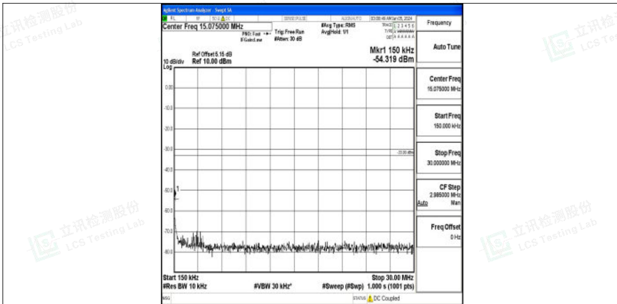
Band2_15MHz_QPSK_19125_1RB#0_0.15~30_0.15~30
