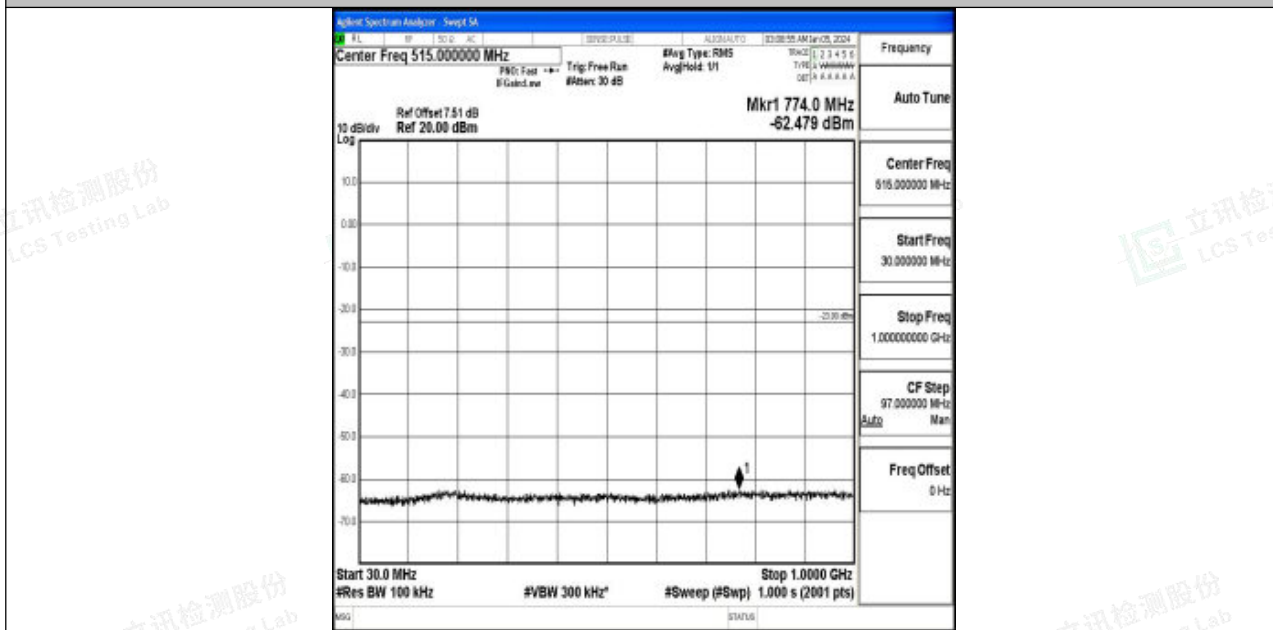
Band2_15MHz_QPSK_19125_1RB#0_30~1000_30~1000
