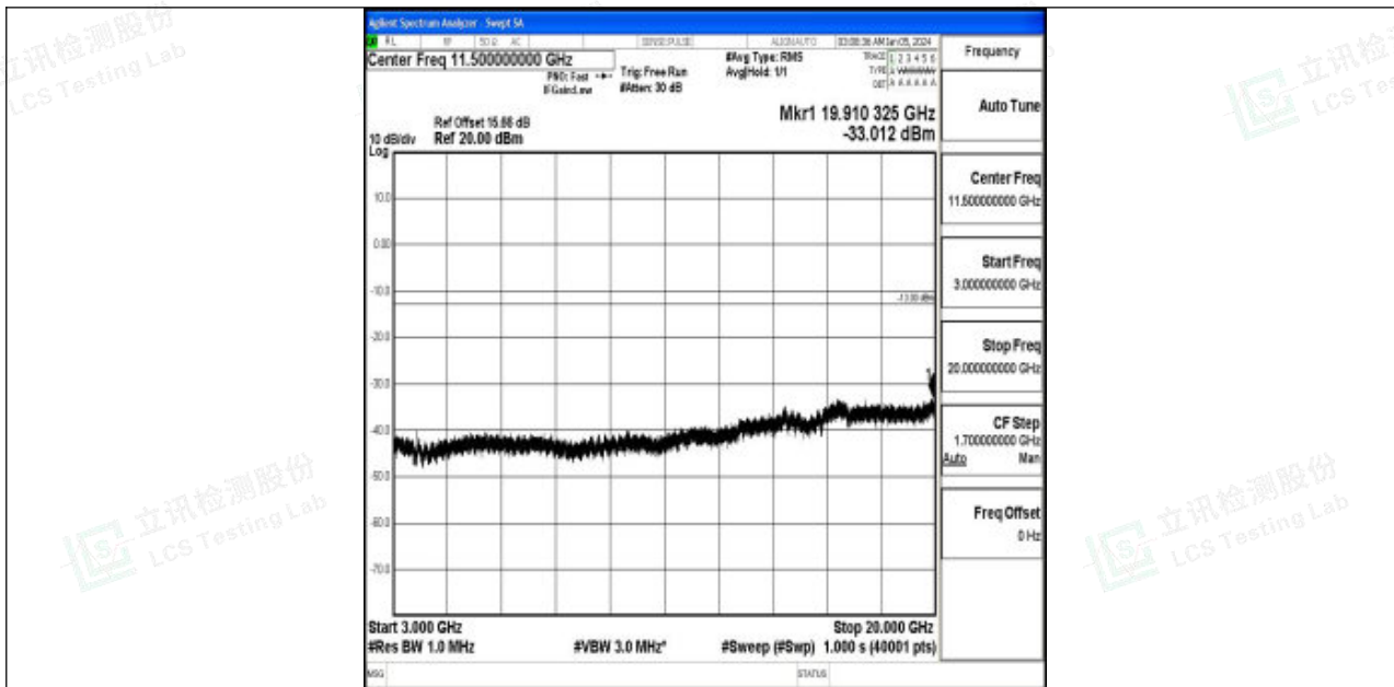
Band2_15MHz_16QAM_18900_1RB#0_3000~20000_3000~20000
