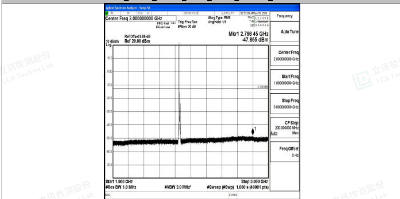
Band2_10MHz_16QAM_18650_1RB#0_1000~3000_1000~3000
