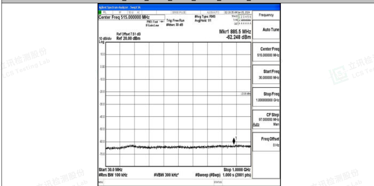
Band2_3MHz_QPSK_18900_1RB#0_30~1000_30~1000
