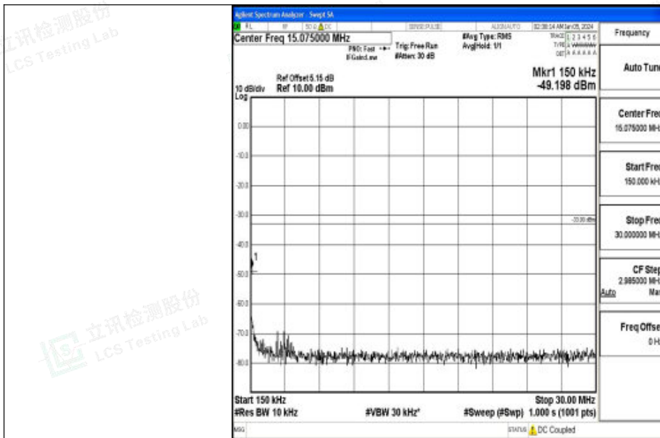
Band2_5MHz_QPSK_19175_1RB#0_0.15~30_0.15~30
