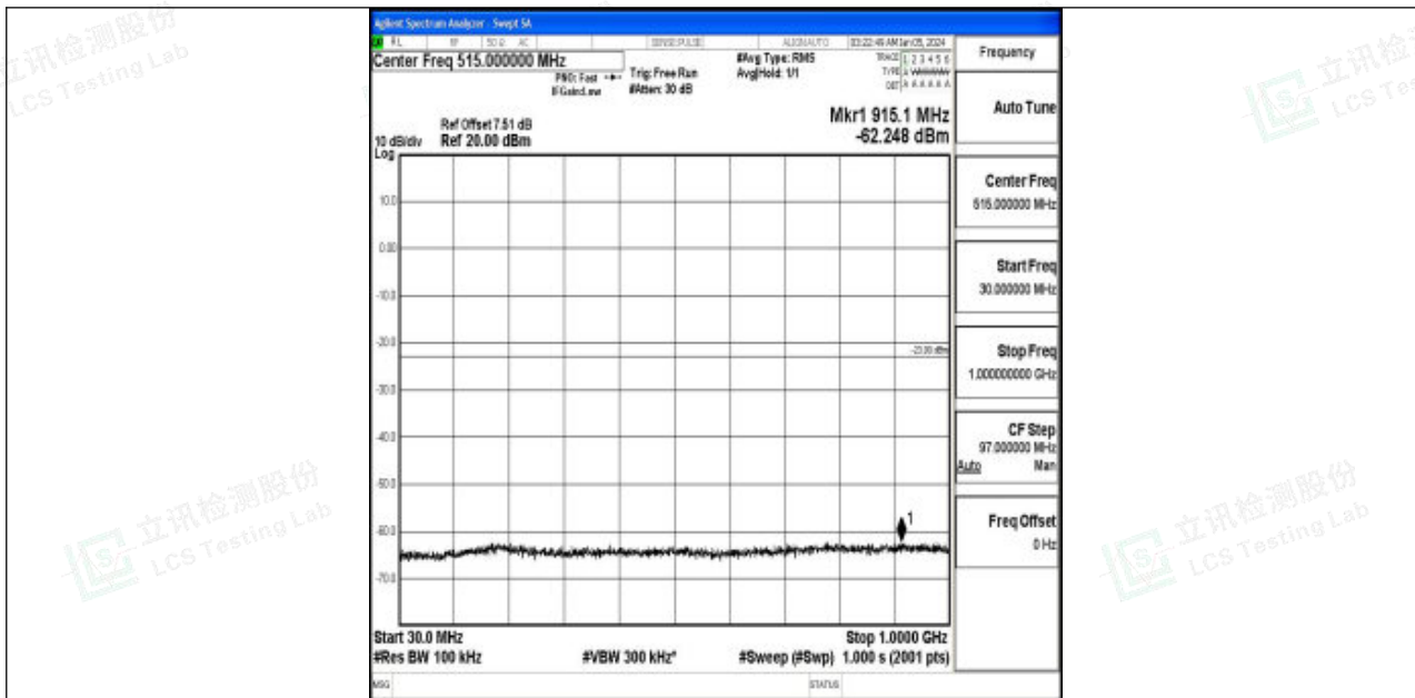
Band2_20MHz_16QAM_19100_1RB#0_30~1000_30~1000
