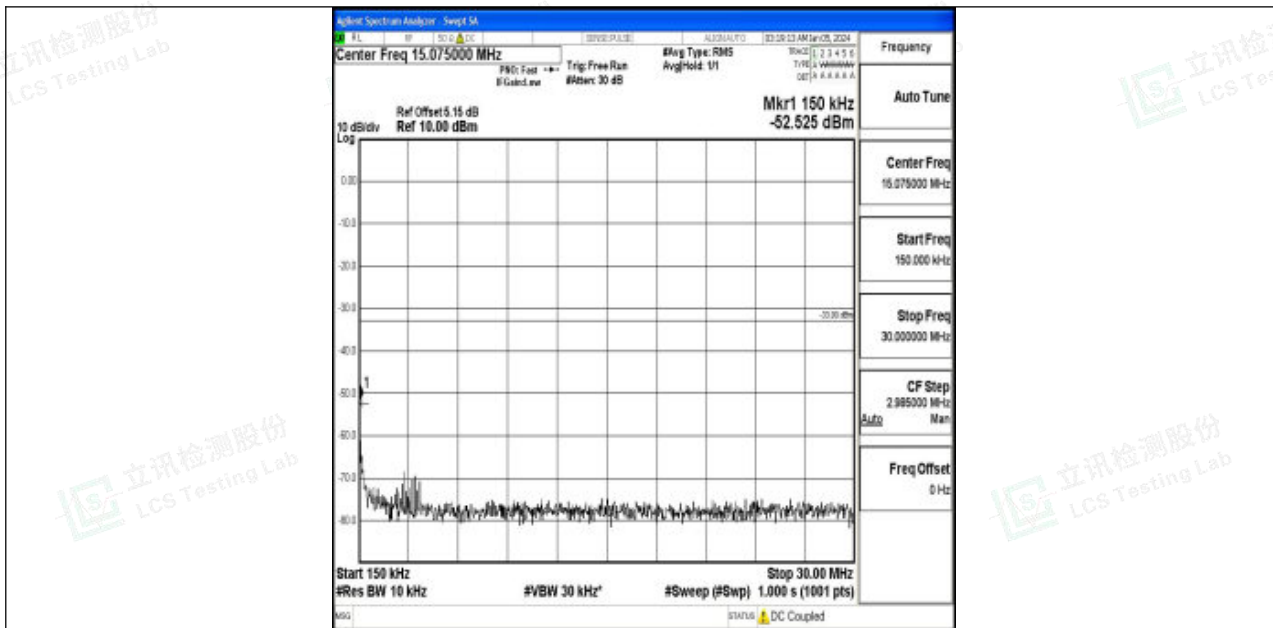
Band2_20MHz_QPSK_18700_1RB#0_0.15~30_0.15~30
