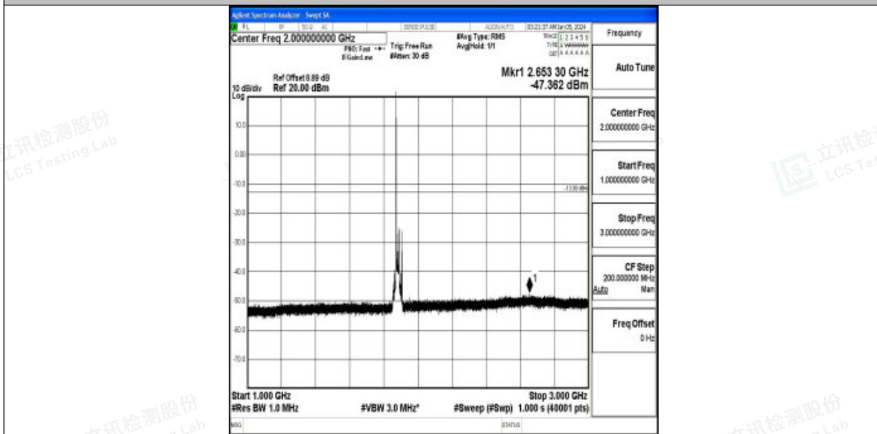
Band2_20MHz_16QAM_18900_1RB#0_1000~3000_1000~3000
