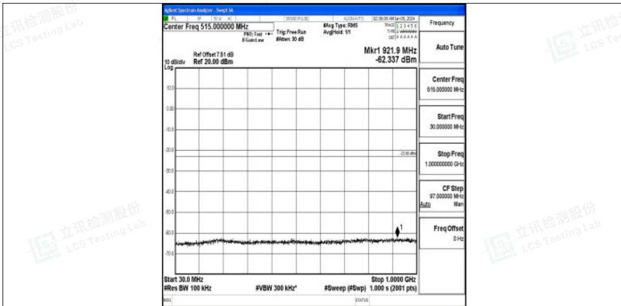
Band2_5MHz_16QAM_18625_1RB#0_30~1000_30~1000
