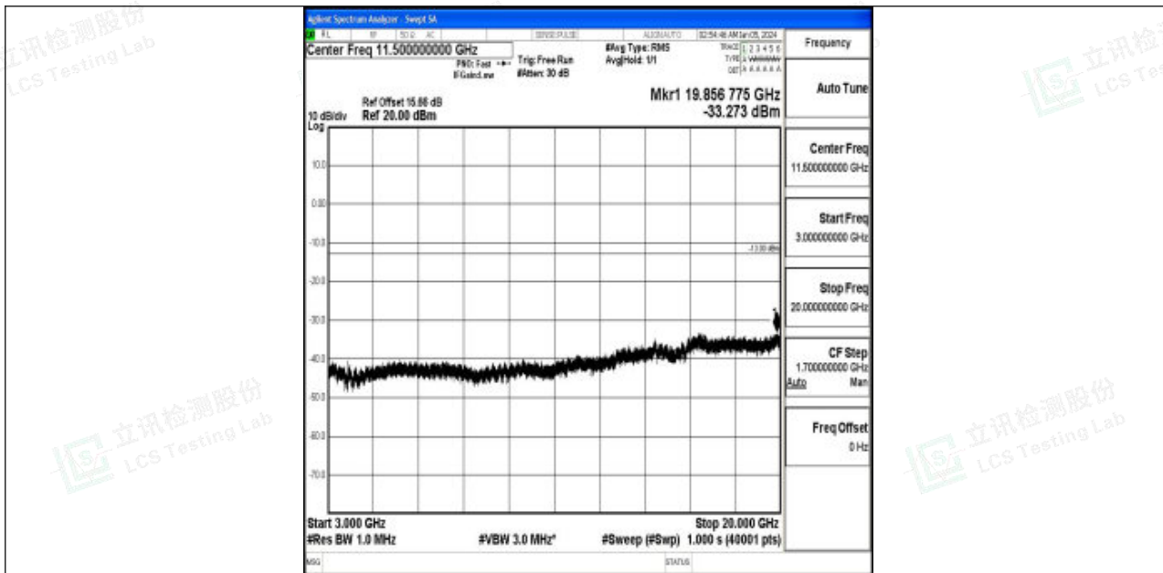
Band2_10MHz_16QAM_18900_1RB#0_3000~20000_3000~20000
