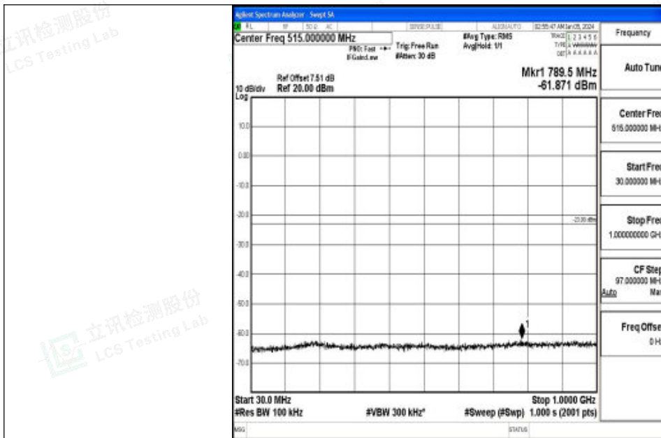
Band2_10MHz_16QAM_19150_1RB#0_30~1000_30~1000
