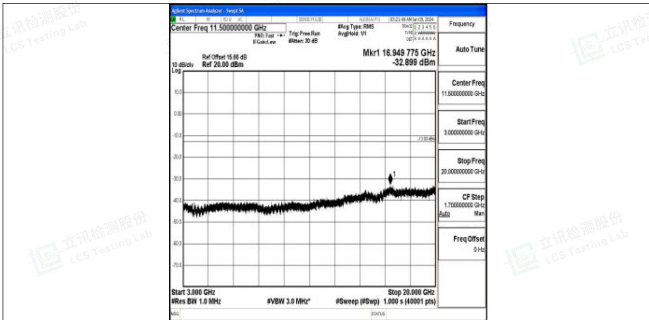
Band2_20MHz_16QAM_18900_1RB#0_3000~20000_3000~20000
