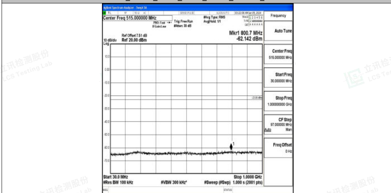
Band2_20MHz_QPSK_19100_1RB#0_30~1000_30~1000
