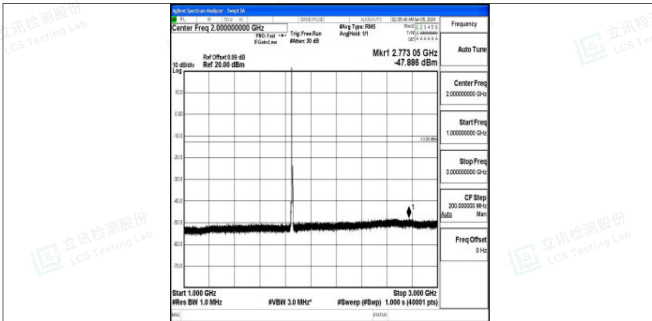
Band2_5MHz_QPSK_18625_1RB#0_1000~3000_1000~3000
