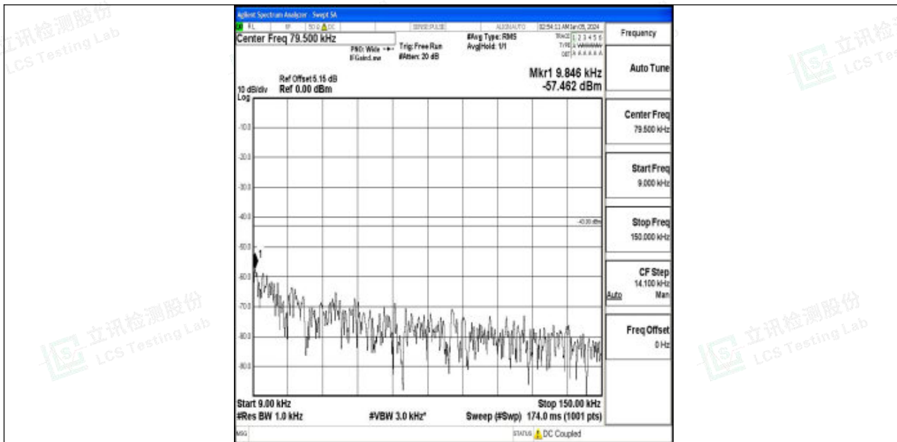
Band2_10MHz_16QAM_18900_1RB#0_0.009~0.15_0.009~0.15
