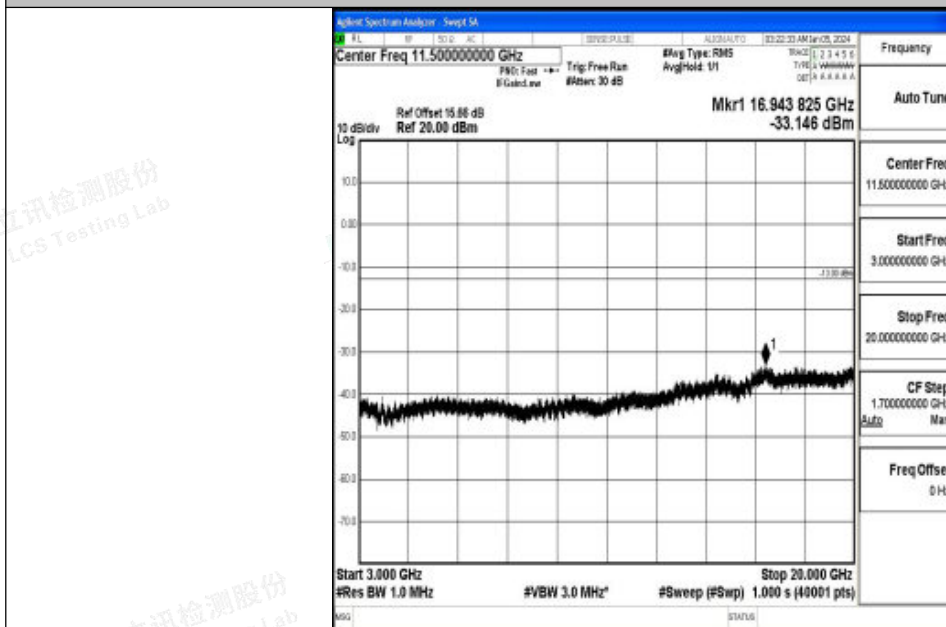
Band2_20MHz_QPSK_19100_1RB#0_3000~20000_3000~20000
