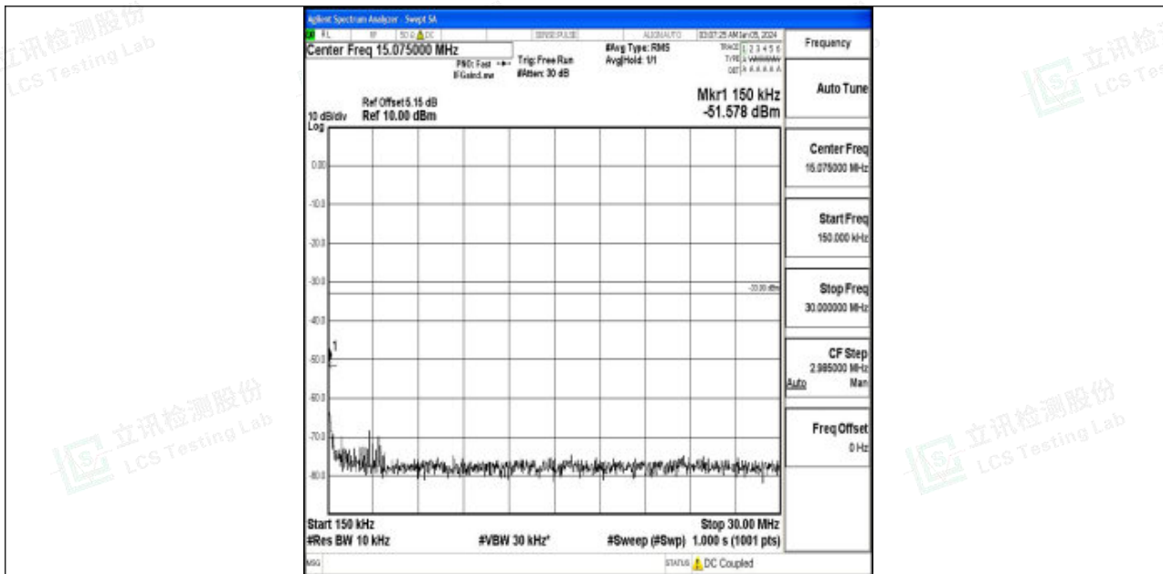
Band2_15MHz_QPSK_18900_1RB#0_0.15~30_0.15~30
