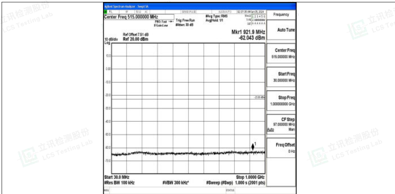
Band2_5MHz_16QAM_18900_1RB#0_30~1000_30~1000
