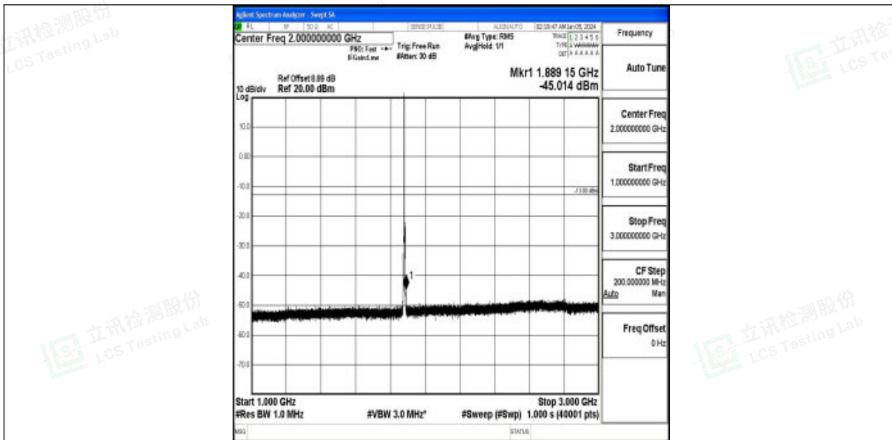
Band2_3MHz_QPSK_18900_1RB#0_1000~3000_1000~3000
