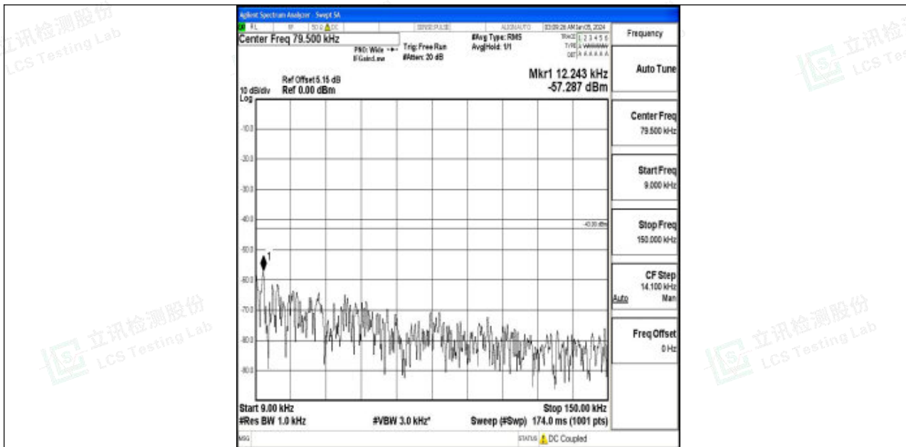
Band2_15MHz_16QAM_19125_1RB#0_0.009~0.15_0.009~0.15
