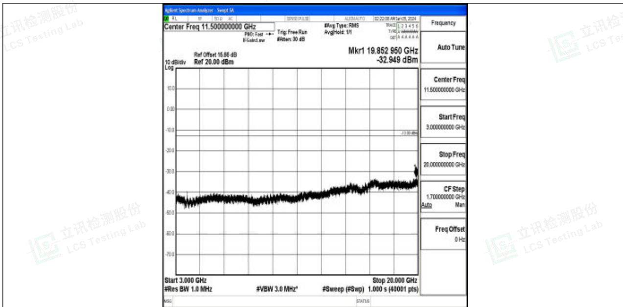
Band2_3MHz_16QAM_19185_1RB#0_3000~20000_3000~20000
