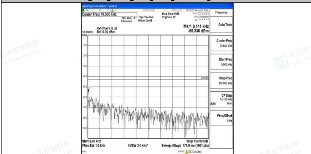
Band2_5MHz_QPSK_18625_1RB#0_0.009~0.15_0.009~0.15
