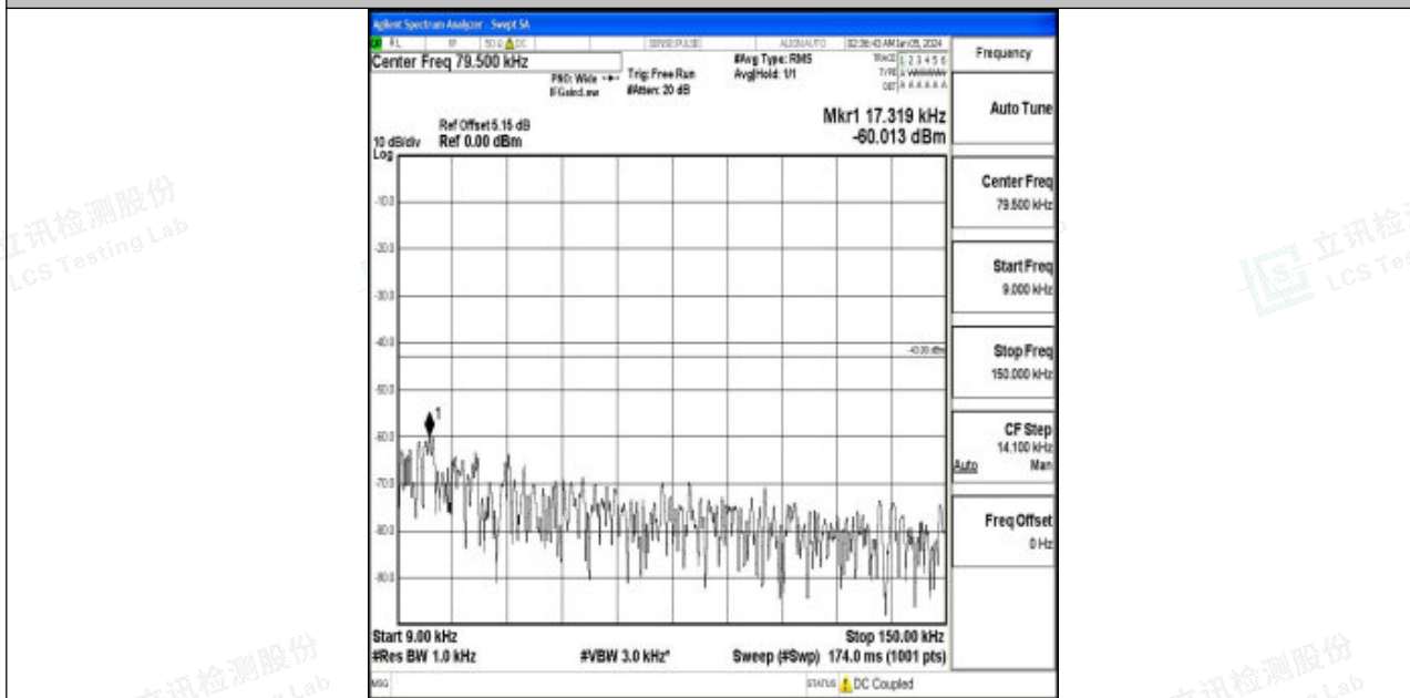
Band2_5MHz_QPSK_18900_1RB#0_0.009~0.15_0.009~0.15
