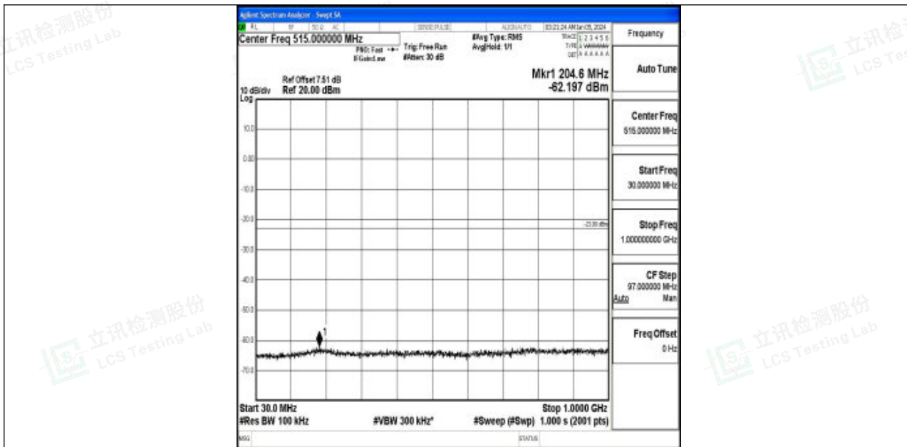
Band2_20MHz_16QAM_18900_1RB#0_30~1000_30~1000
