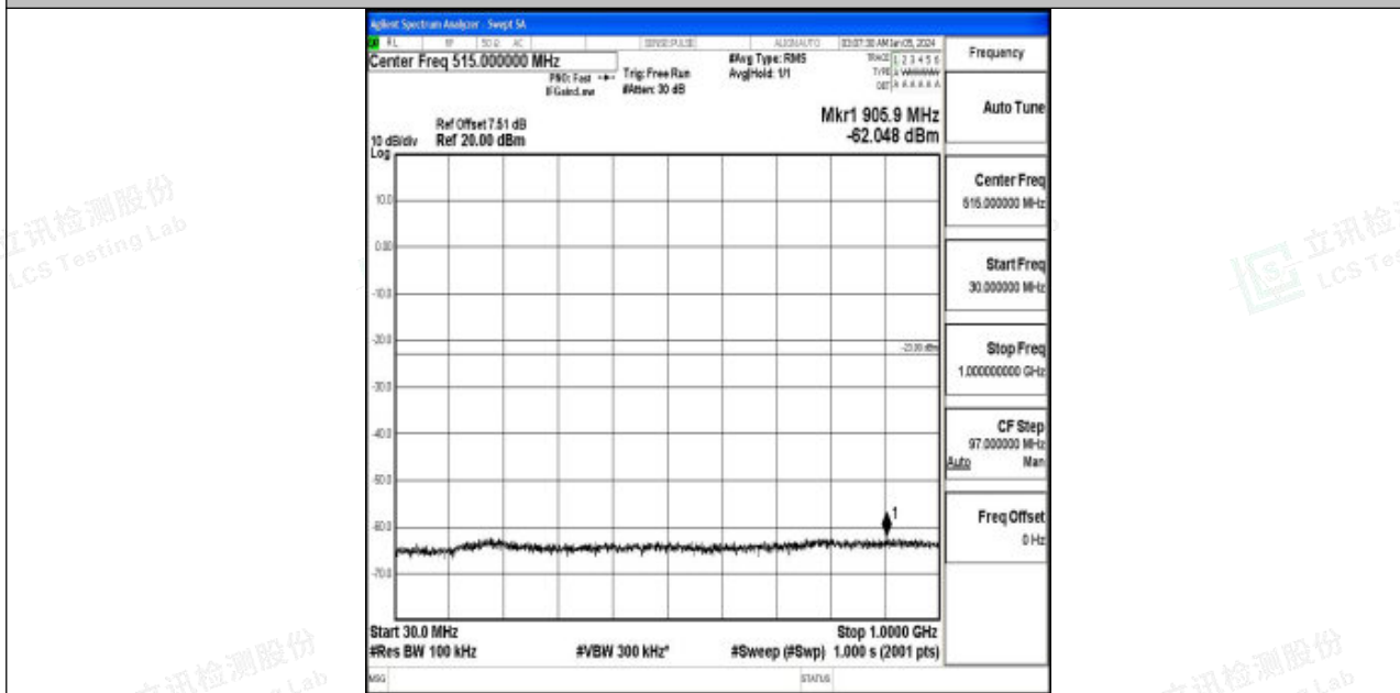
Band2_15MHz_QPSK_18900_1RB#0_30~1000_30~1000
