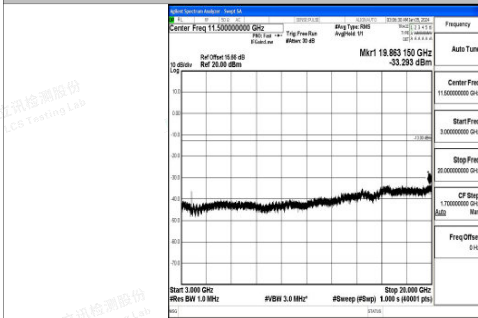
Band2_15MHz_QPSK_18675_1RB#0_3000~20000_3000~20000
