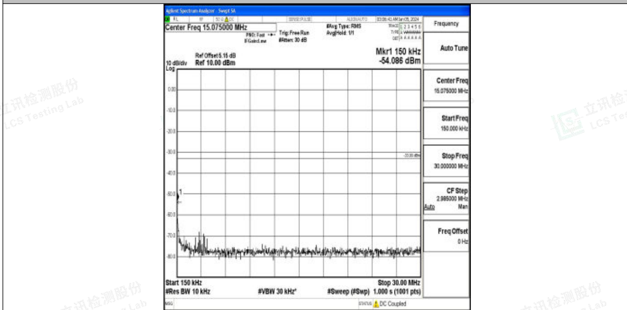
Band2_15MHz_16QAM_18675_1RB#0_0.15~30_0.15~30
