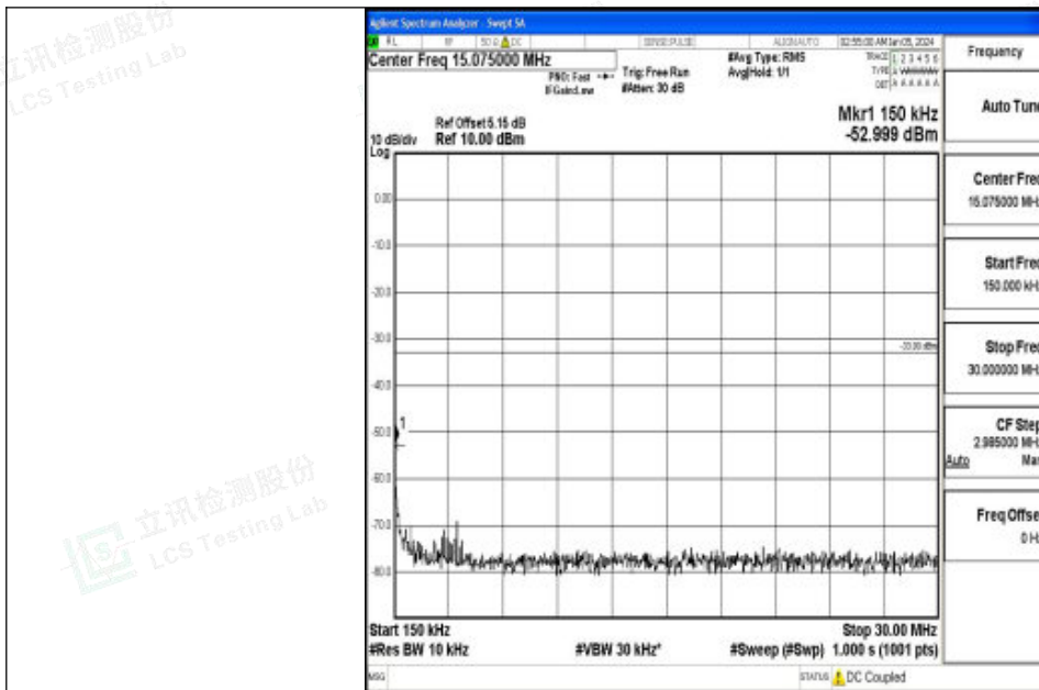
Band2_10MHz_QPSK_19150_1RB#0_0.15~30_0.15~30
