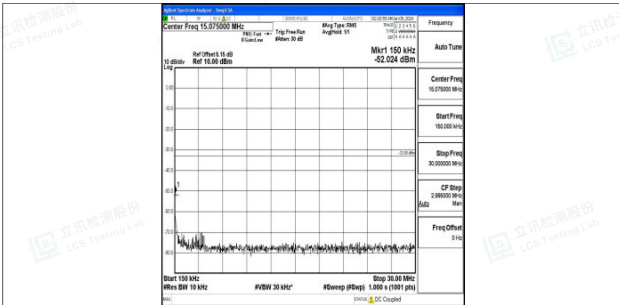
Band2_3MHz_QPSK_19185_1RB#0_0.15~30_0.15~30
