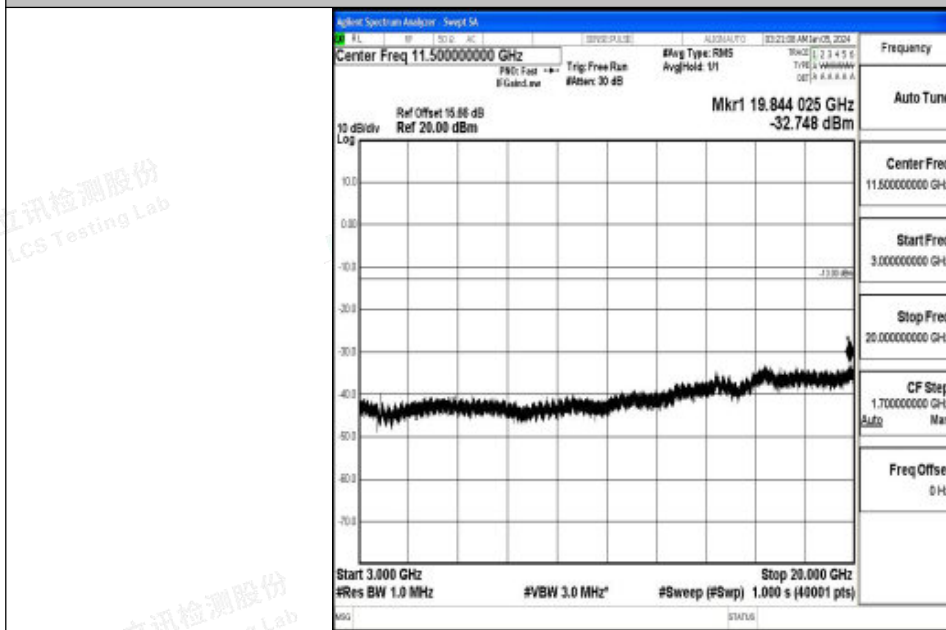
Band2_20MHz_QPSK_18900_1RB#0_3000~20000_3000~20000
