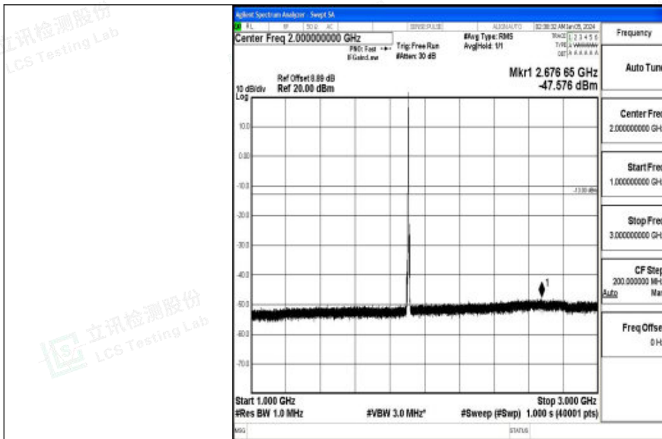
Band2_5MHz_QPSK_19175_1RB#0_1000~3000_1000~3000
