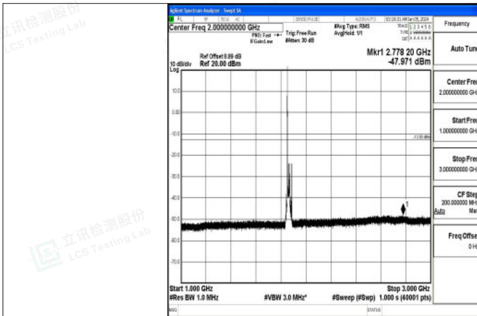
Band2_20MHz_QPSK_18700_1RB#0_1000~3000_1000~3000
