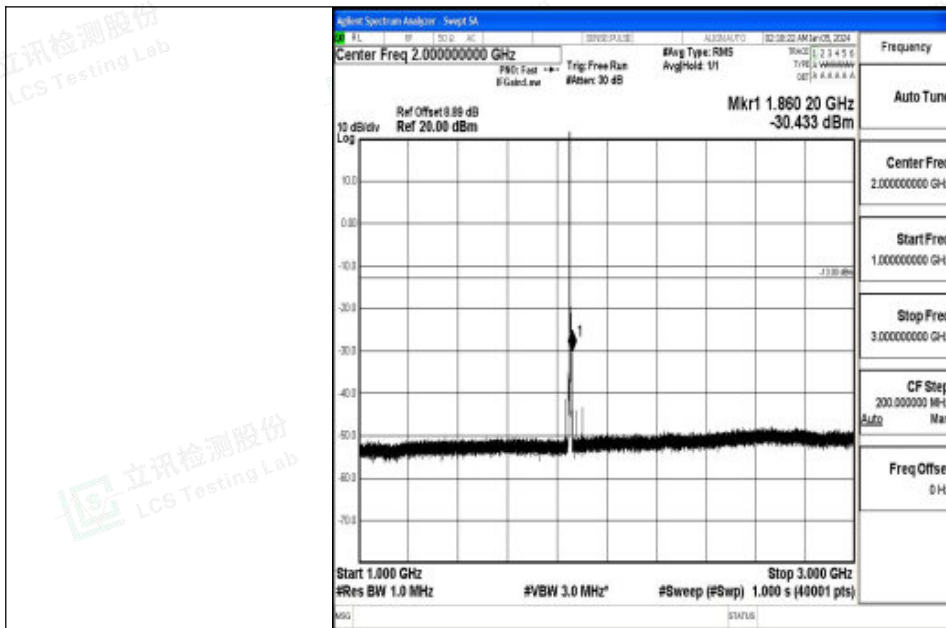
Band2_3MHz_QPSK_18615_1RB#0_1000~3000_1000~3000
