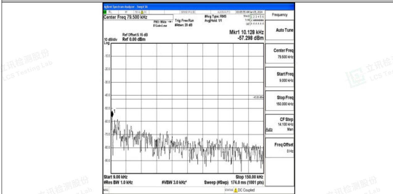
Band2_15MHz_QPSK_18675_1RB#0_0.009~0.15_0.009~0.15
