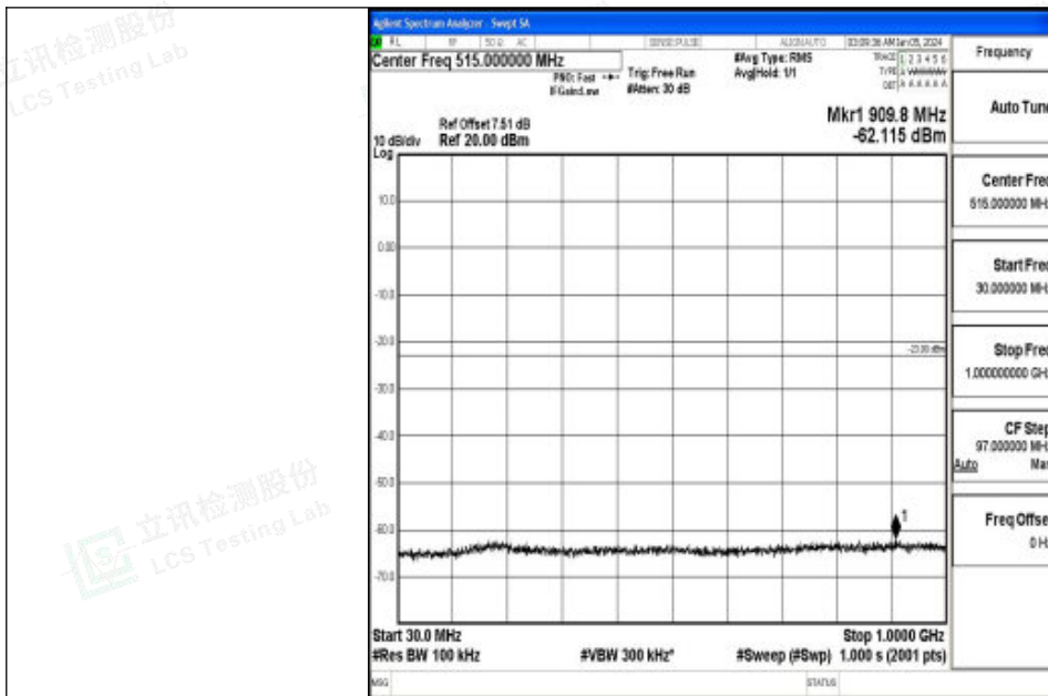
Band2_15MHz_16QAM_19125_1RB#0_30~1000_30~1000
