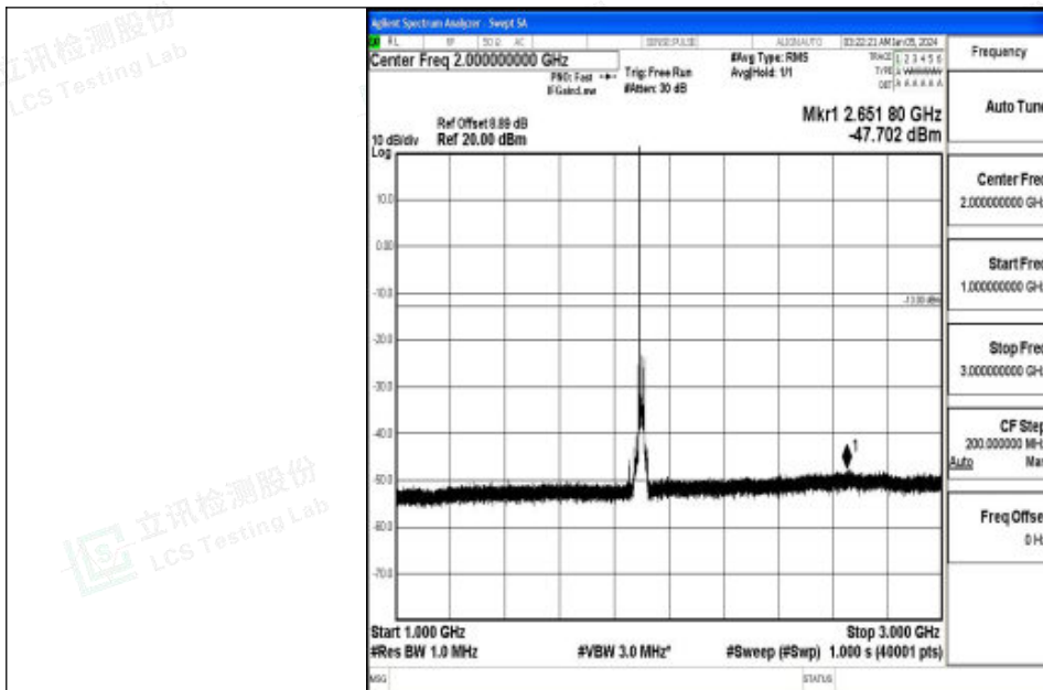
Band2_20MHz_QPSK_19100_1RB#0_1000~3000_1000~3000
