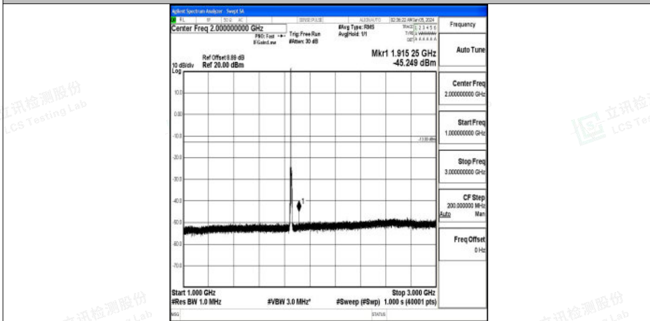
Band2_5MHz_16QAM_18625_1RB#0_1000~3000_1000~3000
