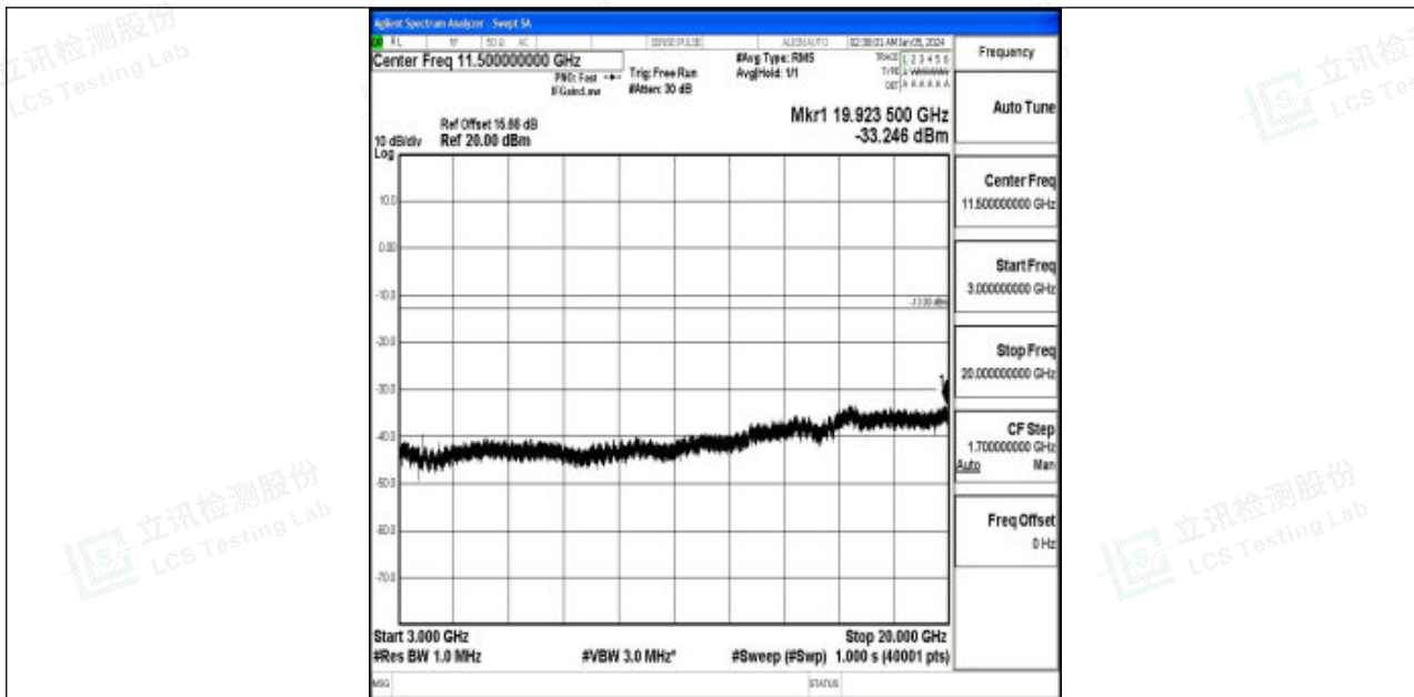
Band2_5MHz_16QAM_18900_1RB#0_3000~20000_3000~20000
