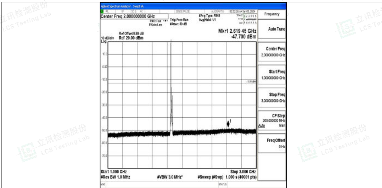
Band2_10MHz_QPSK_18650_1RB#0_1000~3000_1000~3000
