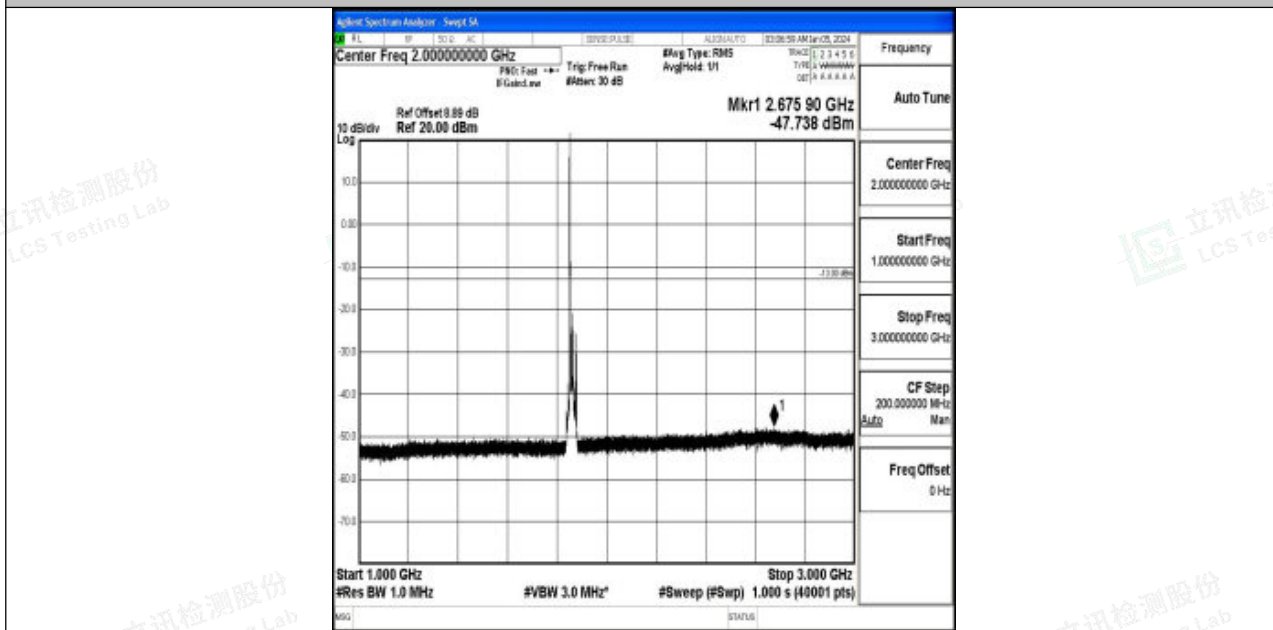
Band2_15MHz_16QAM_18675_1RB#0_1000~3000_1000~3000
