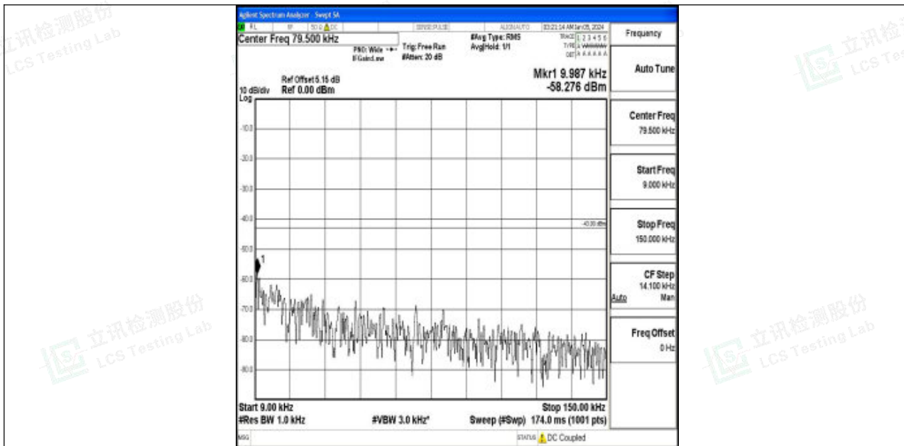
Band2_20MHz_16QAM_18900_1RB#0_0.009~0.15_0.009~0.15
