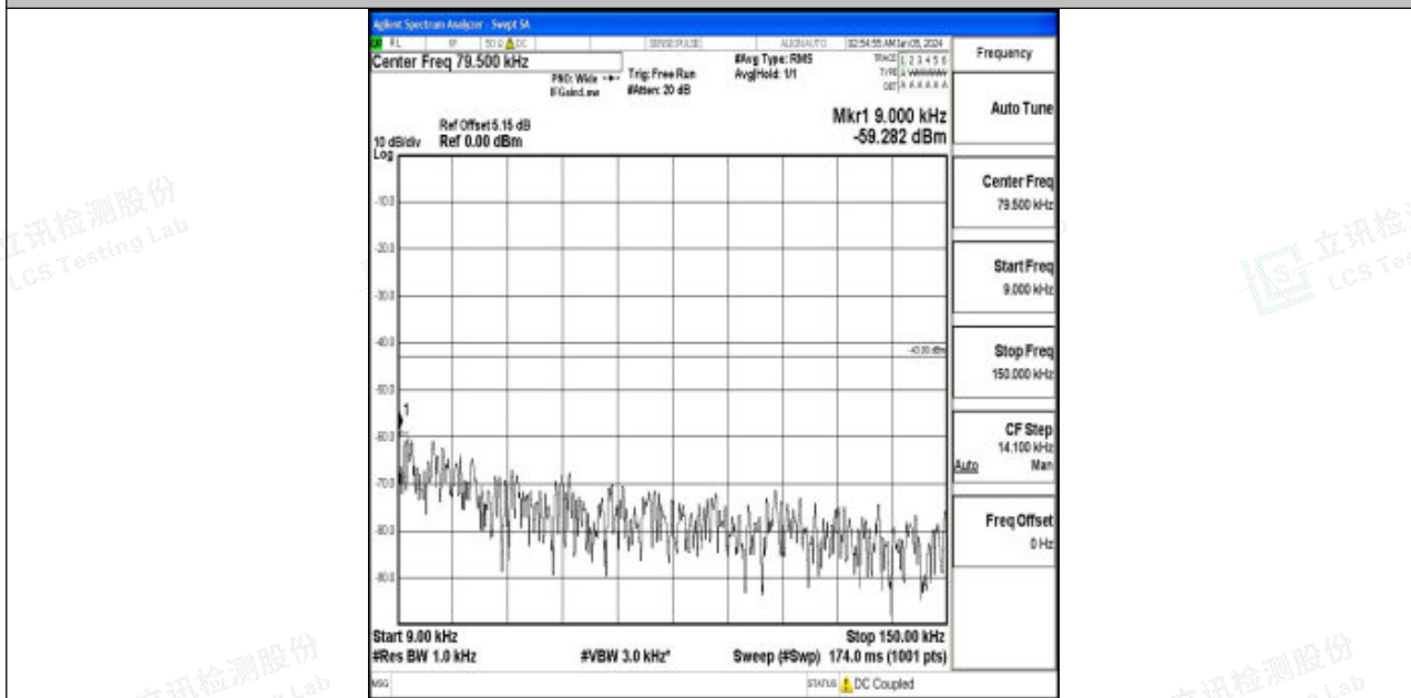
Band2_10MHz_QPSK_19150_1RB#0_0.009~0.15_0.009~0.15
