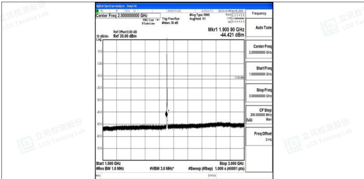
Band2_3MHz_QPSK_19185_1RB#0_1000~3000_1000~3000
