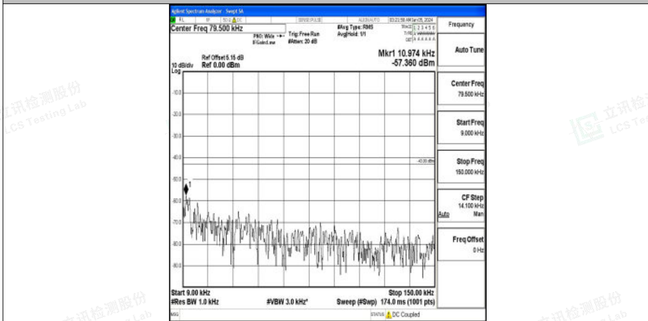
Band2_20MHz_QPSK_19100_1RB#0_0.009~0.15_0.009~0.15
