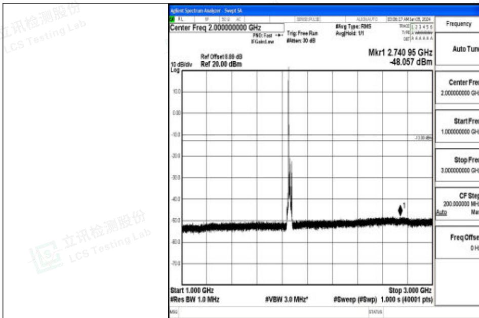
Band2_15MHz_QPSK_18675_1RB#0_1000~3000_1000~3000
