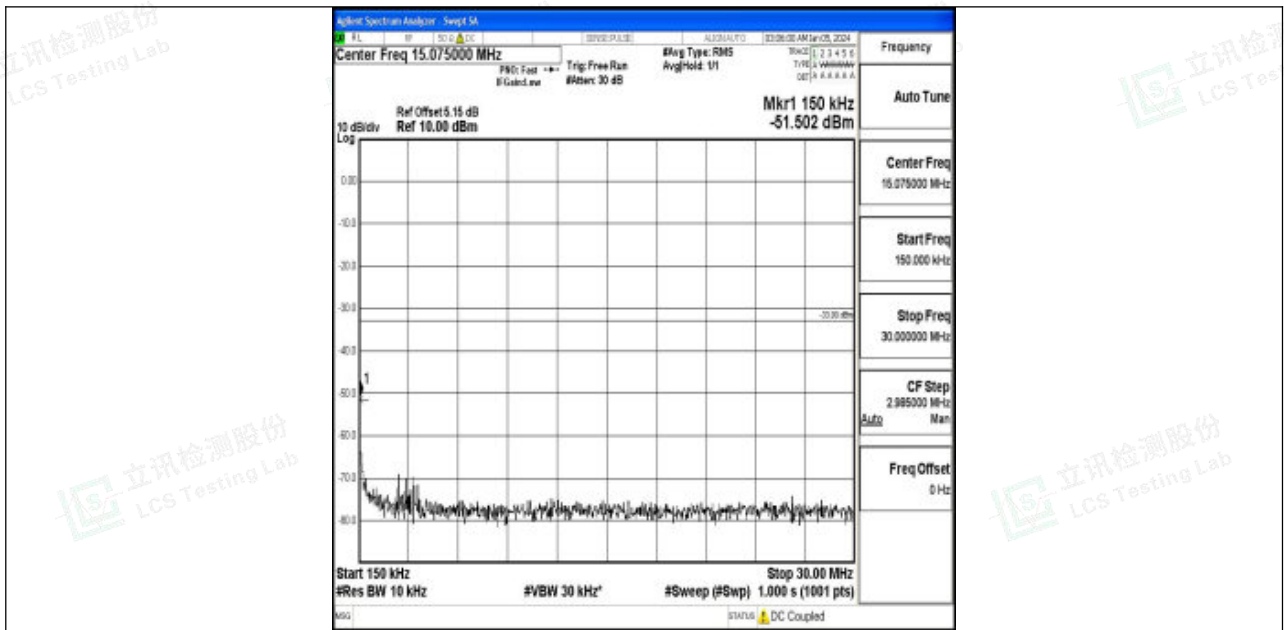
Band2_15MHz_QPSK_18675_1RB#0_0.15~30_0.15~30
