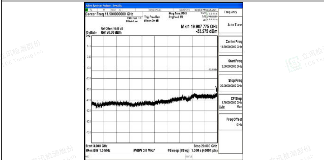
Band2_10MHz_QPSK_19150_1RB#0_3000~20000_3000~20000
