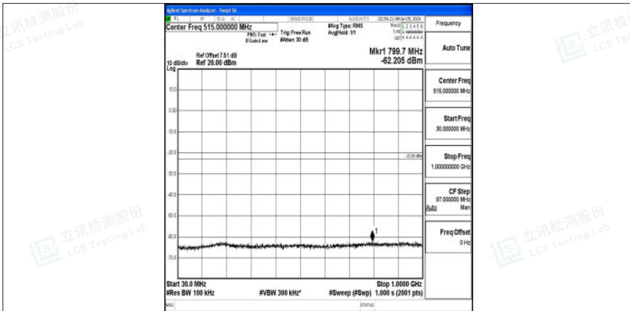
Band2_10MHz_16QAM_18900_1RB#0_30~1000_30~1000
