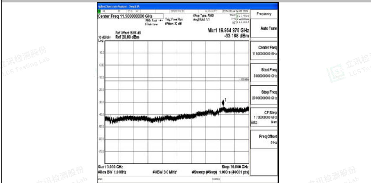
Band2_10MHz_QPSK_18900_1RB#0_3000~20000_3000~20000
