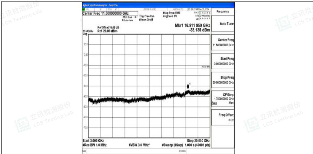
Band2_5MHz_16QAM_19175_1RB#0_3000~20000_3000~20000
