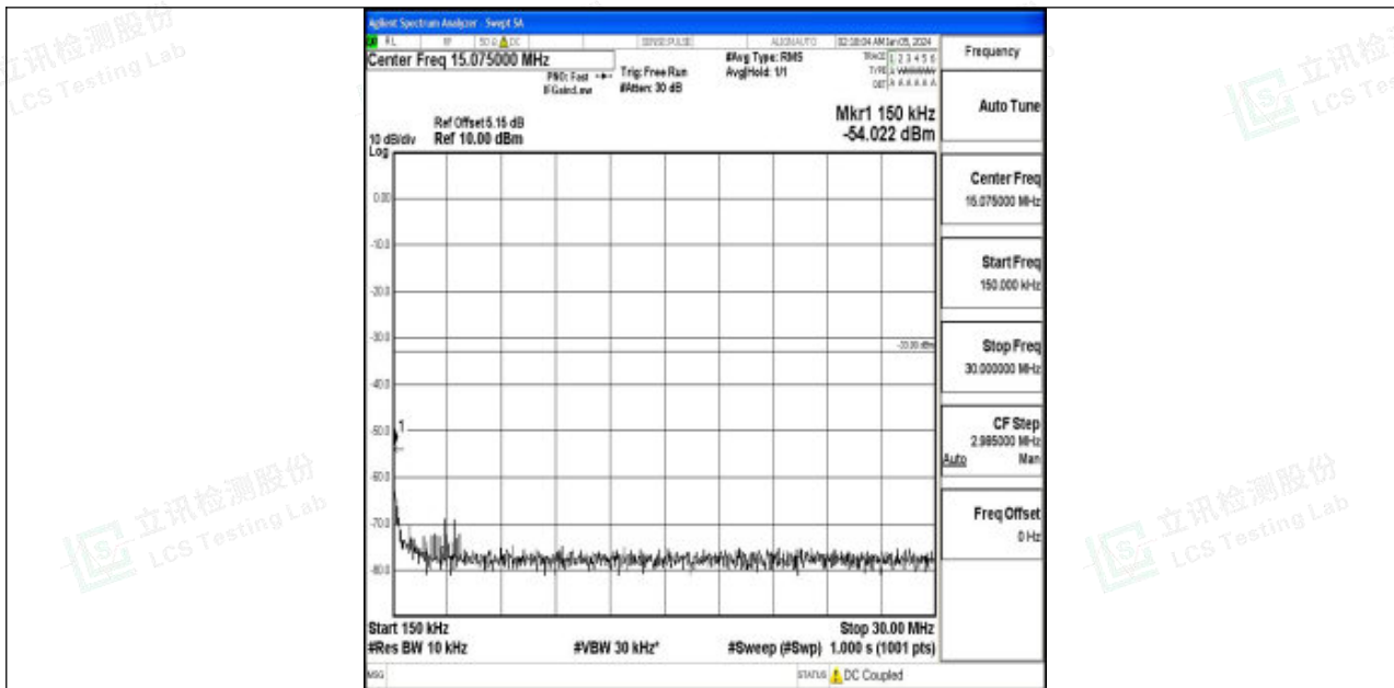
Band2_3MHz_QPSK_18615_1RB#0_0.15~30_0.15~30
