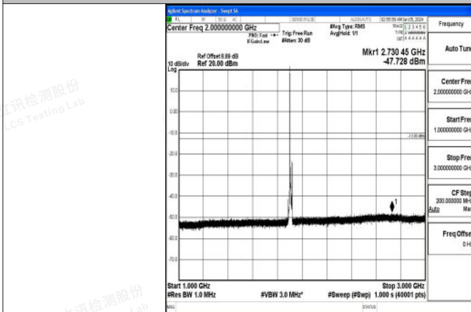
Band2_10MHz_16QAM_19150_1RB#0_1000~3000_1000~3000
