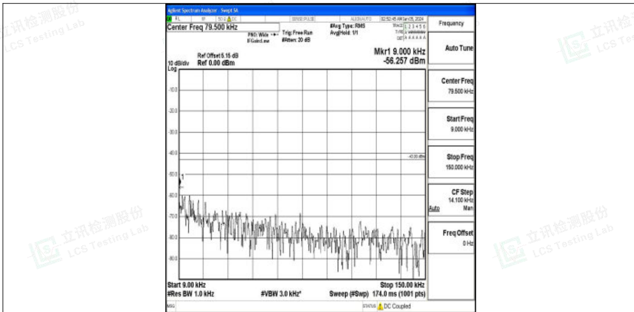
Band2_10MHz_16QAM_18650_1RB#0_0.009~0.15_0.009~0.15
