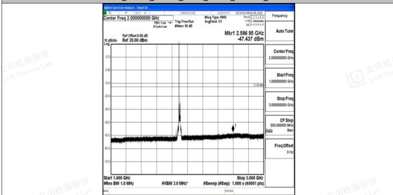
Band2_20MHz_16QAM_19100_1RB#0_1000~3000_1000~3000
