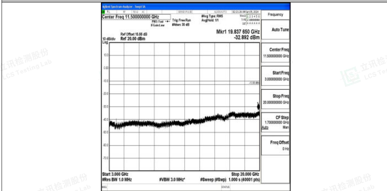
Band2_3MHz_QPSK_19185_1RB#0_3000~20000_3000~20000
