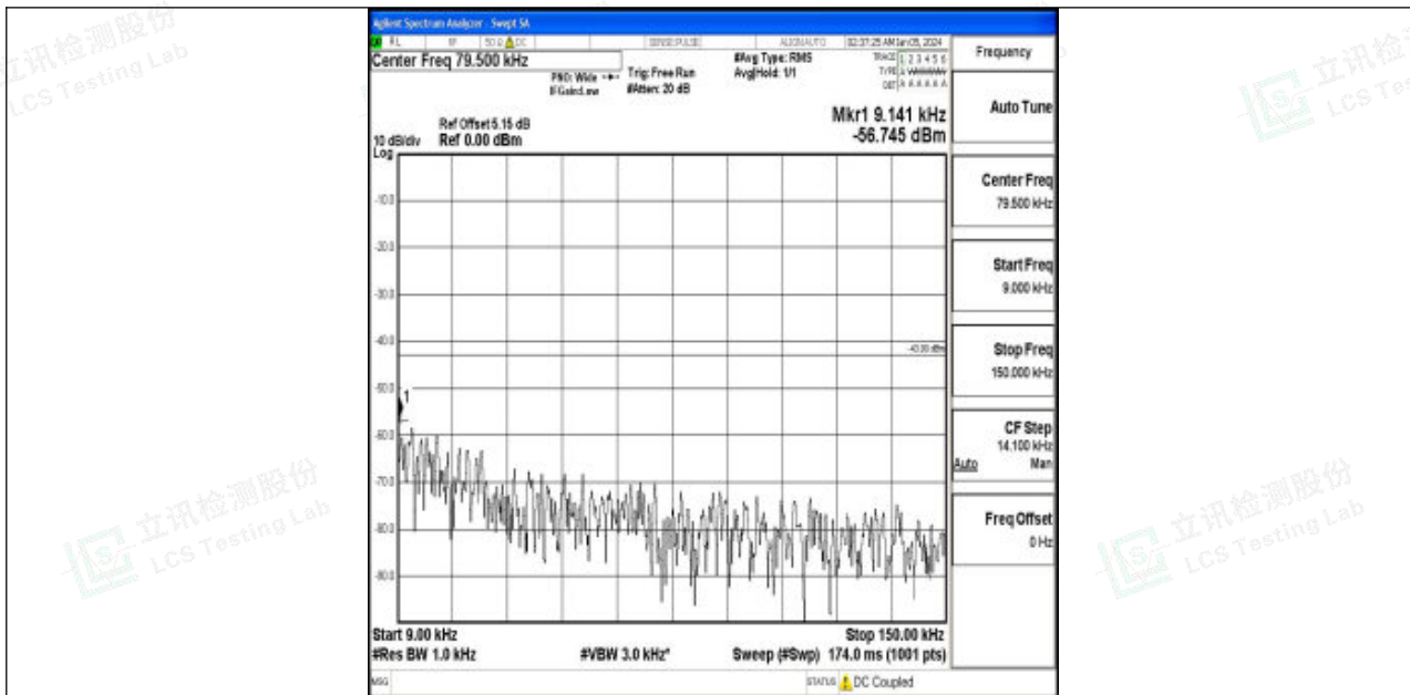
Band2_5MHz_16QAM_18900_1RB#0_0.009~0.15_0.009~0.15
