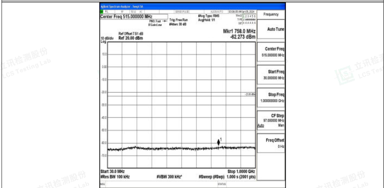
Band2_15MHz_QPSK_18675_1RB#0_30~1000_30~1000
