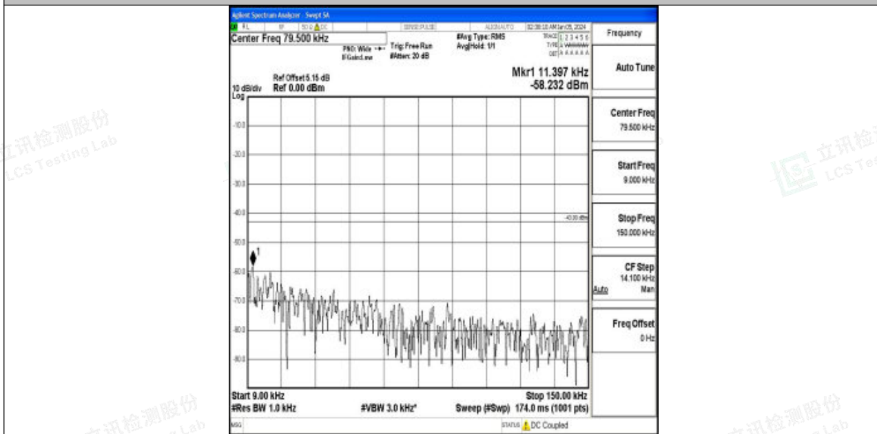
Band2_5MHz_QPSK_19175_1RB#0_0.009~0.15_0.009~0.15
