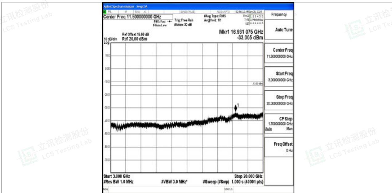
Band2_10MHz_16QAM_19150_1RB#0_3000~20000_3000~20000
