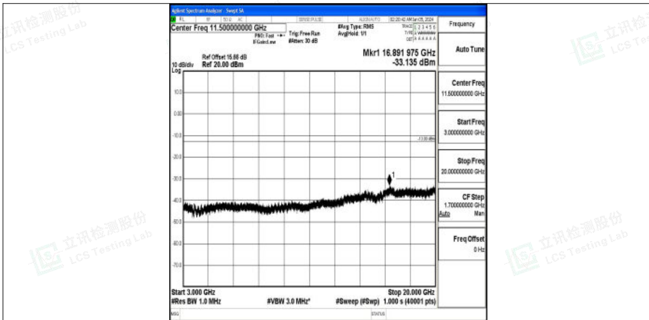
Band2_3MHz_16QAM_18900_1RB#0_3000~20000_3000~20000
