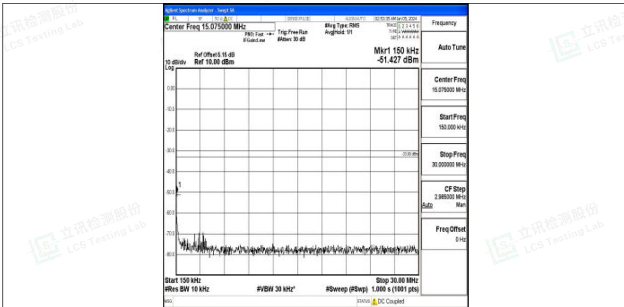
Band2_10MHz_QPSK_18900_1RB#0_0.15~30_0.15~30
