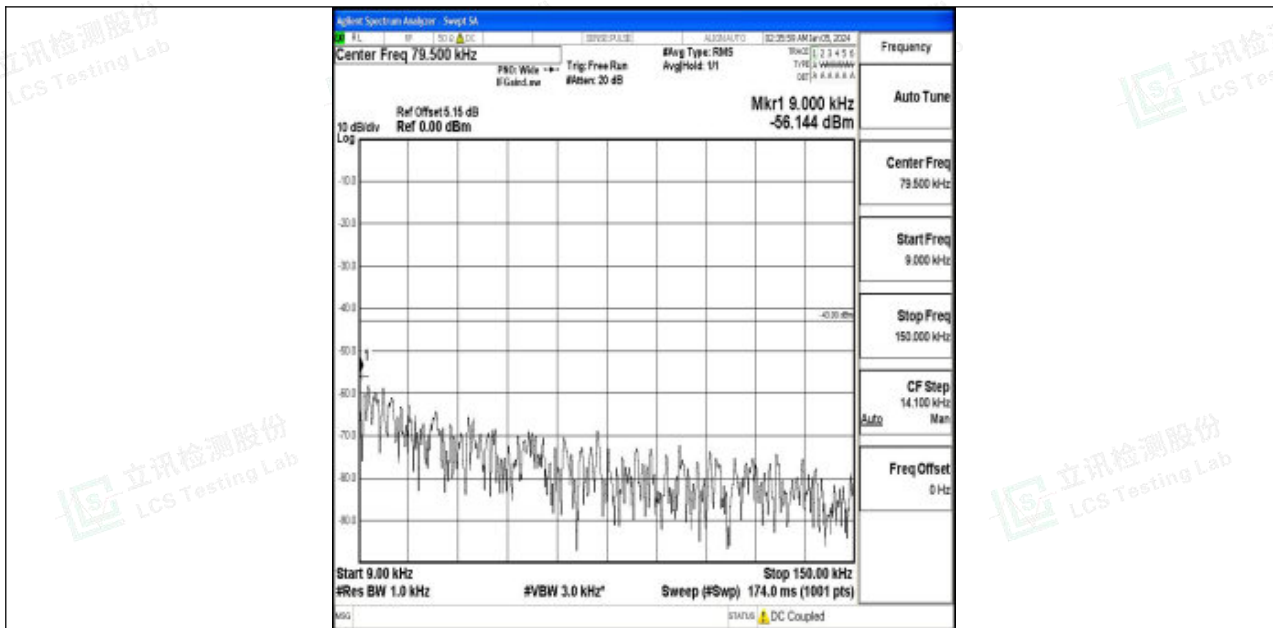
Band2_5MHz_16QAM_18625_1RB#0_0.009~0.15_0.009~0.15
