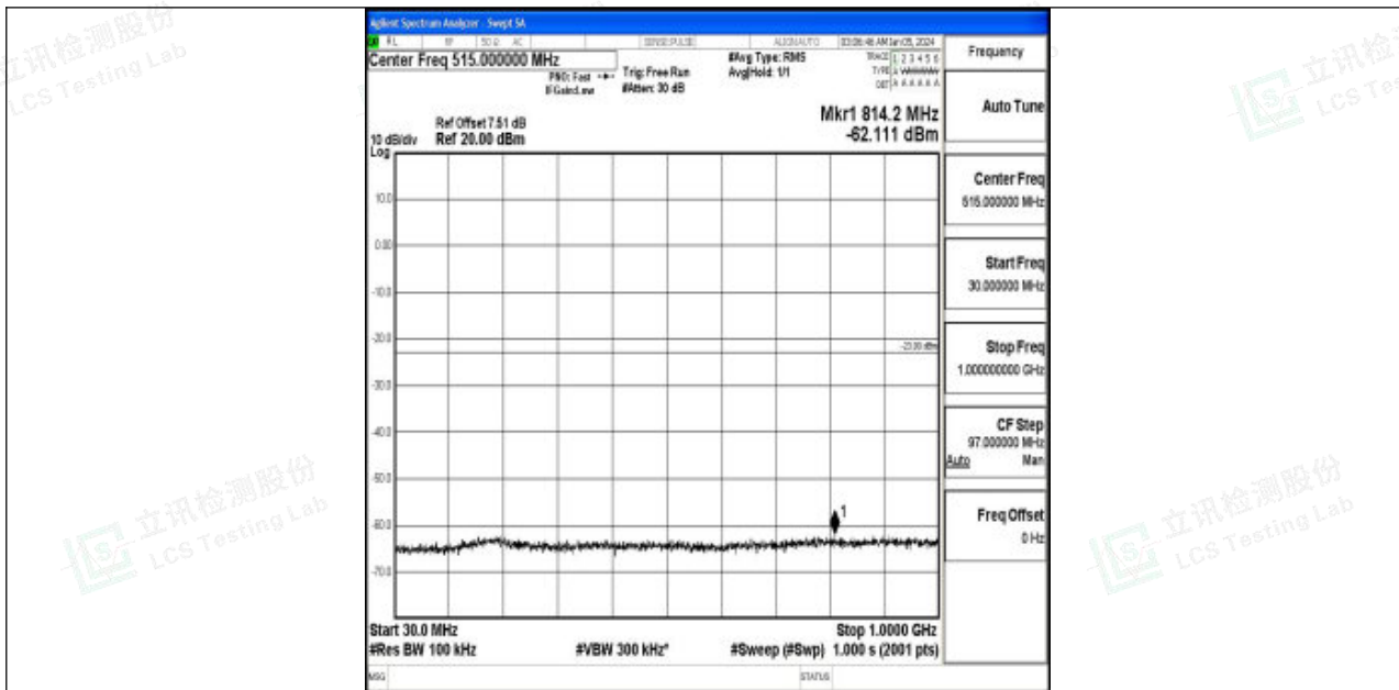
Band2_15MHz_16QAM_18675_1RB#0_30~1000_30~1000
