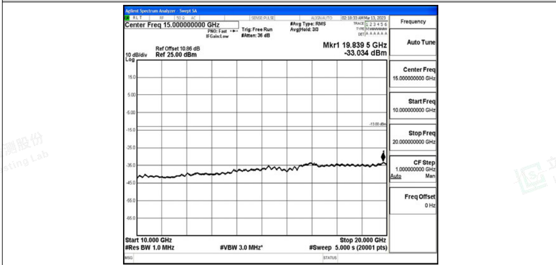
Band66-20MHz-16QAM-132572-1RB#0-Range5: 10000~20000MHz
