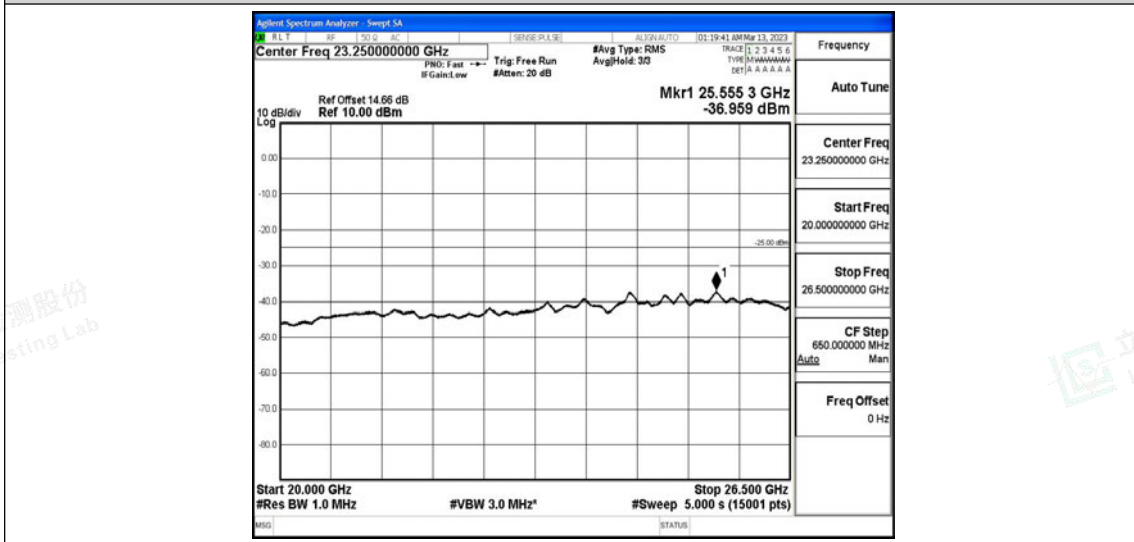
Band41-20MHz-16QAM-41490-1RB#0-Range6:20000~26500MHz
