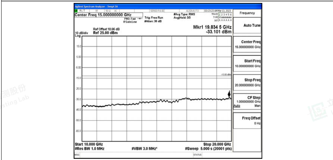
Band25-20MHz-16QAM-26590-1RB#0-Range5:10000~20000MHz
