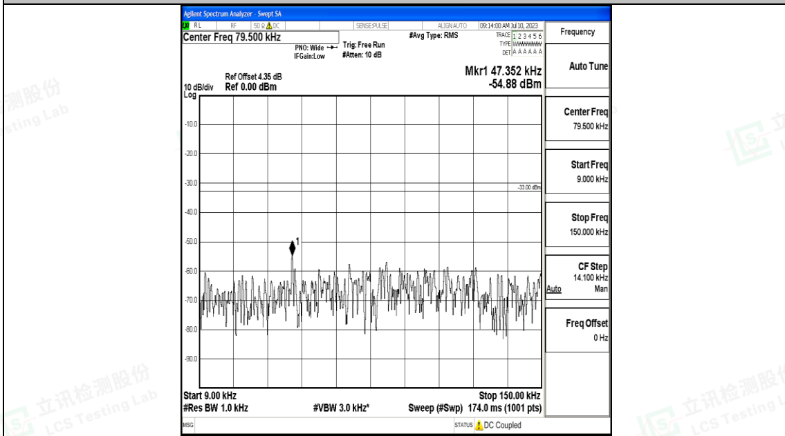
Band71_10MHz_QPSK_133172_1RB#0_0.009~0.15_0.009~0.15
