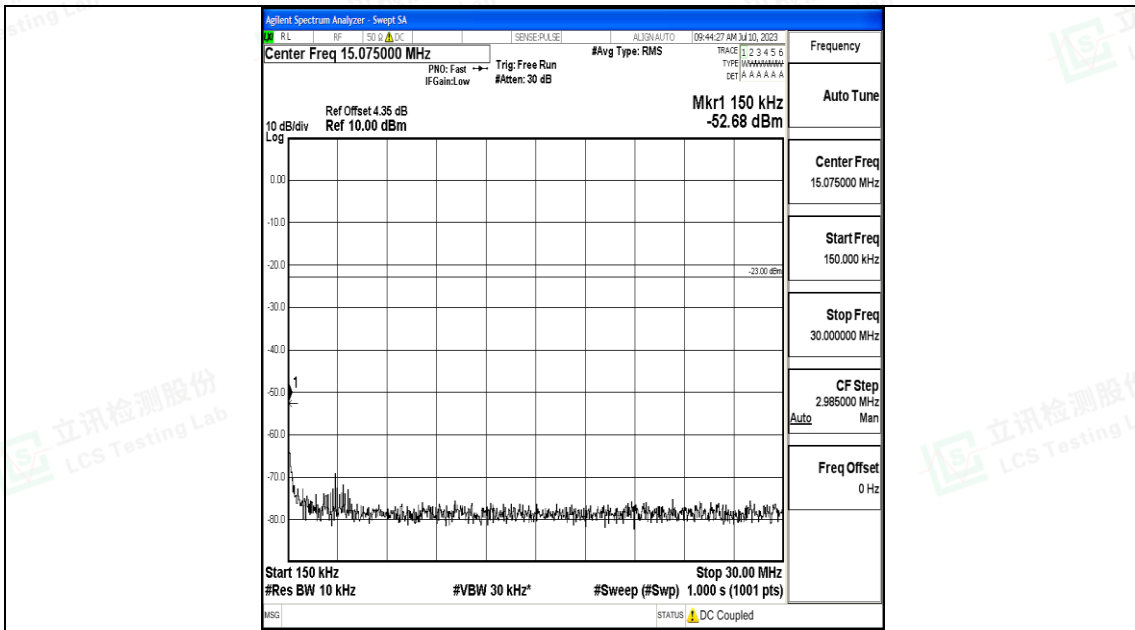
Band71_20MHz_QPSK_133322_1RB#0_0.15~30_0.15~30
