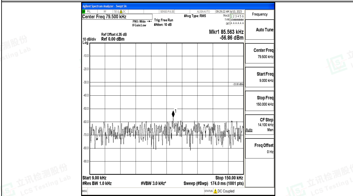
Band71_15MHz_QPSK_133197_1RB#0_0.009~0.15_0.009~0.15
