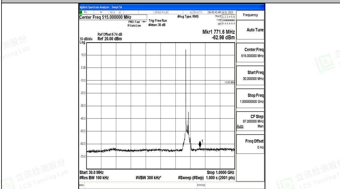
Band71_20MHz_QPSK_133372_1RB#0_30~1000_30~1000
