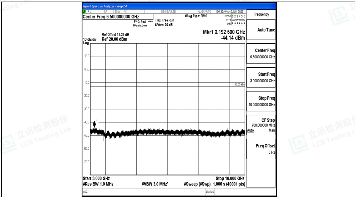
Band71_15MHz_16QAM_133397_1RB#0_3000~10000_3000~10000
