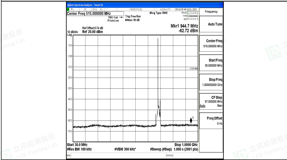
Band71_10MHz_QPSK_133422_1RB#0_30~1000_30~1000
