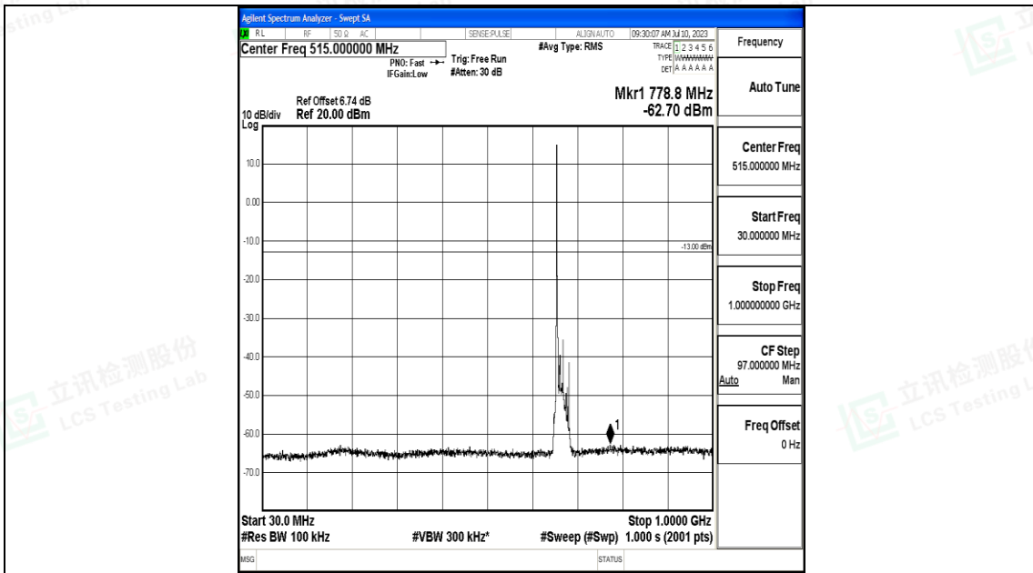
Band71_15MHz_16QAM_133197_1RB#0_30~1000_30~1000
