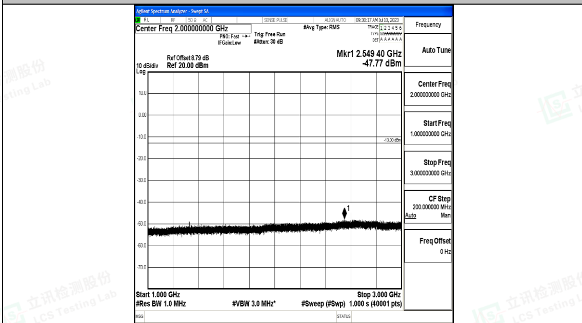
Band71_15MHz_16QAM_133197_1RB#0_1000~3000_1000~3000
