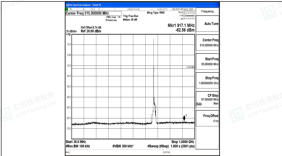
Band71_10MHz_16QAM_133297_1RB#0_30~1000_30~1000
