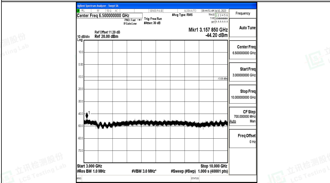
Band71_20MHz_QPSK_133322_1RB#0_3000~10000_3000~10000
