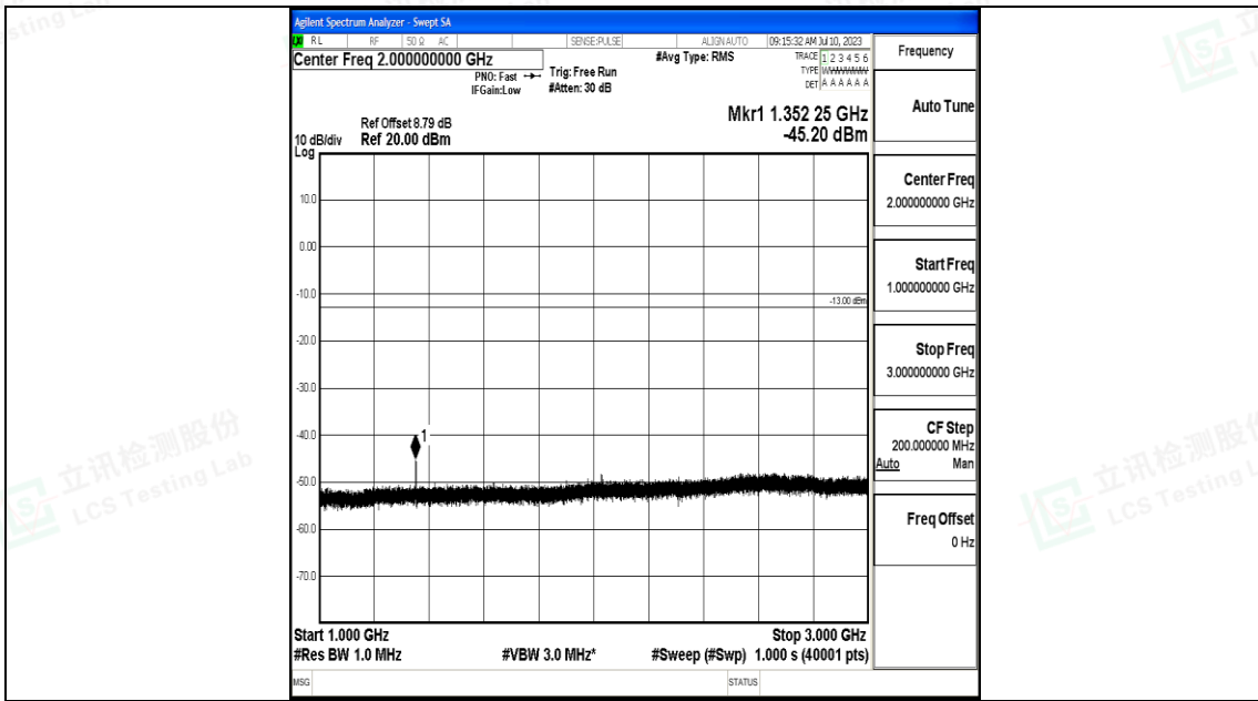
Band71_10MHz_QPSK_133297_1RB#0_1000~3000_1000~3000
