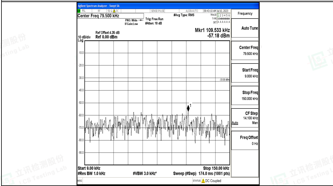
Band71_20MHz_QPSK_133222_1RB#0_0.009~0.15_0.009~0.15
