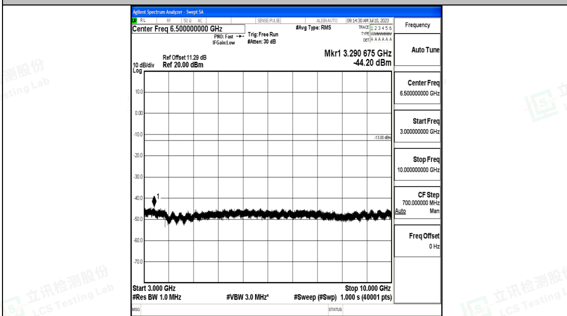
Band71_10MHz_QPSK_133172_1RB#0_3000~10000_3000~10000
