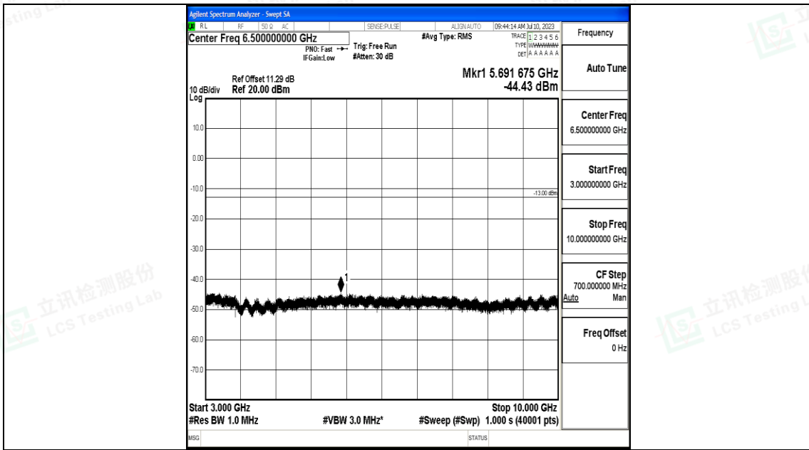
Band71_20MHz_16QAM_133222_1RB#0_3000~10000_3000~10000
