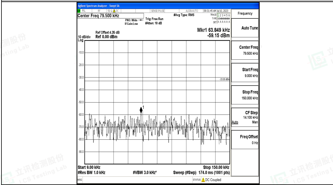
Band71_15MHz_QPSK_133397_1RB#0_0.009~0.15_0.009~0.15
