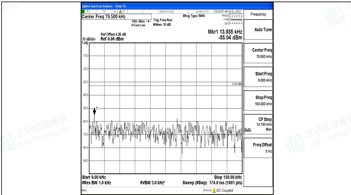
Band71_15MHz_16QAM_133197_1RB#0_0.009~0.15_0.009~0.15
