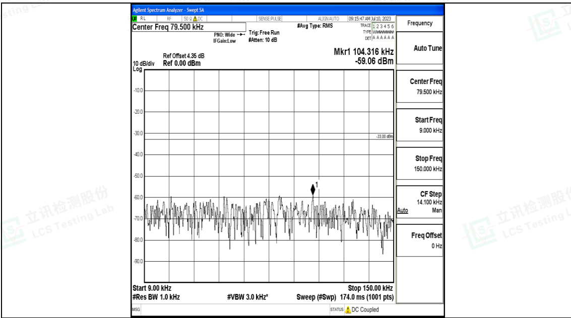
Band71_10MHz_16QAM_133297_1RB#0_0.009~0.15_0.009~0.15
