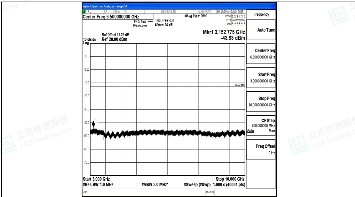
Band71_10MHz_16QAM_133422_1RB#0_3000~10000_3000~10000
