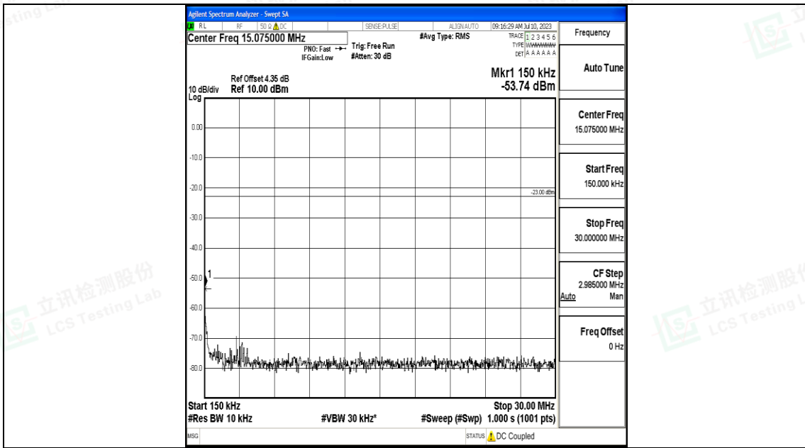
Band71_10MHz_QPSK_133422_1RB#0_0.15~30_0.15~30
