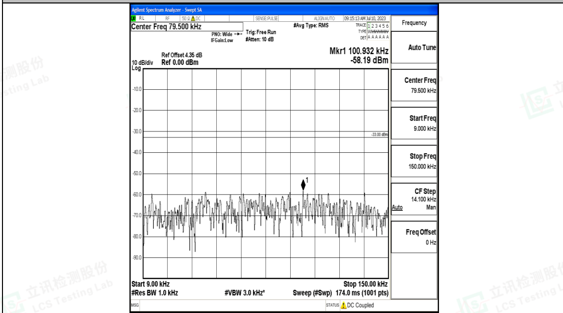
Band71_10MHz_QPSK_133297_1RB#0_0.009~0.15_0.009~0.15
