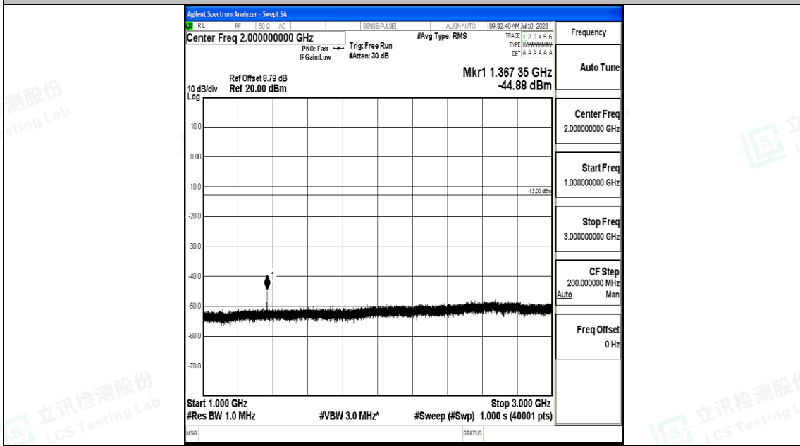
Band71_15MHz_16QAM_133397_1RB#0_1000~3000_1000~3000
