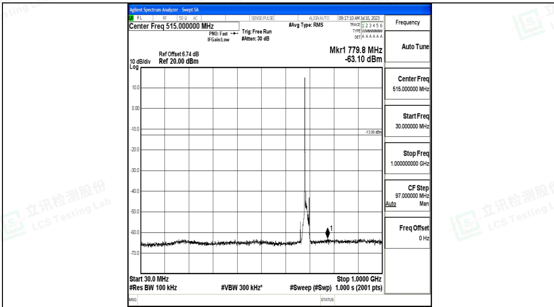
Band71_10MHz_16QAM_133422_1RB#0_30~1000_30~1000
