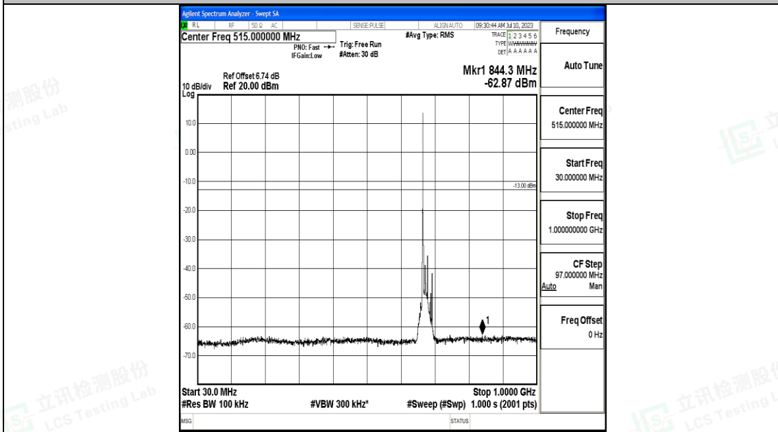
Band71_15MHz_QPSK_133297_1RB#0_30~1000_30~1000
