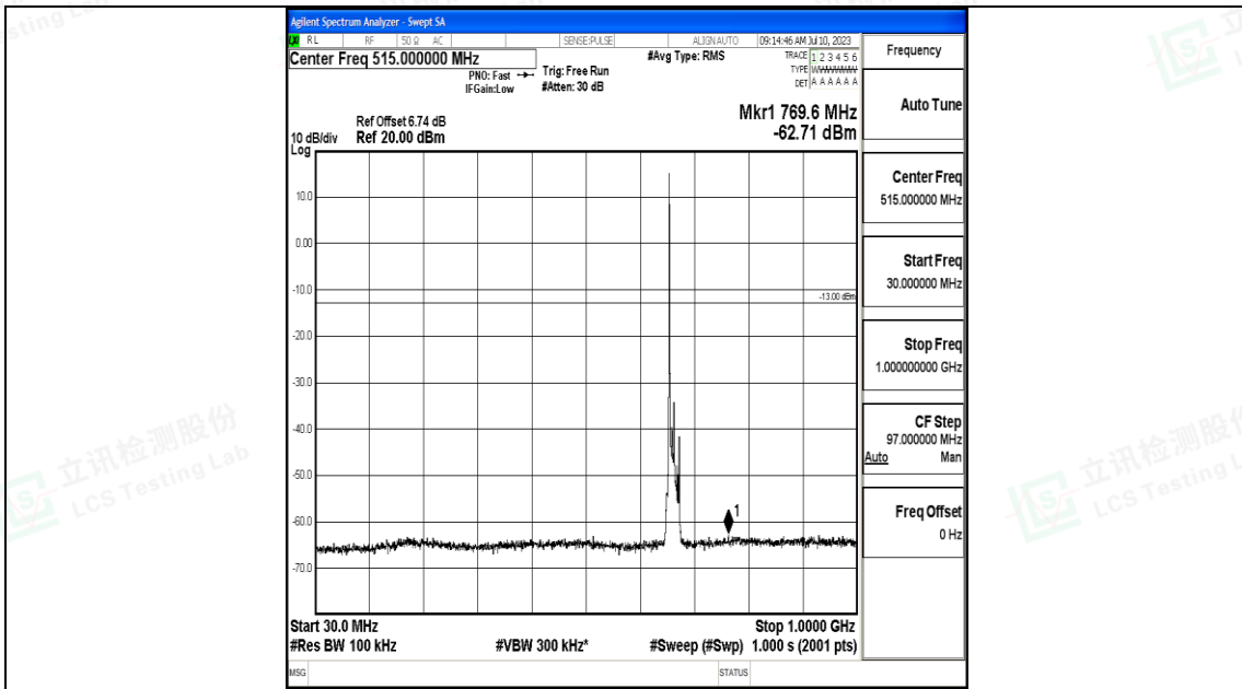
Band71_10MHz_16QAM_133172_1RB#0_30~1000_30~1000
