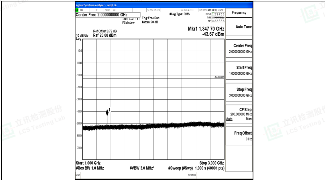
Band71_15MHz_QPSK_133297_1RB#0_1000~3000_1000~3000
