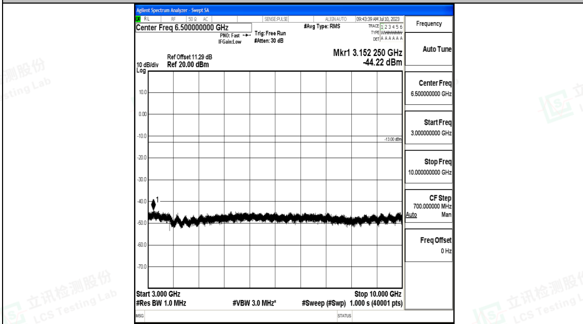
Band71_20MHz_QPSK_133222_1RB#0_3000~10000_3000~10000
