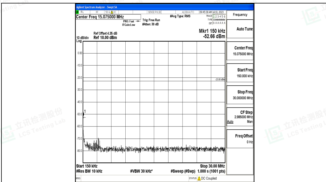
Band71_20MHz_QPSK_133372_1RB#0_0.15~30_0.15~30
