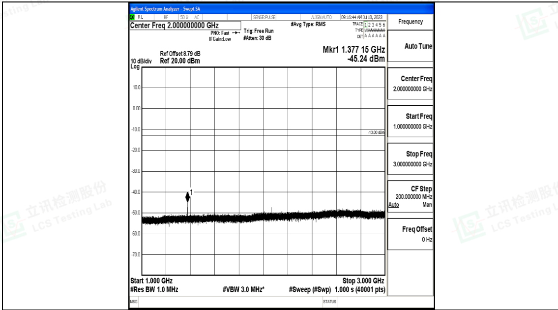
Band71_10MHz_QPSK_133422_1RB#0_1000~3000_1000~3000
