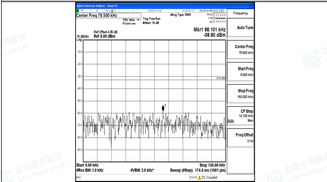
Band71_15MHz_QPSK_133297_1RB#0_0.009~0.15_0.009~0.15
