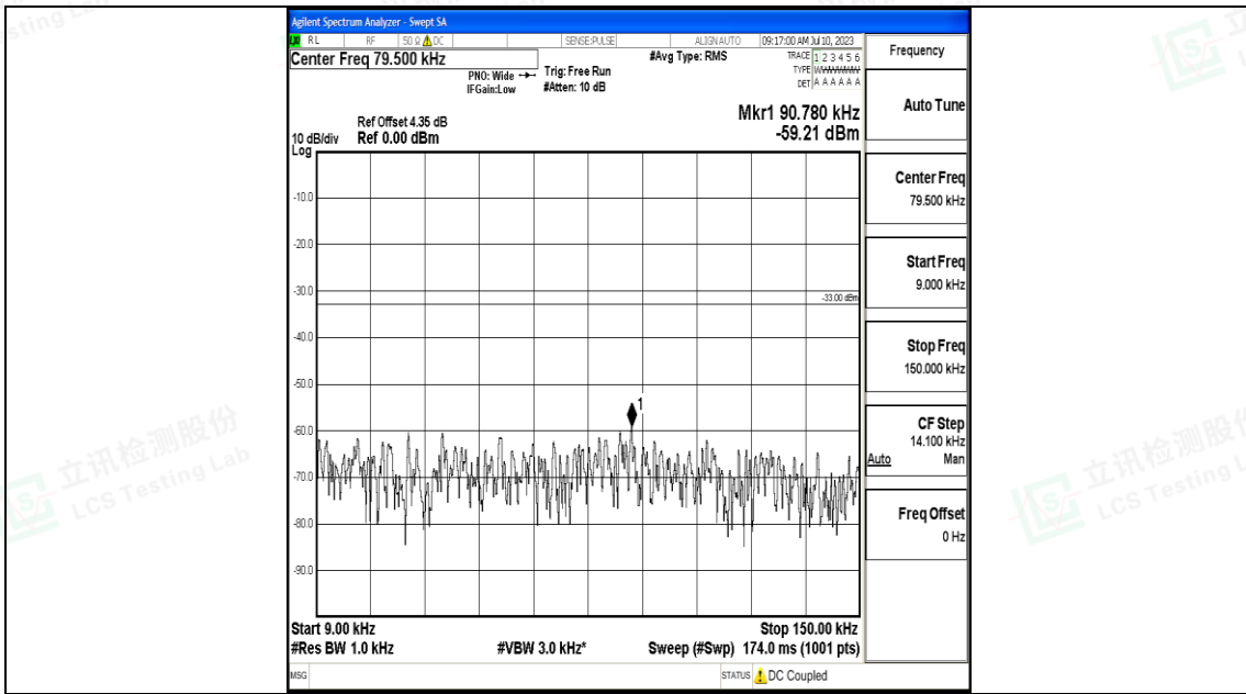
Band71_10MHz_16QAM_133422_1RB#0_0.009~0.15_0.009~0.15
