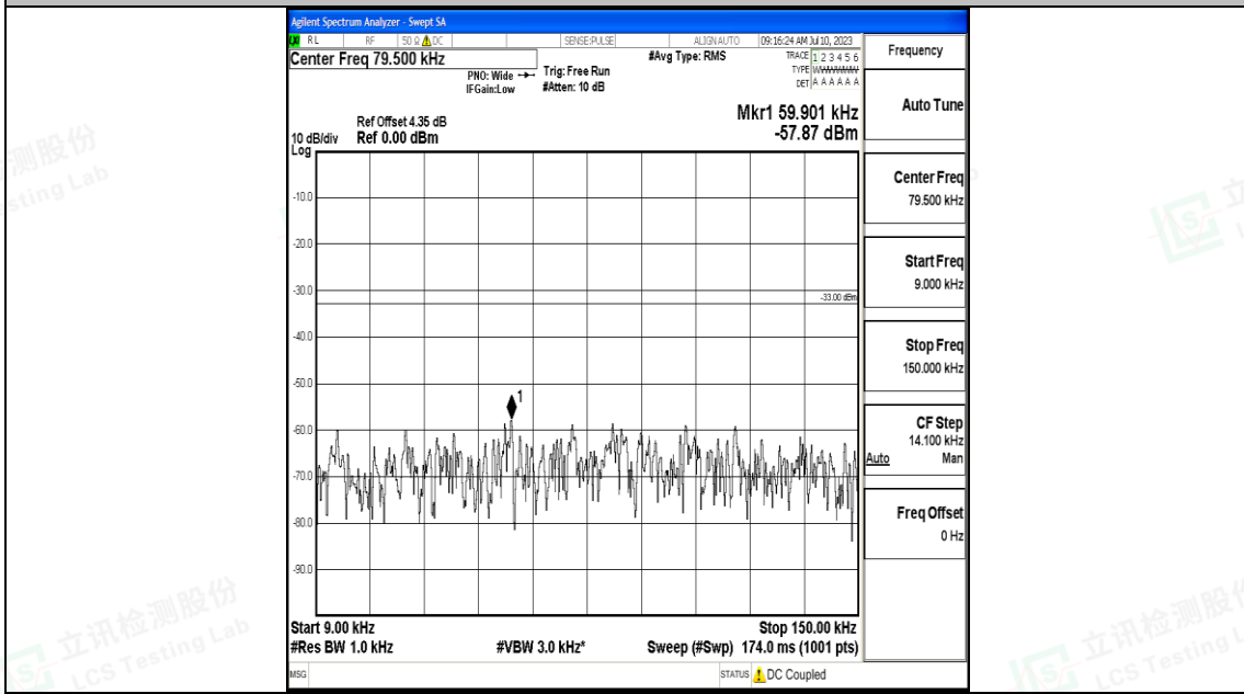
Band71_10MHz_QPSK_133422_1RB#0_0.009~0.15_0.009~0.15
