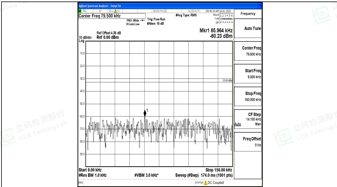
Band71_20MHz_16QAM_133372_1RB#0_0.009~0.15_0.009~0.15
