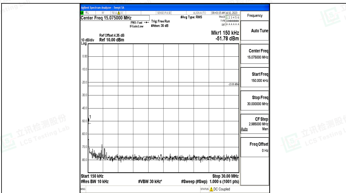
Band71_20MHz_QPSK_133222_1RB#0_0.15~30_0.15~30
