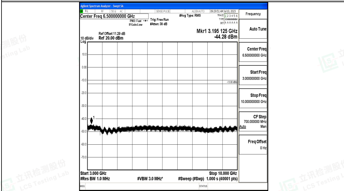
Band71_15MHz_QPSK_133197_1RB#0_3000~10000_3000~10000
