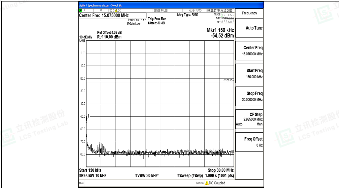
Band71_15MHz_QPSK_133197_1RB#0_0.15~30_0.15~30
