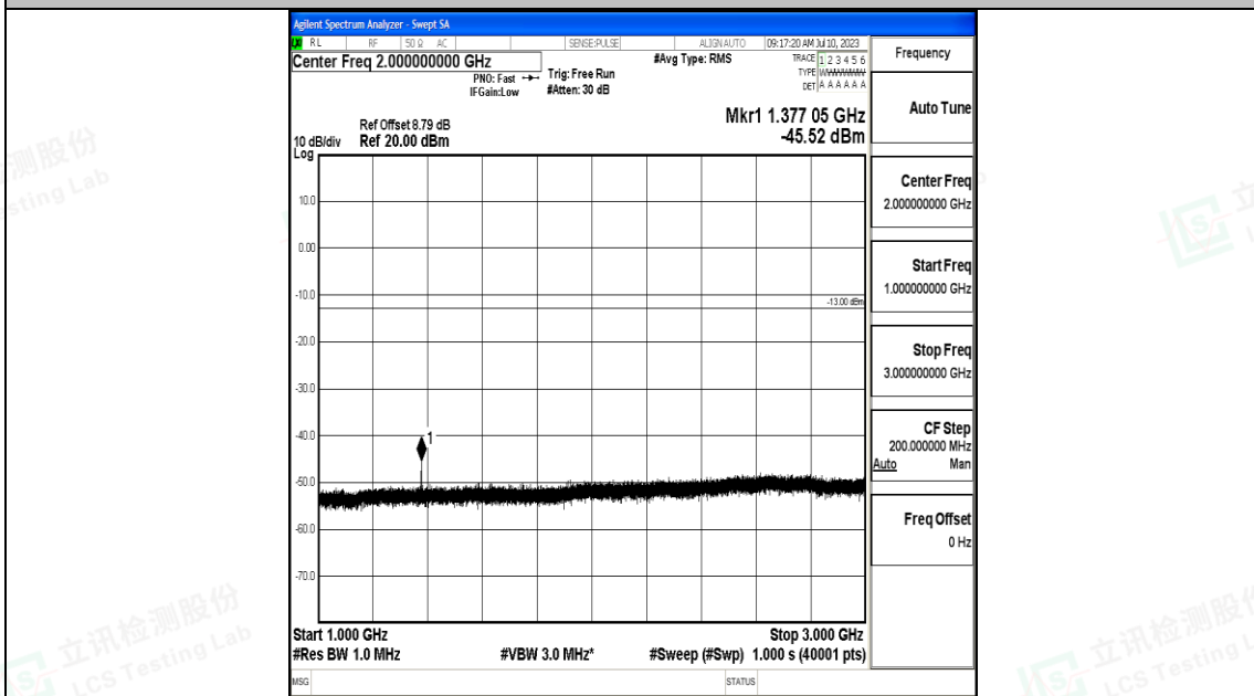
Band71_10MHz_16QAM_133422_1RB#0_1000~3000_1000~3000
