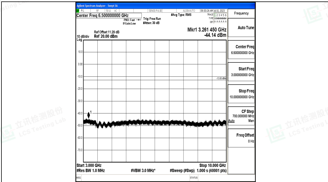
Band71_15MHz_16QAM_133197_1RB#0_3000~10000_3000~10000
