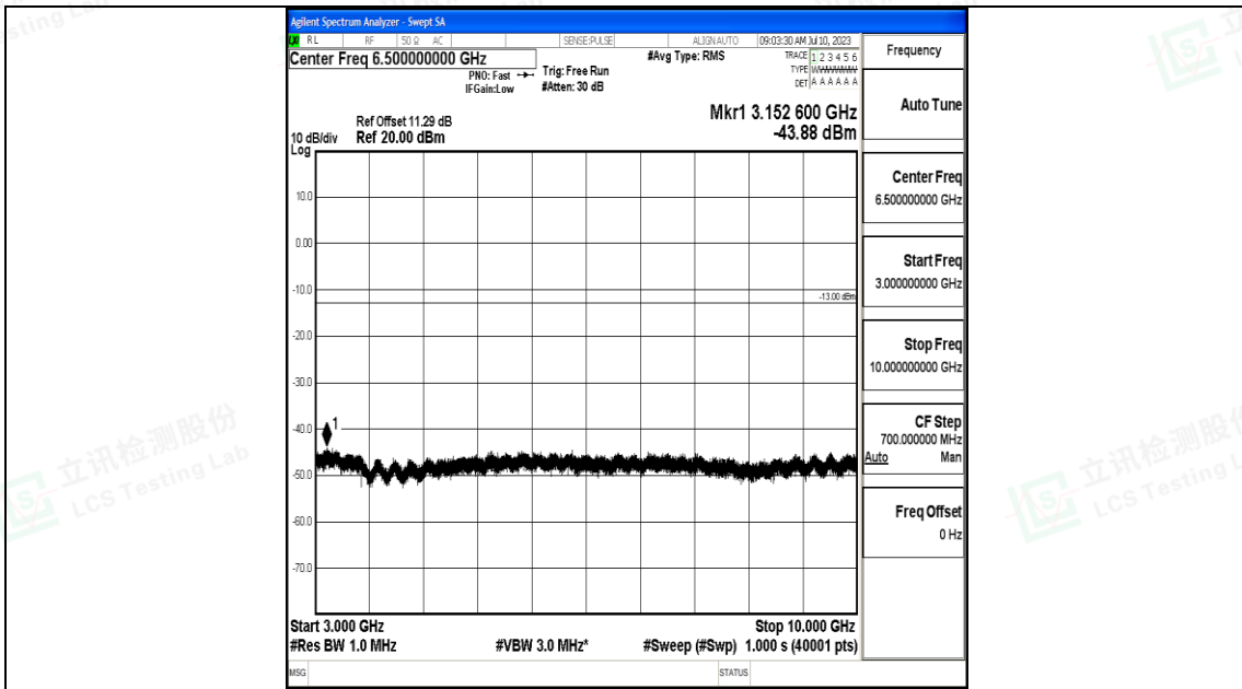
Band71_5MHz_16QAM_133447_1RB#0_3000~10000_3000~10000
