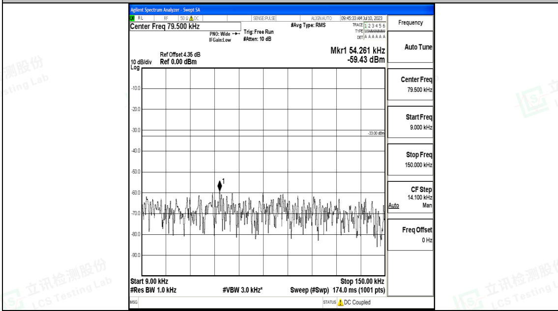
Band71_20MHz_QPSK_133372_1RB#0_0.009~0.15_0.009~0.15
