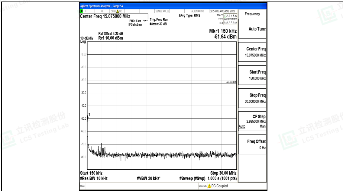
Band71_10MHz_QPSK_133172_1RB#0_0.15~30_0.15~30
