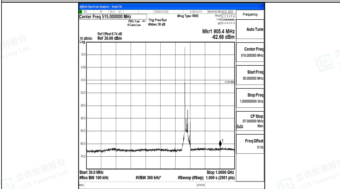
Band71_20MHz_QPSK_133322_1RB#0_30~1000_30~1000
