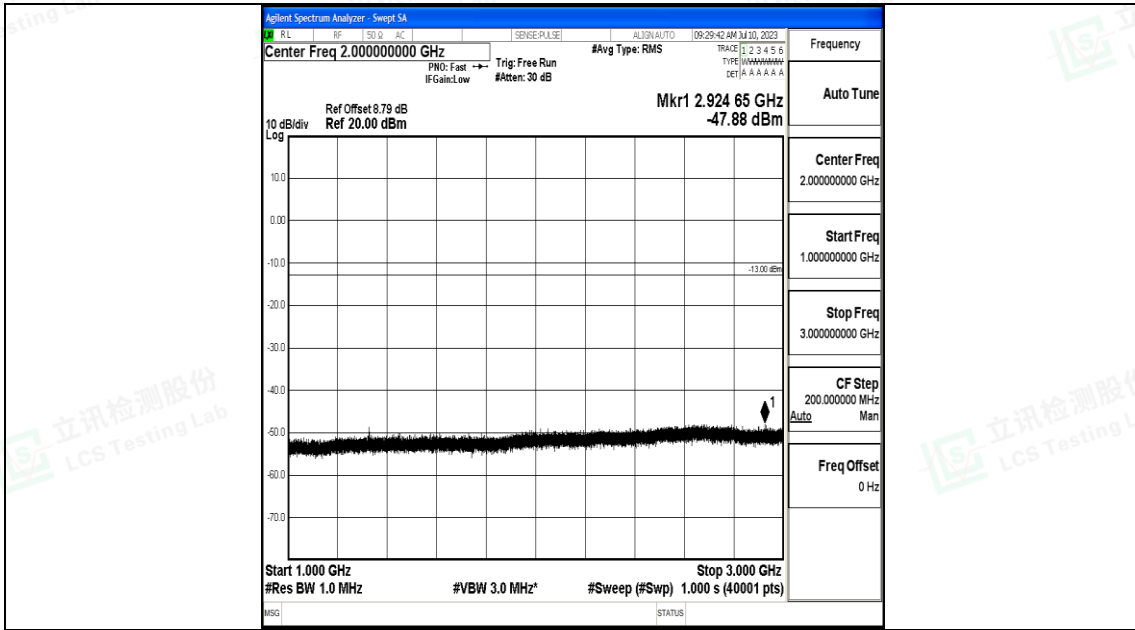
Band71_15MHz_QPSK_133197_1RB#0_1000~3000_1000~3000
