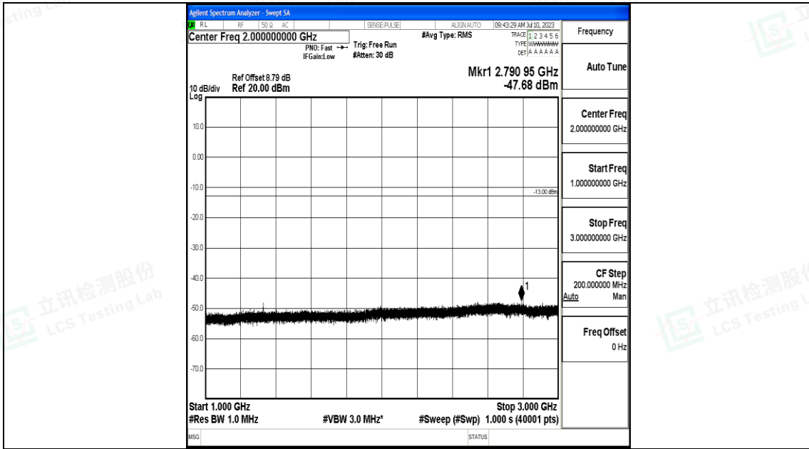
Band71_20MHz_QPSK_133222_1RB#0_1000~3000_1000~3000
