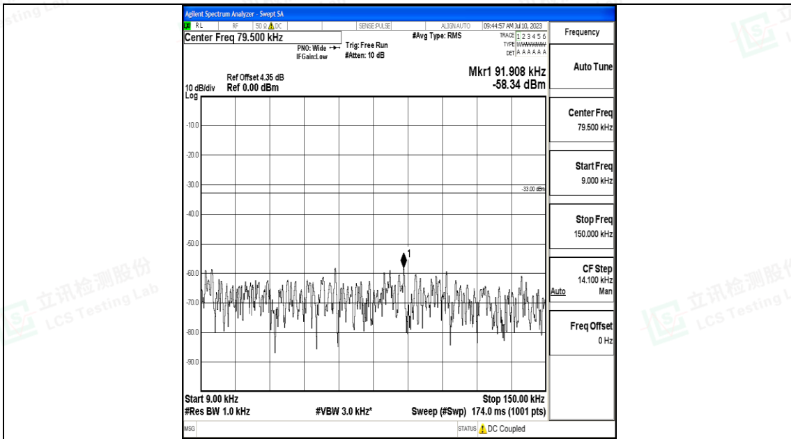
Band71_20MHz_16QAM_133322_1RB#0_0.009~0.15_0.009~0.15
