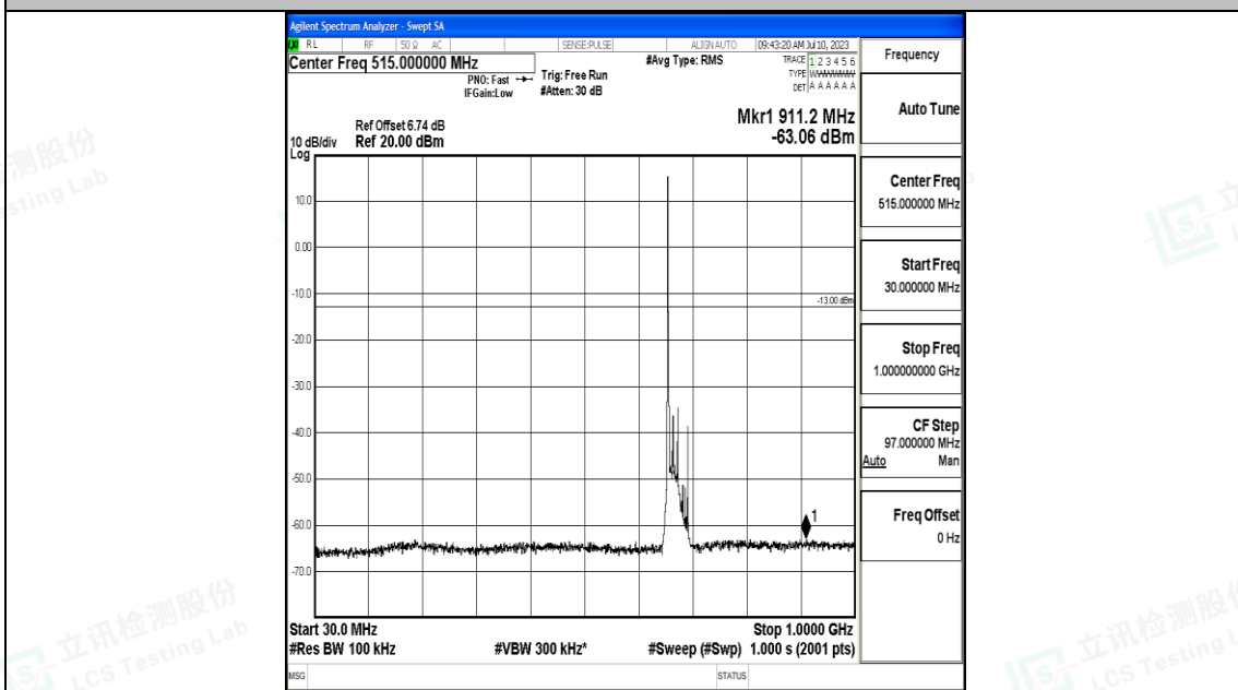
Band71_20MHz_QPSK_133222_1RB#0_30~1000_30~1000
