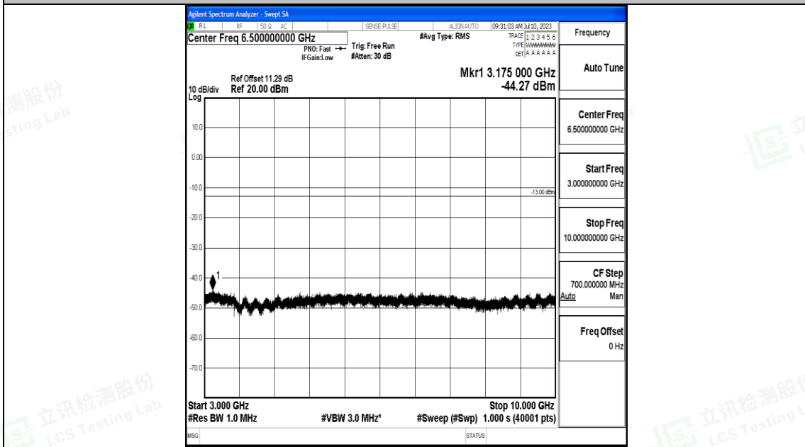
Band71_15MHz_QPSK_133297_1RB#0_3000~10000_3000~10000
