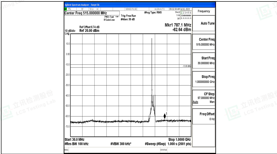
Band71_15MHz_16QAM_133397_1RB#0_30~1000_30~1000
