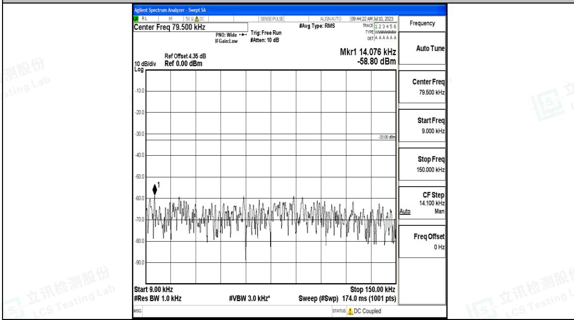
Band71_20MHz_QPSK_133322_1RB#0_0.009~0.15_0.009~0.15
