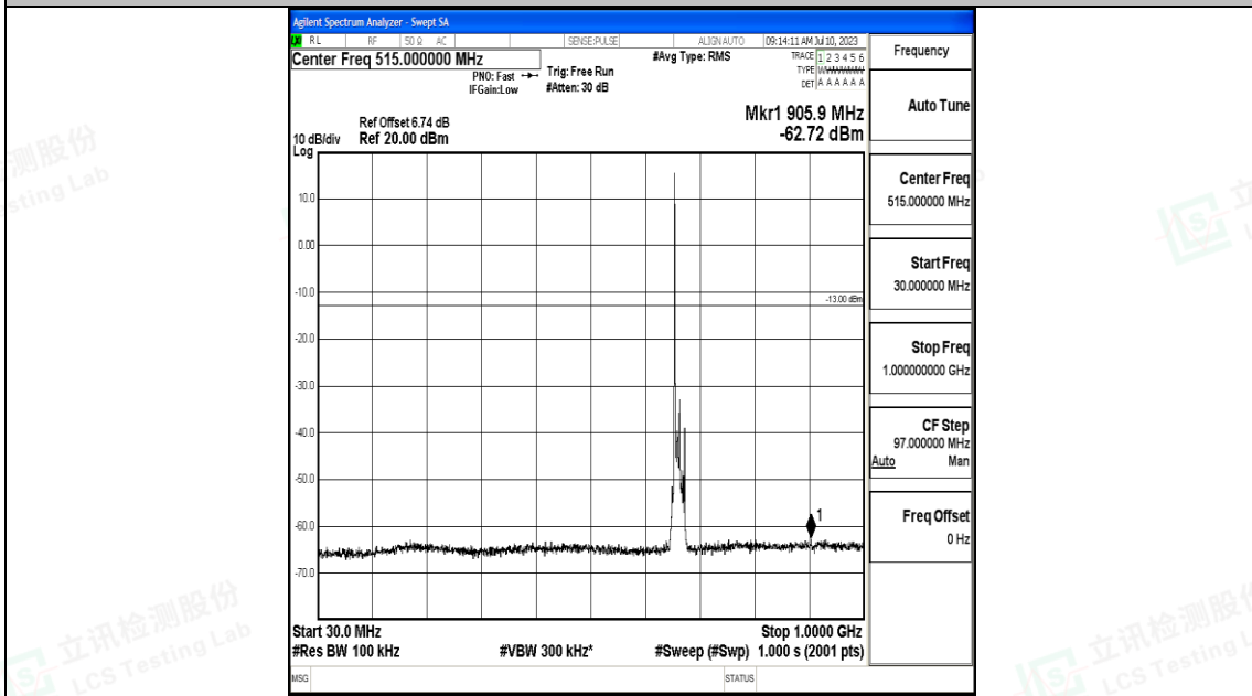
Band71_10MHz_QPSK_133172_1RB#0_30~1000_30~1000
