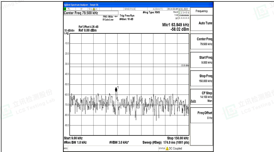
Band71_10MHz_16QAM_133172_1RB#0_0.009~0.15_0.009~0.15
