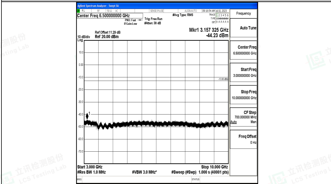
Band71_10MHz_QPSK_133422_1RB#0_3000~10000_3000~10000
