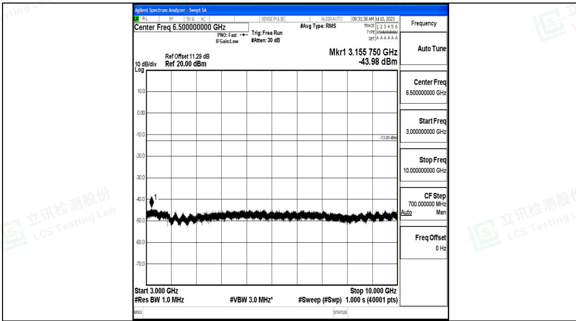
Band71_15MHz_16QAM_133297_1RB#0_3000~10000_3000~10000
