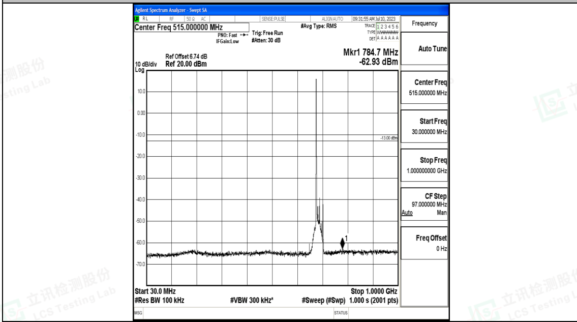
Band71_15MHz_QPSK_133397_1RB#0_30~1000_30~1000
