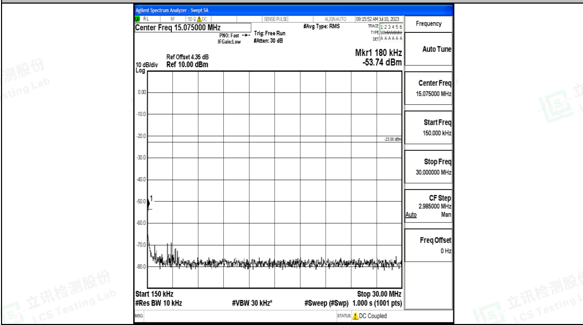
Band71_10MHz_16QAM_133297_1RB#0_0.15~30_0.15~30
