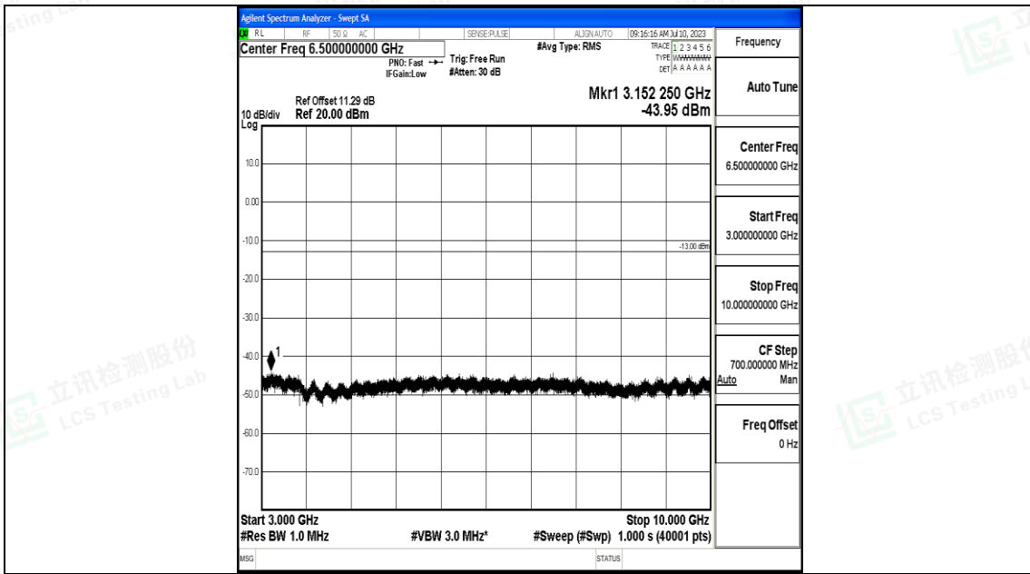
Band71_10MHz_16QAM_133297_1RB#0_3000~10000_3000~10000
