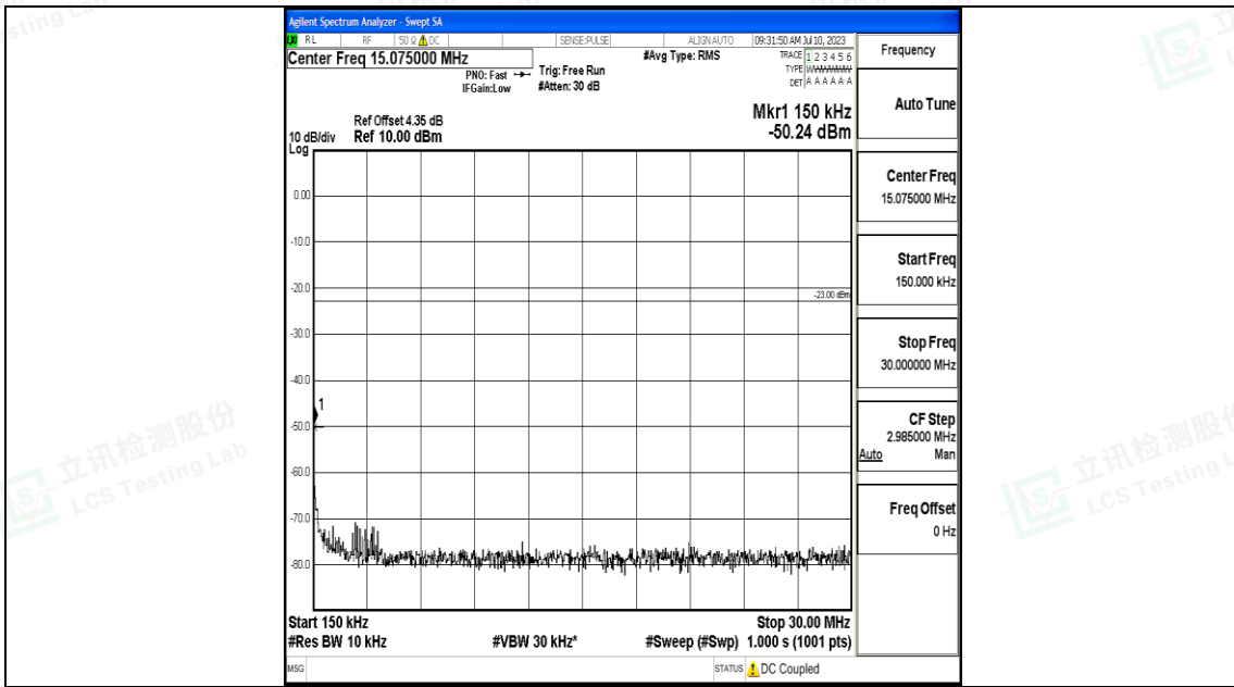
Band71_15MHz_QPSK_133397_1RB#0_0.15~30_0.15~30
