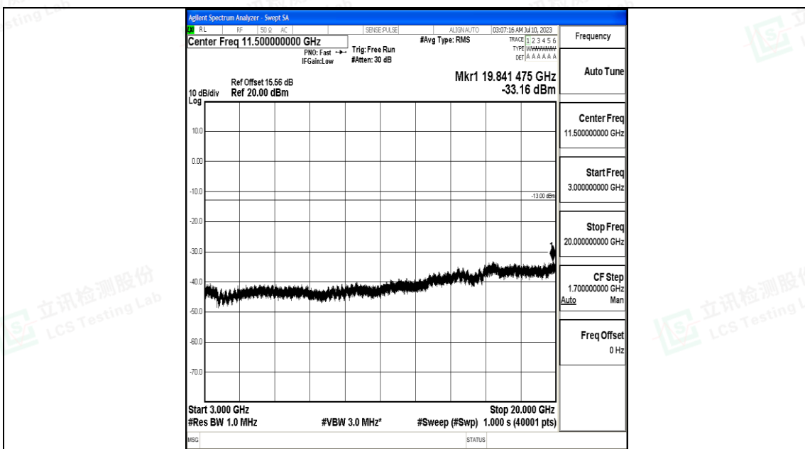
Band66_10MHz_QPSK_132022_1RB#0_3000~20000_3000~20000
