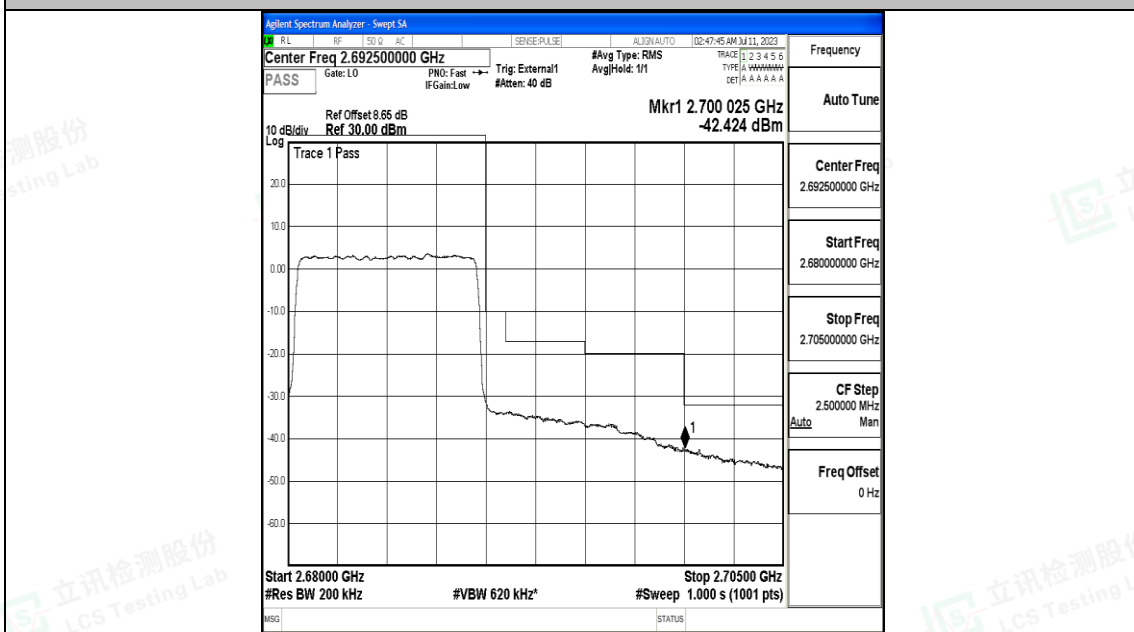
Band41_10MHz_16QAM_41540_50RB#0
