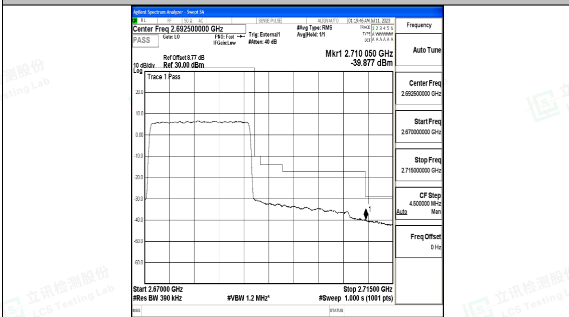
Band41_20MHz_16QAM_41490_100RB#0
