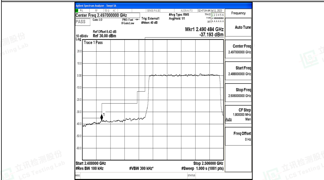
Band41_10MHz_16QAM_39700_50RB#0
