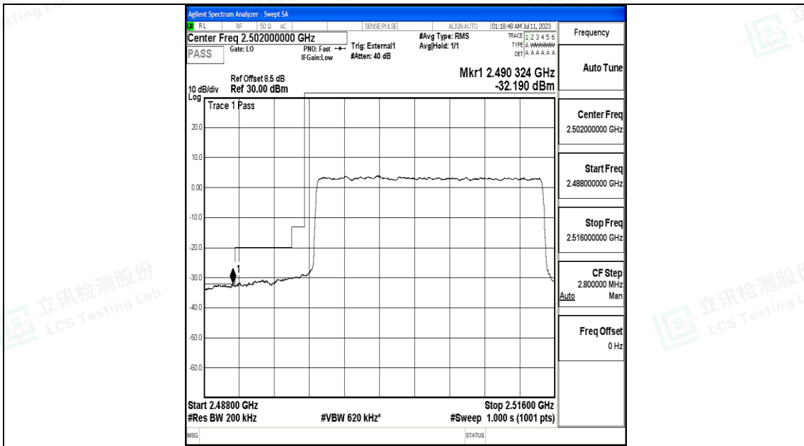
Band41_20MHz_QPSK_39750_100RB#0
