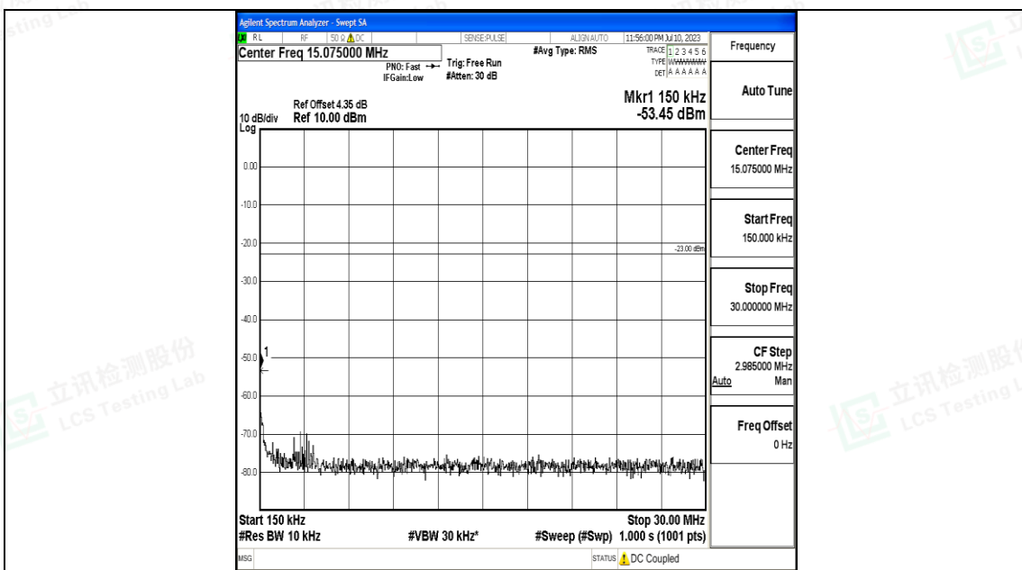
Band26_15MHz_16QAM_26865_1RB#0_0.15~30_0.15~30
