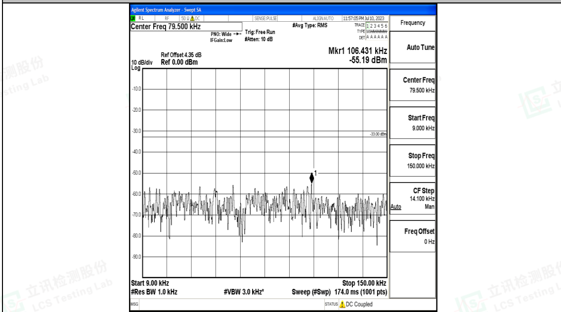
Band26_15MHz_16QAM_26915_1RB#0_0.009~0.15_0.009~0.15
