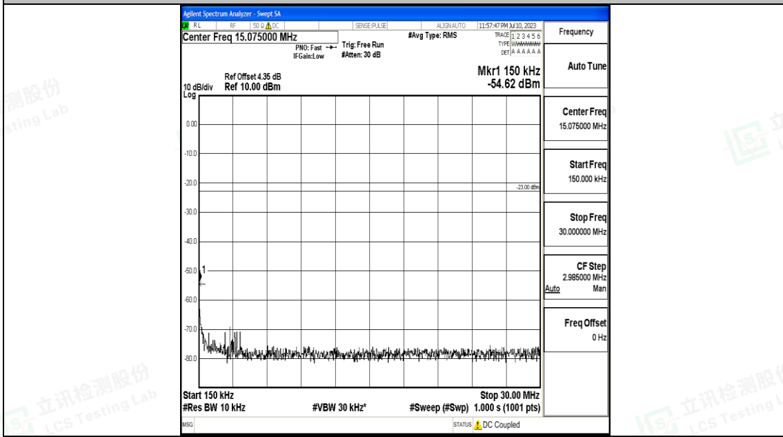
Band26_15MHz_QPSK_26965_1RB#0_0.15~30_0.15~30
