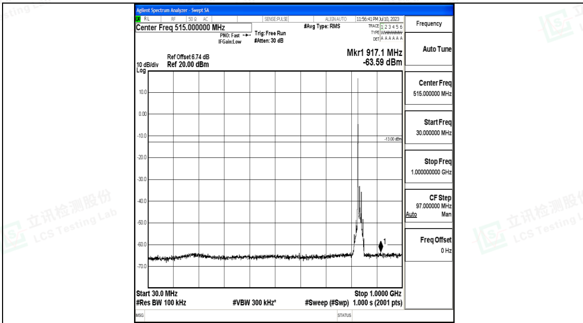
Band26_15MHz_QPSK_26915_1RB#0_30~1000_30~1000
