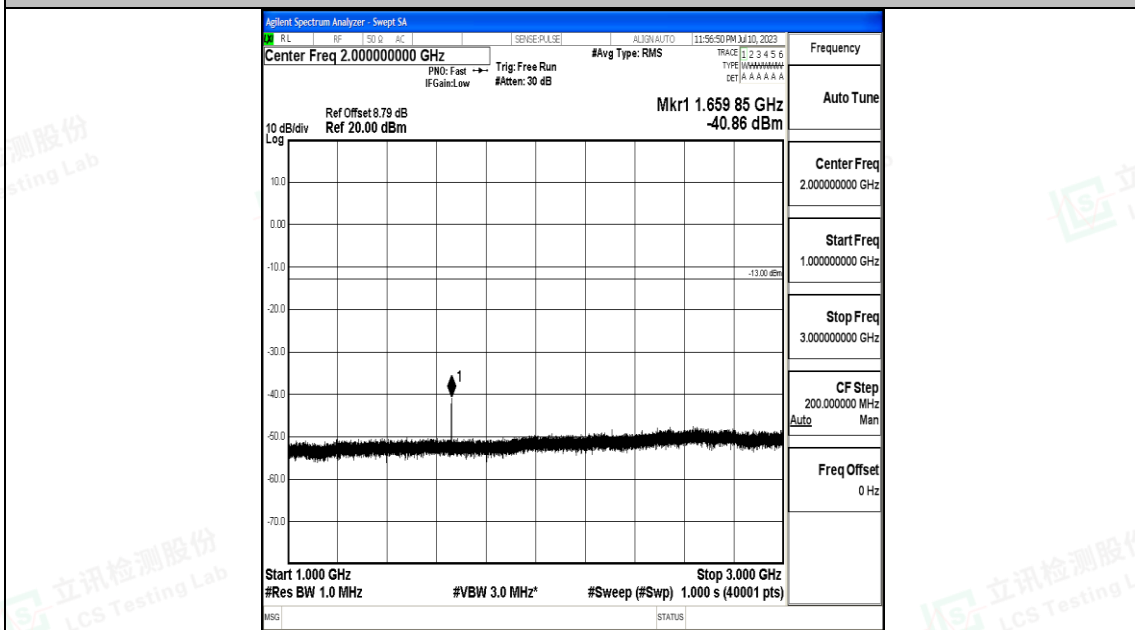
Band26_15MHz_QPSK_26915_1RB#0_1000~3000_1000~3000
