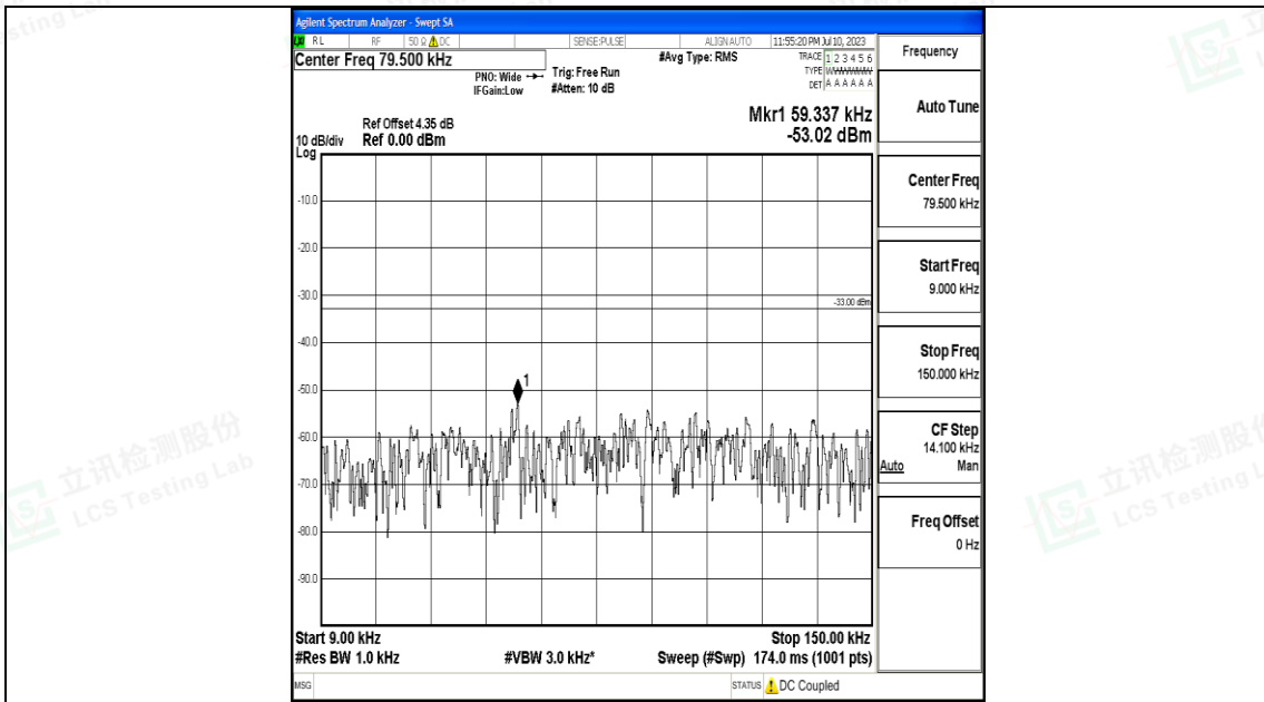
Band26_15MHz_QPSK_26865_1RB#0_0.009~0.15_0.009~0.15
