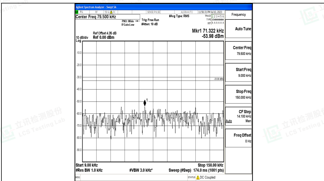
Band26_15MHz_QPSK_26915_1RB#0_0.009~0.15_0.009~0.15
