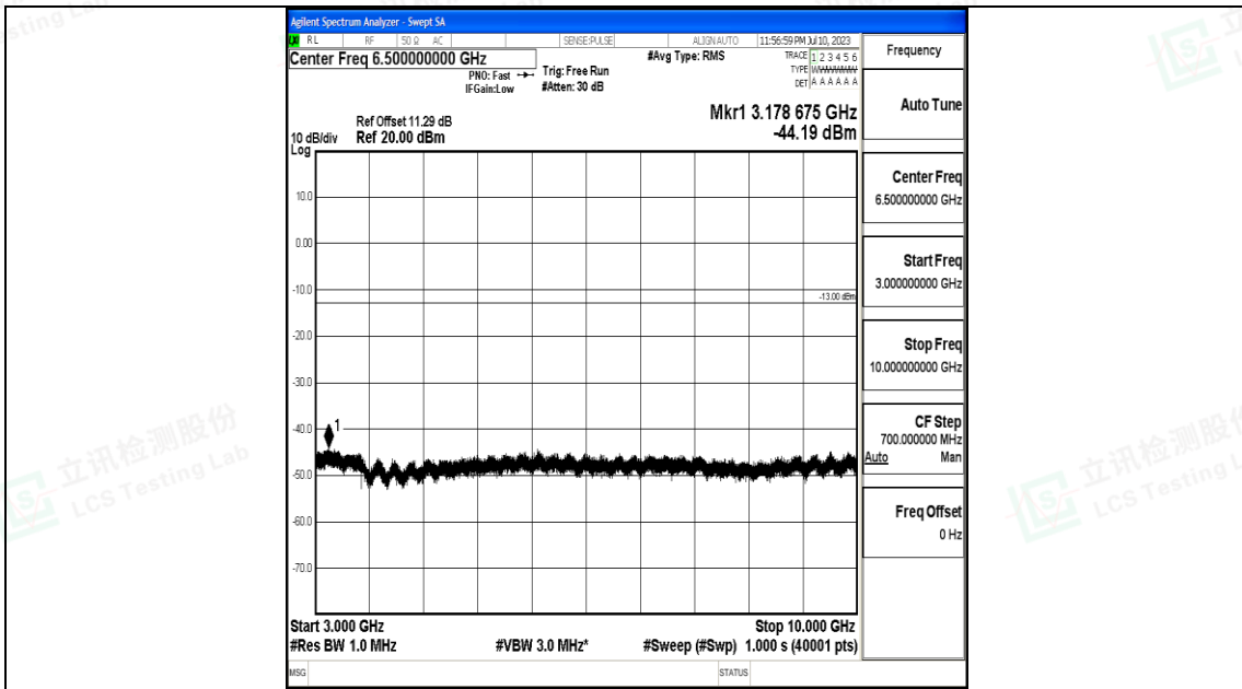
Band26_15MHz_QPSK_26915_1RB#0_3000~10000_3000~10000
