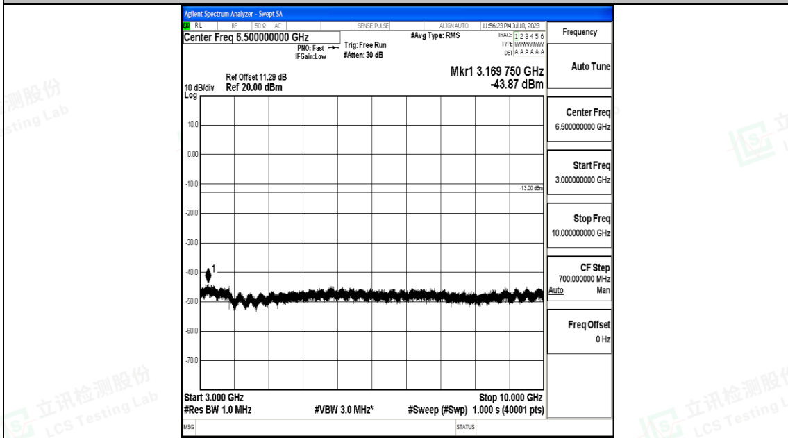
Band26_15MHz_16QAM_26865_1RB#0_3000~10000_3000~10000
