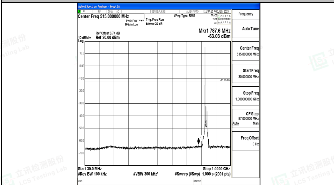
Band26_15MHz_16QAM_26915_1RB#0_30~1000_30~1000
