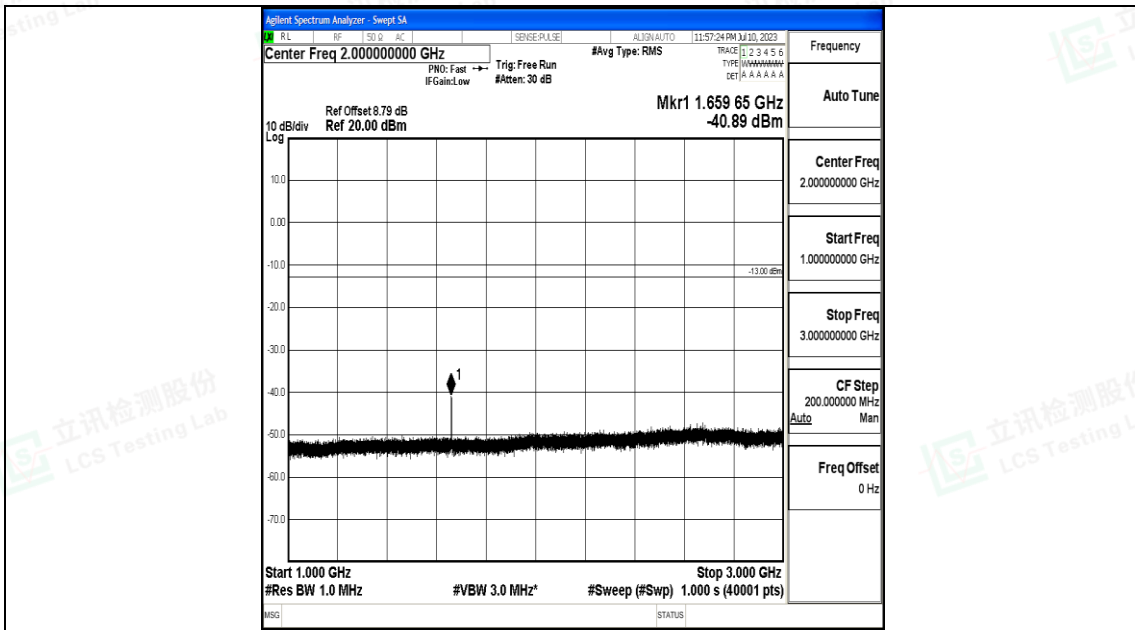
Band26_15MHz_16QAM_26915_1RB#0_1000~3000_1000~3000
