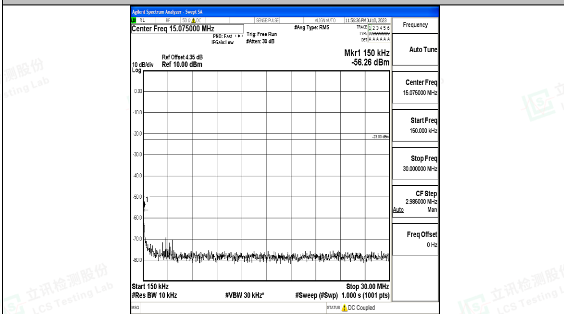
Band26_15MHz_QPSK_26915_1RB#0_0.15~30_0.15~30
