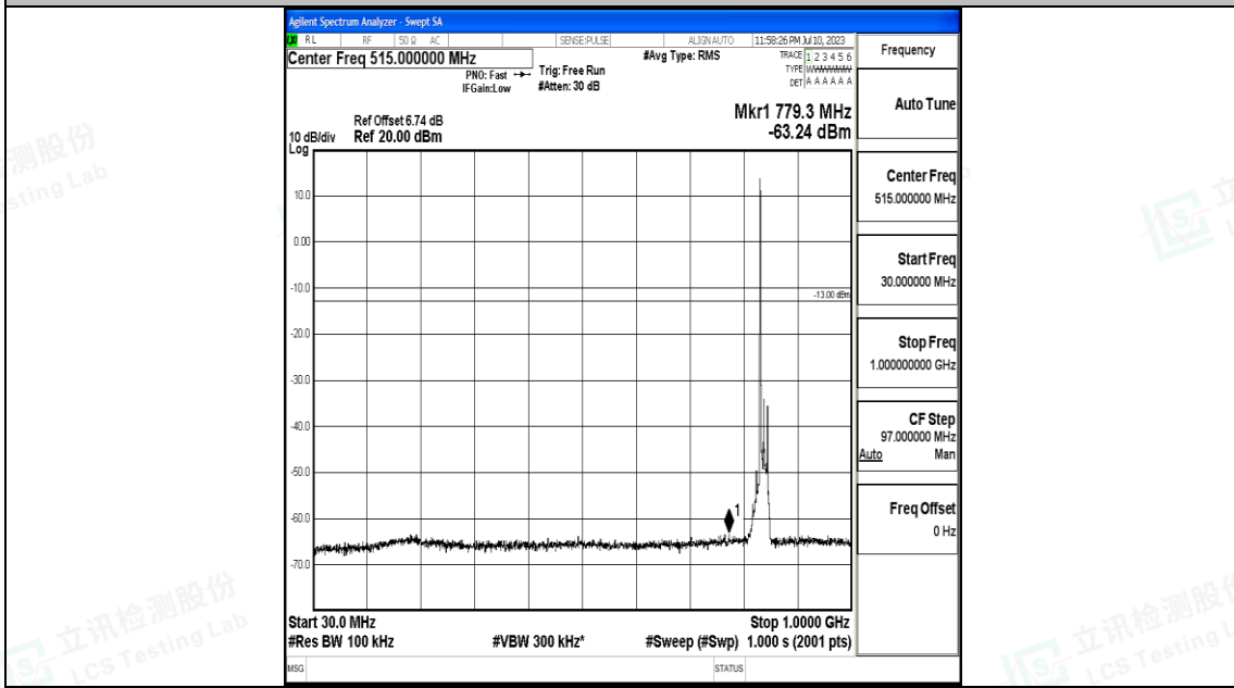
Band26_15MHz_16QAM_26965_1RB#0_30~1000_30~1000
