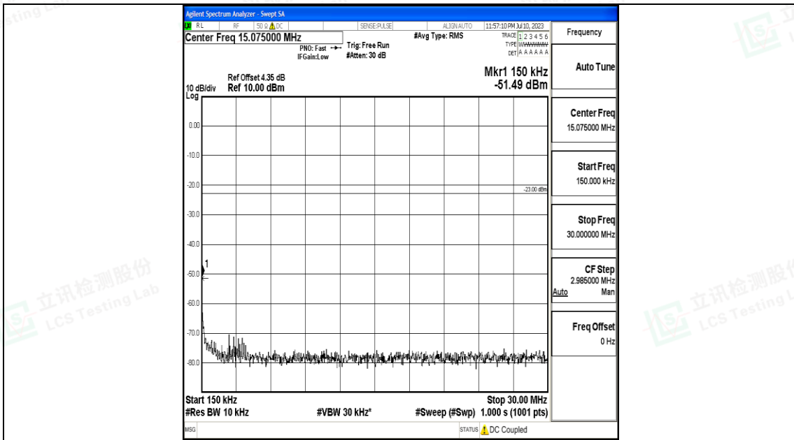
Band26_15MHz_16QAM_26915_1RB#0_0.15~30_0.15~30
