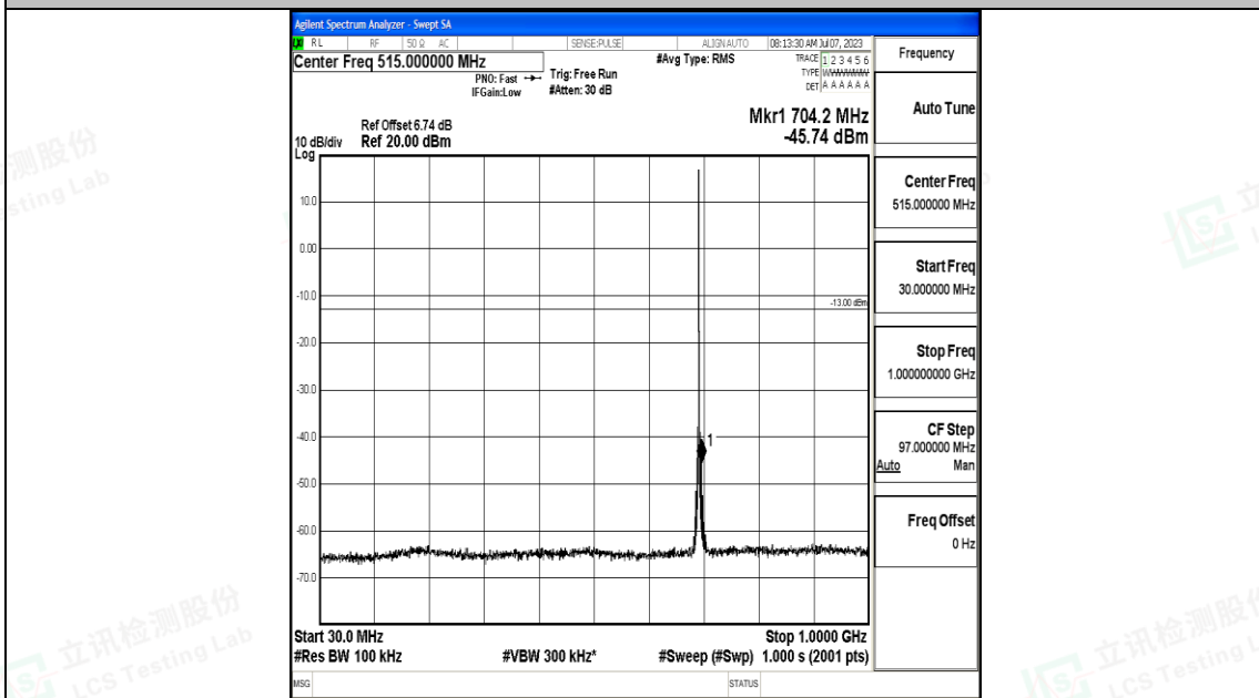
Band12_1.4MHz_QPSK_23017_1RB#0_30~1000_30~1000
