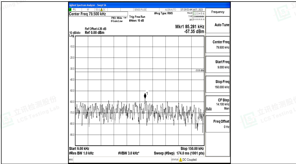
Band5_3MHz_16QAM_20635_1RB#0_0.009~0.15_0.009~0.15
