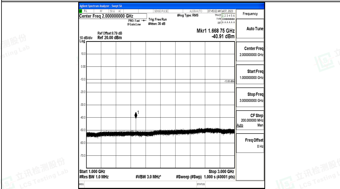
Band5_5MHz_16QAM_20525_1RB#0_1000~3000_1000~3000
