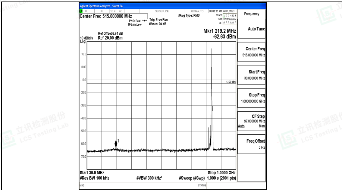
Band5_10MHz_16QAM_20600_1RB#0_30~1000_30~1000
