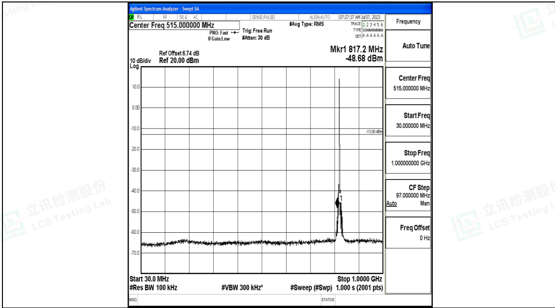
Band5_3MHz_16QAM_20415_1RB#0_30~1000_30~1000
