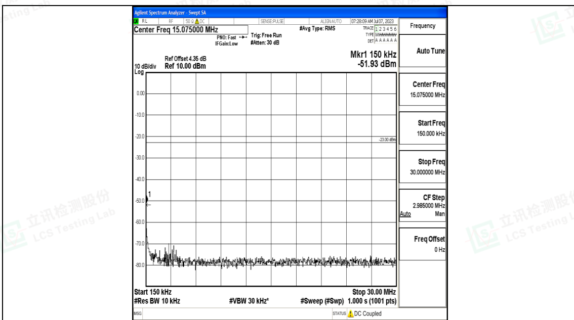
Band5_3MHz_QPSK_20525_1RB#0_0.15~30_0.15~30
