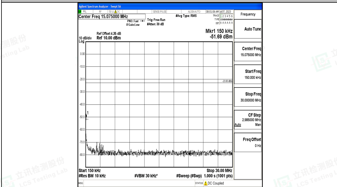
Band5_10MHz_16QAM_20600_1RB#0_0.15~30_0.15~30
