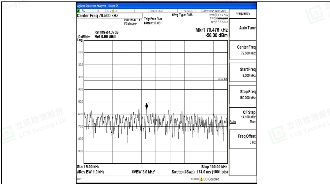
Band5_10MHz_16QAM_20525_1RB#0_0.009~0.15_0.009~0.15
