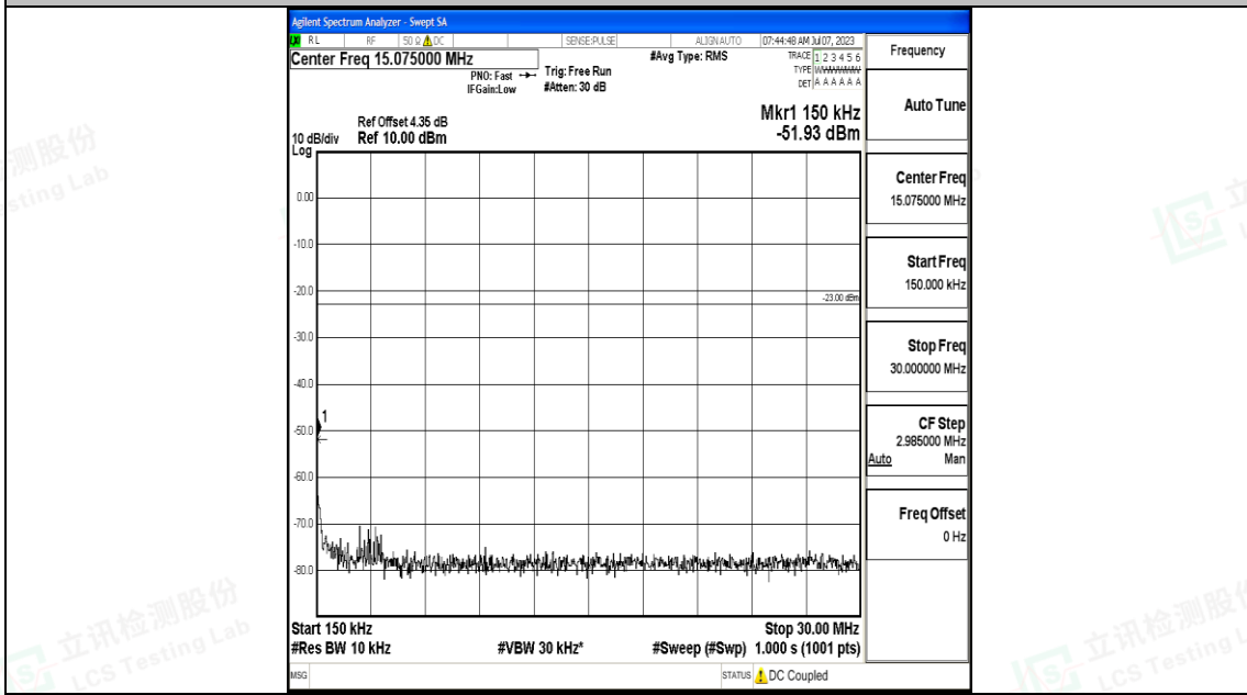
Band5_5MHz_16QAM_20525_1RB#0_0.15~30_0.15~30
