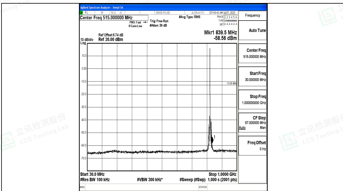
Band5_5MHz_16QAM_20425_1RB#0_30~1000_30~1000
