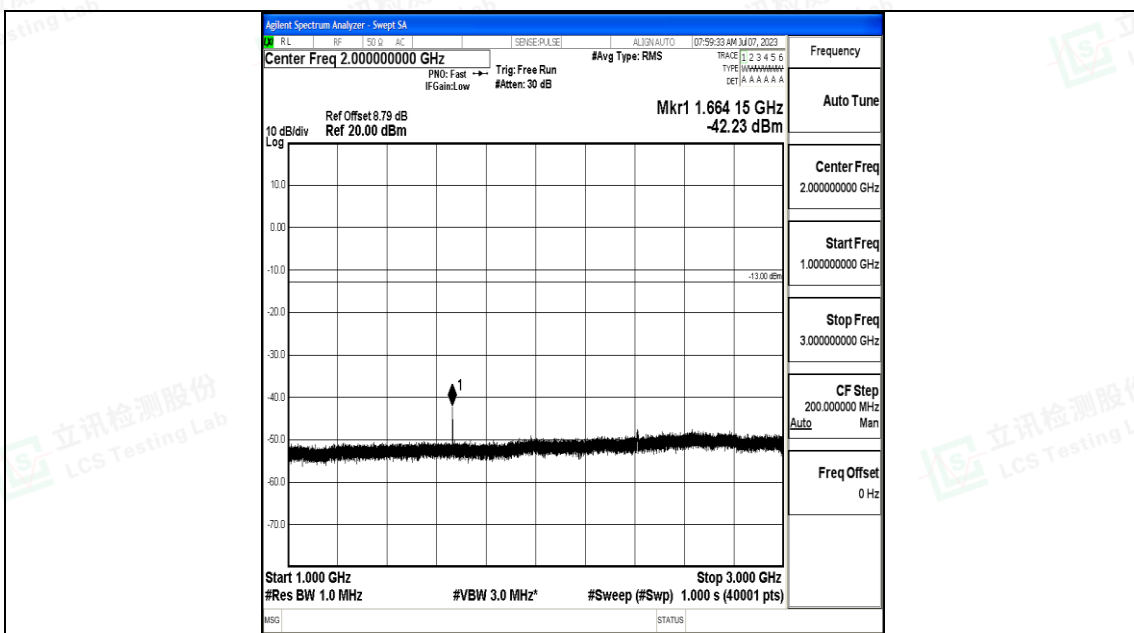
Band5_10MHz_QPSK_20525_1RB#0_1000~3000_1000~3000
