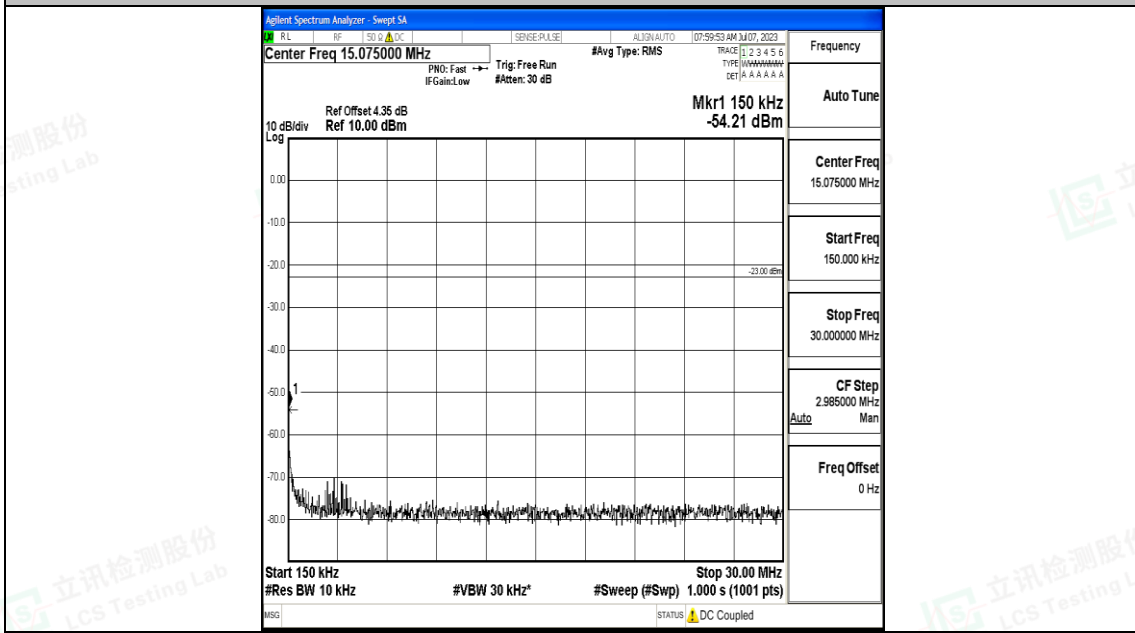
Band5_10MHz_16QAM_20525_1RB#0_0.15~30_0.15~30
