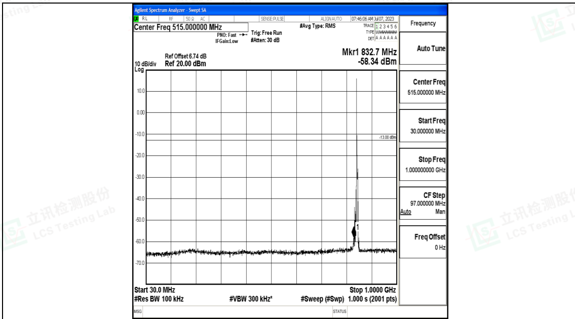
Band5_5MHz_16QAM_20625_1RB#0_30~1000_30~1000
