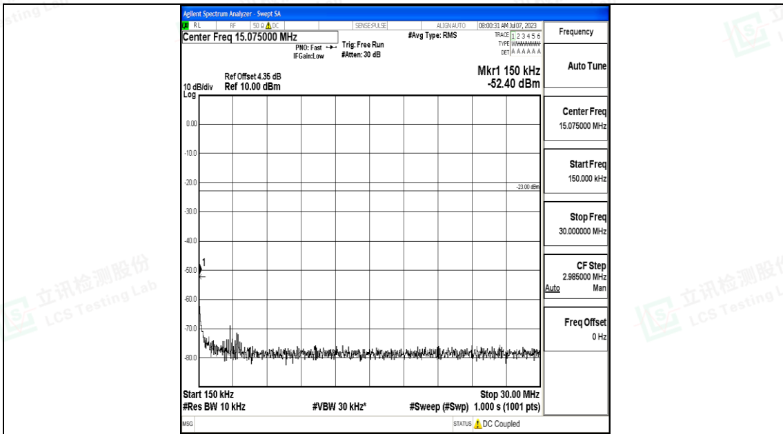
Band5_10MHz_QPSK_20600_1RB#0_0.15~30_0.15~30
