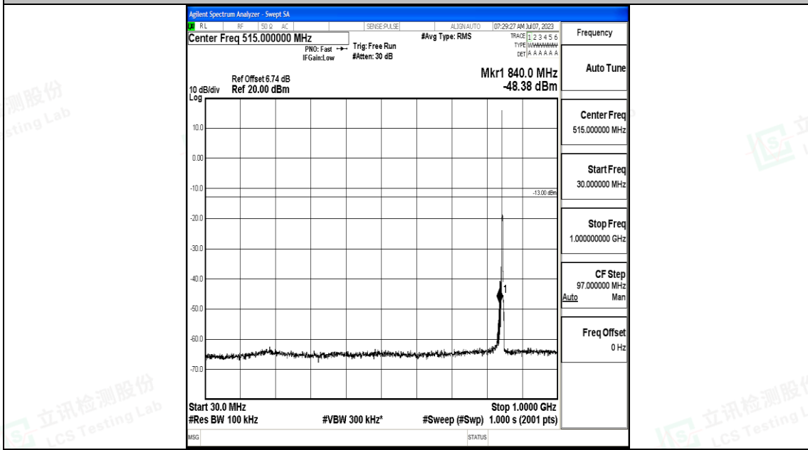
Band5_3MHz_QPSK_20635_1RB#0_30~1000_30~1000
