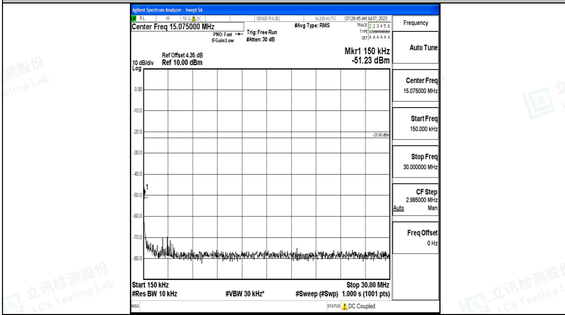
Band5_3MHz_16QAM_20525_1RB#0_0.15~30_0.15~30
