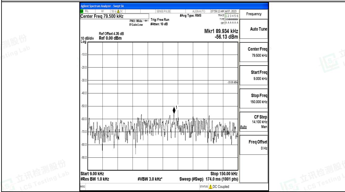
Band5_10MHz_QPSK_20525_1RB#0_0.009~0.15_0.009~0.15
