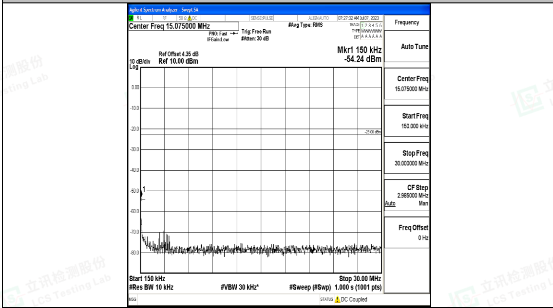
Band5_3MHz_16QAM_20415_1RB#0_0.15~30_0.15~30
