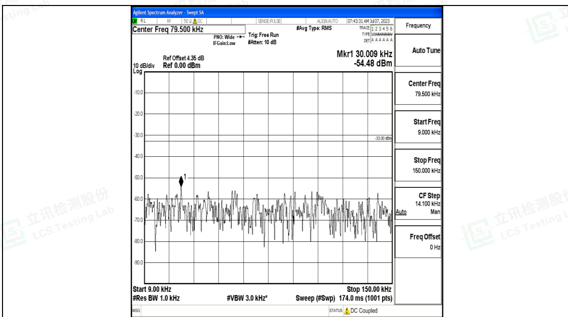
Band5_5MHz_16QAM_20425_1RB#0_0.009~0.15_0.009~0.15
