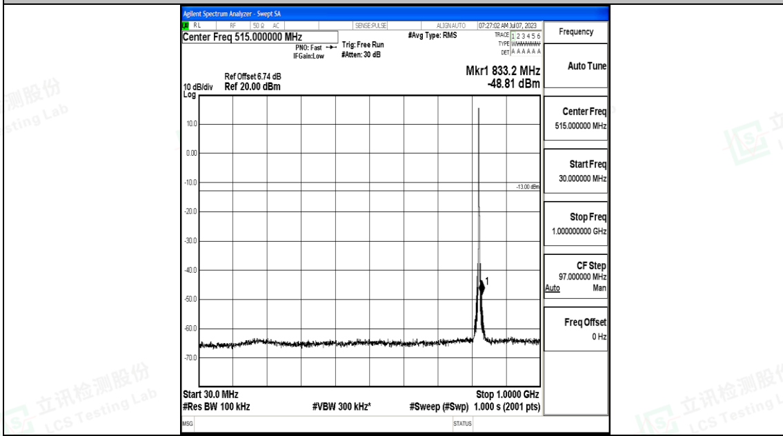
Band5_3MHz_QPSK_20415_1RB#0_30~1000_30~1000
