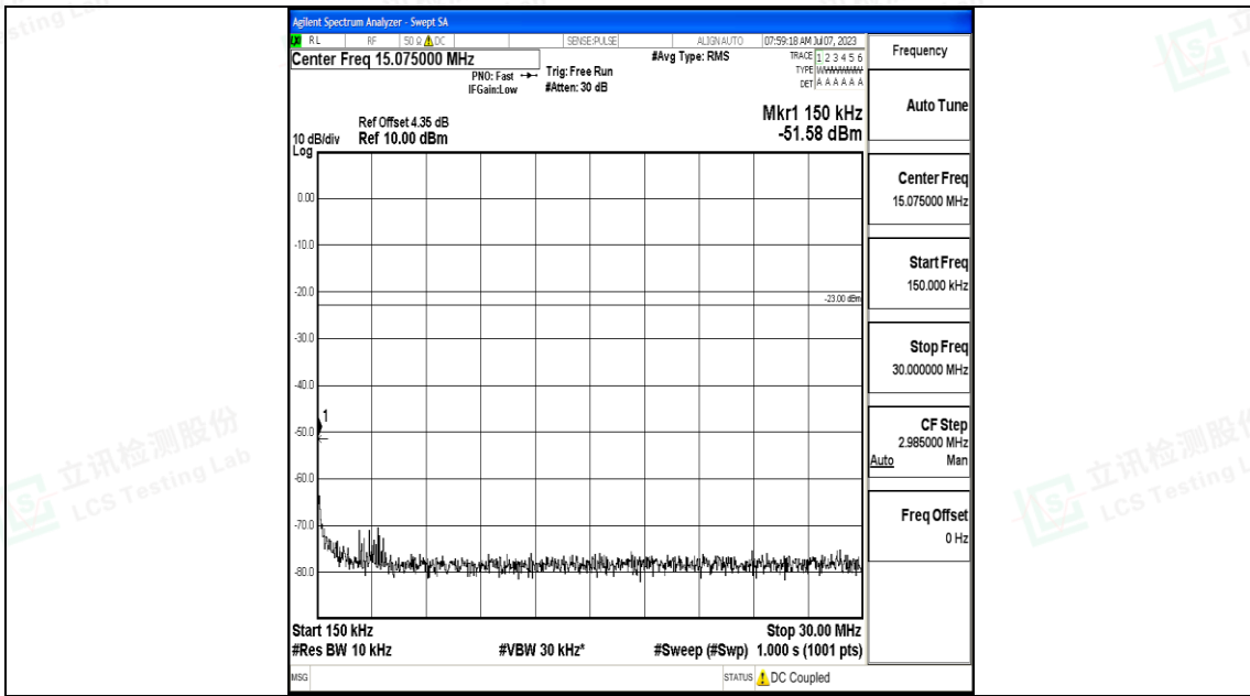
Band5_10MHz_QPSK_20525_1RB#0_0.15~30_0.15~30
