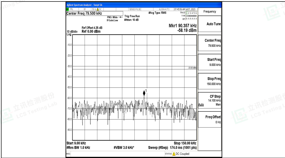
Band5_5MHz_16QAM_20625_1RB#0_0.009~0.15_0.009~0.15
