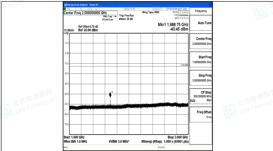
Band5_5MHz_QPSK_20625_1RB#0_1000~3000_1000~3000
