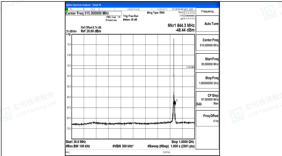
Band5_3MHz_16QAM_20525_1RB#0_30~1000_30~1000
