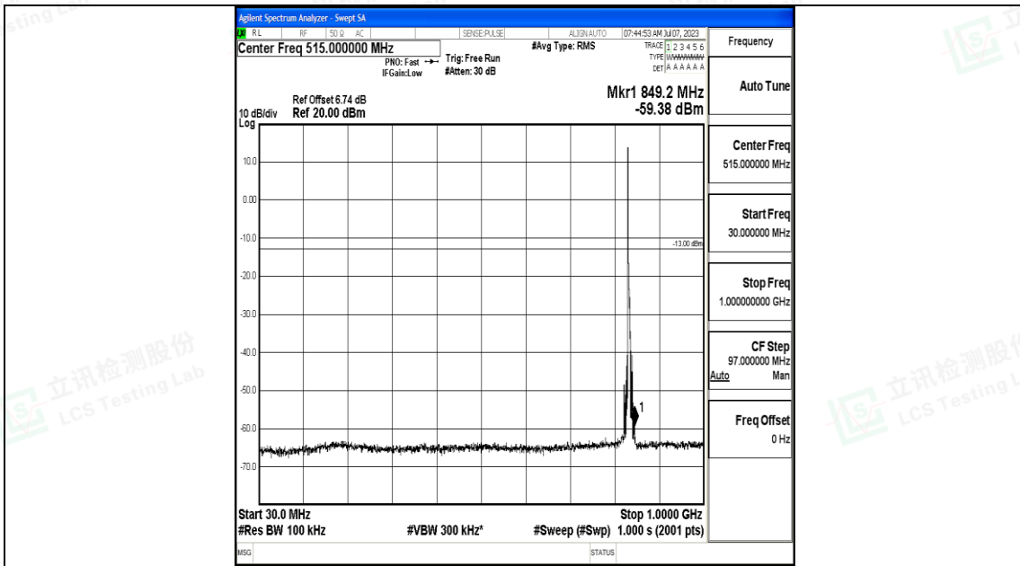
Band5_5MHz_16QAM_20525_1RB#0_30~1000_30~1000
