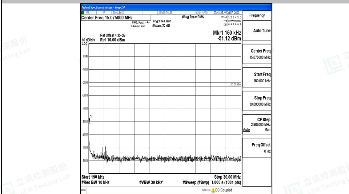
Band5_5MHz_16QAM_20425_1RB#0_0.15~30_0.15~30
