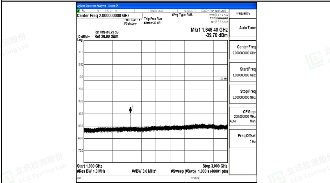
Band5_3MHz_16QAM_20415_1RB#0_1000~3000_1000~3000
