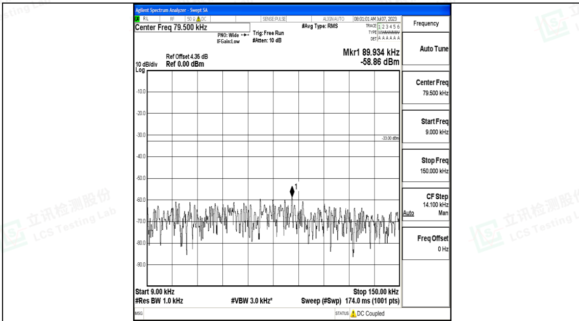
Band5_10MHz_16QAM_20600_1RB#0_0.009~0.15_0.009~0.15
