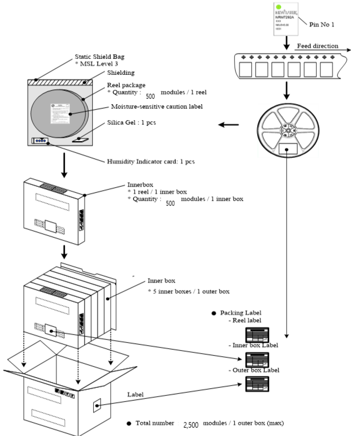
Figure 7.5 Packing process
