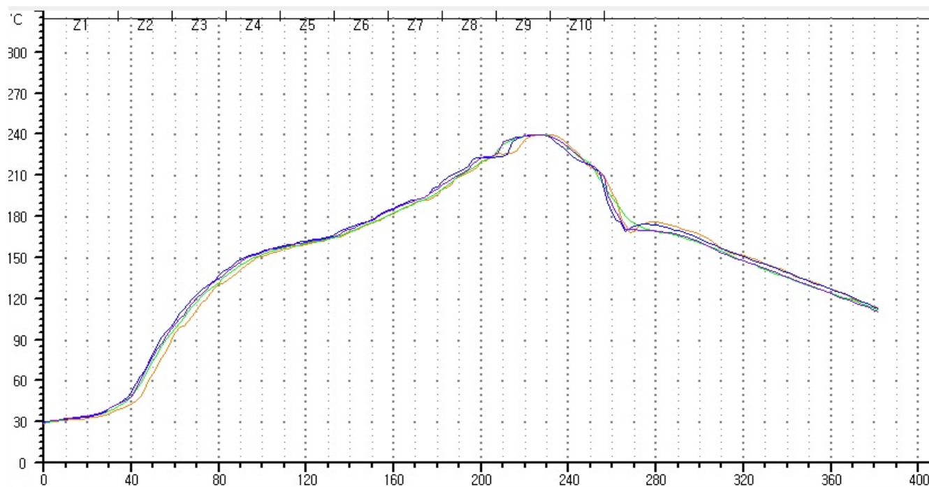
Figure 8.1 Reflow profile
