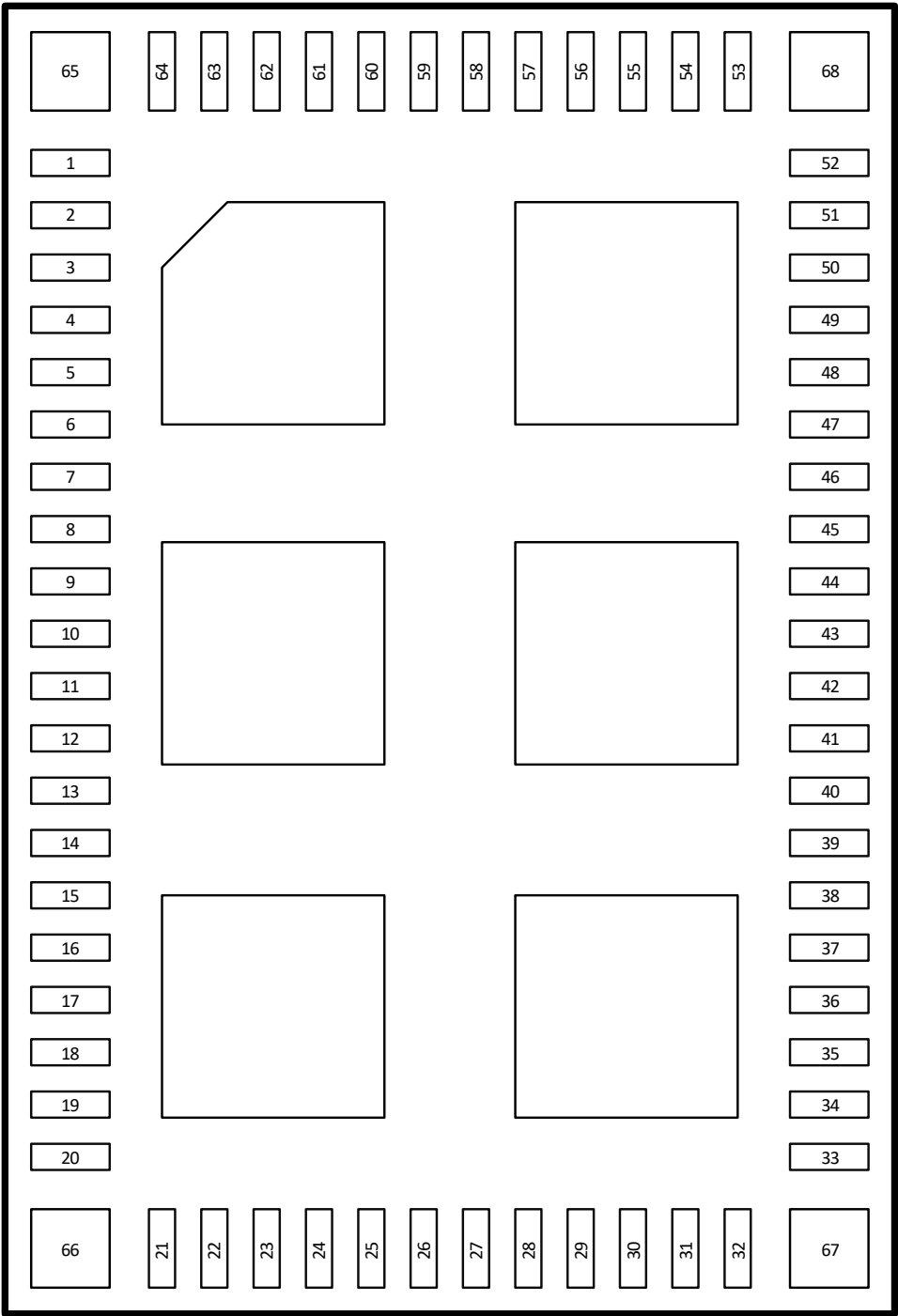
Figure 3.1 NRM7292D module pinout (top view)
