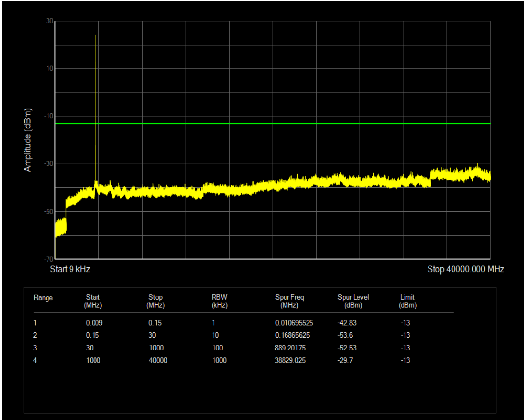
n78(3700-3800) SCS=30kHz DFT_QPSK BW=20MHz Channel=647334 RB=1@50
