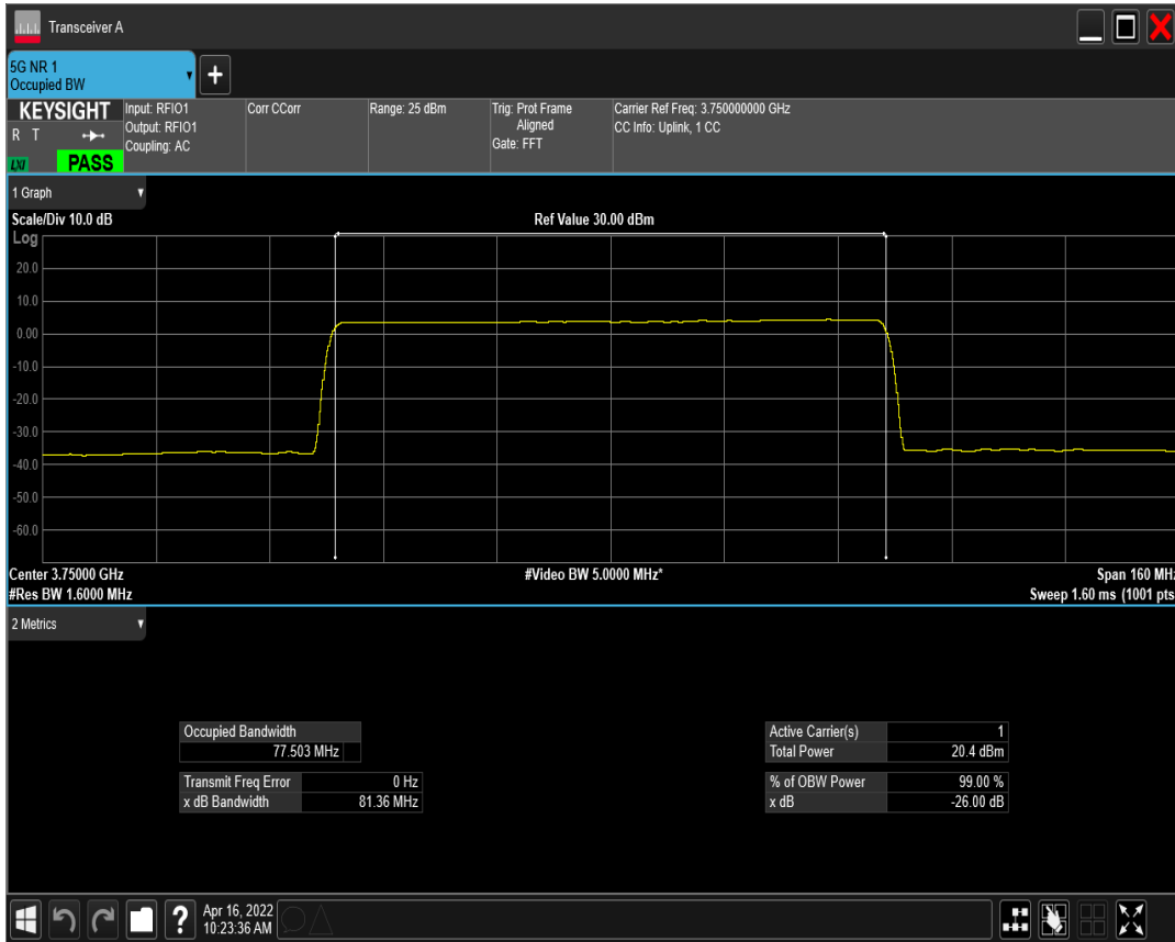
n78(3700-3800) SCS=30kHz CP_QPSK BW=80MHz Channel=650000 RB=217@0
