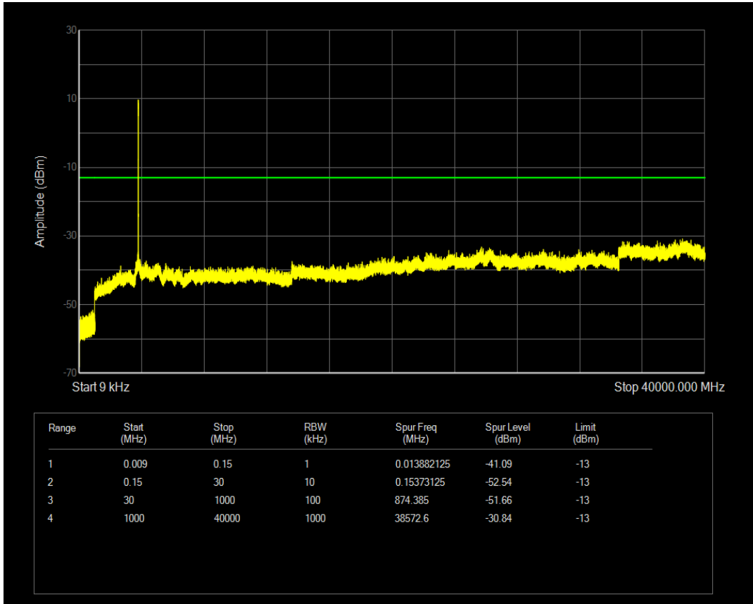
n78(3700-3800) SCS=30kHz DFT_QPSK BW=20MHz Channel=652666 RB=1@50
