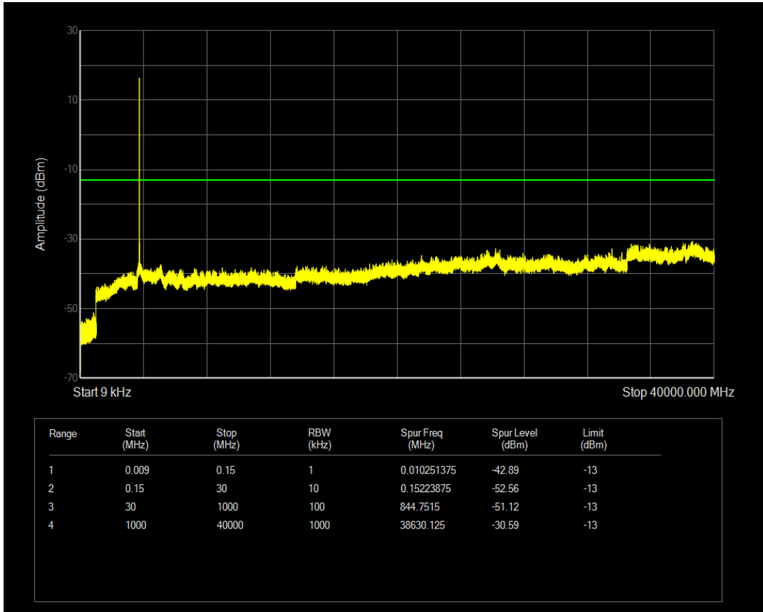
n78(3700-3800) SCS=30kHz DFT_QPSK BW=20MHz Channel=650000 RB=1@50
