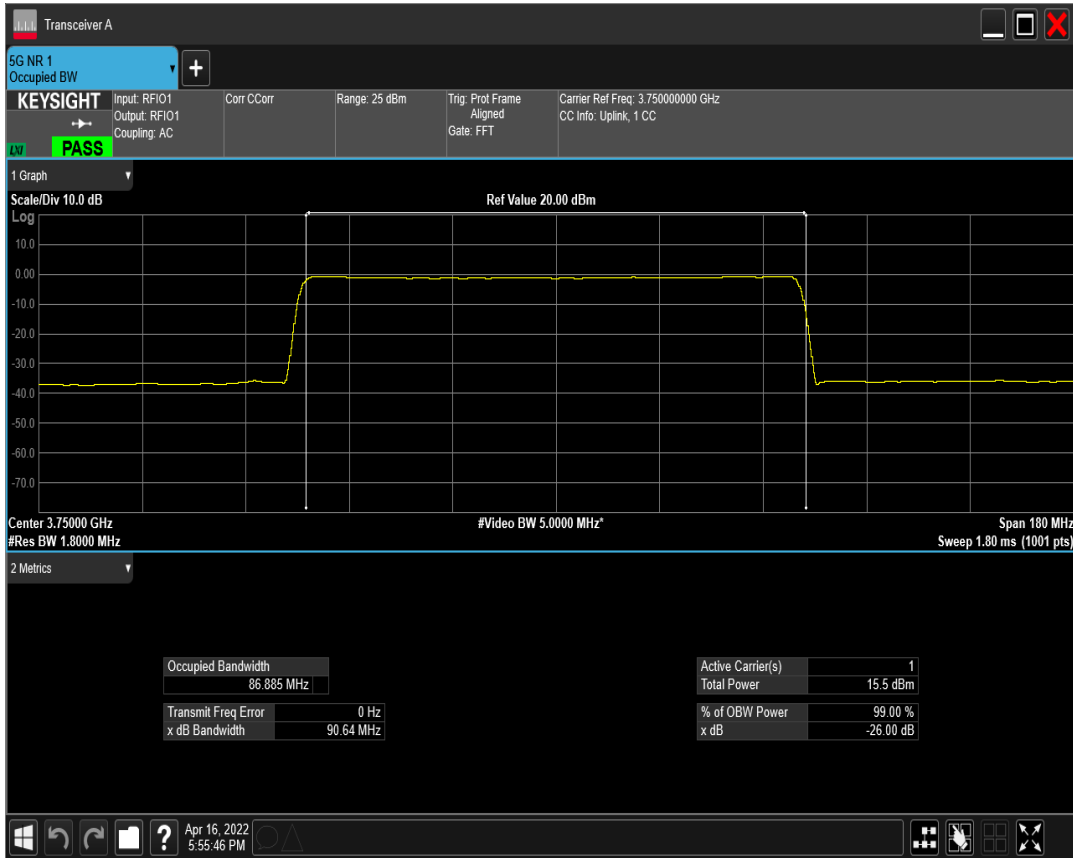
n78(3700-3800) SCS=30kHz CP_QPSK BW=90MHz Channel=650000 RB=245@0
