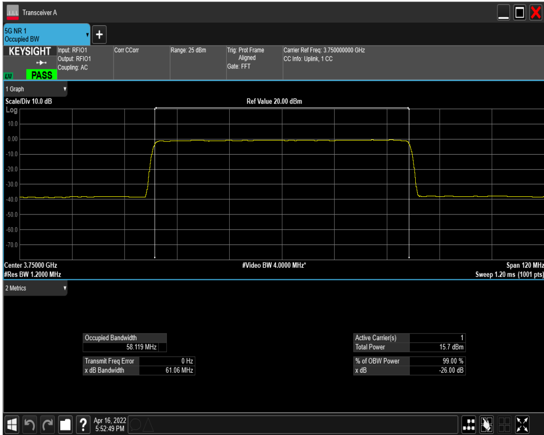
n78(3700-3800) SCS=30kHz CP_QPSK BW=60MHz Channel=650000 RB=162@0
