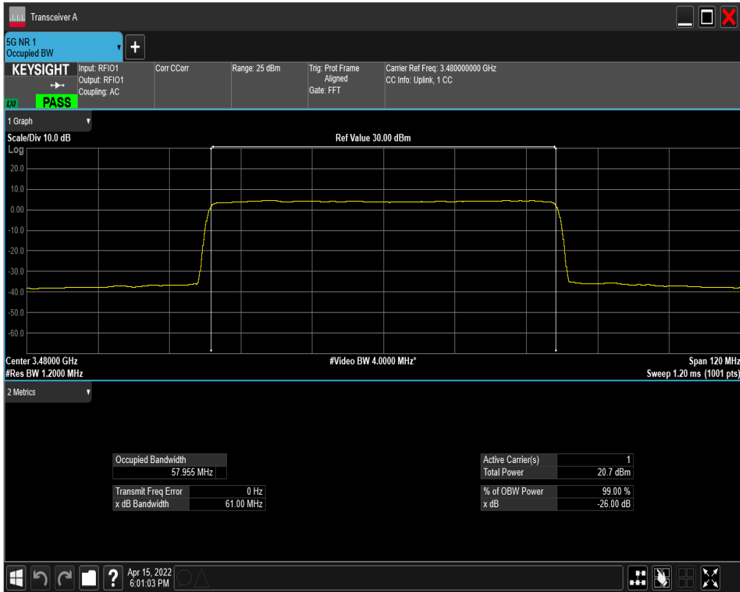
n78(3450-3550) SCS=30kHz CP_QPSK BW=60MHz Channel=632000 RB=162@0
