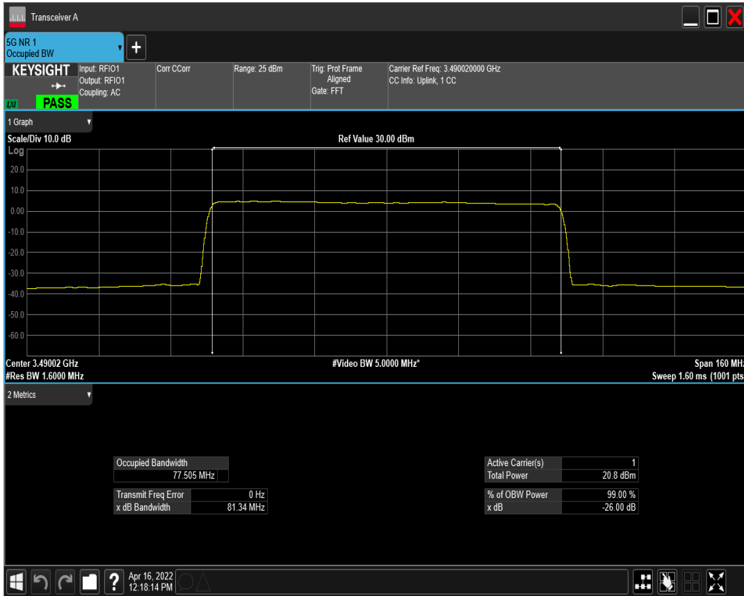
n78(3450-3550) SCS=30kHz CP_QPSK BW=80MHz Channel=632668 RB=217@0
