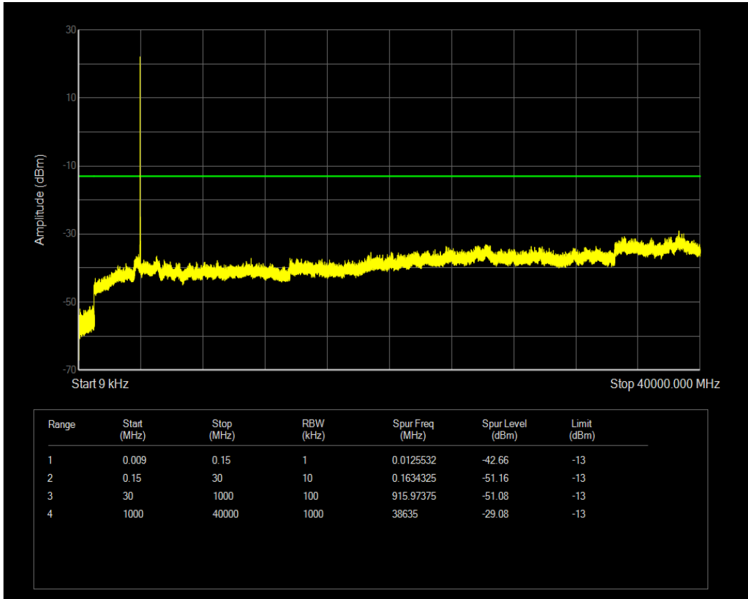
n77(3700-3980) SCS=30kHz DFT_QPSK BW=20MHz Channel=664666 RB=1 @50
