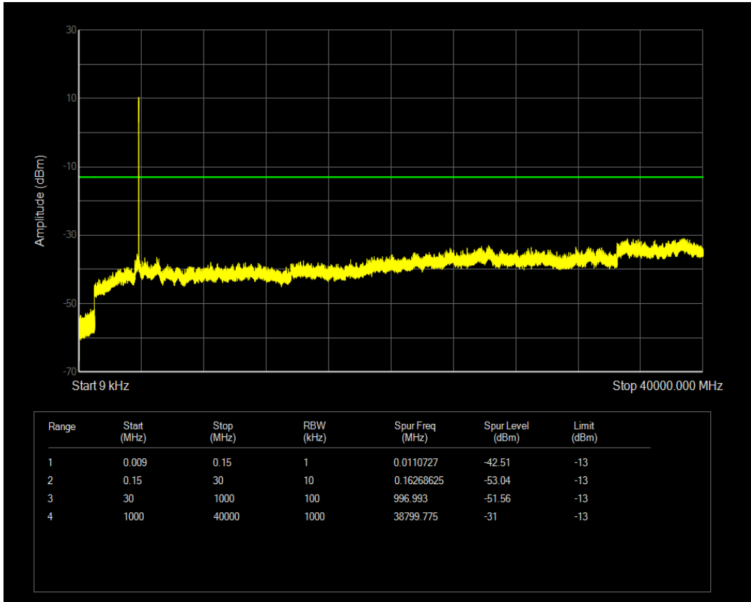
n77(3700-3980) SCS=30kHz DFT_QPSK BW=20MHz Channel=656000 RB=1@50
