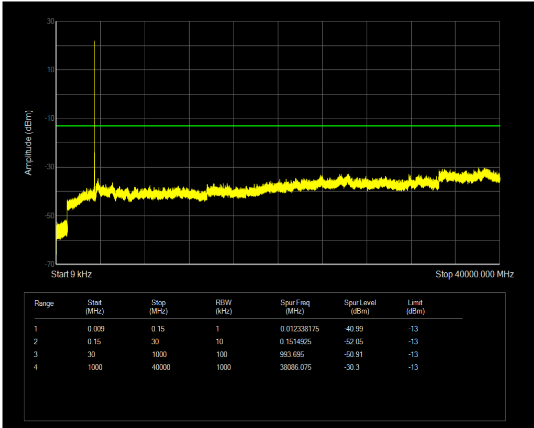
n77(3450-3550) SCS=30kHz DFT_QPSK BW=20MHz Channel=630668 RB=1 @50
