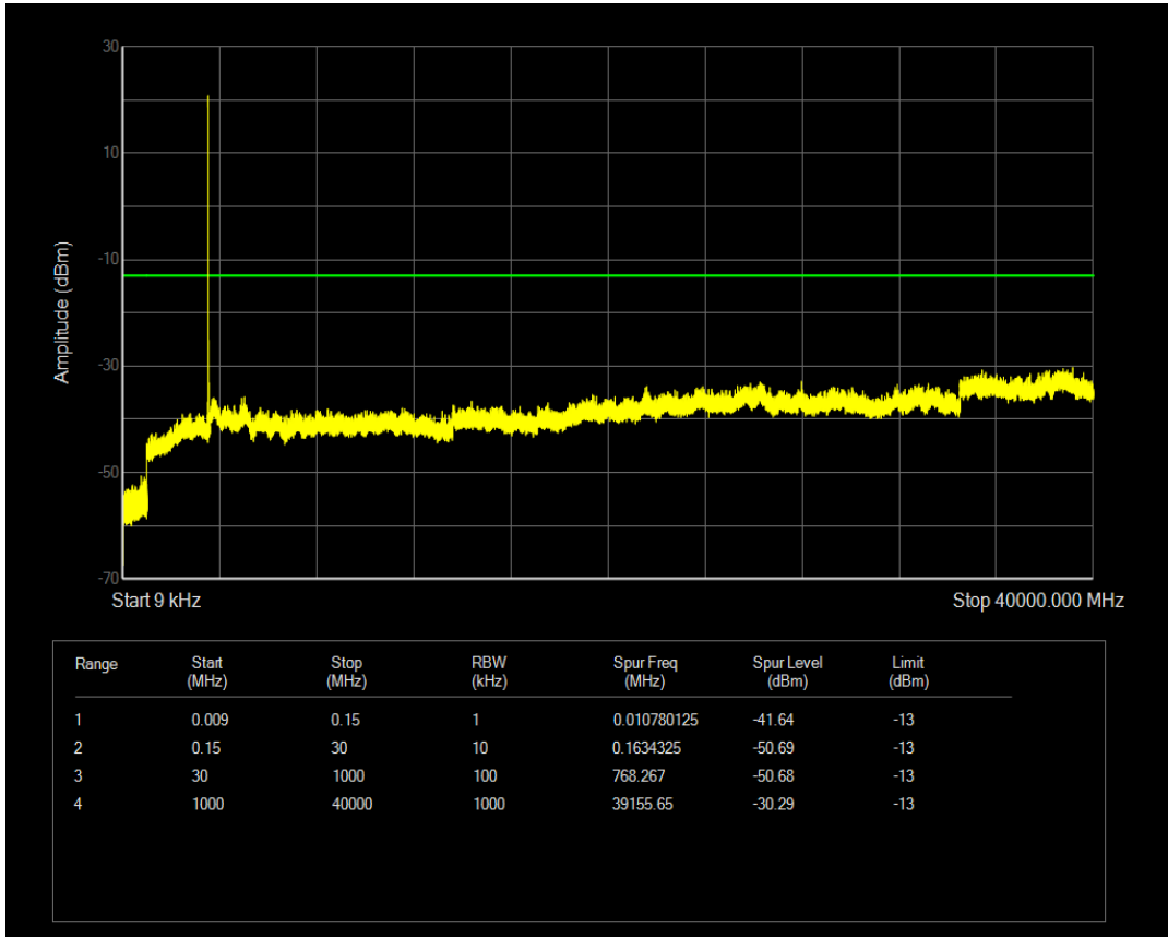
n77(3450-3550) SCS=30kHz DFT_QPSK BW=20MHz Channel=636000 RB=1@50
