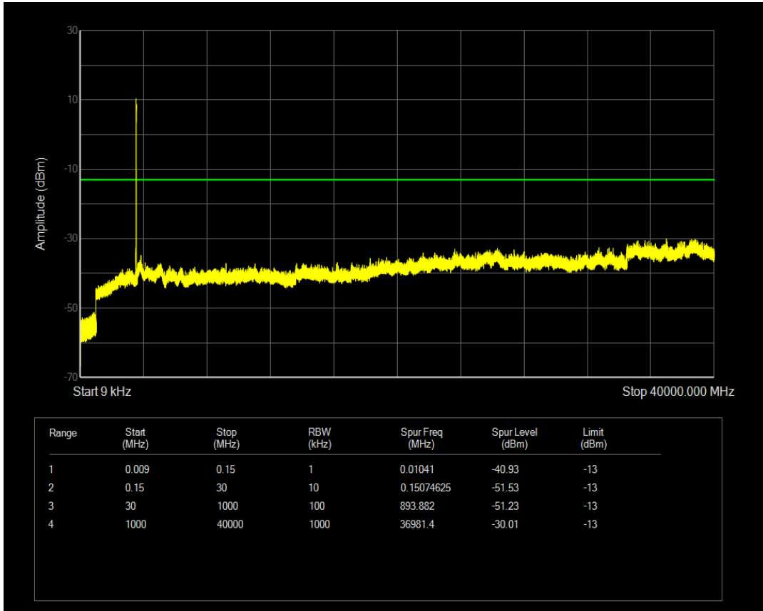
n77(3450-3550) SCS=30kHz DFT_QPSK BW=20MHz Channel=636000 RB=1@0
