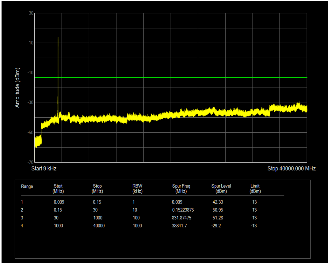
n77(3450-3550) SCS=30kHz DFT_QPSK BW=20MHz Channel=630668 RB=1@0
