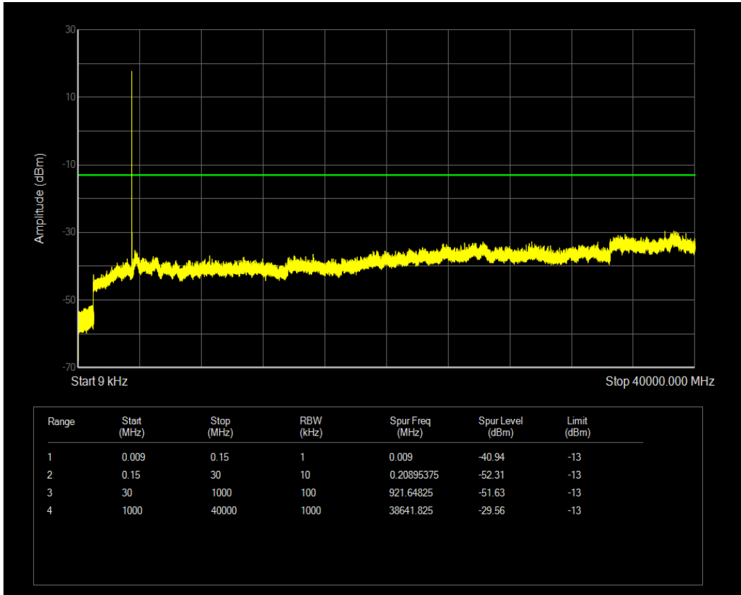
n77(3450-3550) SCS=30kHz DFT_QPSK BW=20MHz Channel=633334 RB=1@50
