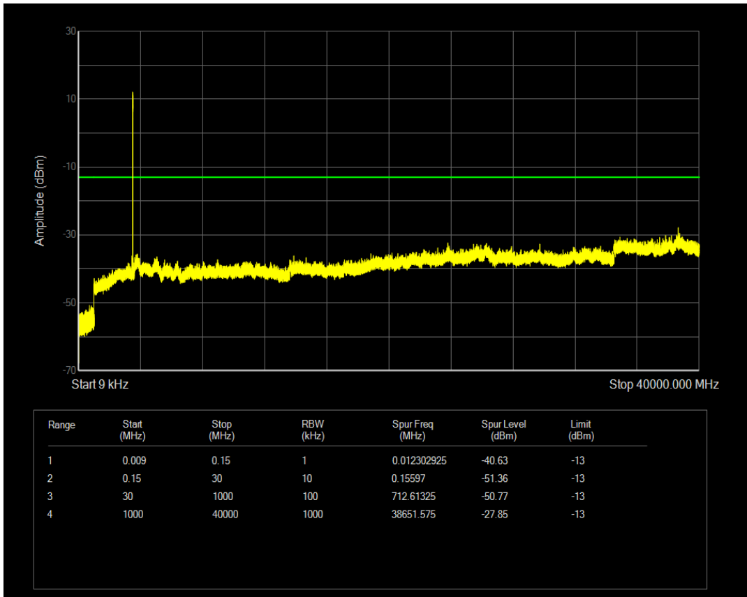
n77(3450-3550) SCS=30kHz DFT_QPSK BW=20MHz Channel=633334 RB=1@0
