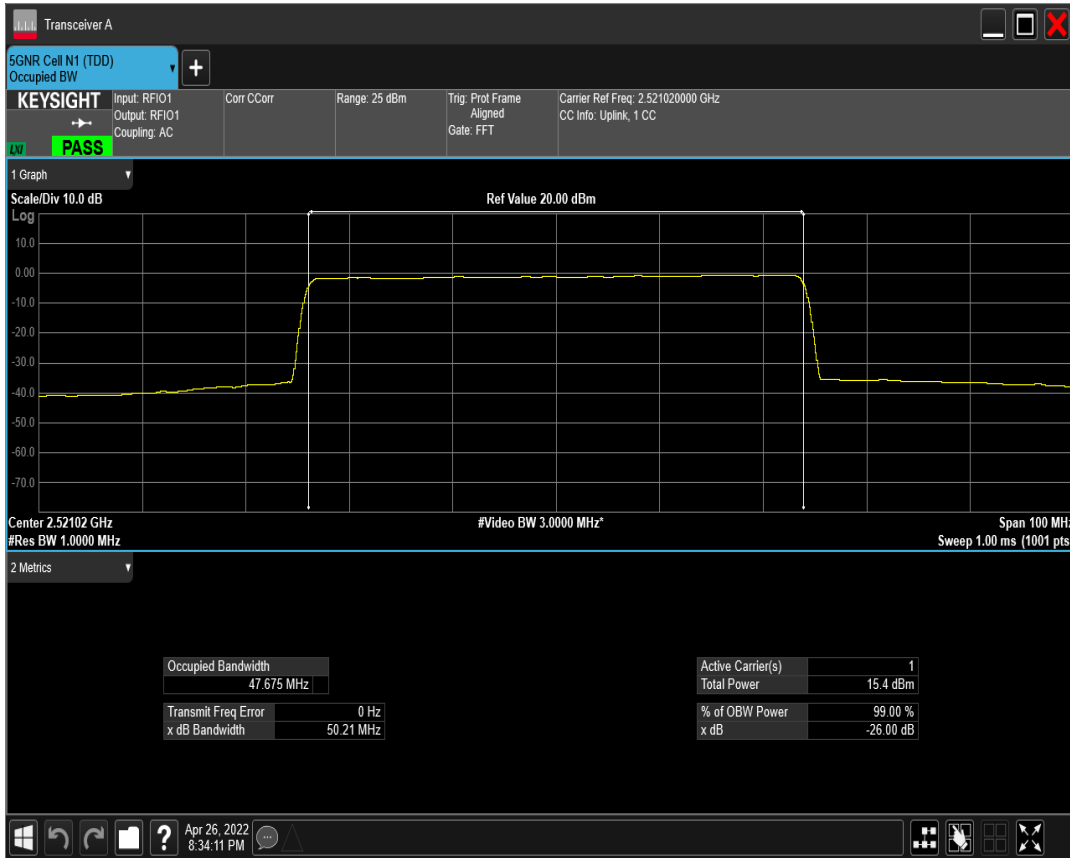
n41 SCS=30kHz CP_QAM256 BW=50MHz Channel=504204 RB=133@0 ant2
