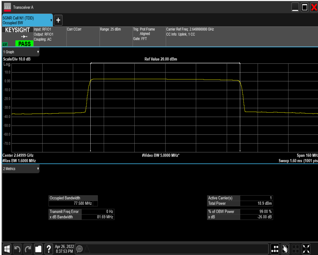
n41 SCS=30kHz CP_QPSK BW=80MHz Channel=529998 RB=217@0 ant2
