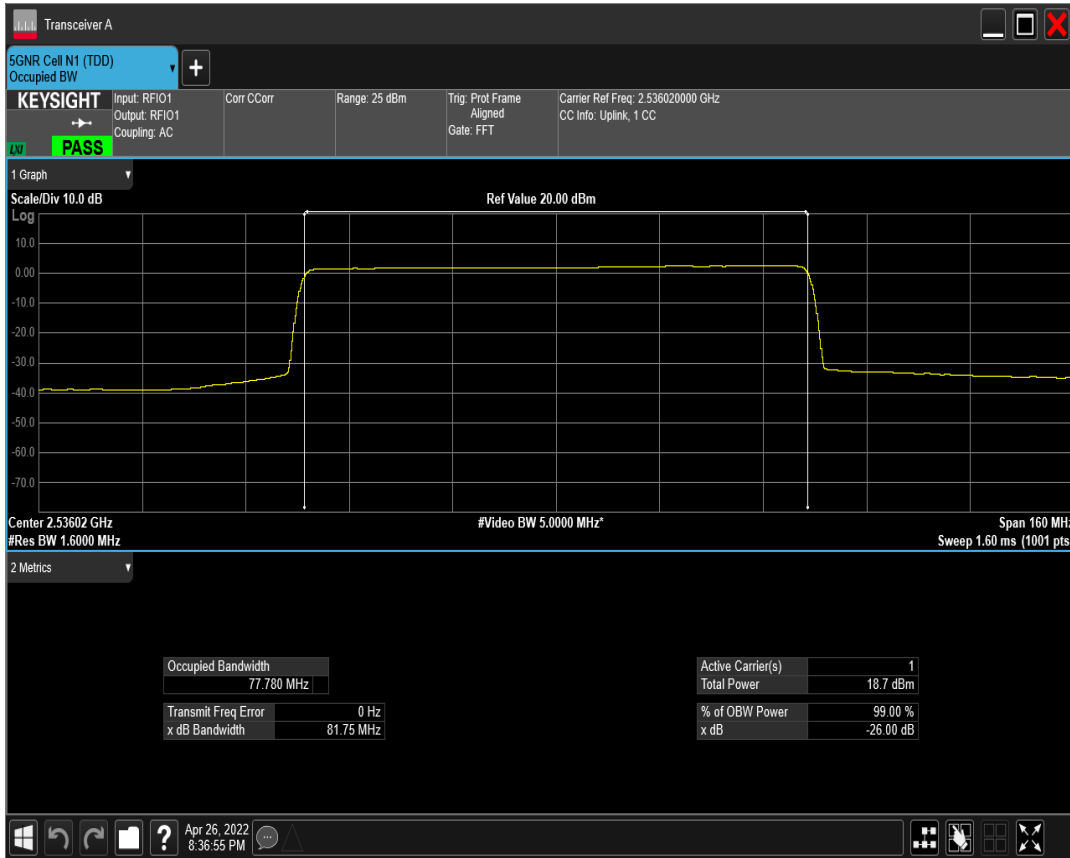
n41 SCS=30kHz CP_QPSK BW=80MHz Channel=507204 RB=217@0 ant2
