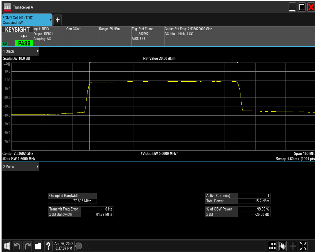
n41 SCS=30kHz CP_QAM256 BW=80MHz Channel=507204 RB=217@0 ant2
