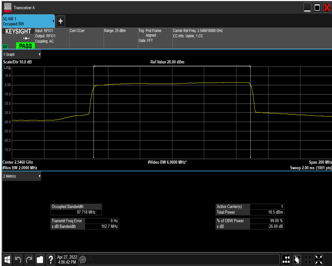
n41 SCS=30kHz CP_QAM64 BW=100MHz Channel=509202 RB=273@0 ant2
