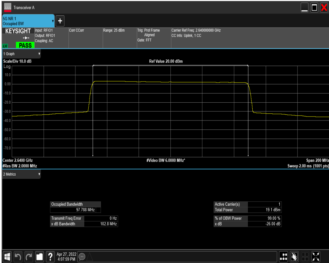
n41 SCS=30kHz CP_QAM16 BW=100MHz Channel=528000 RB=273@0 ant2
