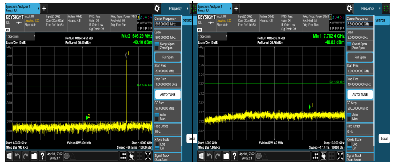
Band26-1.4MHz-16QAM-26783-1RB#0-Range1:30 ~1000MHz
