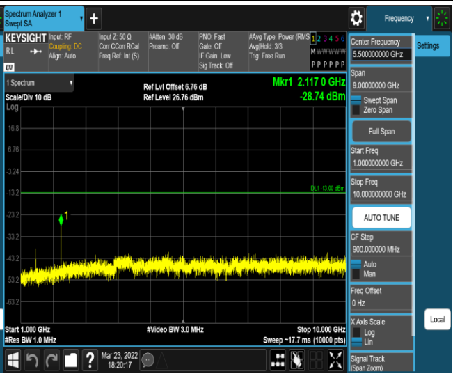
Band17-10MHz-16QAM-23800-1RB#0-Range2:1000~ 10000MHz
