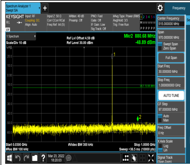
Band17-10MHz-16QAM-23800-1RB#0-Range1:30 ~1000MHz
