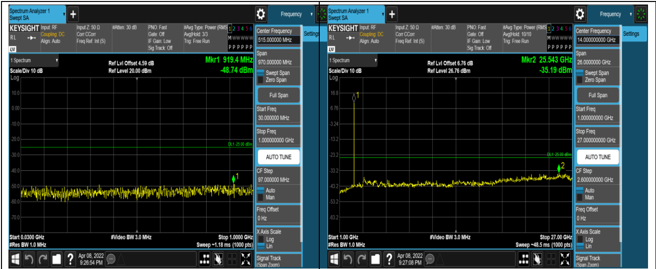
Band38-5MHz-16QAM-37775-1RB#0-Range1:30~1000MHz
