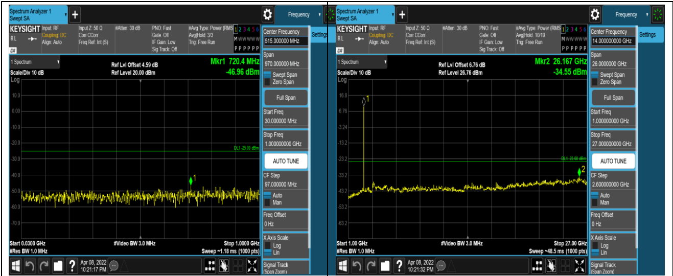
Band41-20MHz-QPSK-39750-1RB#0-Range1:30~1000MHz
