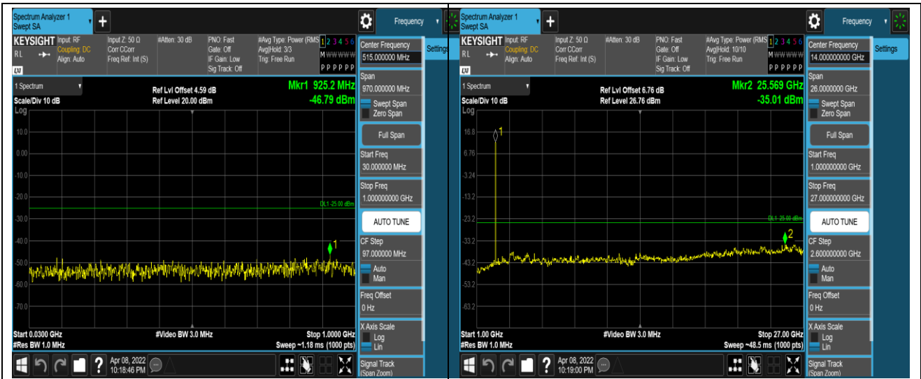
Band41-5MHz-QPSK-40620-1RB#0-Range1:30~1000MHz
