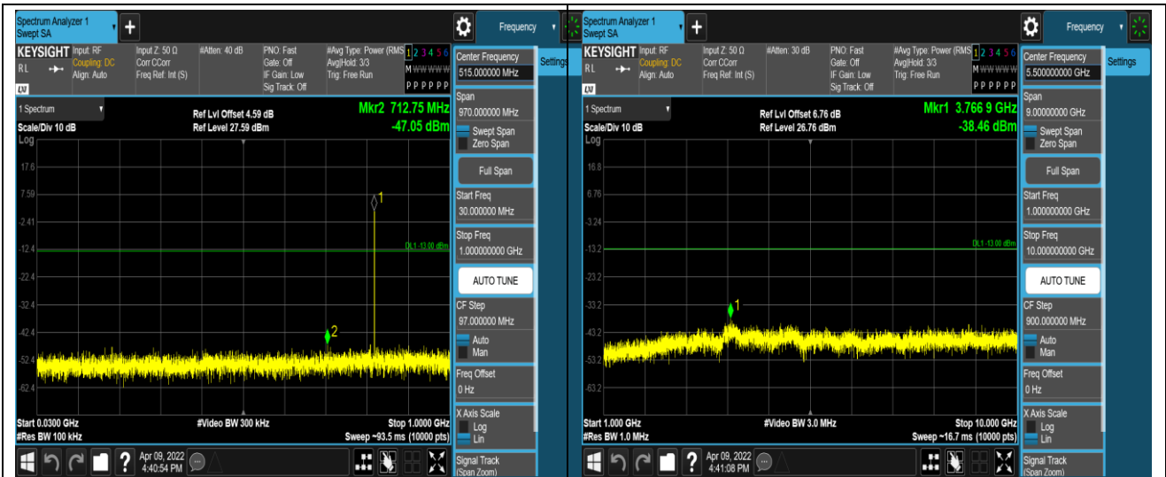
Band26-1.4MHz-QPSK-26797-1RB#0-Range1:30~1000MHz
