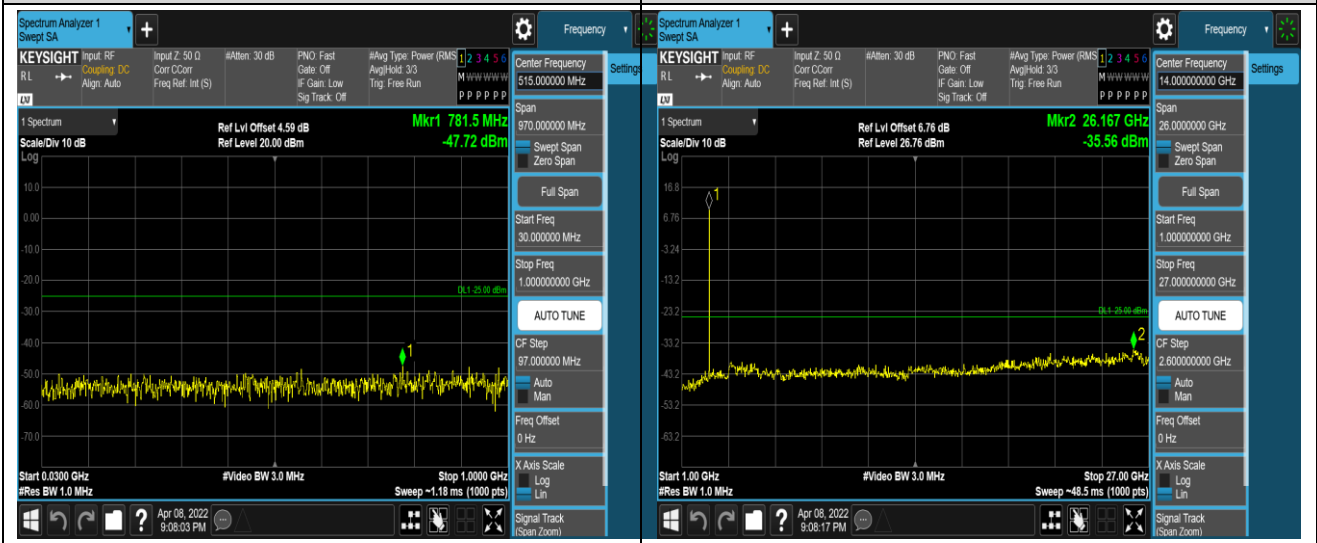
Band7-20MHz-16QAM-21100-1RB#0-Range1:30~1000MHz
