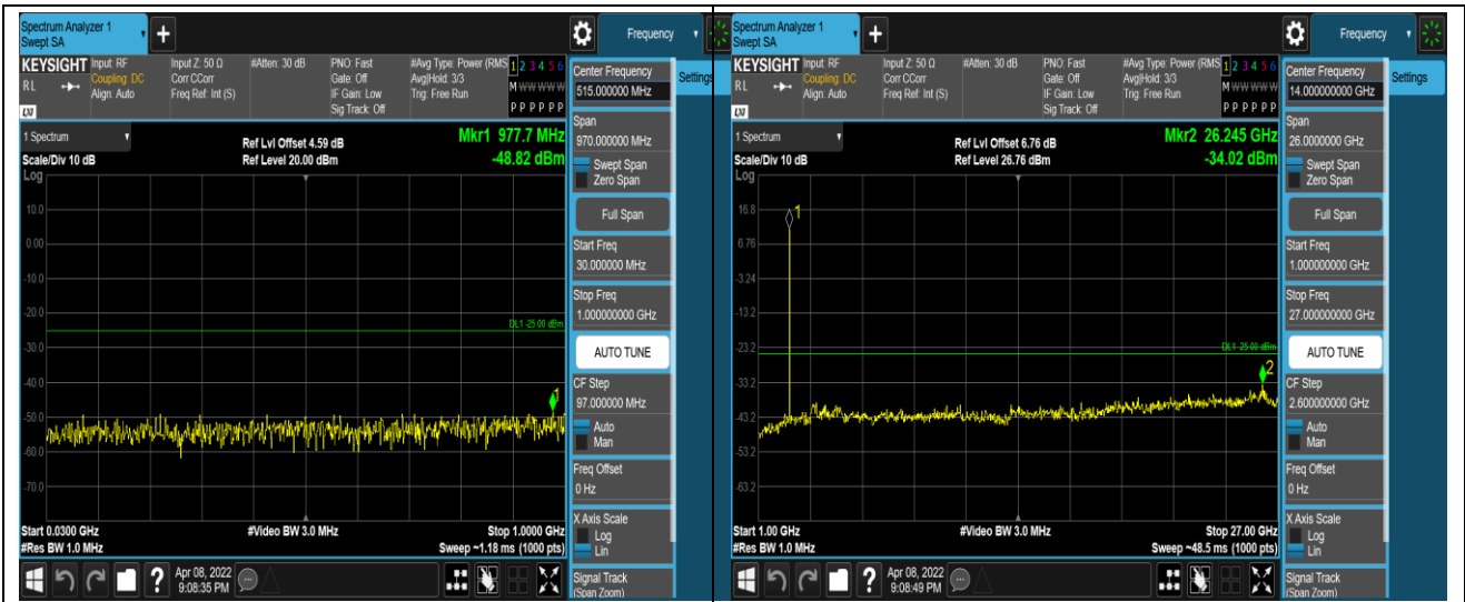
Band7-20MHz-16QAM-20850-1RB#0-Range1:30~1000MHz
