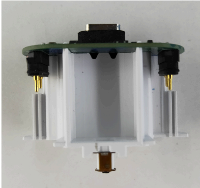
Charger internal photo
