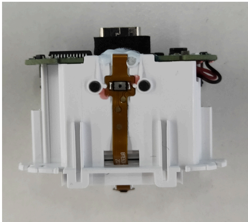
Charger internal photo
