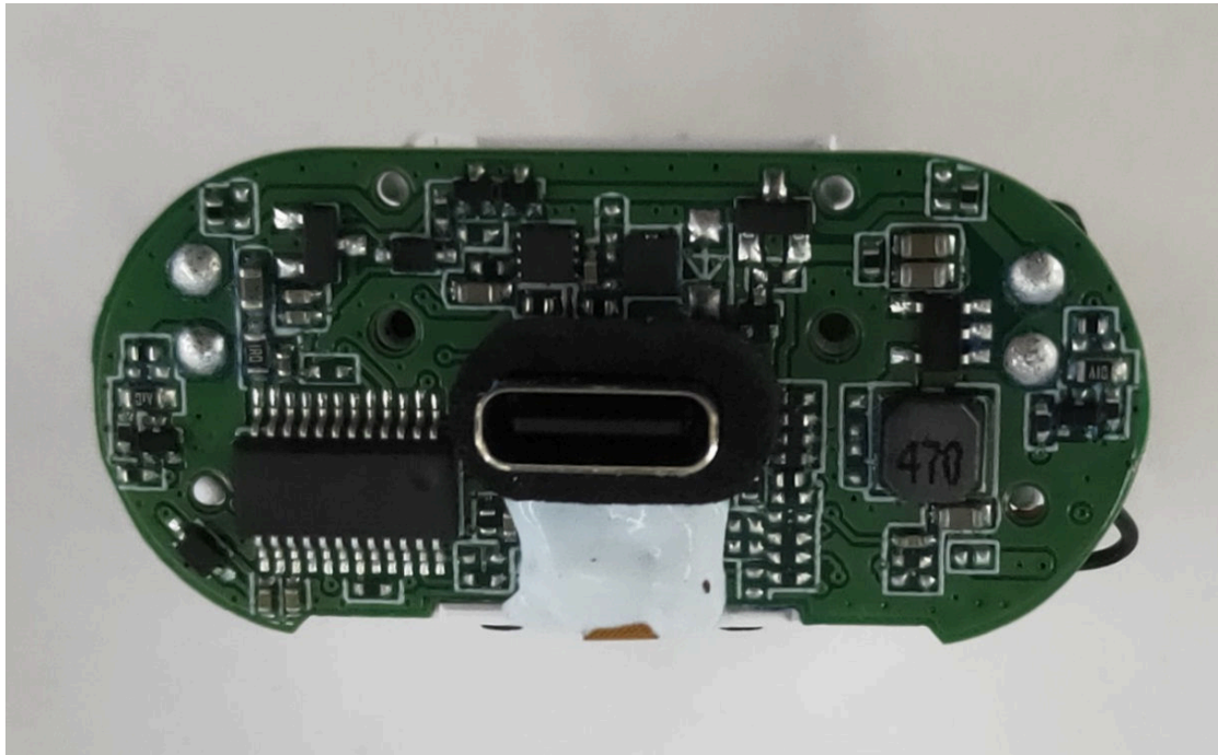
Charger internal photo
