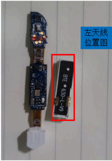
Location diagram of left earphone antenna
