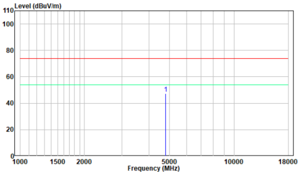
Horizontal
