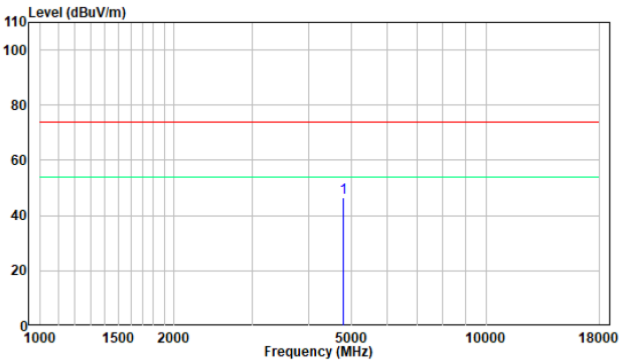
Vertical
