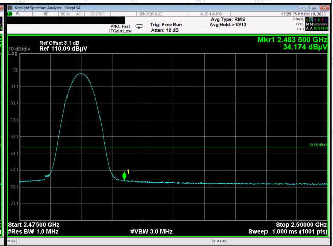
Average Value(Horizontal)
