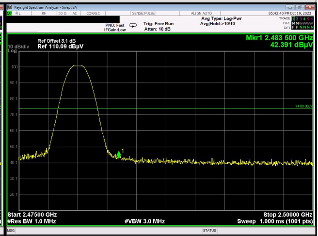
Peak Value(Horizontal)
