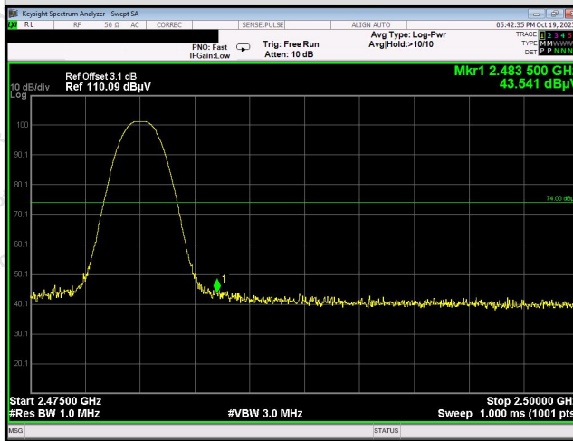
Peak Value(Vertical)
