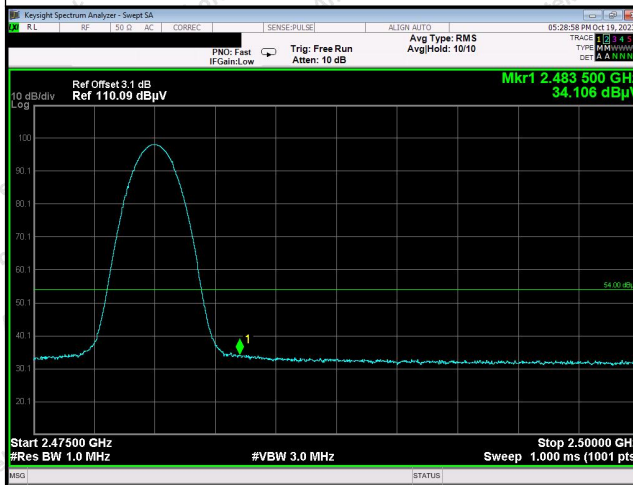
Average Value(Vertical)
