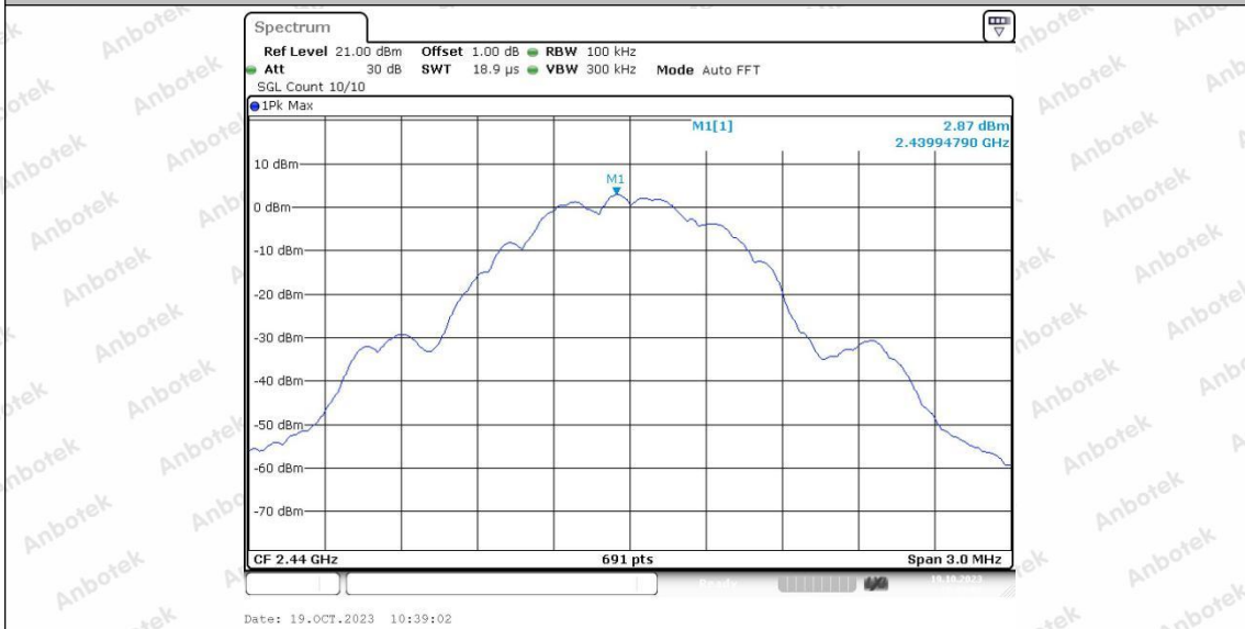
BLE_1M_Ant1_2440_30~1000
