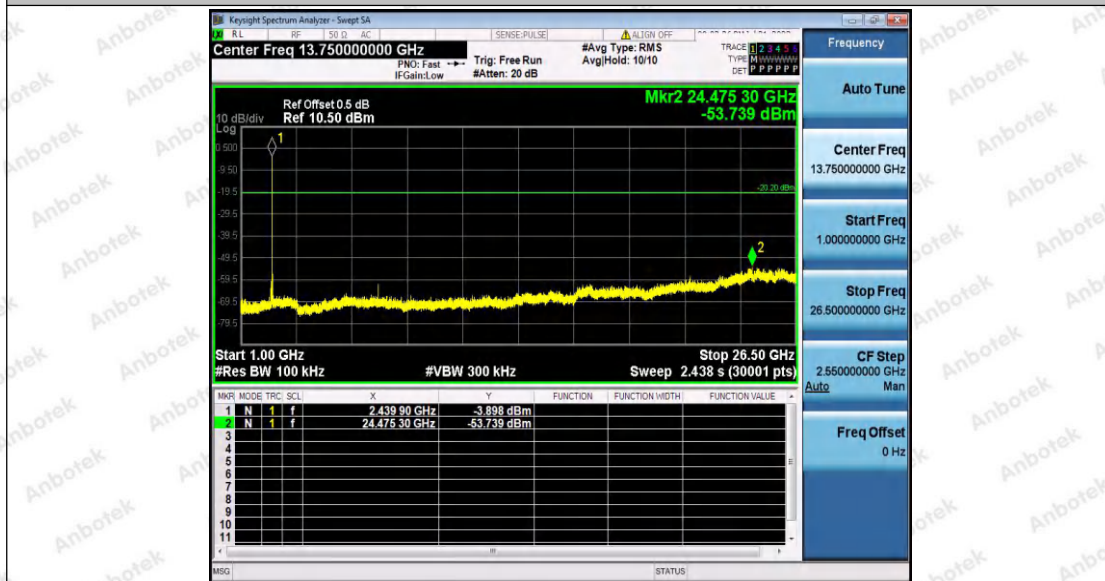
BLE_2M_Ant1_2440_1000~26500
