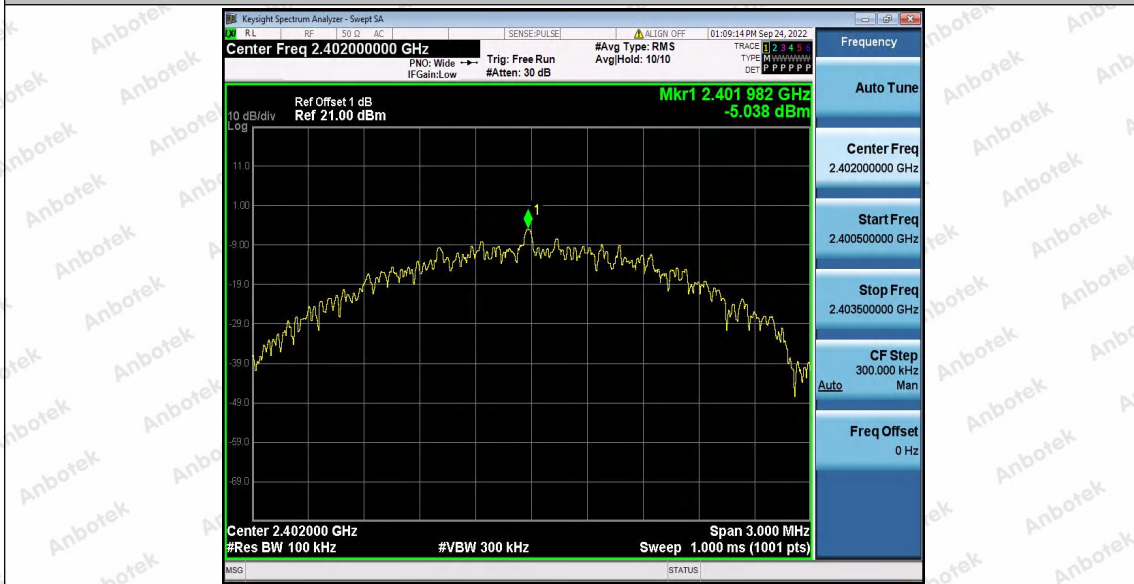
BLE_2M_Ant1_2402_30~100
