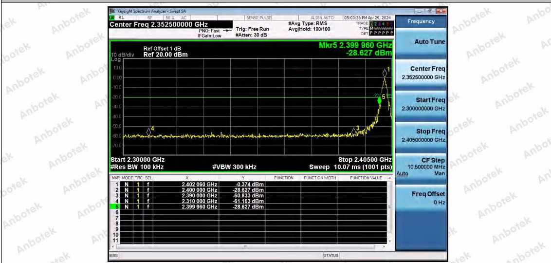
BLE_2M-Ant1-2402-PASS
