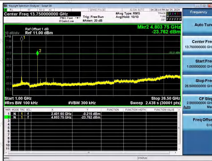
BLE_1M-Ant1-2402-1000~26500-PASS
