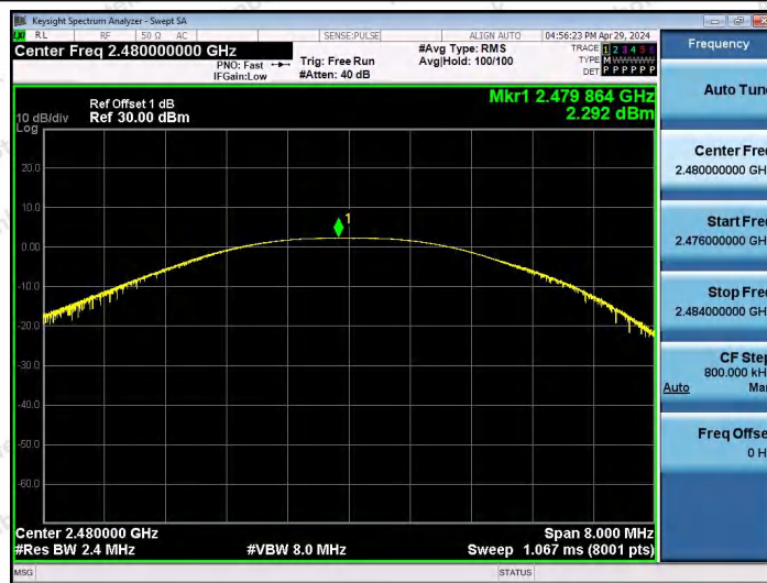
BLE_1M-Ant1-2480-PASS
