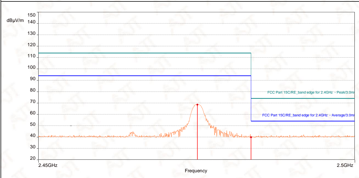
2475MHz Vertical
