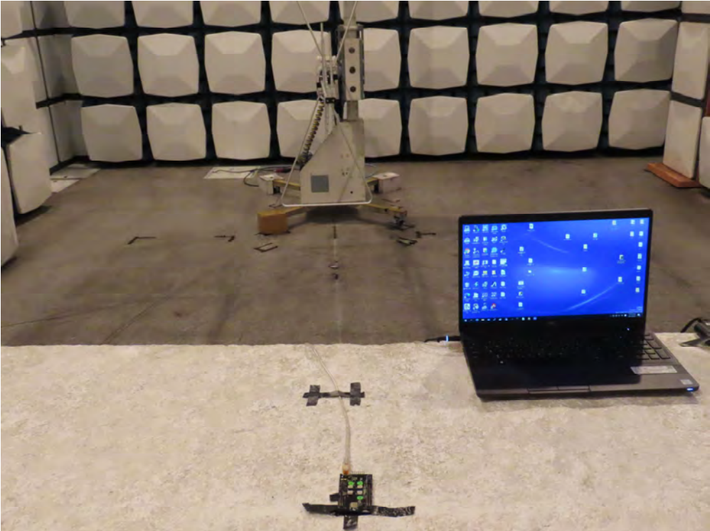
Test Fixture
