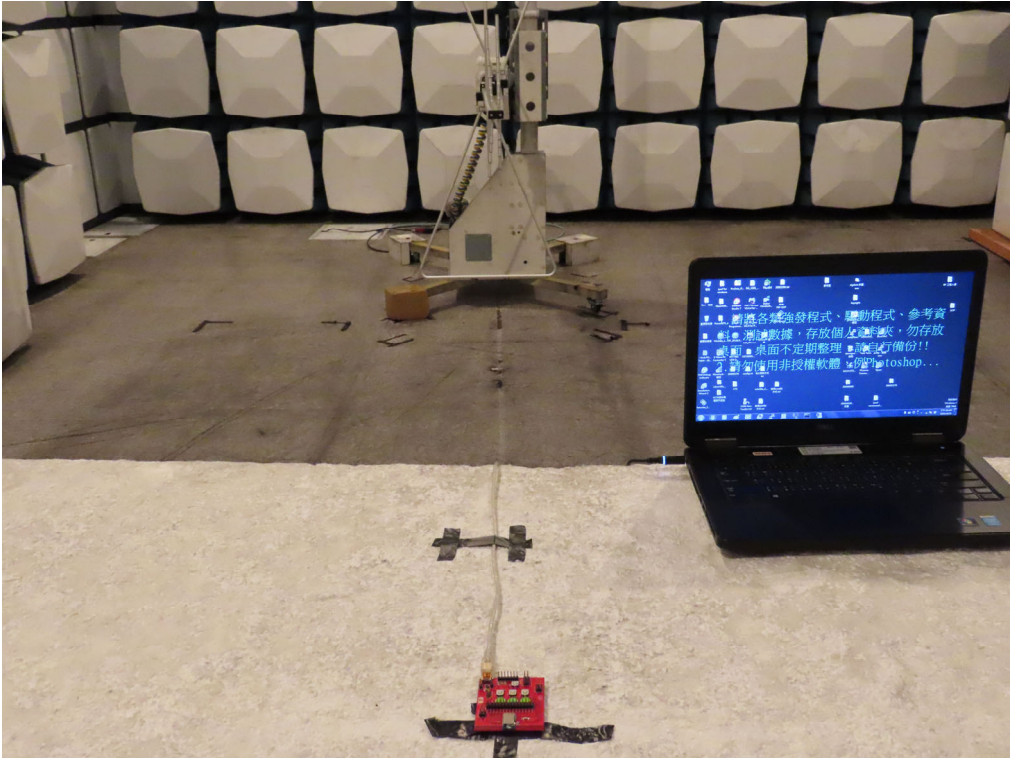
Test Fixture
