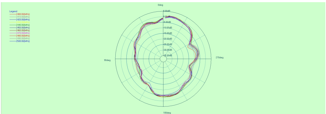
Figure 4: Theta=90°
