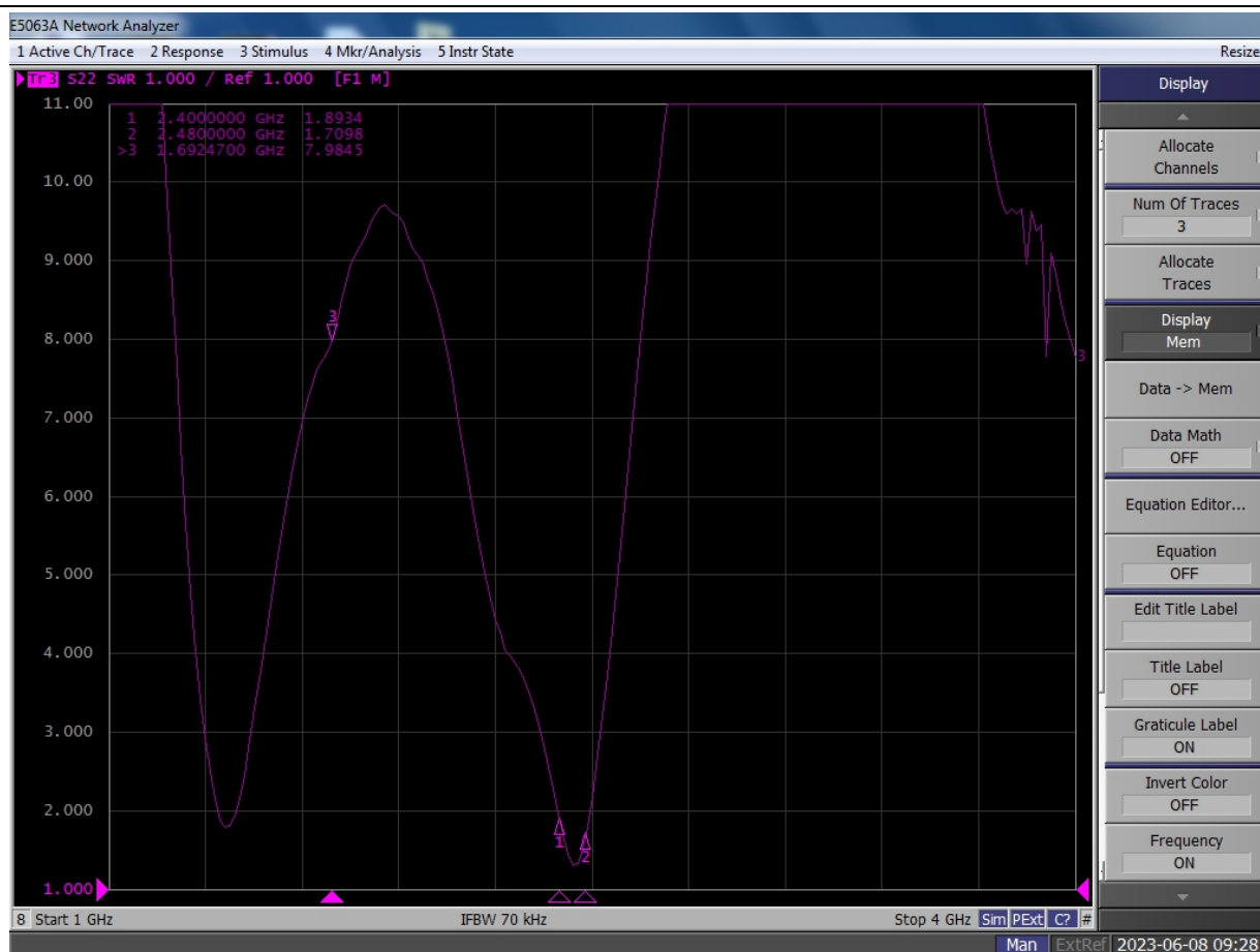
Figure 3: SWR
