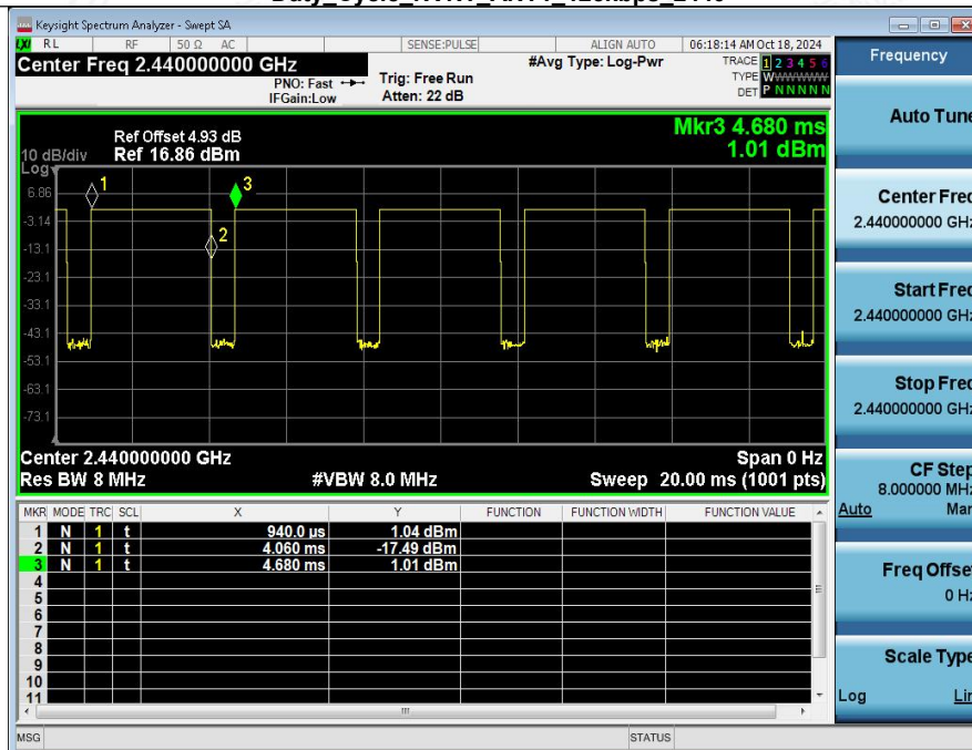
Duty_Cycle_NVNT_ANT1_125kbps_2440
