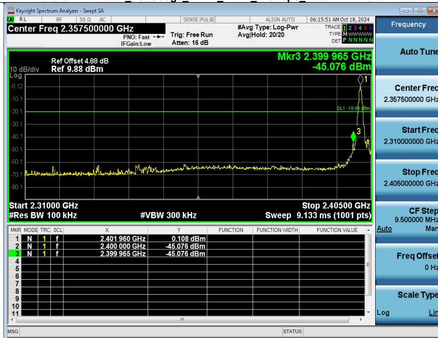
2_Bandedge_NVNT_ANT1_125kbps_2402
