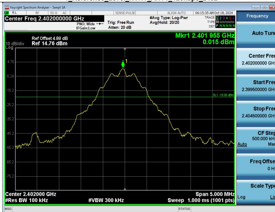
2_Spurious_Emission_NVNT_ANT1_125kbps_2402
