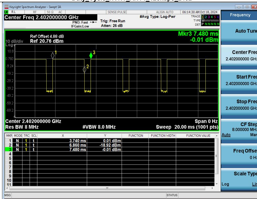
Duty_Cycle_NVNT_ANT1_125kbps_2402
