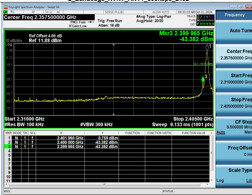
2_Bandedge_NVNT_ANT1_500kbps_2402
