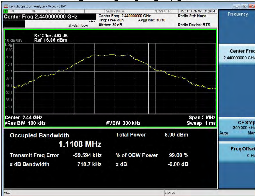
-6dB_Bandwidth_NVNT_ANT1_1Mbps_2440
