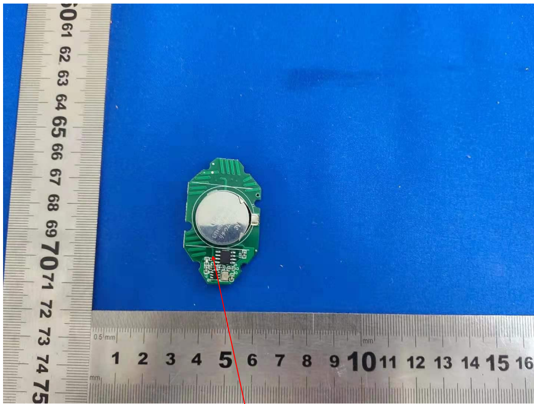
PCB antenna
