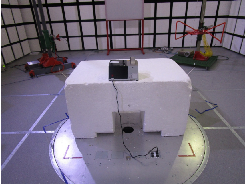
RADIATED SPURIOUS BL1G BACK PHOTO
