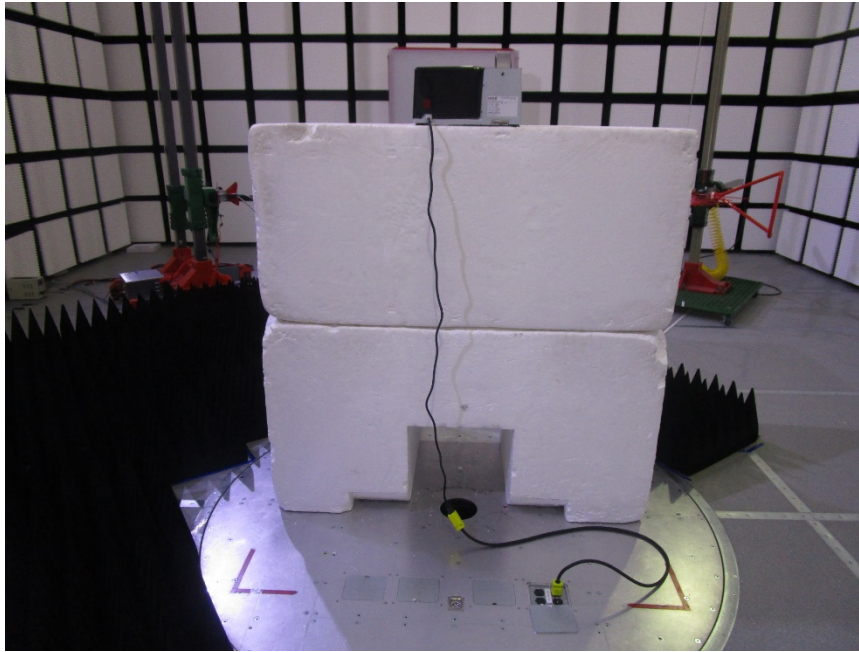
RADIATED SPURIOUS A1G BACK PHOTO
