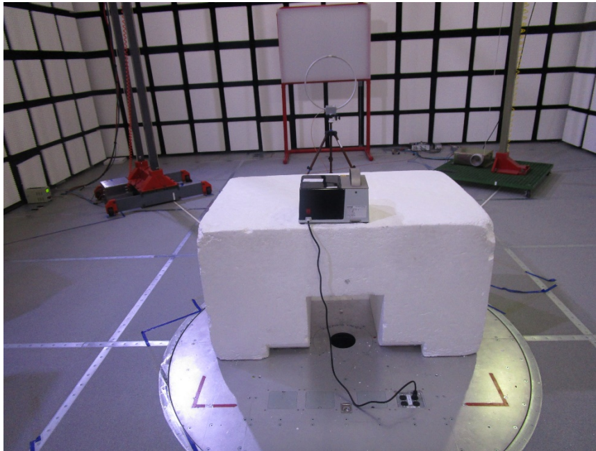
RADIATED SPURIOUS BL30M BACK PHOTO
