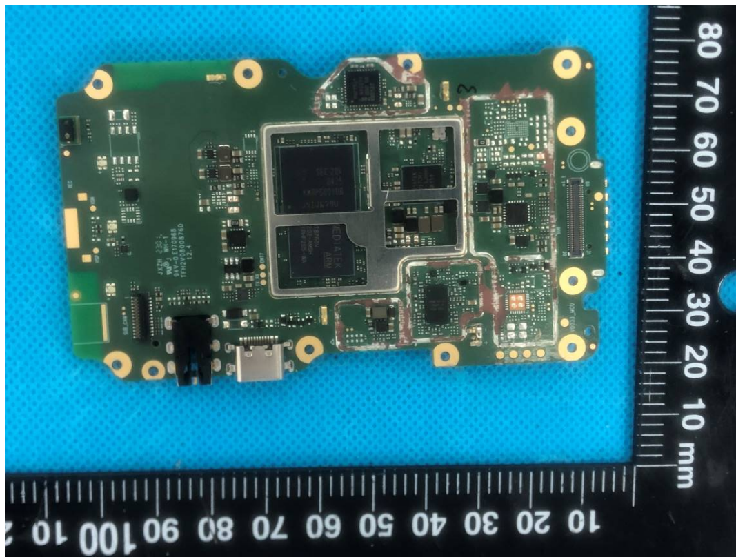
2G 3G 4G Chip
