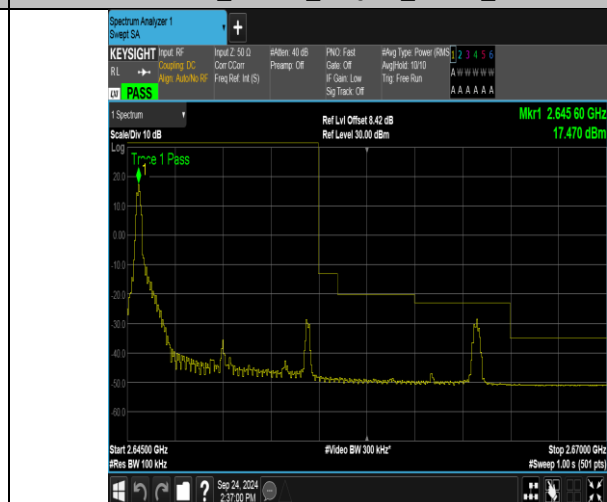
Band41_10MHz_16QAM_41190_1RB#0
