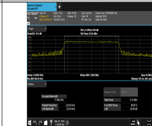
Band41(2535-2655)-20MHz-16QAM-41140-100RB#0-PASS
