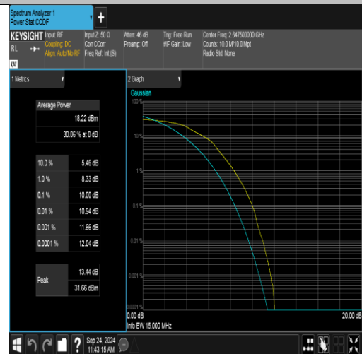
Band41(2535-2655)-15MHz-16QAM-41165-75RB#0-PASS
