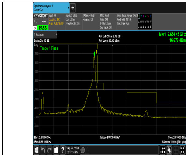
Band41_10MHz_16QAM_41190_1RB#49
