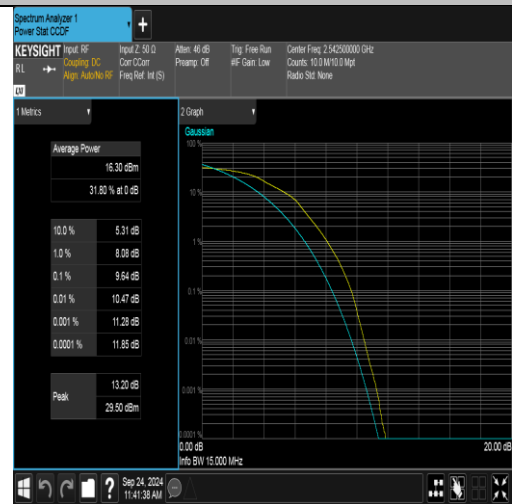
Band41(2535-2655)-15MHz-16QAM-40115-75RB#0-PASS
