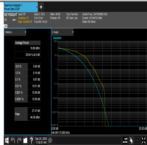
Band41(2535-2655)-15MHz-16QAM-41165-1RB#0-PASS
