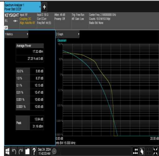
Band41(2535-2655)-15MHz-16QAM-40590-1RB#0-PASS
