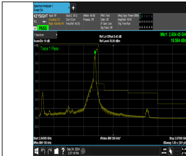
Band41_10MHz_QPSK_41190_1RB#49
