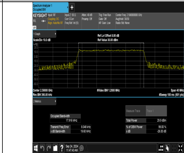
Band41(2535-2655)-20MHz-16QAM-40590-100RB#0-PASS
