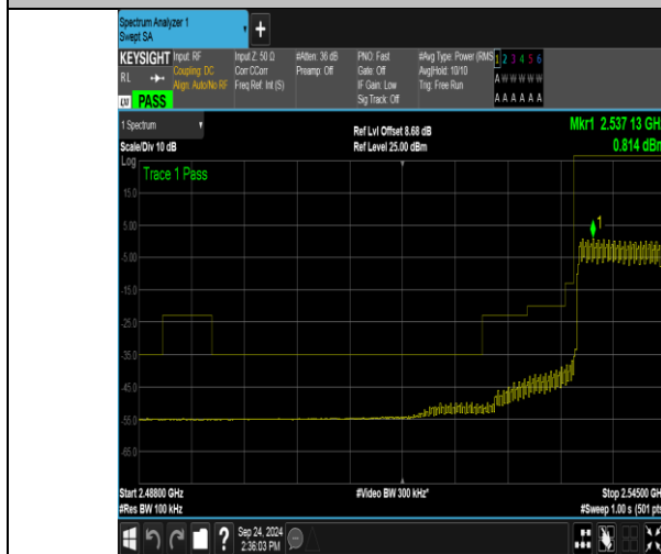
Band41_10MHz_QPSK_40090_50RB#0
