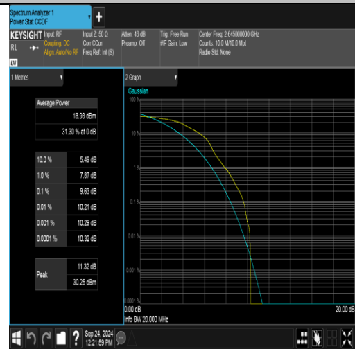
Band41(2535-2655)-20MHz-16QAM-41140-1RB#0-PASS
