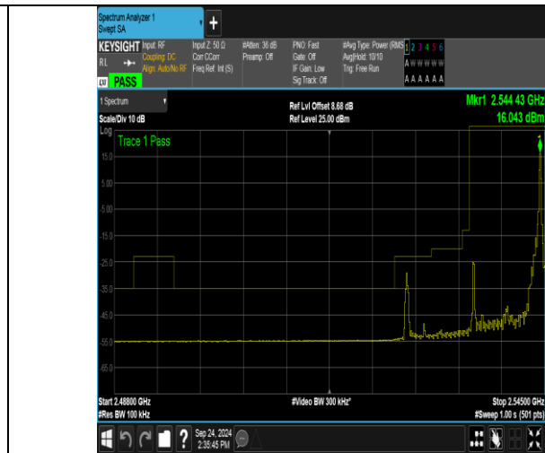
Band41_10MHz_16QAM_40090_1RB#49
