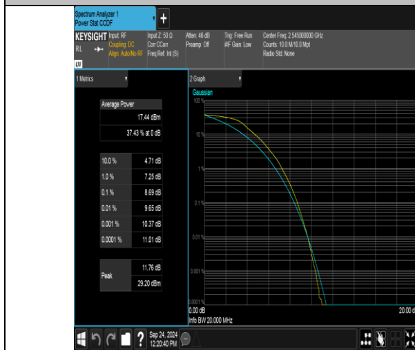
Band41(2535-2655)-20MHz-QPSK-40140-100RB#0-PASS
