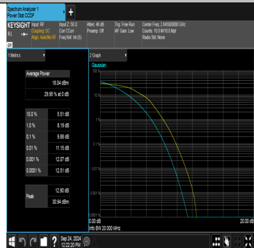
Band41(2535-2655)-20MHz-16QAM-41140-100RB#0-PASS
