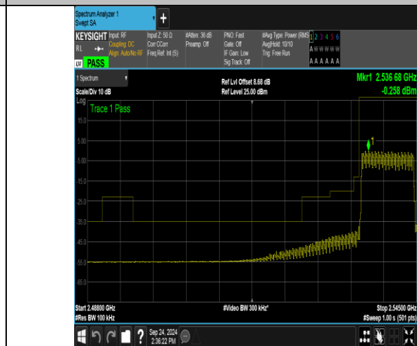
Band41_10MHz_16QAM_40090_50RB#0
