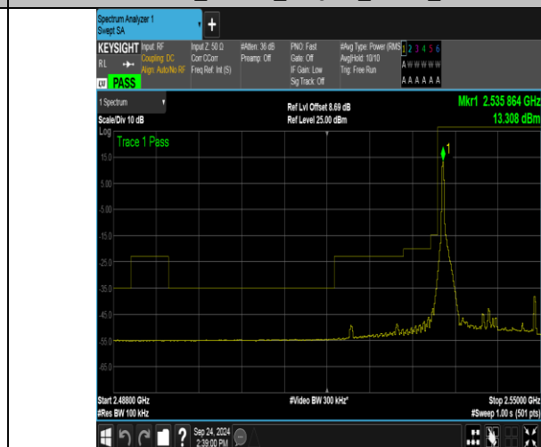
Band41_15MHz_16QAM_40115_1RB#0
