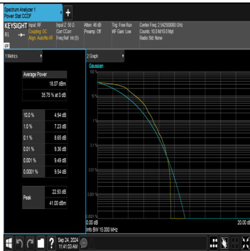
Band41(2535-2655)-15MHz-QPSK-40115-1RB#0-PASS
