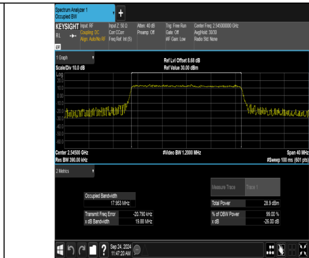
Band41(2535-2655)-20MHz-16QAM-40140-100RB#0-PASS
