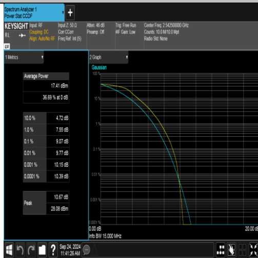
Band41(2535-2655)-15MHz-QPSK-40115-75RB#0-PASS
