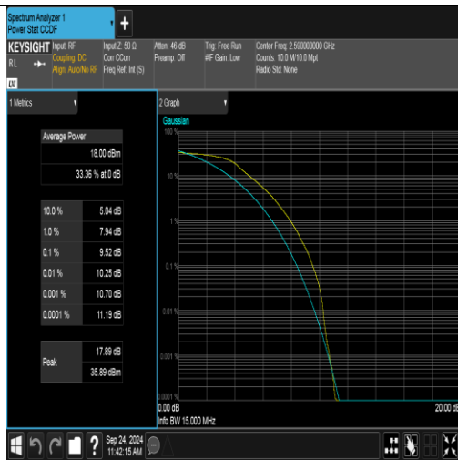
Band41(2535-2655)-15MHz-QPSK-40590-75RB#0-PASS
