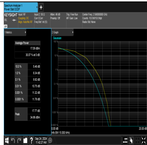
Band41(2535-2655)-15MHz-16QAM-40590-75RB#0-PASS
