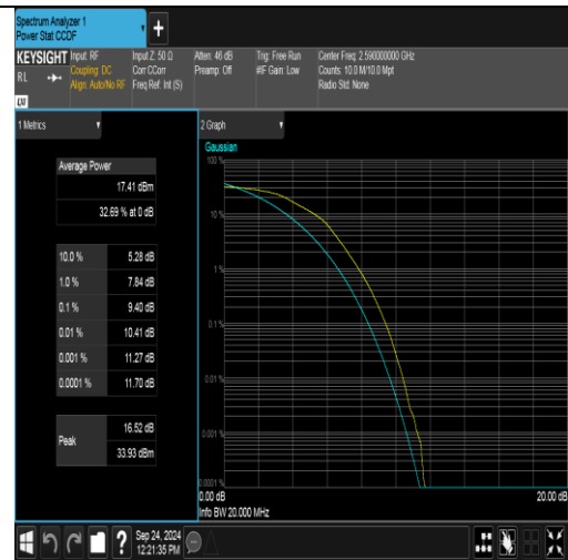
Band41(2535-2655)-20MHz-16QAM-40590-100RB#0-PASS
