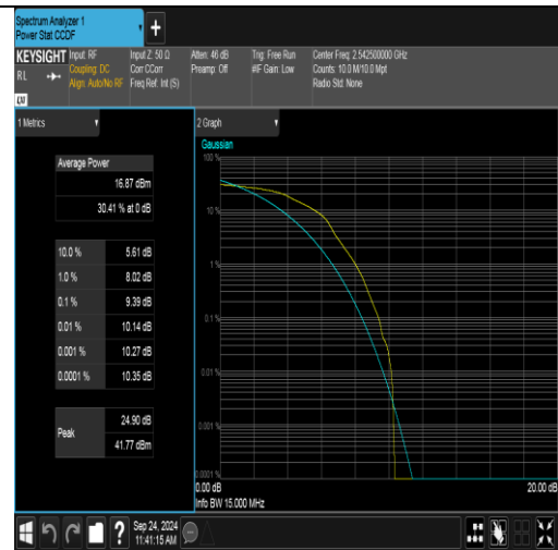
Band41(2535-2655)-15MHz-16QAM-40115-1RB#0-PASS
