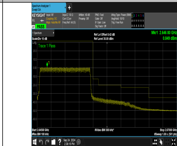
Band41_10MHz_16QAM_41190_50RB#0
