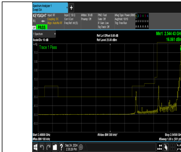
Band41_10MHz_QPSK_40090_1RB#49
