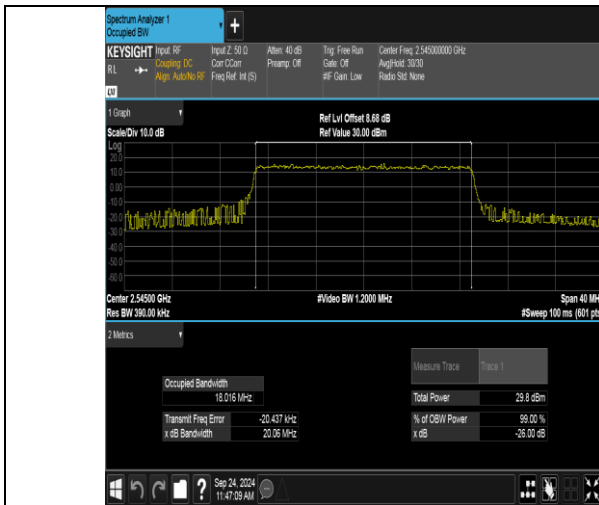
Band41(2535-2655)-20MHz-QPSK-40140-100RB#0-PASS
