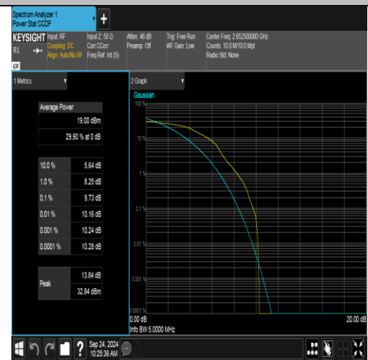
Band41(2535-2655)-5MHz-16QAM-41215-1RB#0-PASS
