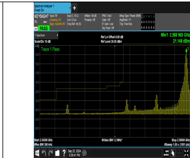
Band38_20MHz_16QAM_37850_1RB#99
