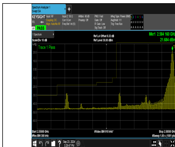
Band38_15MHz_QPSK_37825_1RB#74
