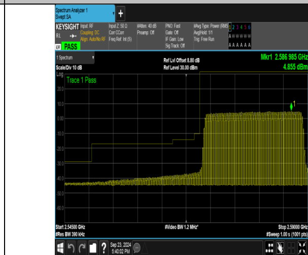
Band38_20MHz_16QAM_37850_100RB#0
