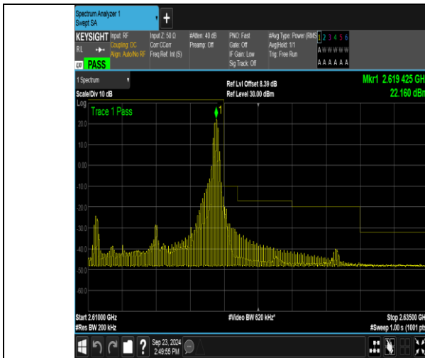
Band38_10MHz_QPSK_38200_1RB#49
