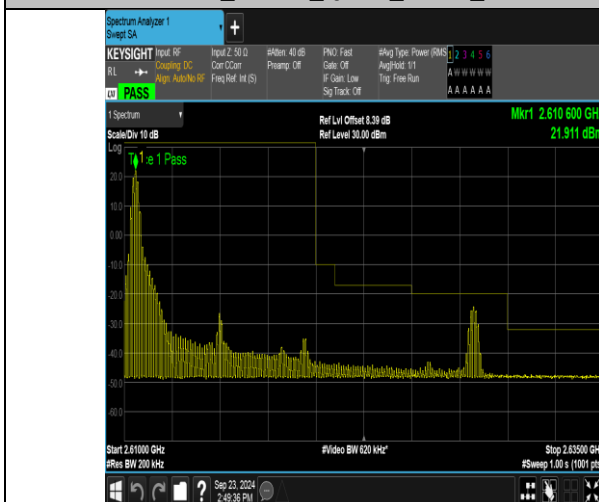
Band38_10MHz_QPSK_38200_1RB#0
