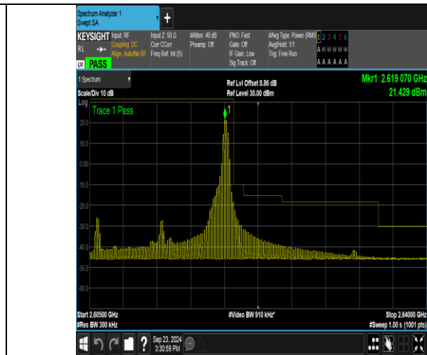
Band38_15MHz_16QAM_38175_1RB#74
