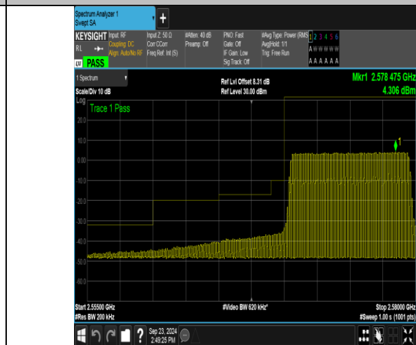
Band38_10MHz_16QAM_37800_50RB#0
