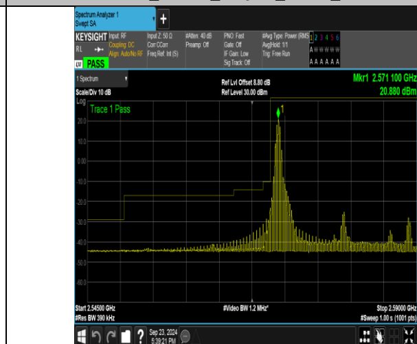
Band38_20MHz_16QAM_37850_1RB#0
