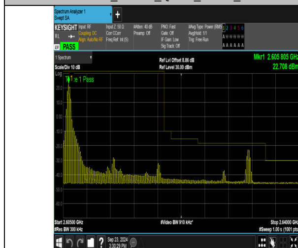
Band38_15MHz_QPSK_38175_1RB#0
