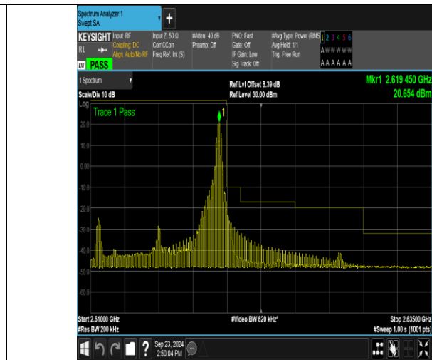
Band38_10MHz_16QAM_38200_1RB#49
