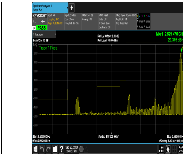
Band38_10MHz_QPSK_37800_1RB#49
