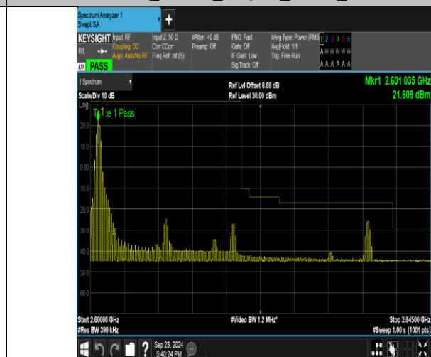
Band38_20MHz_16QAM_38150_1RB#0
