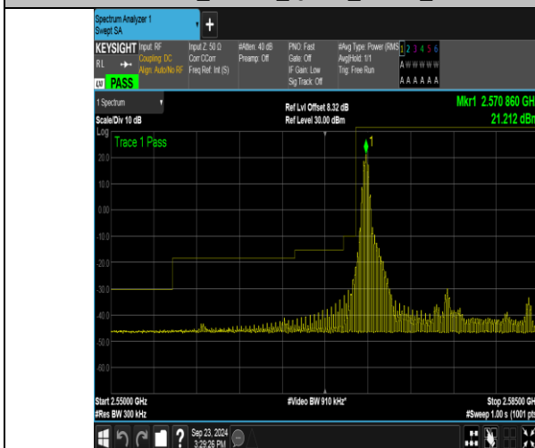
Band38_15MHz_QPSK_37825_1RB#0
