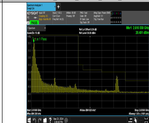
Band38_10MHz_16QAM_38200_1RB#0
