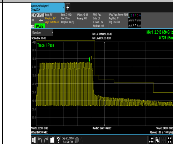
Band38_15MHz_16QAM_38175_75RB#0
