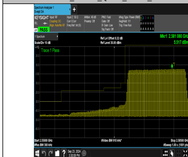
Band38_15MHz_QPSK_37825_75RB#0
