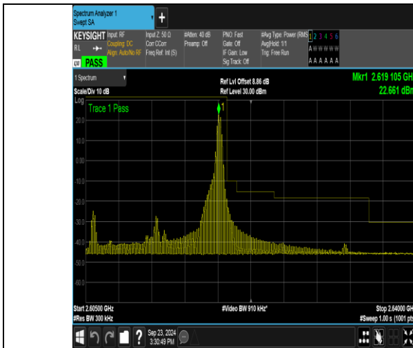
Band38_15MHz_QPSK_38175_1RB#74
