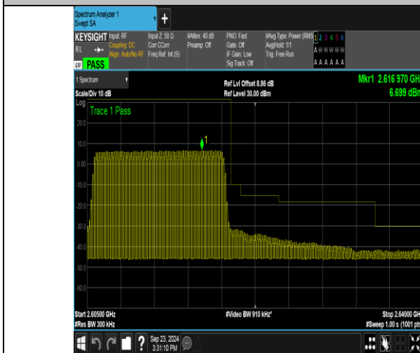
Band38_15MHz_QPSK_38175_75RB#0
