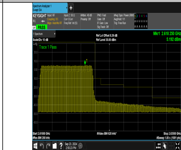
Band38_10MHz_16QAM_38200_50RB#0
