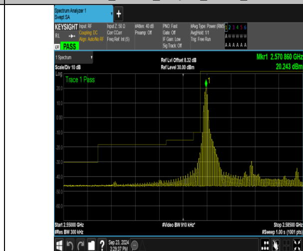
Band38_15MHz_16QAM_37825_1RB#0
