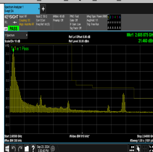
Band38_15MHz_16QAM_38175_1RB#0
