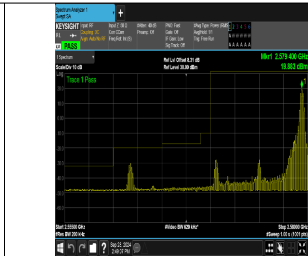
Band38_10MHz_16QAM_37800_1RB#49
