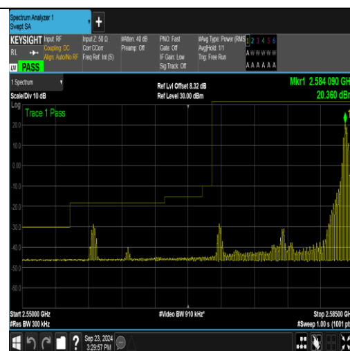
Band38_15MHz_16QAM_37825_1RB#74
