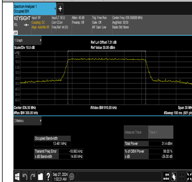
Band26(824-849)-15MHz-QPSK-26915-75RB#0-PASS
