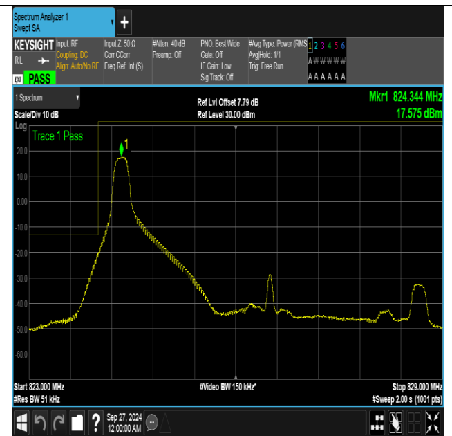
Band26_5MHz_16QAM_26815_1RB#0
