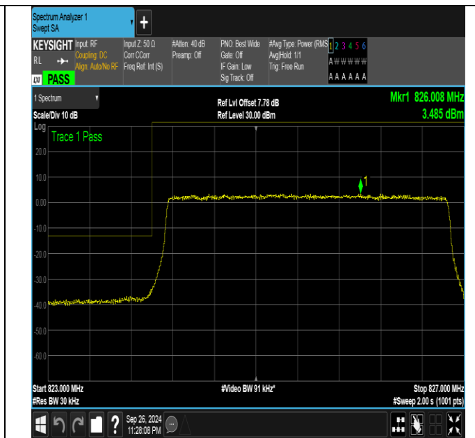
Band26_3MHz_16QAM_26805_15RB#0
