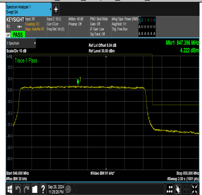
Band26_3MHz_16QAM_27025_15RB#0
