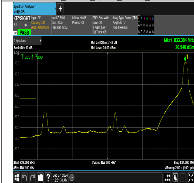
Band26_10MHz_QPSK_26840_1RB#49
