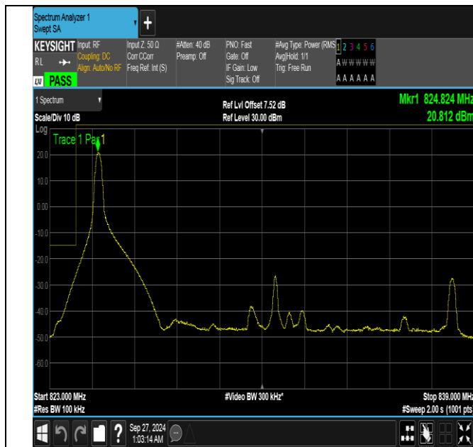
Band26_15MHz_QPSK_26865_1RB#0
