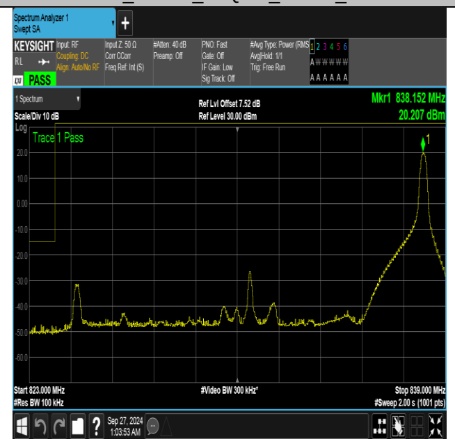
Band26_15MHz_16QAM_26865_1RB#74
