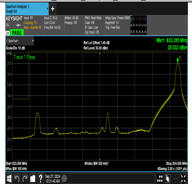
Band26_10MHz_16QAM_26840_1RB#49
