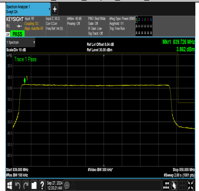
Band26_10MHz_16QAM_26990_50RB#0
