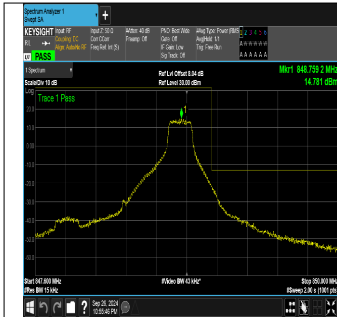
Band26_1.4MHz_QPSK_27033_1RB#5
