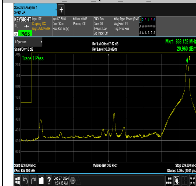
Band26_15MHz_QPSK_26865_1RB#74
