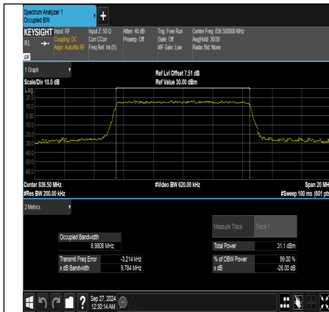
Band26(824-849)-10MHz-QPSK-26915-50RB#0-PASS
