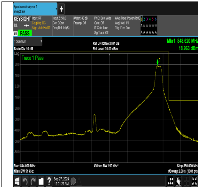
Band26_5MHz_QPSK_27015_1RB#24
