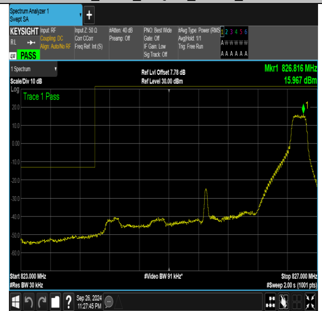
Band26_3MHz_16QAM_26805_1RB#14
