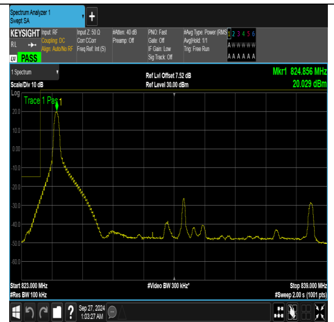
Band26_15MHz_16QAM_26865_1RB#0
