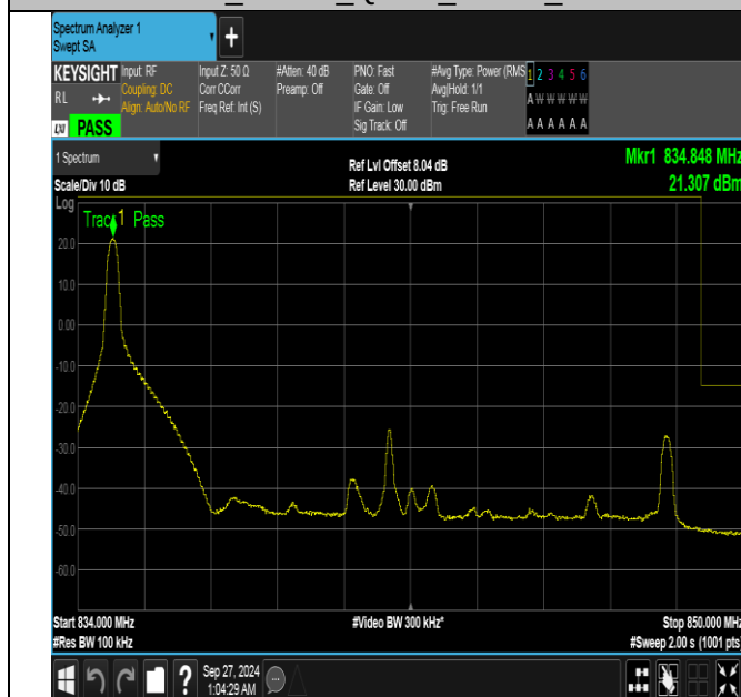
Band26_15MHz_QPSK_26965_1RB#0
