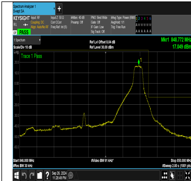
Band26_3MHz_QPSK_27025_1RB#14
