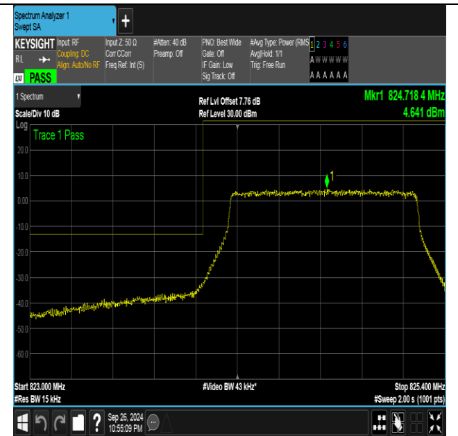
Band26_1.4MHz_16QAM_26797_6RB#0
