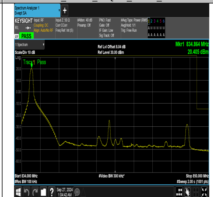
Band26_15MHz_16QAM_26965_1RB#0
