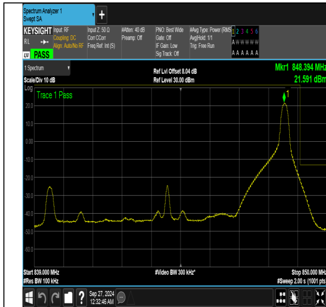
Band26_10MHz_QPSK_26990_1RB#49
