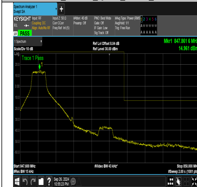
Band26_1.4MHz_QPSK_27033_1RB#0
