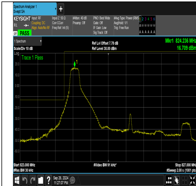
Band26_3MHz_QPSK_26805_1RB#0
