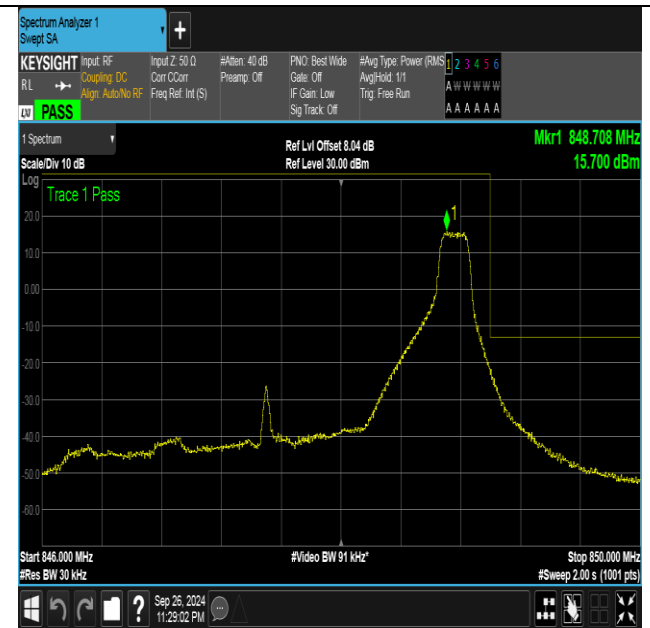
Band26_3MHz_16QAM_27025_1RB#14
