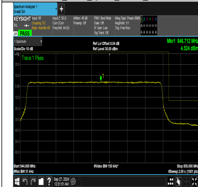
Band26_5MHz_QPSK_27015_25RB#0
