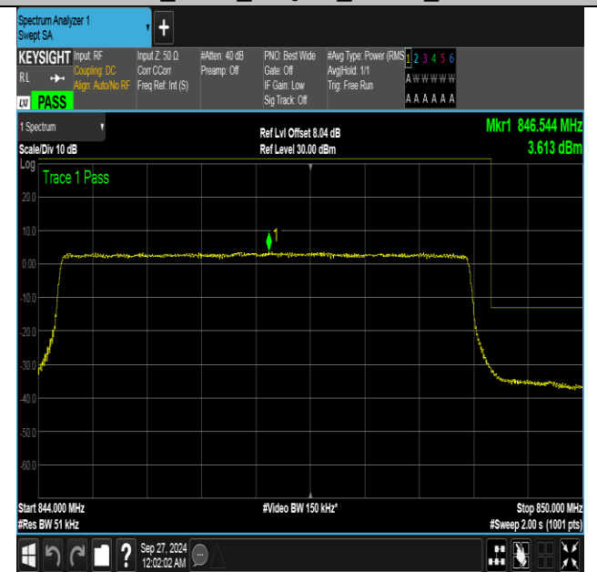
Band26_5MHz_16QAM_27015_25RB#0
