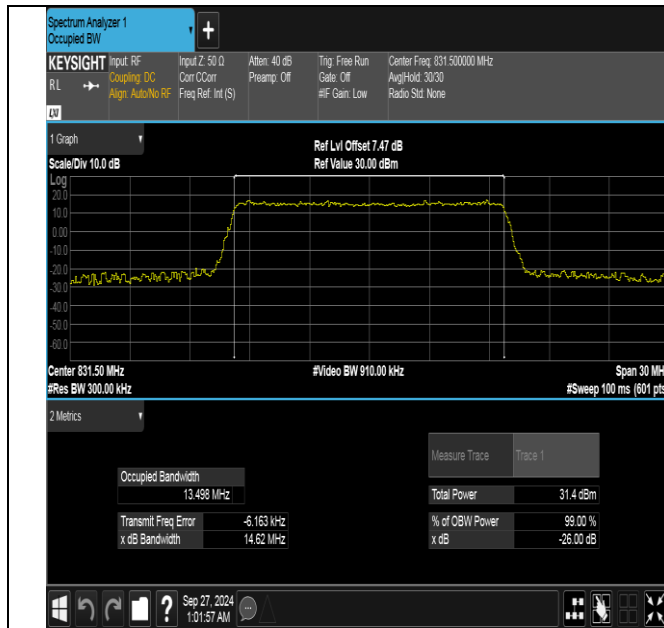
Band26(824-849)-15MHz-QPSK-26865-75RB#0-PASS
