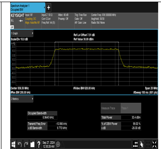
Band26(824-849)-10MHz-16QAM-26915-50RB#0-PASS
