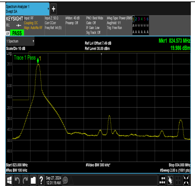
Band26_10MHz_16QAM_26840_1RB#0
