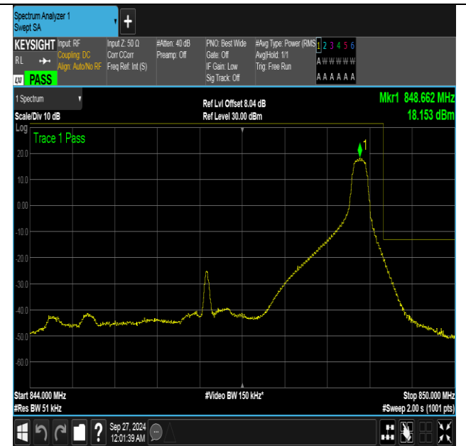
Band26_5MHz_16QAM_27015_1RB#24
