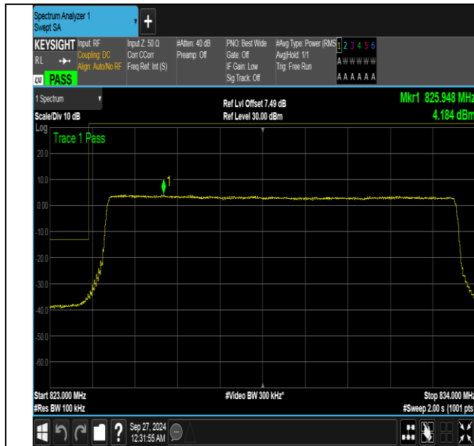
Band26_10MHz_QPSK_26840_50RB#0
