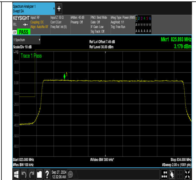
Band26_10MHz_16QAM_26840_50RB#0
