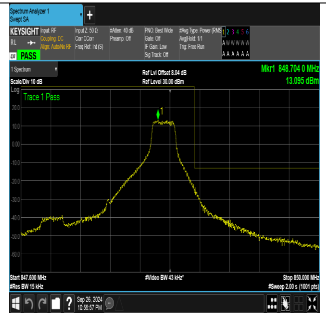
Band26_1.4MHz_16QAM_27033_1RB#5
