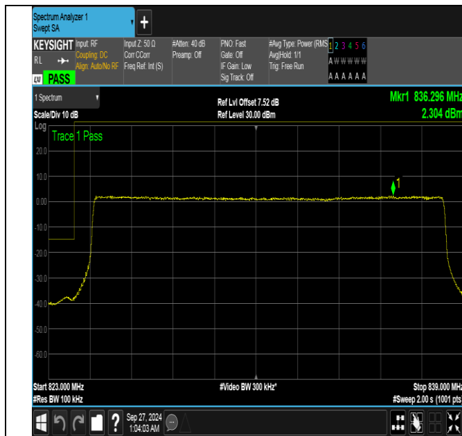
Band26_15MHz_QPSK_26865_75RB#0
