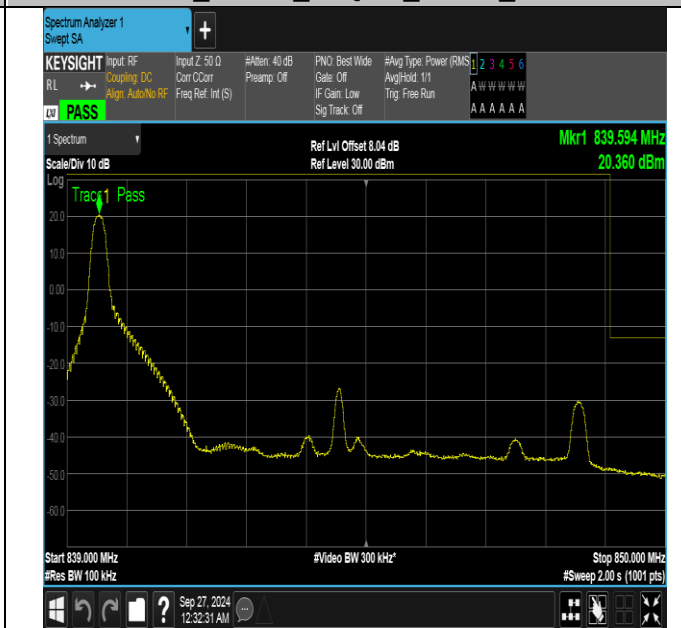
Band26_10MHz_16QAM_26990_1RB#0
