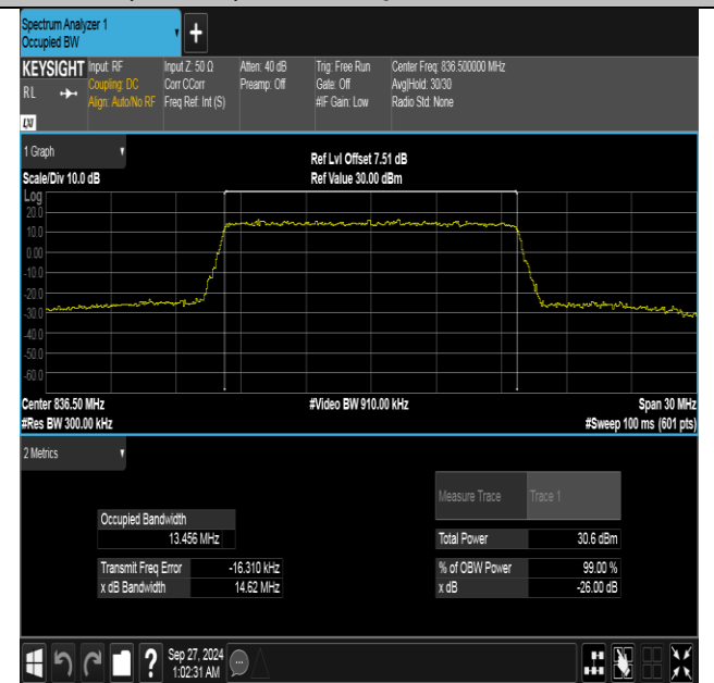
Band26(824-849)-15MHz-16QAM-26915-75RB#0-PASS
