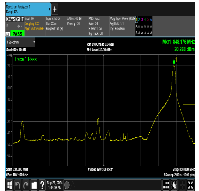
Band26_15MHz_16QAM_26965_1RB#74
