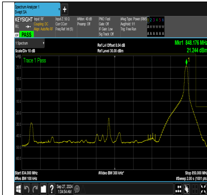
Band26_15MHz_QPSK_26965_1RB#74
