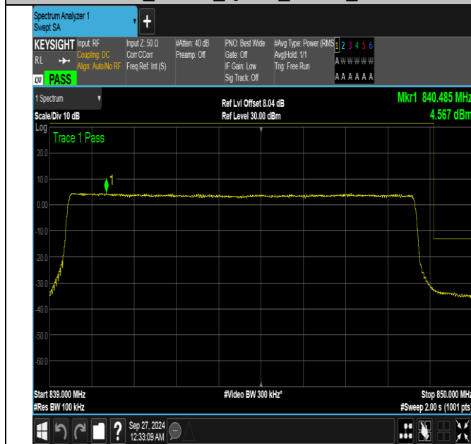
Band26_10MHz_QPSK_26990_50RB#0
