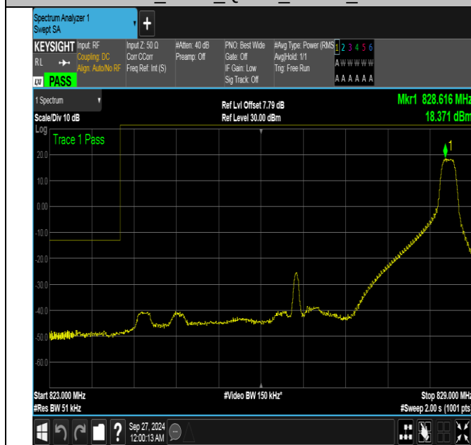
Band26_5MHz_QPSK_26815_1RB#24
