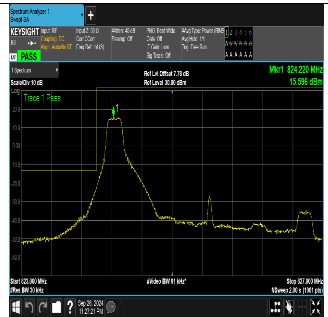
Band26_3MHz_16QAM_26805_1RB#0
