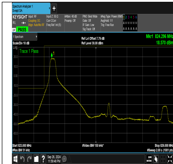
Band26_5MHz_QPSK_26815_1RB#0
