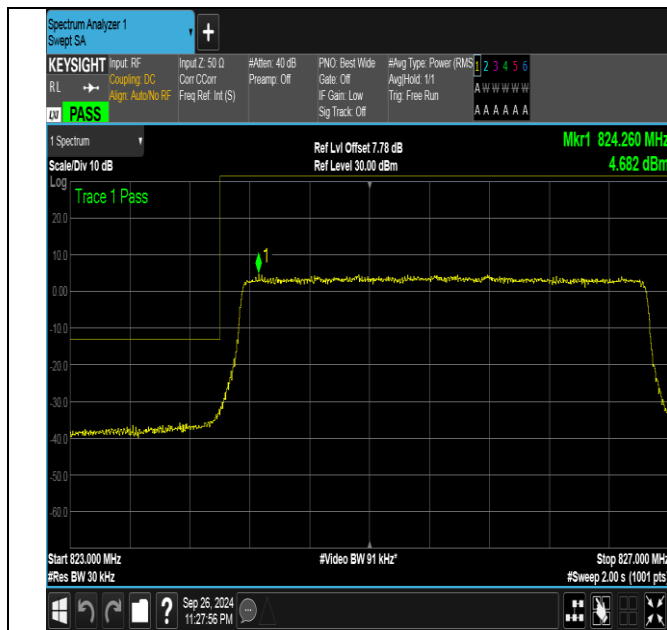
Band26_3MHz_QPSK_26805_15RB#0
