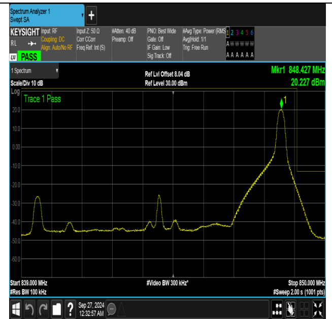
Band26_10MHz_16QAM_26990_1RB#49
