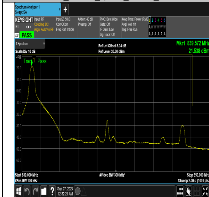
Band26_10MHz_QPSK_26990_1RB#0
