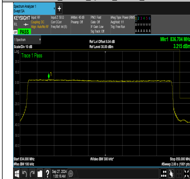
Band26_15MHz_QPSK_26965_75RB#0
