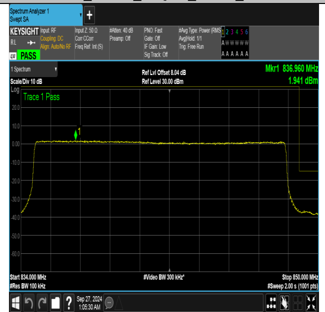
Band26_15MHz_16QAM_26965_75RB#0
