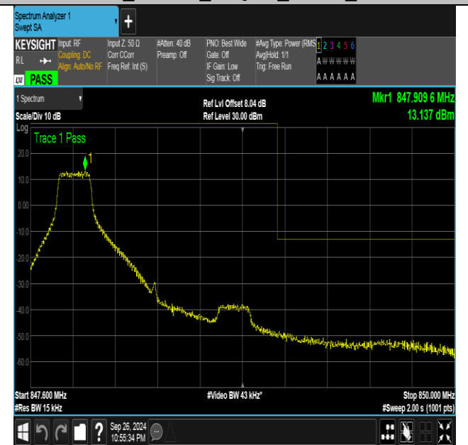
Band26_1.4MHz_16QAM_27033_1RB#0
